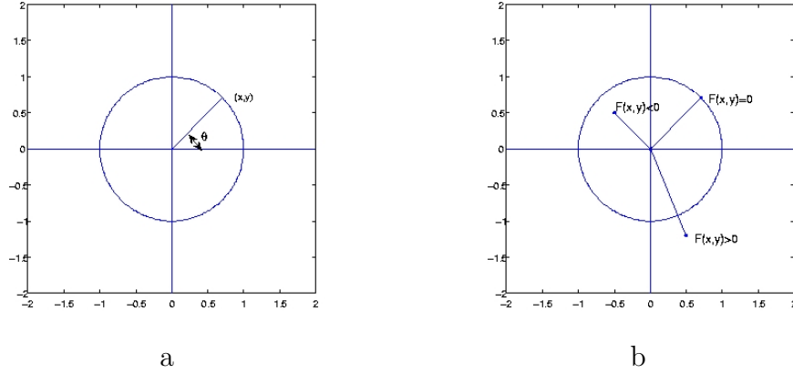
Figure 2-5: The unit circle, a) an explicit representation, b) an implicit representation.
