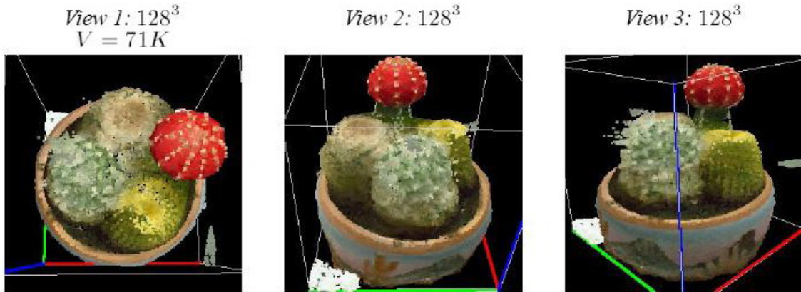
Figure 6–24: Cactus reconstruction by approximate space carving. Reprinted from Kutulakos [89] with permission, ©2000 Springer-Verlag.
