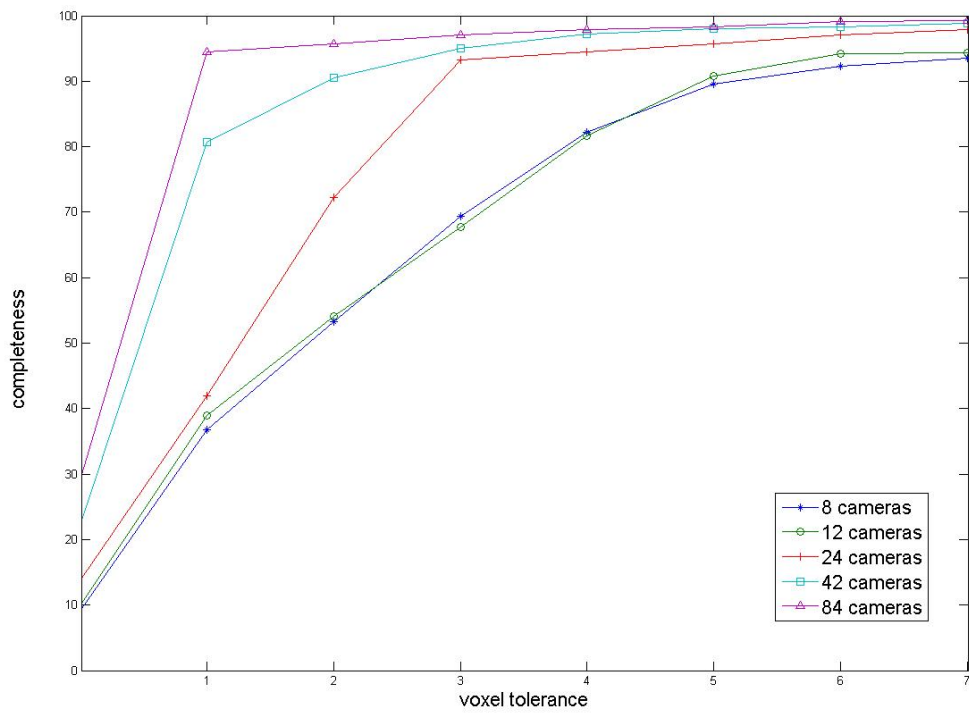
Figure 6–28: Surface voxel completeness within n-voxel tolerance for the deer data set.
