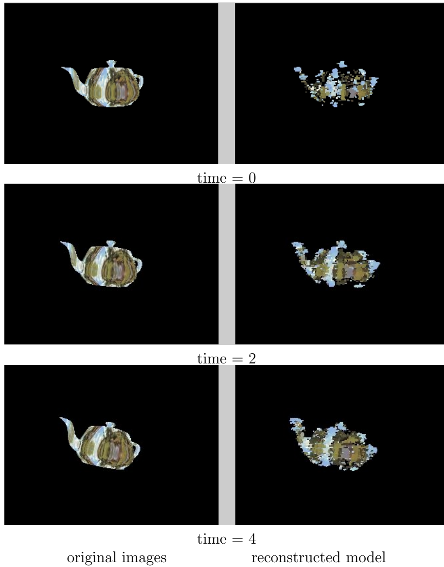
Figure 7-2: Model updating. The images from one camera (of a total of 24) at different times are shown here. The object undergoes both translation and rotation. The reconstructed models are projected to the same camera position.
