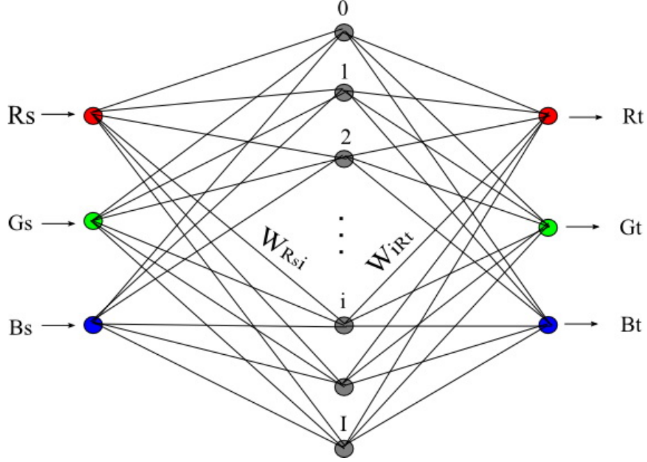
Figure 3–3: the BPNN architecture
