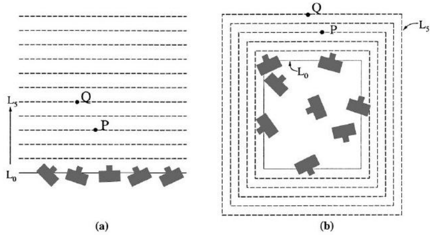
Figure 2-11: Two one-pass point scan examples. Reprinted from Seitz and Dyer [141] with permission.
