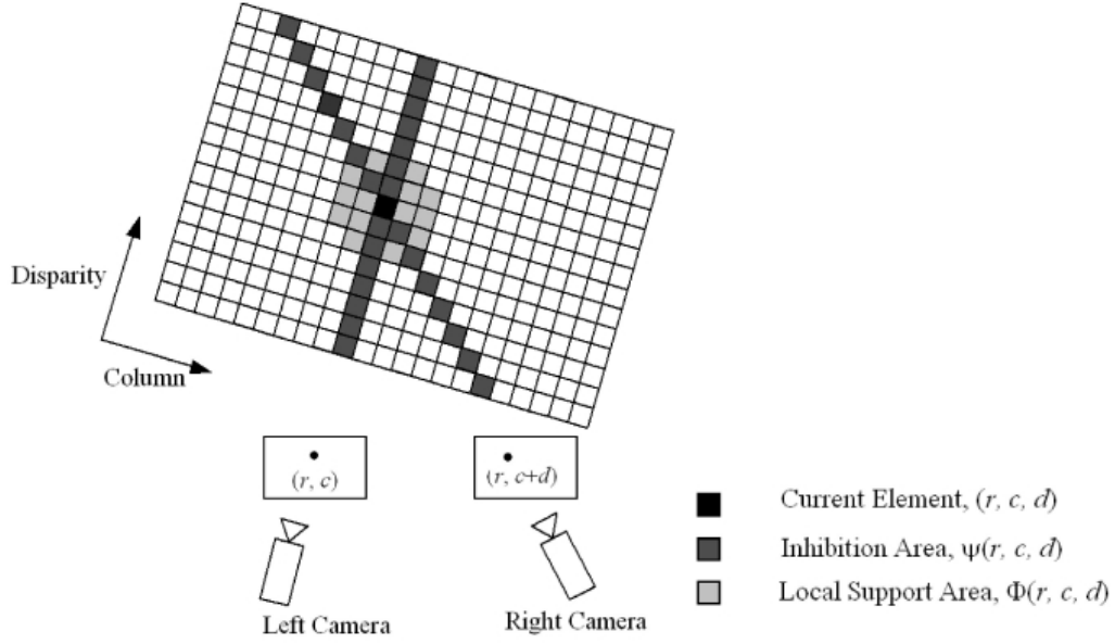
Figure 2–2: 2D slice of the 3D disparity space. The current element is shown in black. The inhibitory regions are designed to constrain the element’s disparity to a single value. The support region enhances smoothness, so that neighboring elements have similar disparity values. Reprinted from Zitnick and Kanade [172] with permission, ©2000 IEEE.
