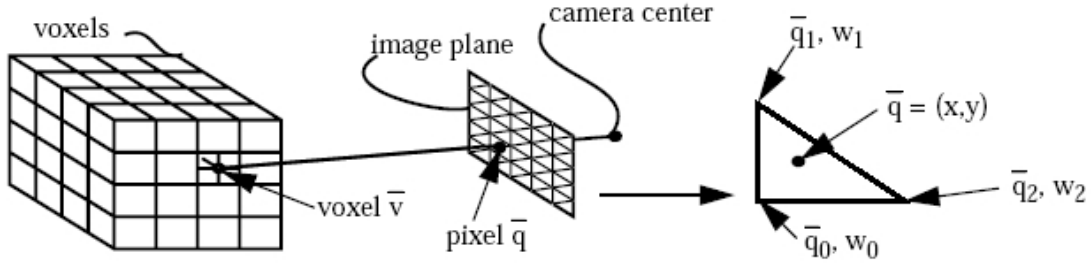
Figure 2–4: Basic operation in computing signed distance. Each voxel is projected into the image plane of each camera using the camera models already computed for stereo. The depth of the voxel can be extracted from this process. The range image is interpolated to compute the depth from the camera to the surface. The signed distance from the voxel to the surface is computed by subtracting these depths. Reprinted from Rander [126] with permission.
