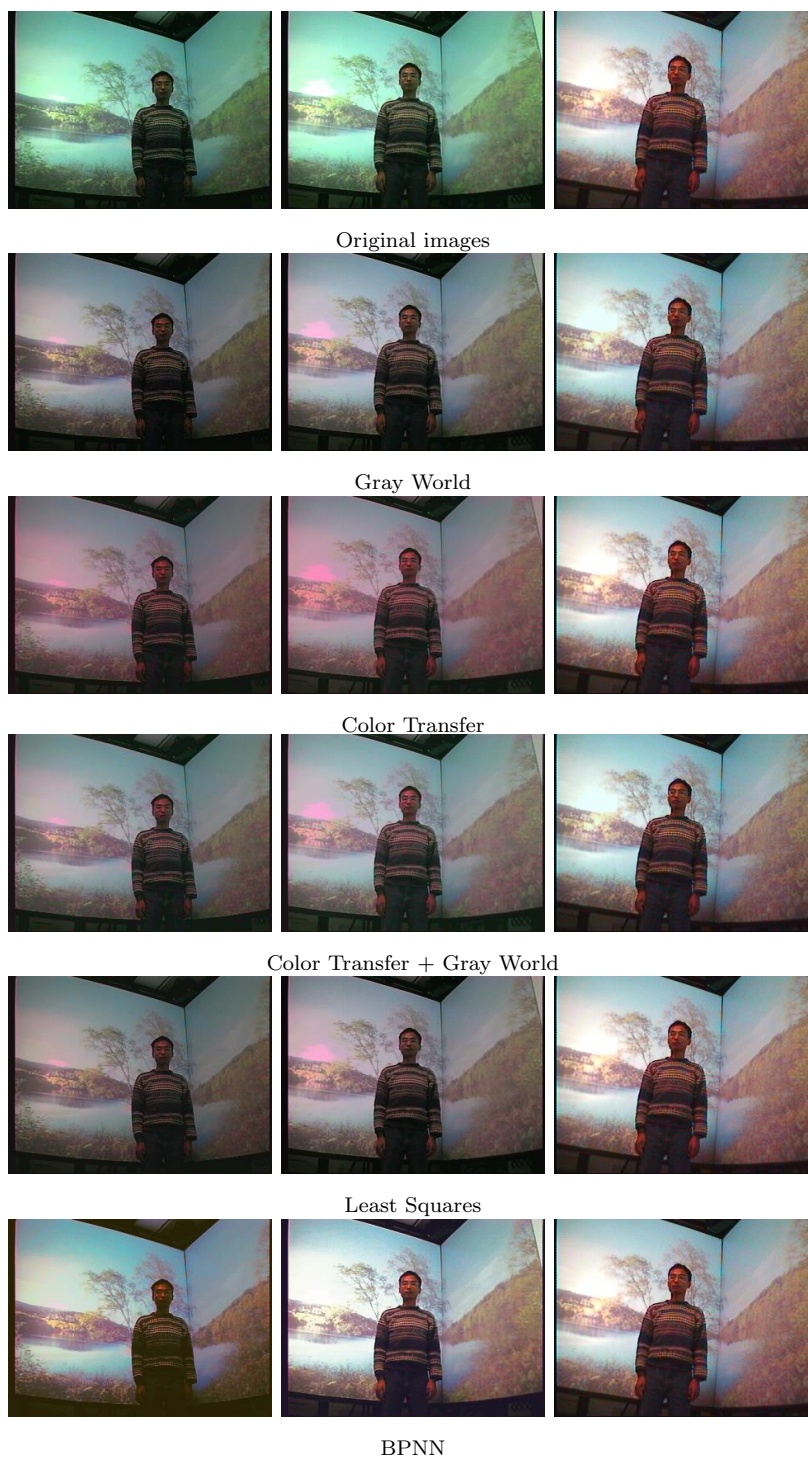
Figure 3–6: Color correction results including a person standing in the scene.
