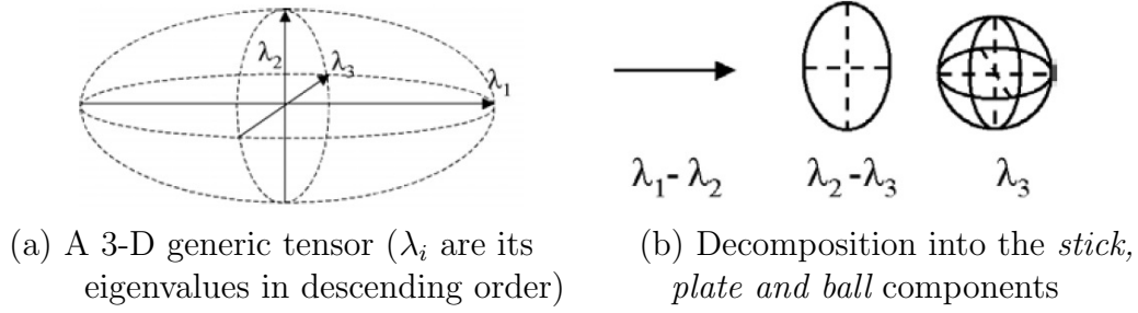
Figure 6-7: A second order generic tensor and its decomposition in 3D. Reprinted from Mordohai [110] with permission.
