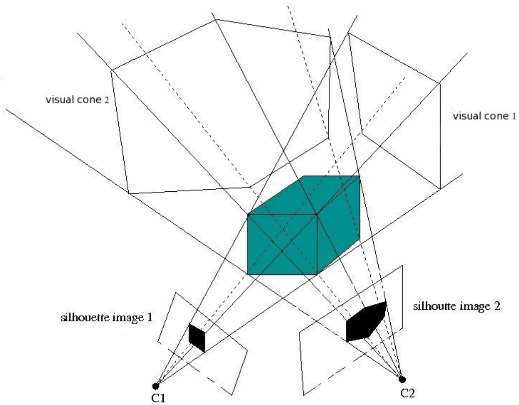
Figure 1–4: Shape from Silhouettes. The shape of an object can be estimated by intersecting the visual cones.
