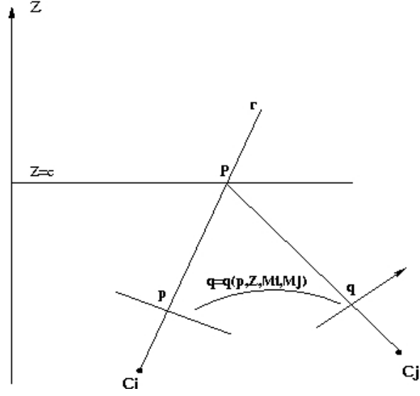
Figure 4-1: Scene point computing and reprojection
