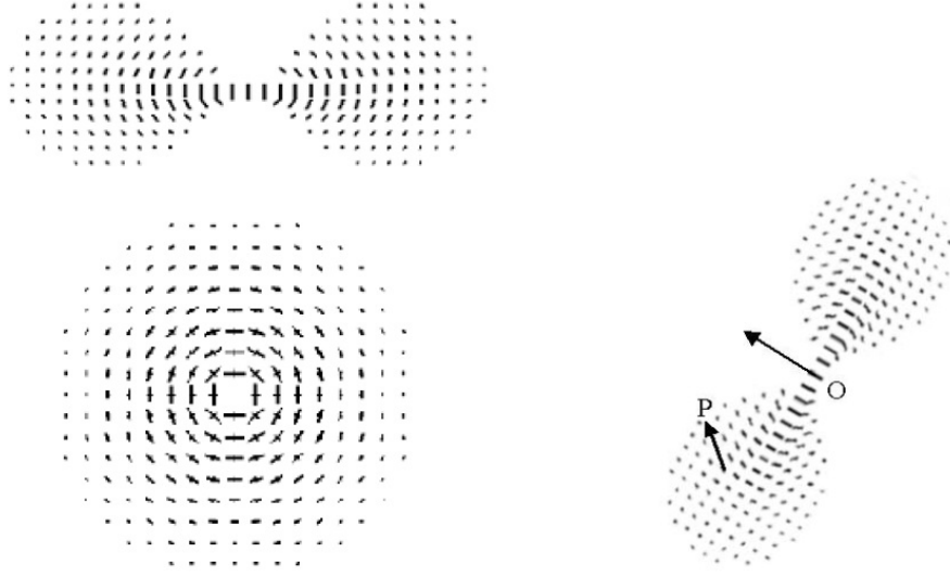
(a) The 2-D stick and ball fields
