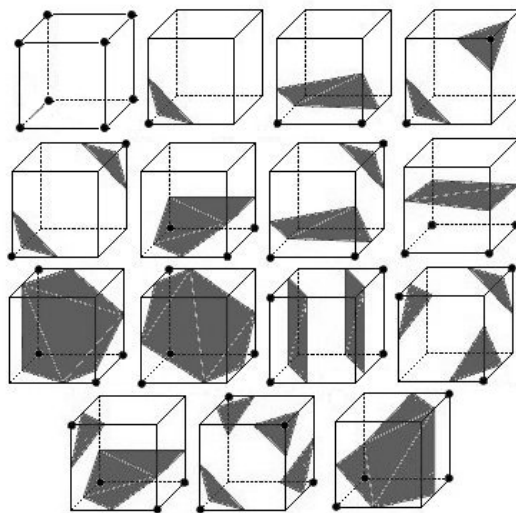
Figure 2–3: The 15 cube combinations for marching cubes.
