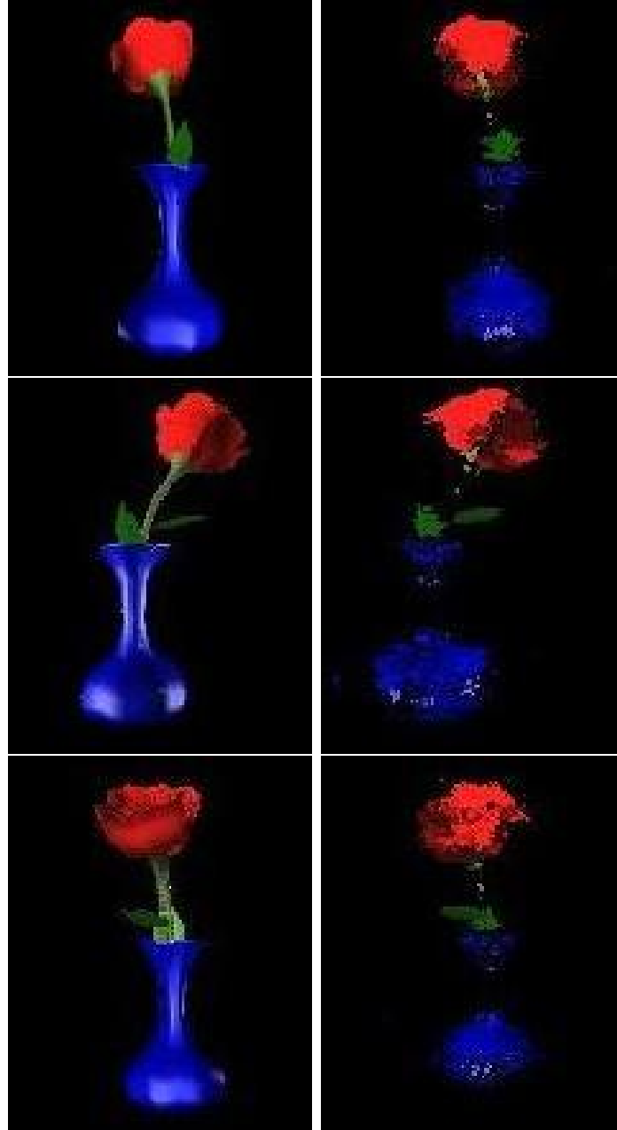
Figure 5–3: Rose reconstruction: volumetric reconstruction based on most frequent color estimation. The first column shows original images, the second column is reconstructed. Twenty four cameras are used, of which three are shown here. The reconstructed models are rendered to the same camera positions for comparison.
