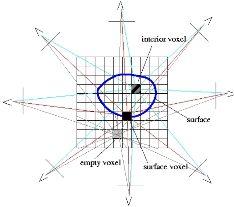
Figure 5-1: Voxel categories.
