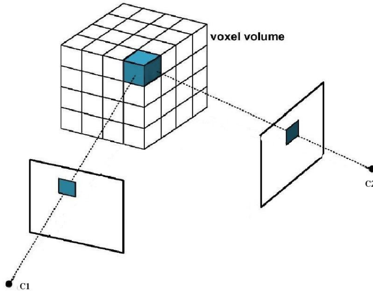
Figure 1-5: Volumetric Reconstruction.
