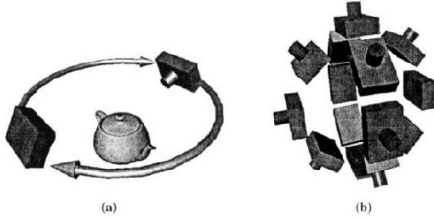
Figure 2-10: Two camera configurations satisfying the ordinal visibility constraint. Reprinted from Seitz and Dyer [141] with permission.
