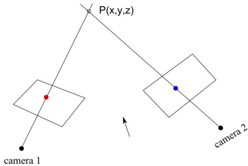
Figure 1-3: Stereo Vision.(a) stereo matching tries to find a pixel along the epipolar line in the right image corresponding to the pixel in the left image; (b) Once a pair of matching pixels is found, the corresponding 3D point P(x,y,z) can be calculated by triangulation.
