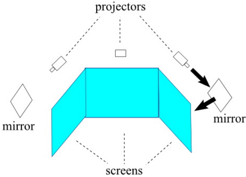
Figure 3-4: Illustration of the rear projection environment used for our application. Images are sent from projectors to mirrors and reflected to screens.
