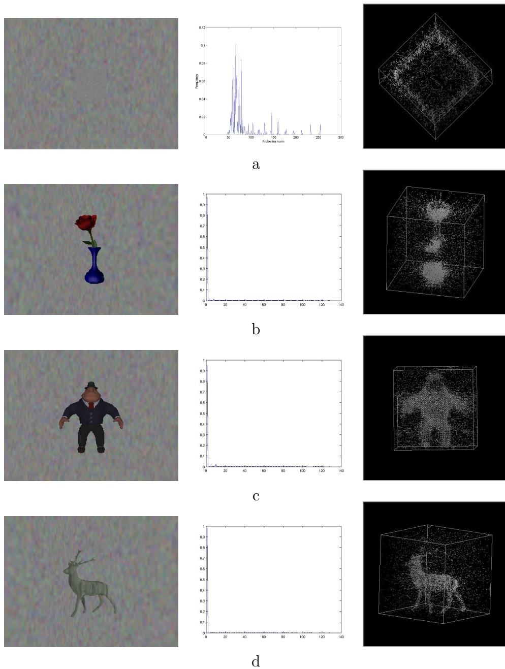
Figure 6-1: Reconstruction based on F-norms. 1st column: one of 24 reference images. 2nd column: histogram of F-norms. 3rd column: initial occupancy. Here, the background are planar screens texture-mapped with a random-color image. In a, the foreground is a synthesized box texture-mapped with the same image as the background, while in b-d, the foregrounds are scanned objects rendered by OpenGL.
