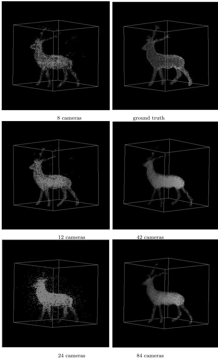
Figure 6–26: Performance of F-norm algorithm with different number of cameras for the deer data set.
