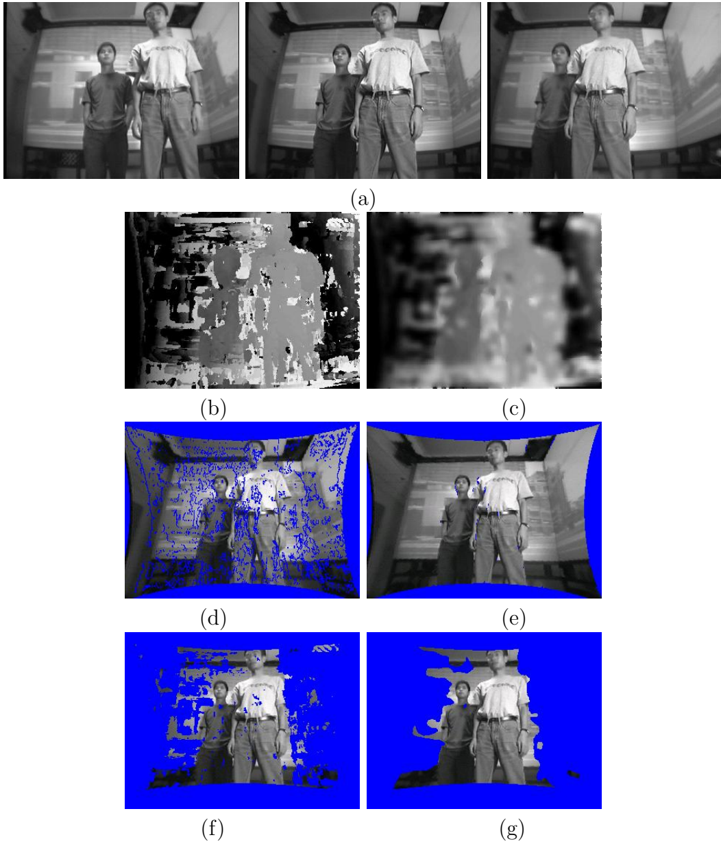
Figure 4-7: (a) original images, (b) depth map, (c) depth map after diffusion, (d) reconstruction based on (b), (e) reconstruction based on (c), (f) segmentation based on (b), (g) segmentation based on (c)
