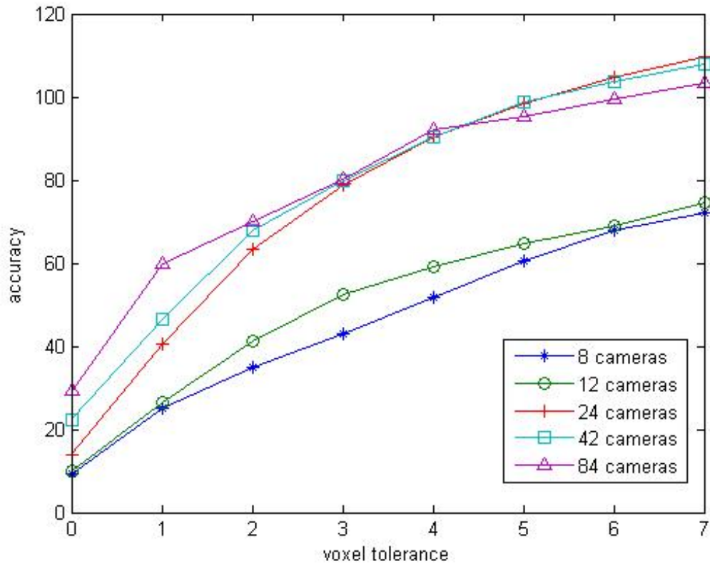
Figure 6-27: Reconstruction accuracy within n-voxel tolerance for the deer data set.
