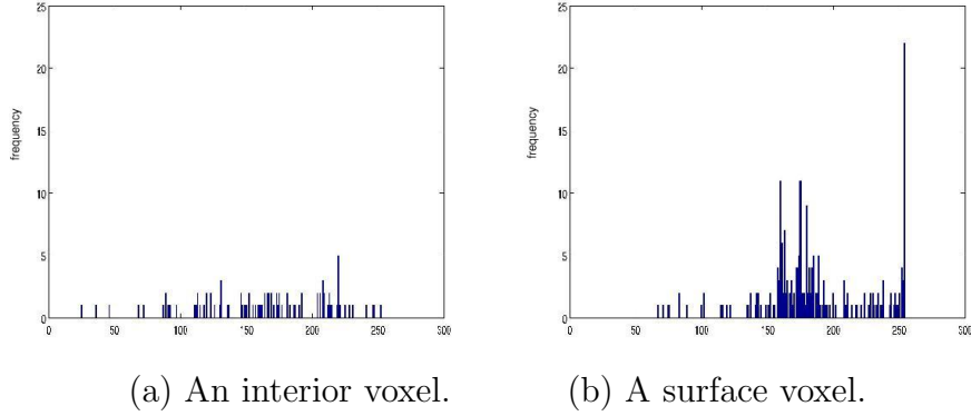
Figure 5-2: Color histogram of different voxels. A surface voxel usually has a color whose frequency is much higher than others.
