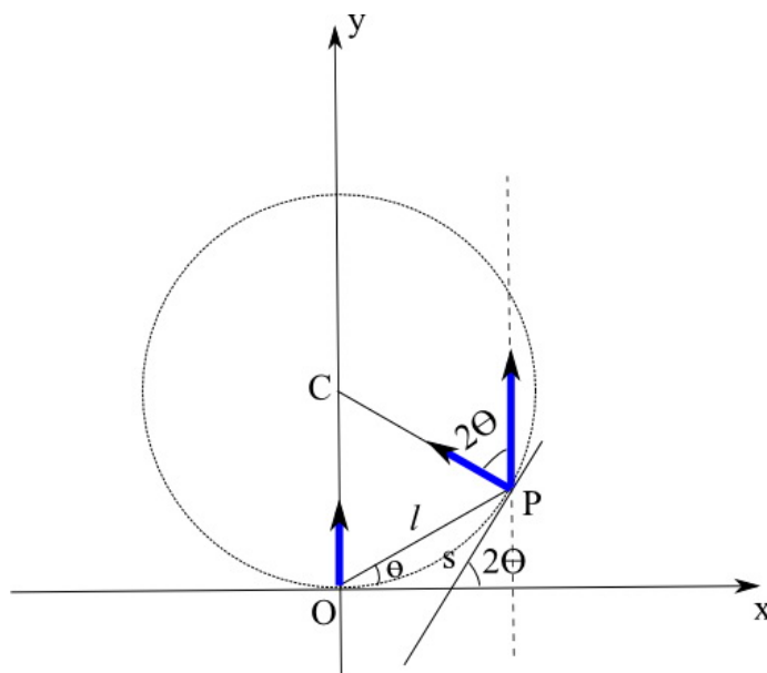
Figure 6–5: Second order vote cast by a stick tensor located at the origin. Note the orientation at the receiver P is a rotation of 2\theta degrees of the voter O 's orientation.
