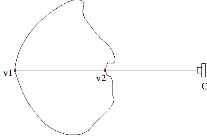
Figure 2–9: The coupled problem of visibility and the photo consistency test. Whether v1 is visible to camera C depends on the occupancy of v2 , which in turn depends on the photo consistency test on v2 . In order to test the photo consistency of v2 , one must first determine its visibility. Note that this is a global problem, as v1 and v2 can be far apart.
