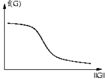
Figure 4–3: The qualitative shape of f(\cdot) .
