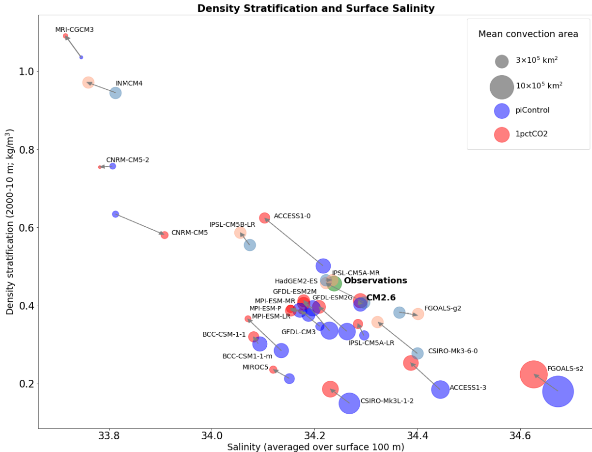
FIG. 6. Mean convection area over the piControl (blue) and 1pctCO 2 (red) simulations in the open ocean Weddell Sea as a function of their respective annual surface salinity over the top 100 m and annual density stratification (2000 - 10 m density difference). Pale coloured models correspond to non-convective models in the Weddell Sea, defined as models that do not have a year where the September convection area exceeds 10 5 km 2 . Averages are calculated over the full 80 years of each simulation as not all models convect during the same periods. Observations (green) are plotted with the average convection area of the 1970's Weddell Sea Polynya and average salinity and density stratification of the WOD profiles spanning from 1920 to 2018. Most CMIP5 models undergo an increase in stratification in response to the 1pctCO 2 forcing (visible by the arrow pointing up), concurrent with a decrease in surface salinity (arrows pointing to the left) and decrease in convection are (larger blue than red circles).
