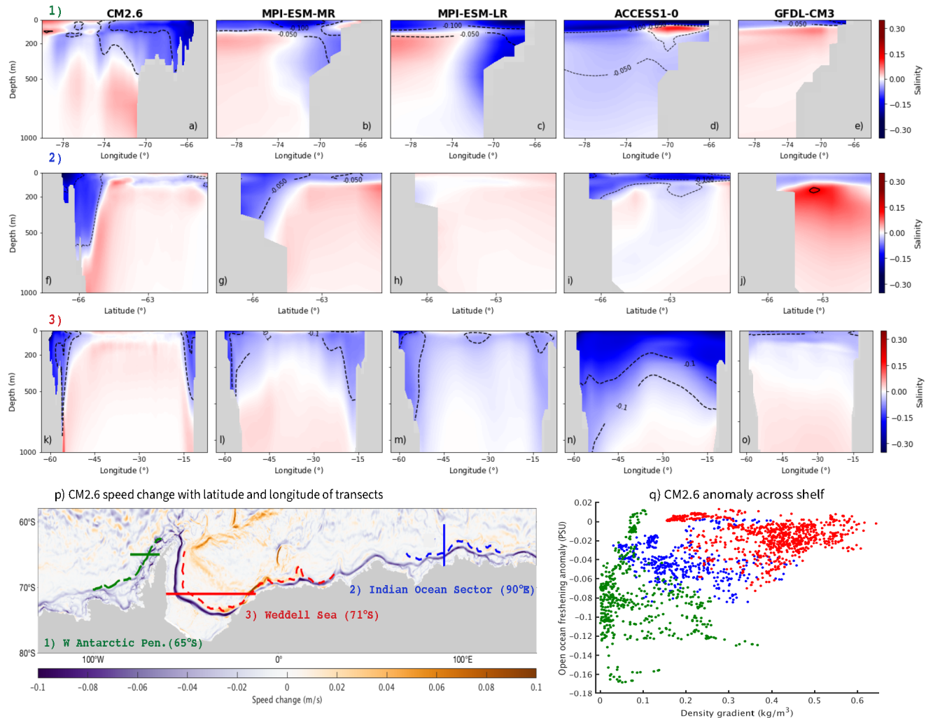
FIG. 10. (Top three rows) Same as top three rows of Fig. 9 but for salinity change (1pctCO 2 minus piControl). Note that the LLC_4320 model is not displayed as this model does not have any corresponding climate change simulation. p) Average speed (0 - 1000 m) change in CM2.6, and transects used for the salinity cross-sections. A justification for the position of transects can be found in Section 7a. q) Scatter plot of cross-shelf density gradients in the piControl (as a measure of the ASC strength) versus salinity change (1pctCO 2 minus piControl) in the open ocean in CM2.6. Calculations are made over the top 150 m, with gradients calculated as the difference between the 0 - 800 m and 3000 - 3400 m isobaths. Open ocean salinity is calculated over the top 150 m and in the 3000 - 3400 m isobaths. In strong ASC regions, such as the Weddell Sea (red dots), we see large density gradients associated with weak open ocean freshening. Each point on q) is calculated at each grid point for CM2.6 along the dashed lines (1300 m isobath) on p).
