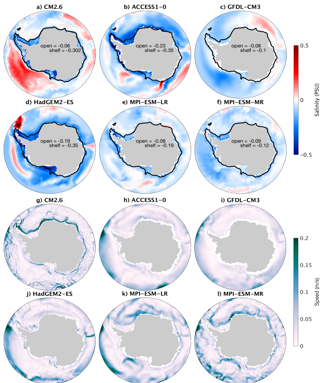
FIG. 8. (a-f) Salinity change (1pctCO 2 minus piControl) averaged over the top 50 m, and 1000 m isobath (black contour) for CM2.6 and a subset of the 23 models. Numbers over the continent correspond to the top 50 m depth averaged salinity change (lower number) in the shelf region and (upper number) in the open ocean region of the Weddell Sea. (g-l) Speed averaged over the top 1000 m in the piControl simulation for CM2.6 and a subset of the 23 models.
