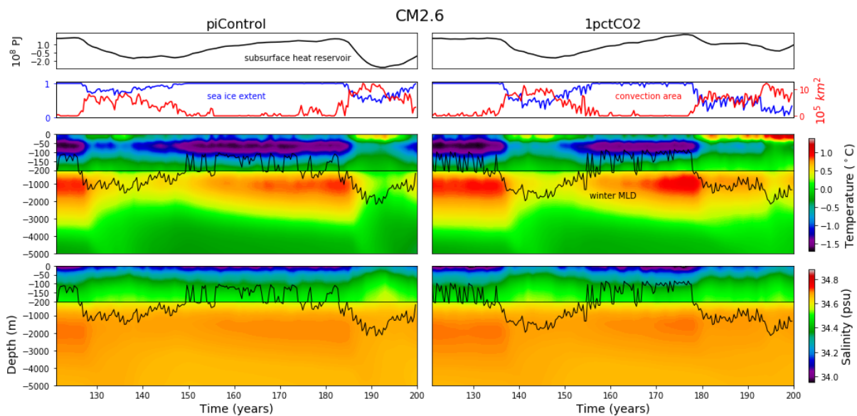
FIG. 3. Sea ice and thermohaline properties of CM2.6 piControl (left column) and 1pctCO 2 (right column) simulations averaged over the open ocean Weddell Sea region (see Section 2.d and Fig. 1). The top panel contains time series of the subsurface heat reservoir ( 10^8 PJ) defined as the annual heat anomaly, relative to the average heat content over the entire control simulation, in the depth range of 200 - 2000 m. The second from top row contains the dimensionless winter sea ice extent (July-September; blue line) and September convection area (red line; Section 2.d). Sea ice extent is defined using a 15% sea ice concentration threshold. The two lower panels are Hovmöller diagrams (depth vs time) of annual mean potential temperature ( ^{\circ} C) and salinity (psu) overlaid with timeseries of winter MLD in the open ocean Weddell Sea (averaged between July-September; black line). Note that there is a zoom on the upper 200 m of the salinity and potential temperature fields. In addition, salinity and potential temperature fields are not fully saturated to allow for visual comparison with Fig.4.
