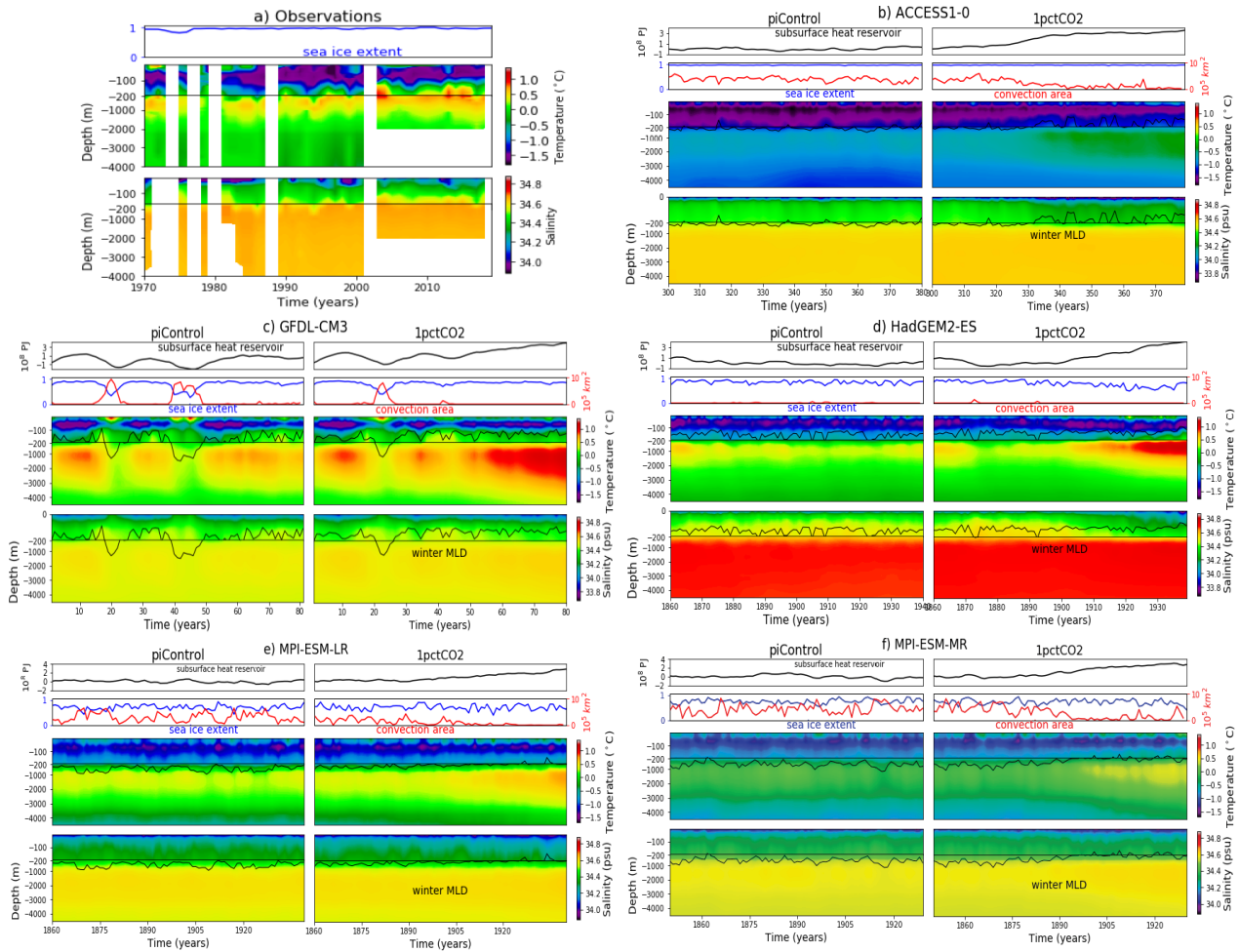
FIG. 4. a) Sea ice and thermohaline properties for observations over the open ocean Weddell Sea (see Section 2c). The top panel contains time series of winter sea ice extent (July–September; blue line) from the Hadley Centre Sea Ice and Sea Surface Temperature data set (HadISST; Rayner et al. 2003) from 1970 to 2018. Note that the start at 1970 is chosen to show the Weddell Sea Polynya that occurred in 1974–1976, but does not extend further back as the dataset prior to 1979 is of lower resolution and is less homogeneous (using multiple algorithms) compared to the current satellite period from 1979 onwards. The two lower panels are Hovmöller diagrams (depth vs time) of annual mean potential temperature ( ^{\circ}\text{C} ) and salinity (psu) observations from the WOD spanning from 1970 to 2018 (see Section.2c). The sea ice extent is defined using a 15% sea ice concentration threshold. White colors corresponds to missing data. b–f) Same as Fig. 3 but for the b) ACCESS1-0, c) GFDL-CM3, d) HadGEM2-ES, e) MPI-ESM-LR and f) MPI-ESM-MR.
