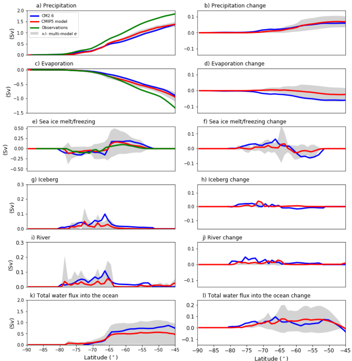
FIG. 7. Freshwater transport (in Sv) into the ocean (left) in the piControl simulations and (right) in response to climate change (1pctCO 2 minus piControl) for CM2.6 (blue) and the CMIP5 model mean (red). The transport is calculated as the zonally integrated water flux into the ocean (wfo output) and is binned into 1° latitude bins. The total freshwater transport (k-l) is the sum of transports from liquid and solid precipitation (a-b), evaporation (c-d), sea ice melting/freezing (e-f), iceberg calving (g-h), and river run-off (i-j). For comparison with models (green), we show (a,c) precipitation and evaporation averaged between 1979 and 2018 from ERA-Interim reanalysis (Dee et al. 2011; see Section.2c), and (e) sea ice freezing and melting flux averaged between 1982 and 2008 from observational estimates described in Haumann et al. 2016 (see Section.2c). Positive values denote a positive flux into the ocean. Not all variables were available for the 23 CMIP5 models used in this study. The models used to compute the CMIP5 models means (red) and standard deviations (grey shades) for each panel are listed in Table S3. CMIP5 model precipitation and evaporation fluxes (a-d) are for all 23 CMIP5 models used in this study. All
