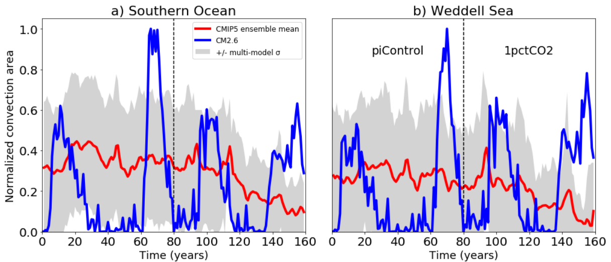
FIG. 5. Normalized convection area for the CMIP5 model mean (red) and CM2.6 (blue) for the open ocean of a) the Southern Ocean and b) the Weddell Sea. The grey shading denotes \pm 1 standard deviation across the CMIP5 models. For each model, the area is normalized by the maximum areal extent of convection recorded over all simulations for that model. The first 80 years denote the piControl, while the following 80 years (years 80-160) denote the 1pctCO 2 simulation. The CMIP5 model mean (red) and CM2.6 model (blue) lines are computed as a 5 year running mean.
