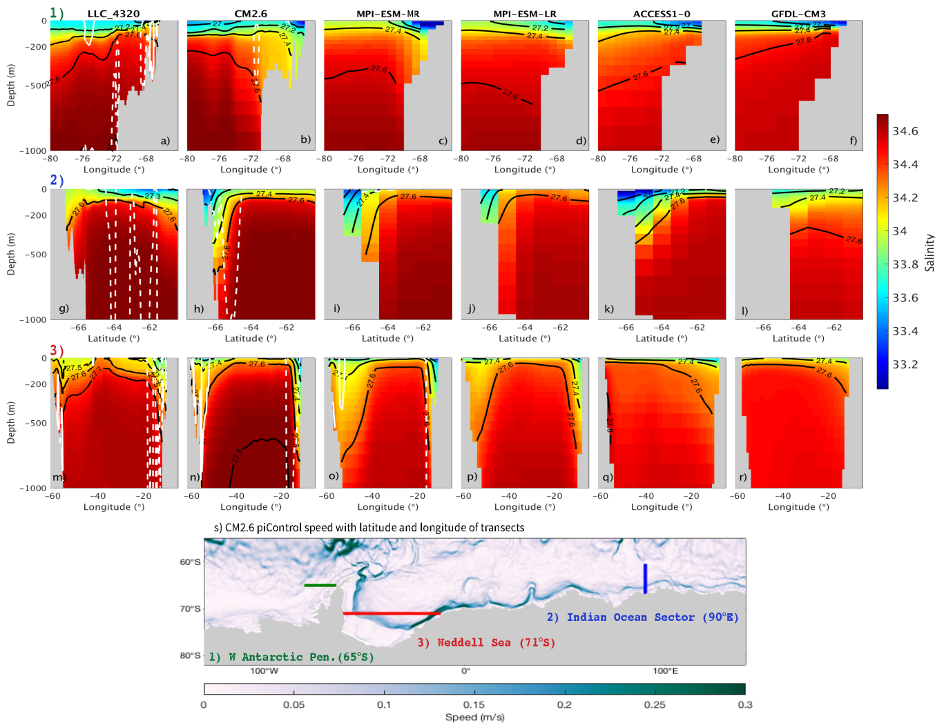
FIG. 9. Salinity cross-sections at (1, first row) 65° S, (2, second row) 90°E and (3, third row) 71° S for LLC_4320 (a,g,m), and the piControl simulation of CM2.6 (b,h,n), and of a subset of the 23 CMIP5 models: MPI-ESM-MR (c,i,o), MPI-ESM-LR (d,j,p), ACCESS1-0 (e,k,q) and GFDL-CM3 (f,l,r). A justification for the position of the transects can be found in Section 7a. (a-r) Black contours correspond to potential density referenced to the surface ( \sigma_0 in kg/m 3 ) white contours to \pm 0.08 m/s zonal velocity contours (in m/s). (q) Average speed (0 - 1000 m) in the piControl simulation of CM2.6, and transects used for the salinity cross-sections.
