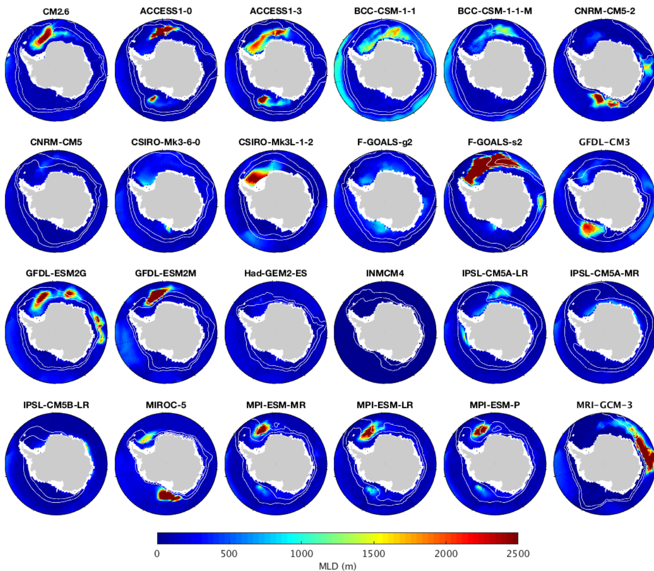
FIG. 2. Winter mixed layer depth (shading) and sea ice concentrations at 25% & 75% (white contours) averaged over the piControl experiment for all models analysed. Winter averages are taken over July to September. The masked shelf region appear in white.
