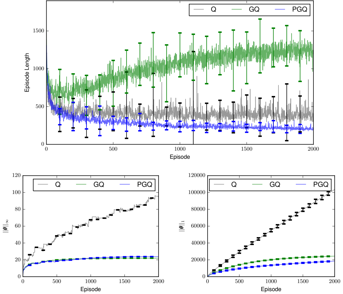
Figure 4.3: Episode length, infinity norm, and L1 norm of the value function parameter \theta on the Acrobot task. Both plots show data from the same experiments and the curves show the averages and standard deviations of 20 repeats. Q-learning uses a learning rate of \alpha = 0.2 . GQ and PGQ both use \alpha = 0.1 and \beta = 0.005 .
