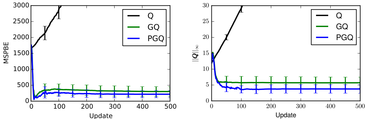
Figure 4.1: MSPBE and maximum of all state-action values for off-policy control averaged over 20 runs. The behaviour policy temperature is \tau = 10 . The temperature of the target policy used by GQ and PGQ is \tau = 0.2 . Q-learning uses a learning rate \alpha = 0.01 while GQ and PGQ both use \alpha = 0.1 and \beta = 0.1 .
