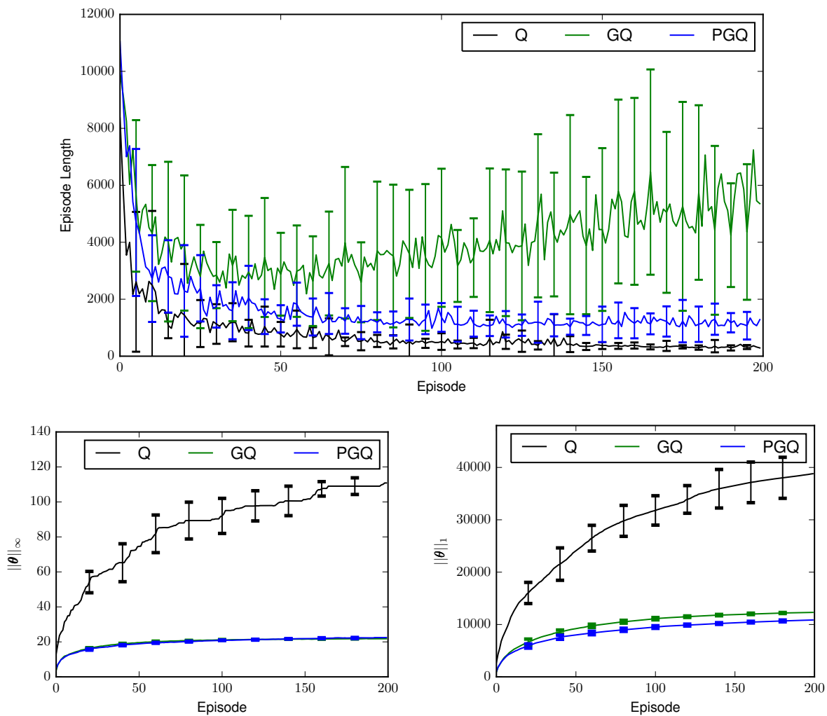
Figure 4.2: Episode length, infinite norm, and L1 norm of the value function parameter \theta on the Mountain car task. Both plots show the same dataset. Each experiment is repeated 20 times. Q-learning uses a learning rate \alpha = 0.5 while GQ and PGQ use learning rates \alpha = 0.1 and \beta = 0.005 .
