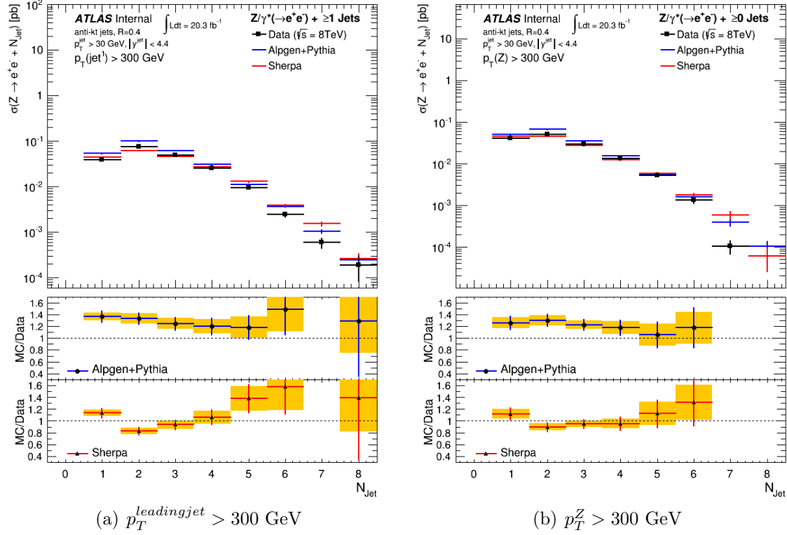
Figure 10.2: Exclusive jet multiplicity for (a) p_T^{\text{leading jet}} > 300 GeV and (b) p_T^Z > 300 GeV in Z/\gamma^*(\rightarrow ee)+\text{jets} events for data unfolded to particle level compared to predictions from Alpgen+Pythia and Sherpa. The yellow band in the ratio plots represent the total systematic uncertainty. The error bars represent the total systematic and statistical uncertainty.
