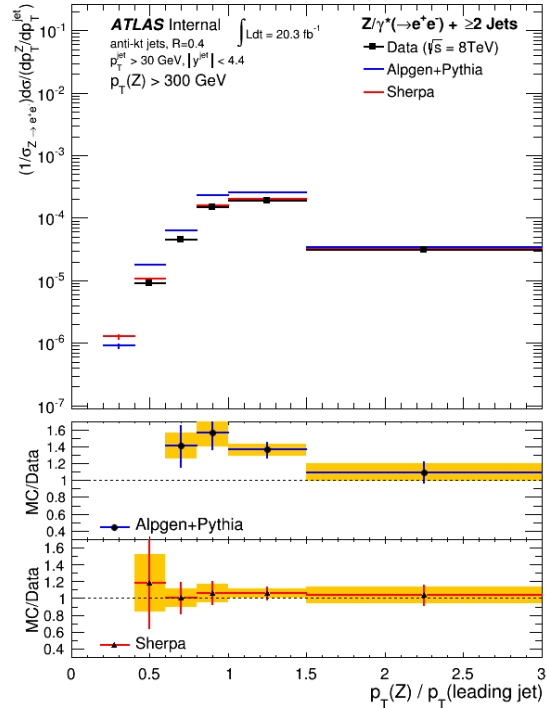
(c) p_T(Z) > 300 \text{ GeV}
