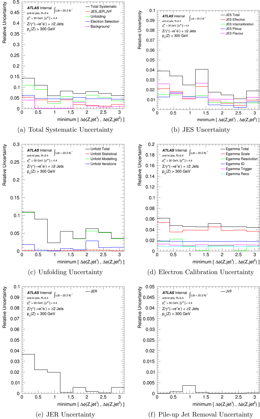
Figure C.17: Minimum \Delta\phi between the Z boson and either of the two leading jets in the event ( \min \Delta\phi^{Zjj} ) in events with at least two jets for p_T^Z > 300 GeV.
