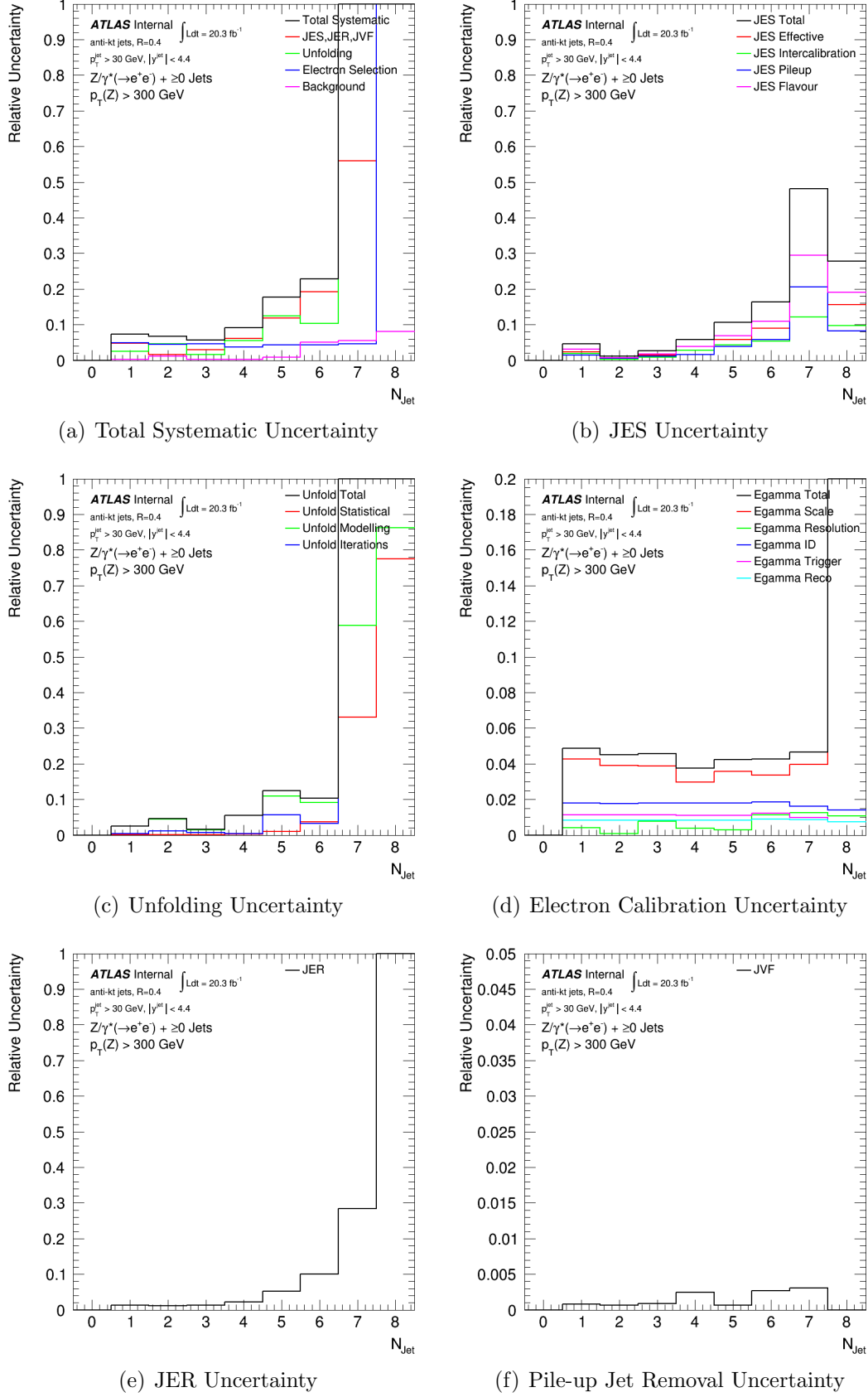
Figure C.3: Exclusive jet multiplicity ( N_{\text{Jet}} ) for p_T^Z > 300 GeV.
