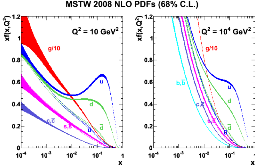
Figure 2.3: MSTW 2008 NLO PDFs for Q^2 = 10 \text{ GeV}^2 and Q^2 = 10^4 \text{ GeV}^2 [36].
