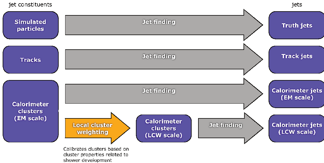
Figure 5.6: Schematic overview of the ATLAS jet reconstruction. After the jet finding, the jet four momentum is defined as the four momentum sum of its constituents.
