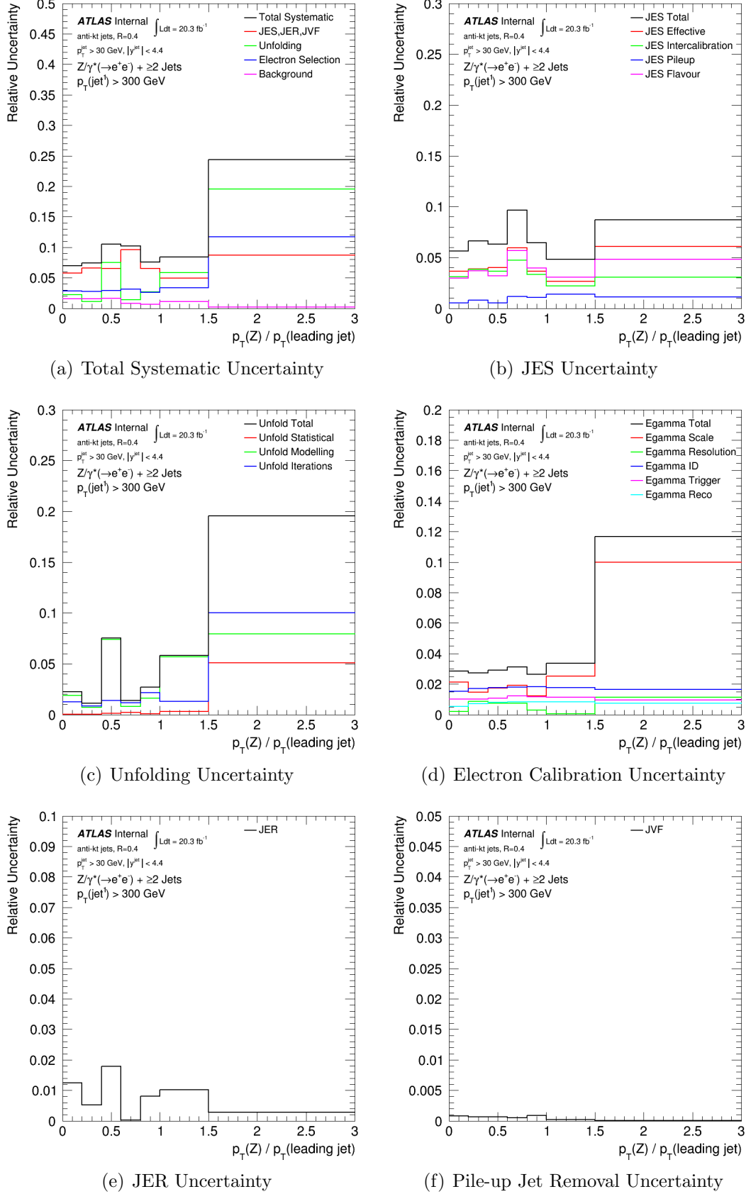
Figure C.13: p_T ratio between Z boson and leading jet ( Rp_T^{jj} ) in events with at least two jets for p_T^{\text{leading jet}} > 300 GeV.
