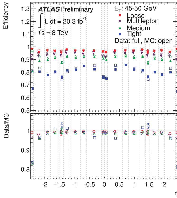
Figure 5.5: Identification efficiency in data as a function of \eta for E_T = 45 - 50 GeV for the cut-based loose, multilepton, medium and tight selections, compared to the MC expectation for electrons from Z \rightarrow ee decay [119].
