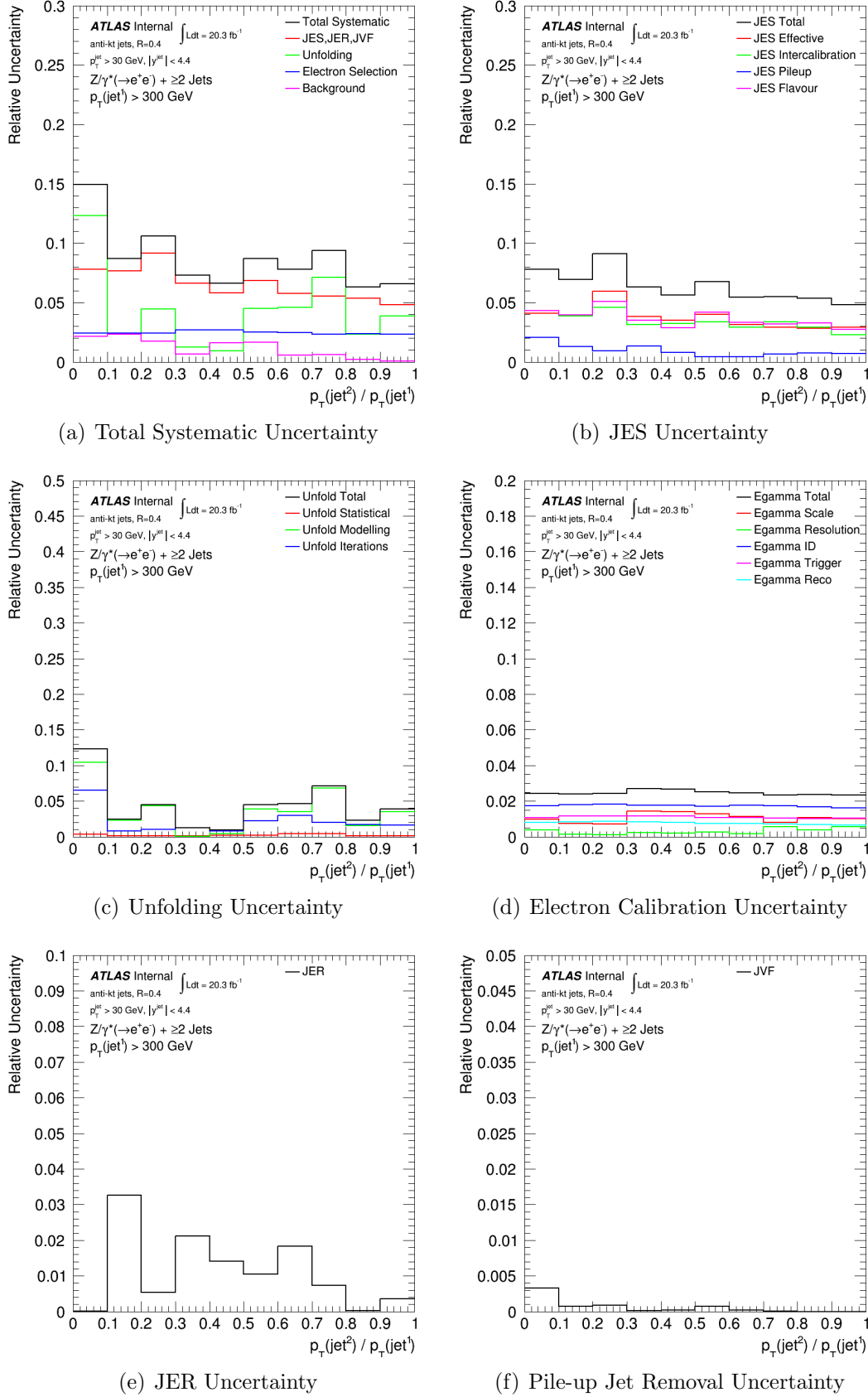
Figure C.10: p_T ratio between sub-leading jet and leading jet ( Rp_T^{jj} ) in events with at least two jets for p_T^{\text{leading jet}} > 300 GeV.
