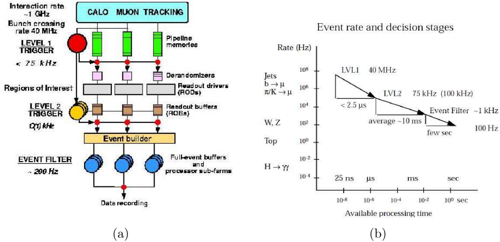
Figure 3.11: (a) Functional overview of the ATLAS TDAQ system and (b) the event rates and processing times for various physics processes at each trigger level.
