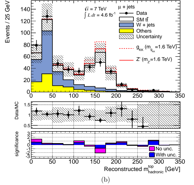
Figure C–1: Reconstructed jet mass of the hadronic top candidate in the e + \text{jets} (a) and the \mu + \text{jets} (b) channels, after the final selection of events, except the requirements on the candidates reconstructed mass and Q_W observables. The uncertainty corresponds to the (bin by bin) quadratic sum of all sources of uncertainties (including the statistical uncertainty of the MC samples) considered in the analysis. The statistical significance of the difference between data and the predicted background is shown in the bottom inset. Hypothetical signals (a Z' with m_{Z'} = 1.6 \text{ TeV} and a g_{KK} with m_{g_{KK}} = 1.6 \text{ TeV} ) are shown on top of the expected Standard Model background.
