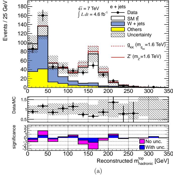
Figure C–1: Reconstructed jet mass of the hadronic top candidate in the e + \text{jets} (a) and the \mu + \text{jets} (b) channels, after the final selection of events, except the requirements on the candidates reconstructed mass and Q_W observables. The uncertainty corresponds to the (bin by bin) quadratic sum of all sources of uncertainties (including the statistical uncertainty of the MC samples) considered in the analysis. The statistical significance of the difference between data and the predicted background is shown in the bottom inset. Hypothetical signals (a Z' with m_{Z'} = 1.6 \text{ TeV} and a g_{KK} with m_{g_{KK}} = 1.6 \text{ TeV} ) are shown on top of the expected Standard Model background.
