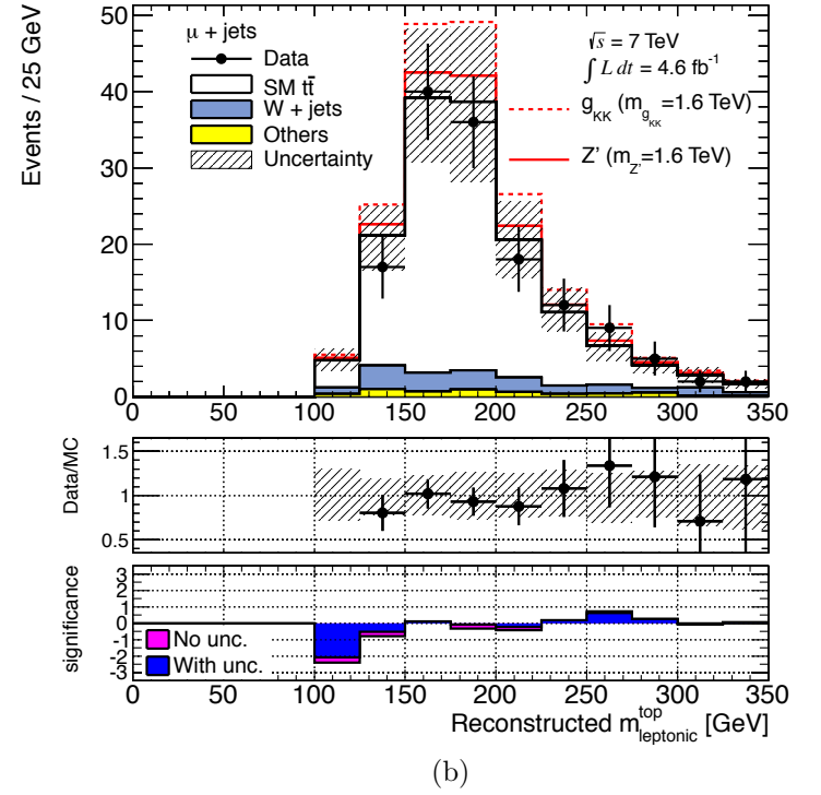
Figure C–3: Leptonic top candidate reconstructed mass in the e+jets (a) and the \mu+jets (b) channels, after the final selection of events, except the requirement on candidates mass. The uncertainty corresponds to the (bin by bin) quadratic sum of all sources of uncertainties (including the statistical uncertainty of the MC samples) considered in the analysis. The statistical significance of the difference between data and the predicted background is shown in the bottom inset. Hypothetical signals (a Z' with m_{Z'} = 1.6 TeV and a g_{KK} with m_{g_{KK}} = 1.6 TeV) are shown on top of the expected Standard Model background.
