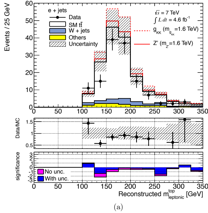
Figure C–3: Leptonic top candidate reconstructed mass in the e+jets (a) and the \mu+jets (b) channels, after the final selection of events, except the requirement on candidates mass. The uncertainty corresponds to the (bin by bin) quadratic sum of all sources of uncertainties (including the statistical uncertainty of the MC samples) considered in the analysis. The statistical significance of the difference between data and the predicted background is shown in the bottom inset. Hypothetical signals (a Z' with m_{Z'} = 1.6 TeV and a g_{KK} with m_{g_{KK}} = 1.6 TeV) are shown on top of the expected Standard Model background.
