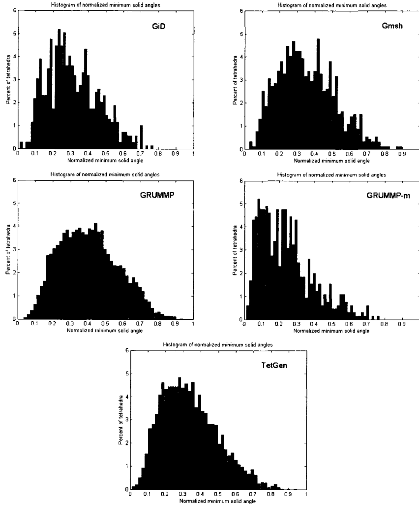
Figure 6.12 Histograms of \theta_{min} for the pillat model
