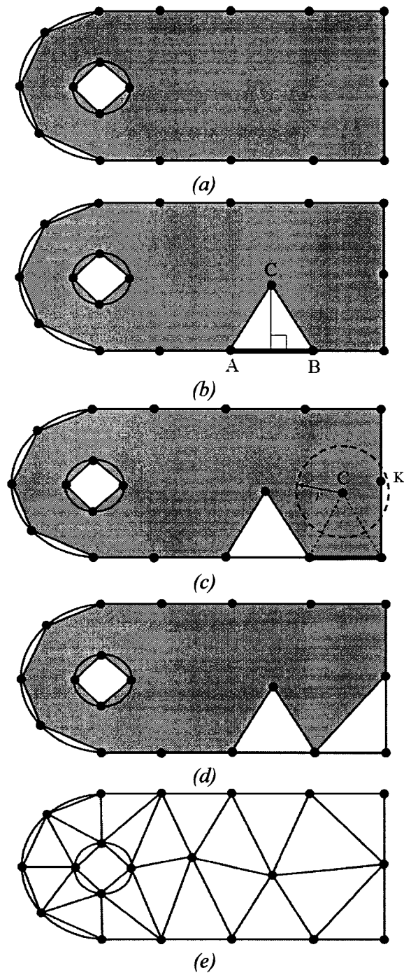
Figure 2.7 The advancing-front method (after Owen 1998)
