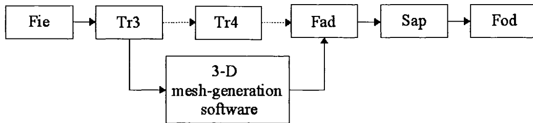
Figure 1.1 Finite-element modeling and simulation pipeline in Auditory Mechanics Laboratory
