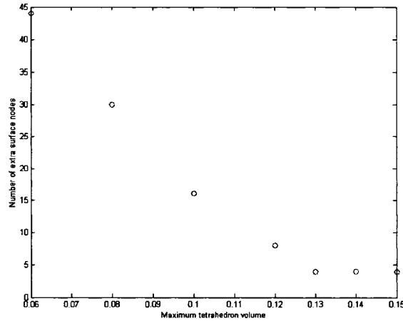
Figure 6.5 Number of extra surface nodes vs. maximum-tetrahedron-volume constraint in TetGen
