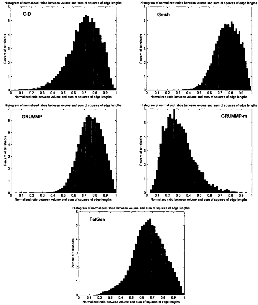
Figure 6.19 Histograms of \eta for Incus model
