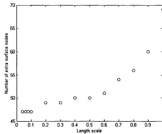
Figure 6.3 Number of extra surface nodes vs. length scale in GRUMMP
