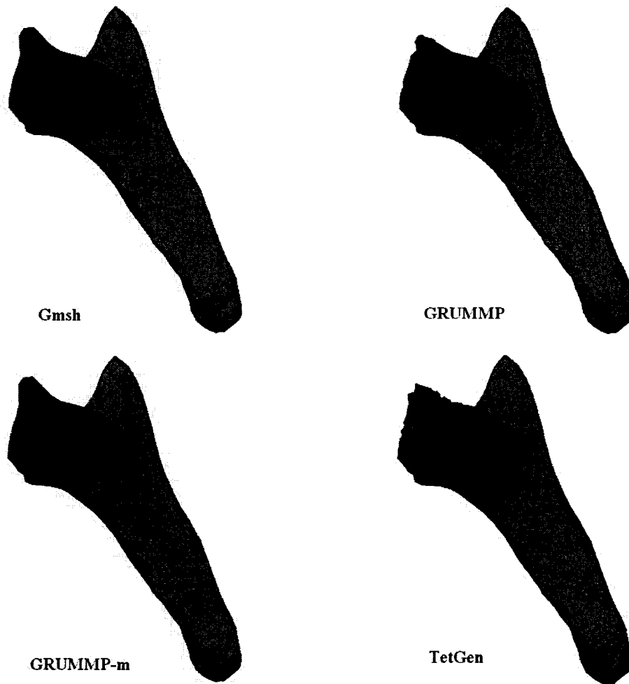
Figure 6.11 Cutting-plane views of the malleus model (GiD fails in this case)
