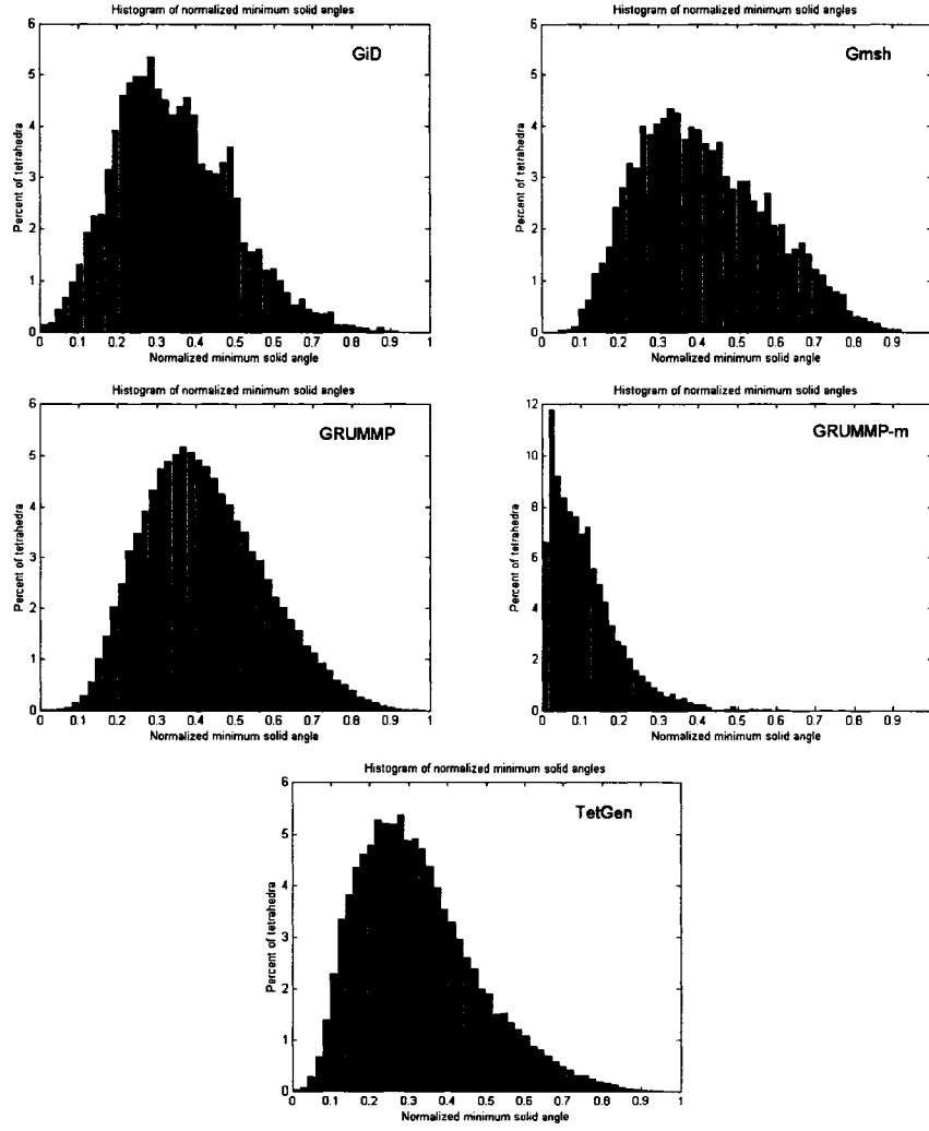
Figure 6.17 Histograms of \theta_{min} for the incus model
