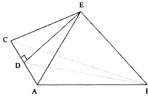
Figure 3.4 Dihedral angle in a tetrahedron
