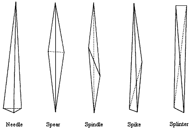
Figure 3.1 Badly shaped narrow tetrahedral elements
