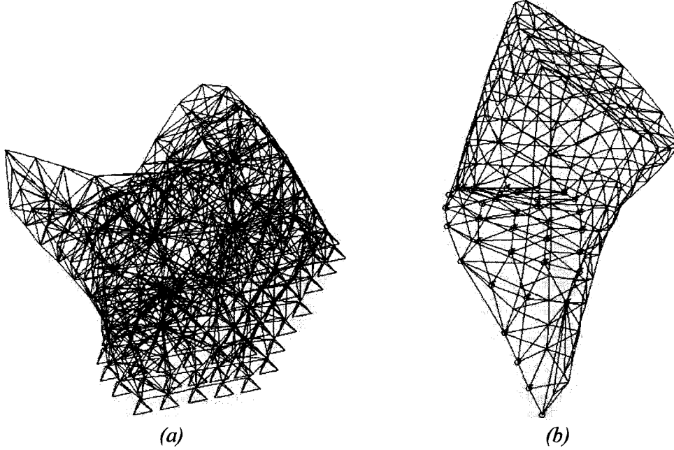
Figure 6.27 Boundary conditions (a) and load conditions (b) for the pillat model
