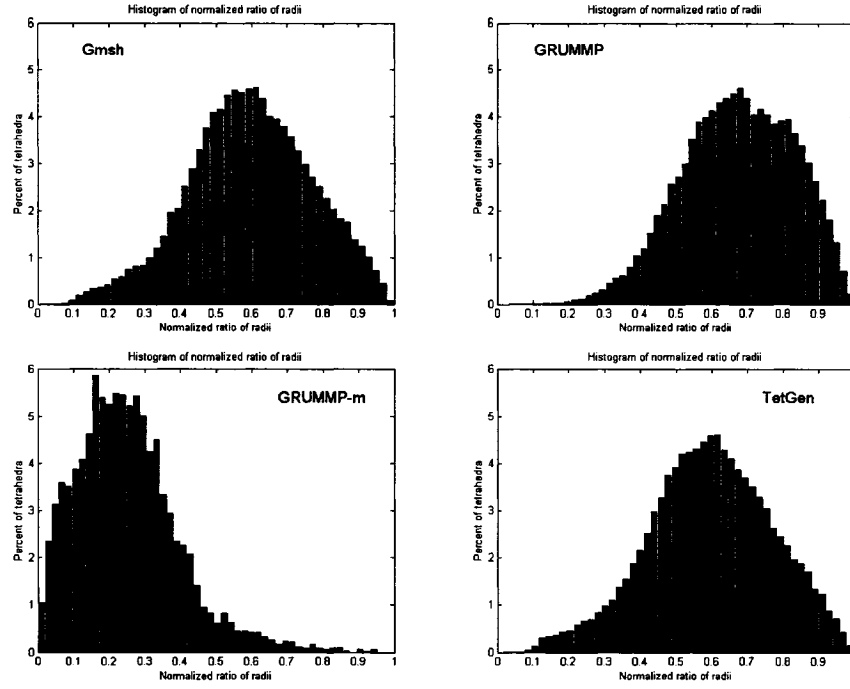
Figure 6.23 Histograms of \rho for the malleus model (GiD fails in this case)
