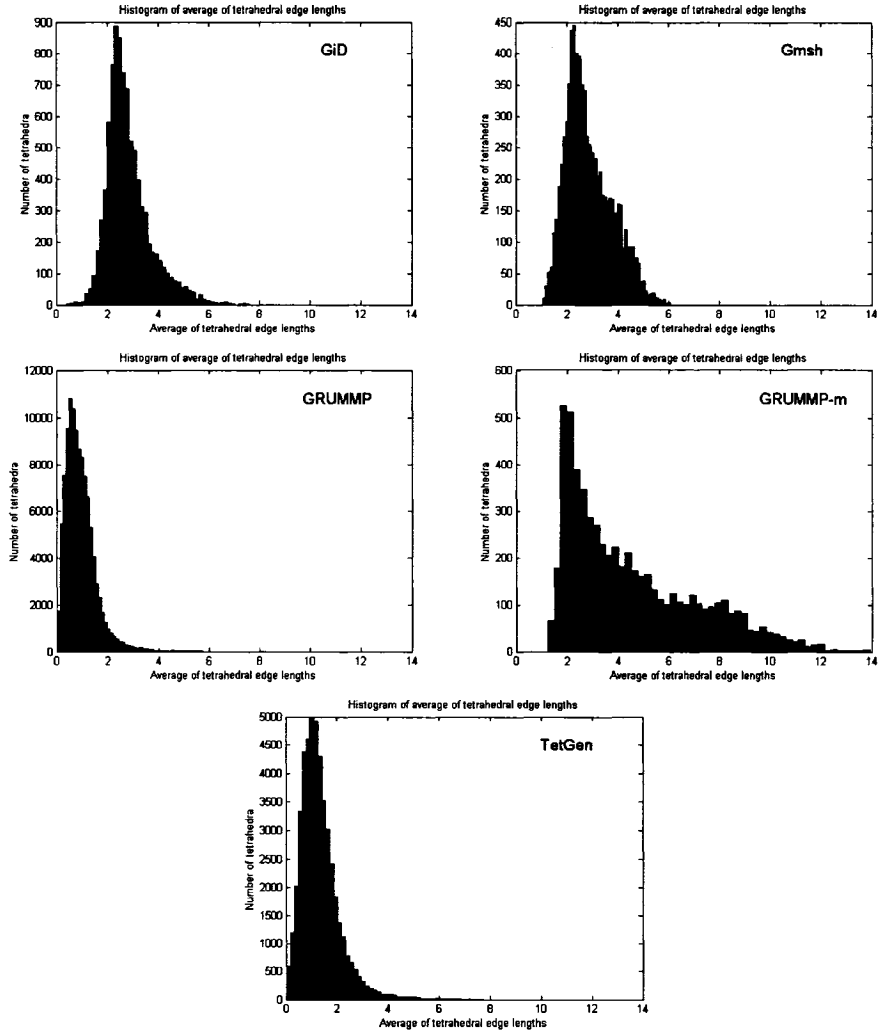
Figure 6.21 Histograms of l_{avg} scaled by 10^4 for the incus model
