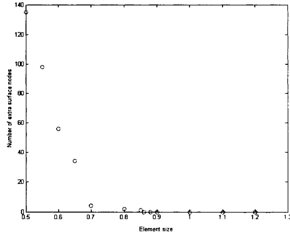
Figure 6.1 Number of extra surface nodes vs. element size in GiD
