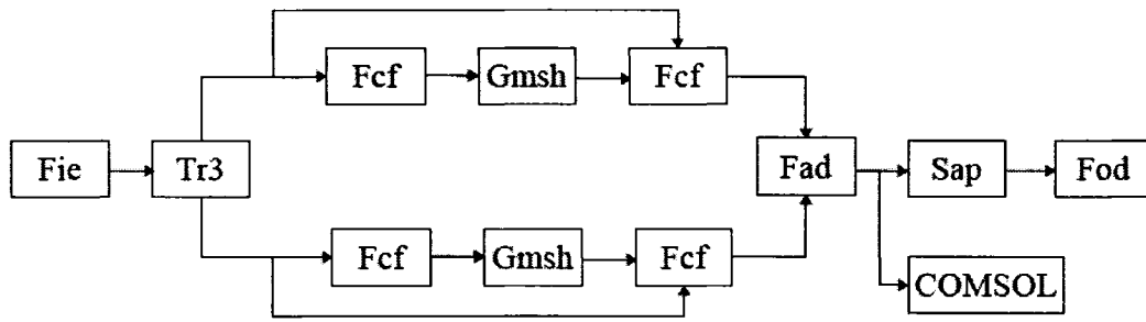
Figure 7.1 Finite-element modeling and simulation pipeline in Auditory Mechanics Laboratory
