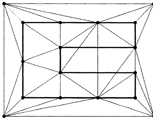
Figure 2.4 Missing boundary edges in the initial triangulation (after Owen 1998)
