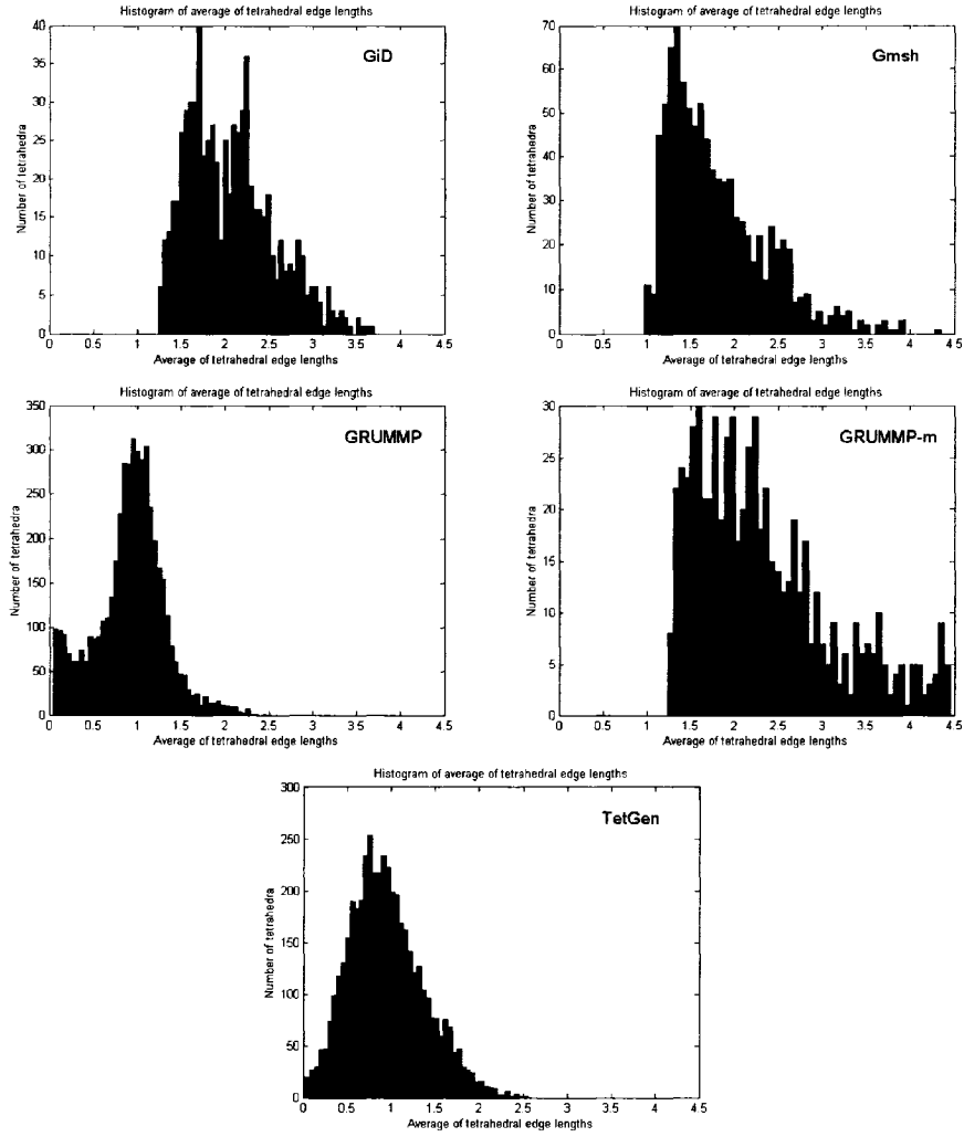
Figure 6.16 Histograms of l_{avg} scaled by 10^4 for the pillat model
