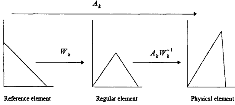
Figure 3.5 Relationships of Jacobian matrices among the reference, regular and physical triangles
