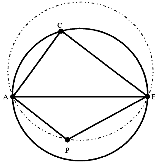
Figure 2.1 Delaunay criterion
