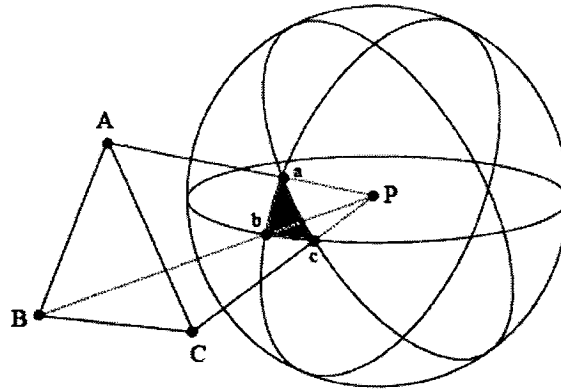
Figure 3.3 Solid angle represented by the shaded area abc in a tetrahedron
