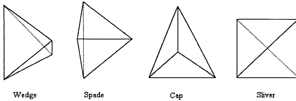
Figure 3.2 Badly shaped flat tetrahedral elements
