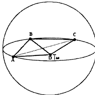
Figure 2.6 Sliver
