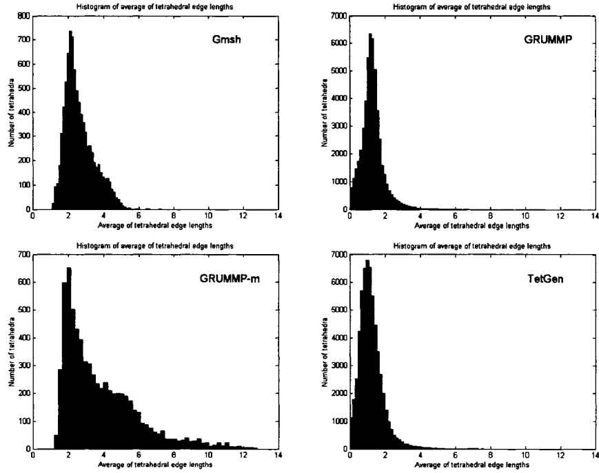
Figure 6.26 Histograms of l_{avg} scaled by 10^4 for the malleus model (GiD fails in this case)
