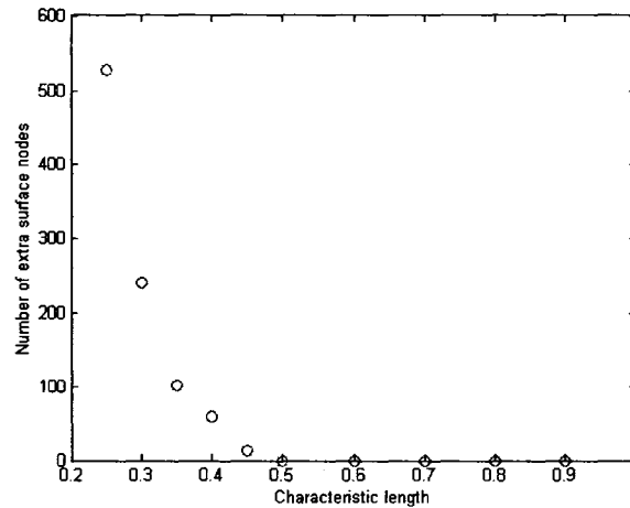
Figure 6.2 Number of extra surface nodes vs. characteristic length in Gmsh
