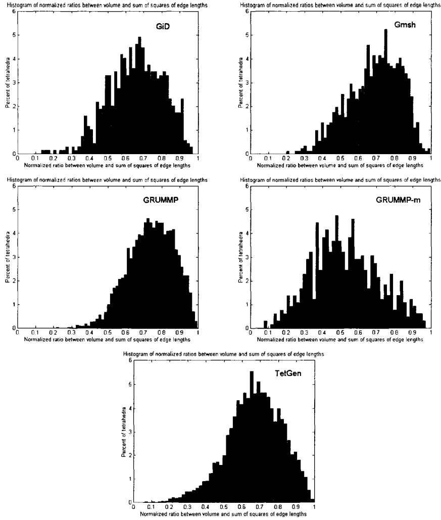
Figure 6.14 Histograms of \eta for the pillat model
