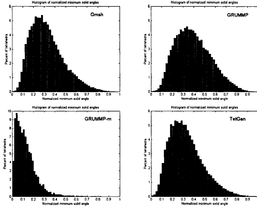
Figure 6.22 Histograms of \theta_{min} for the malleus model (GiD fails in this case)
