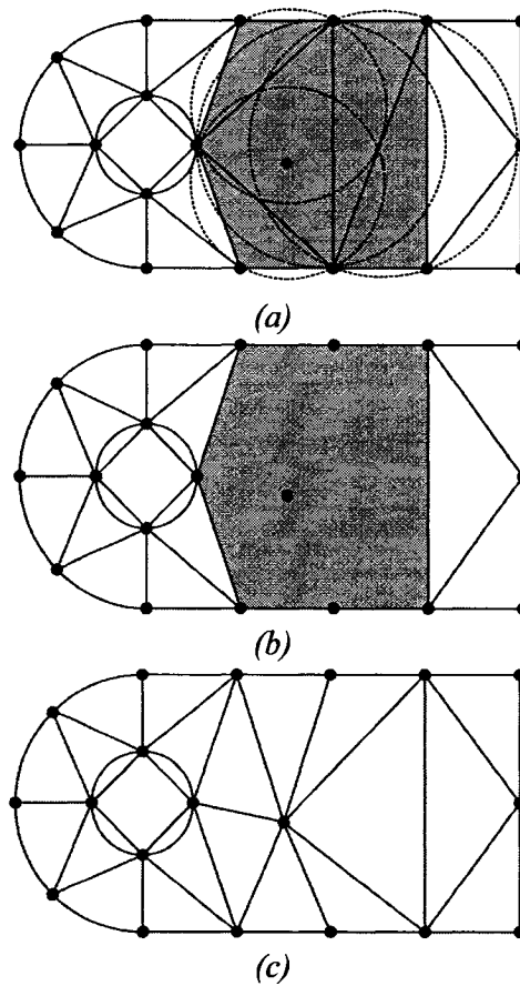
Figure 2.3 Delaunay kernel
