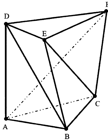
Figure 2.12 Schonhardt polyhedron
