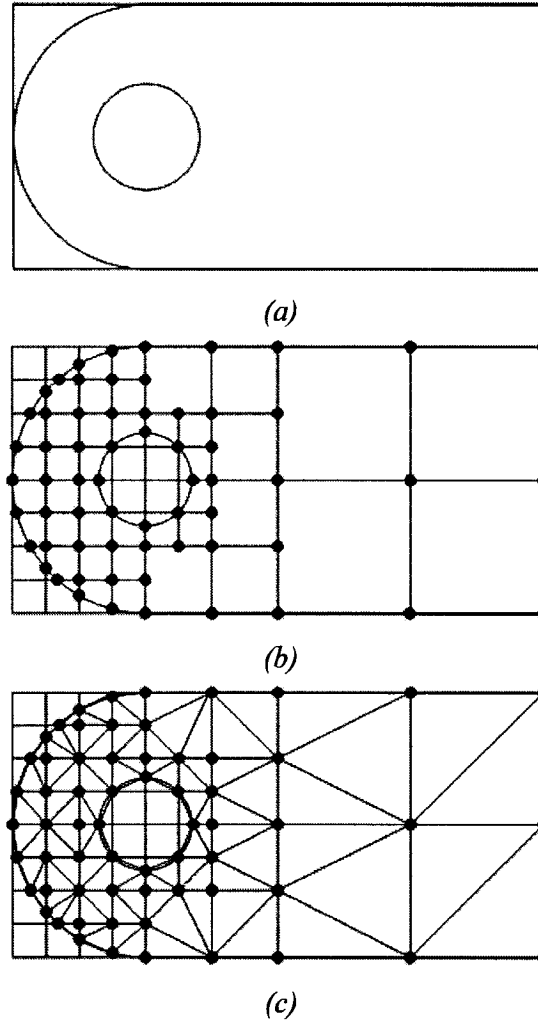
Figure 2.10 The quadtree-based method (after Owen 1998)
