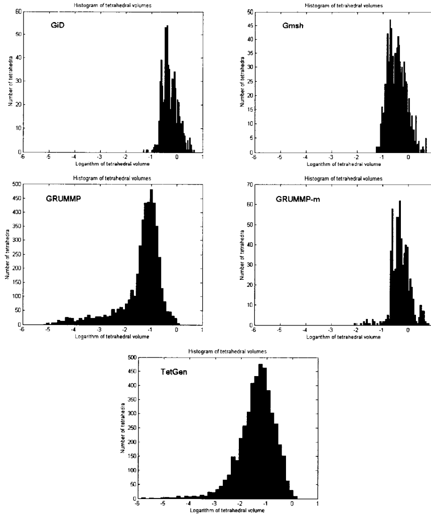
Figure 6.15 Histograms of v scaled by 10^{12} for the pillat model
