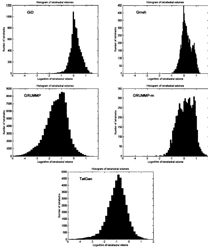
Figure 6.20 Histograms of v scaled by 10^{12} for the incus model
