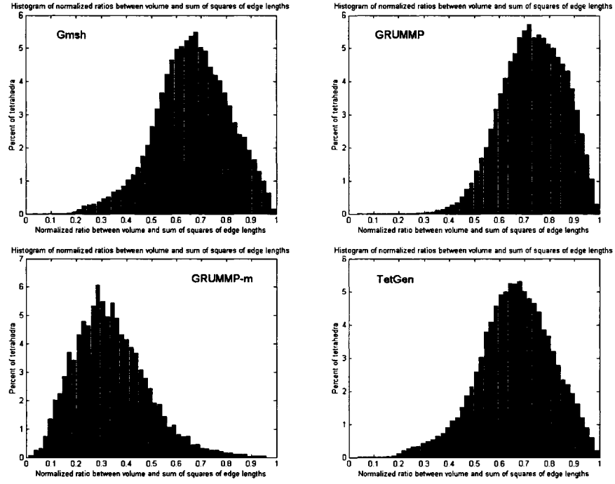
Figure 6.24 Histograms of \eta for the malleus model (GiD fails in this case)
