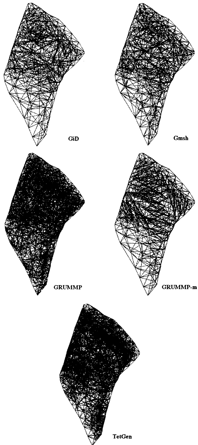
Figure 6.6 Wire-frame views of the pillat model
