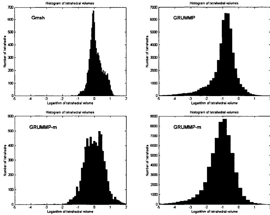
Figure 6.25 Histograms of v scaled by 10^{12} for the malleus model (GiD fails in this case)
