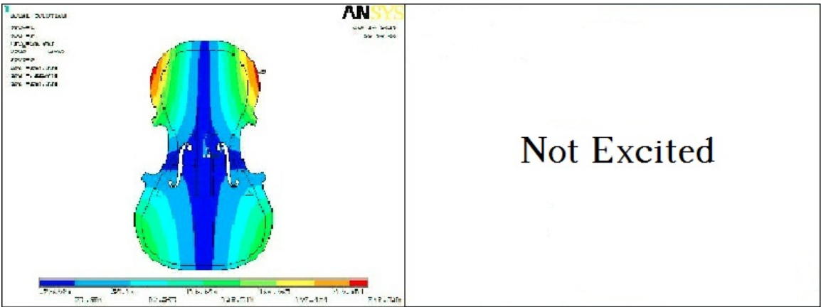
Fig. 4.25 Comparison of Mode 1 of the composite plate #2 by the FEM and the Modal Analysis
