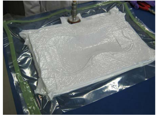
Fig. 4.12 Stage 2 of making a composite plate (air extracted)
