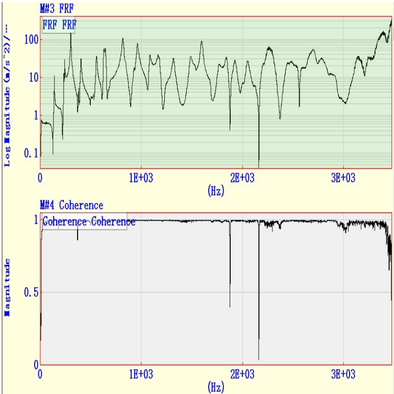
Fig. 3.14 The FRF and the coherence function of point 2
