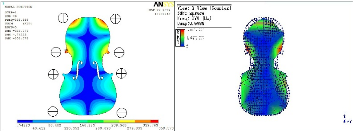
Fig. 4.9 Comparison of Mode 6 of the spruce plate by the FEM and the Modal Analysis
