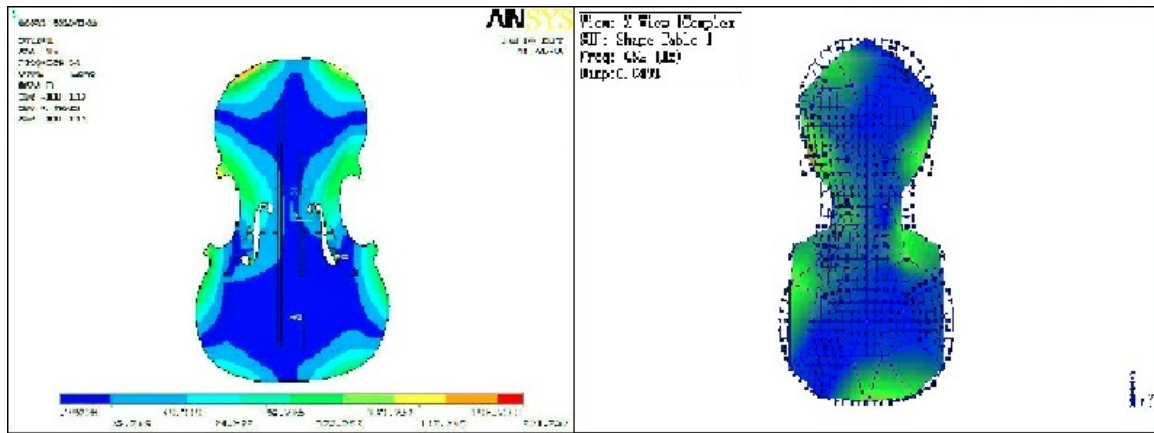
Fig. 4.23 Comparison of Mode 6 of the composite plate #1 by the FEM and the Modal Analysis
