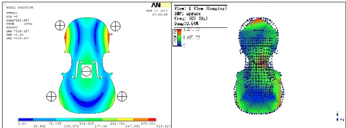
Fig. 4.8 Comparison of Mode 5 of the spruce plate by the FEM and the Modal Analysis
