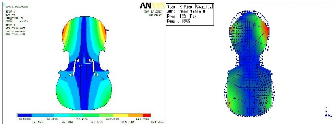
Fig. 4.18 Comparison of Mode 1 of the composite plate #1 by the FEM and the Modal Analysis
