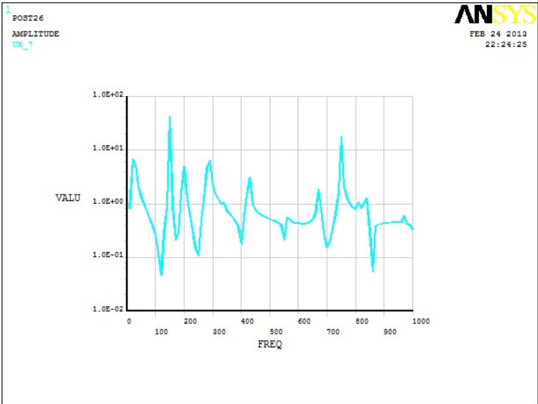
Fig. 5.4 FRF of the spruce plate by the FEM
