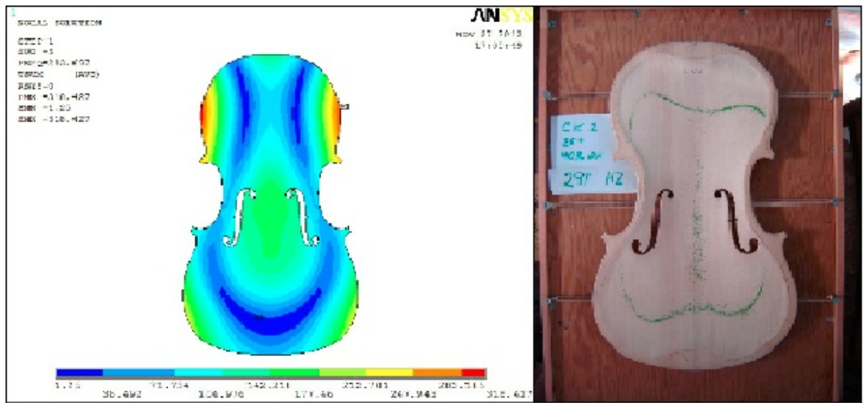
Fig. 4.3 Mode 5 of the spruce plate by the FEM and the Chladni Method
