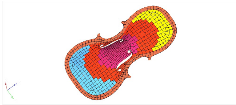
Fig. 3.5 Collectors of the top plate
