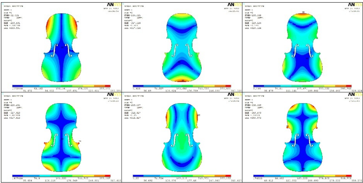
Fig. 5.3 The first six modes of the spruce plate by the FEM
