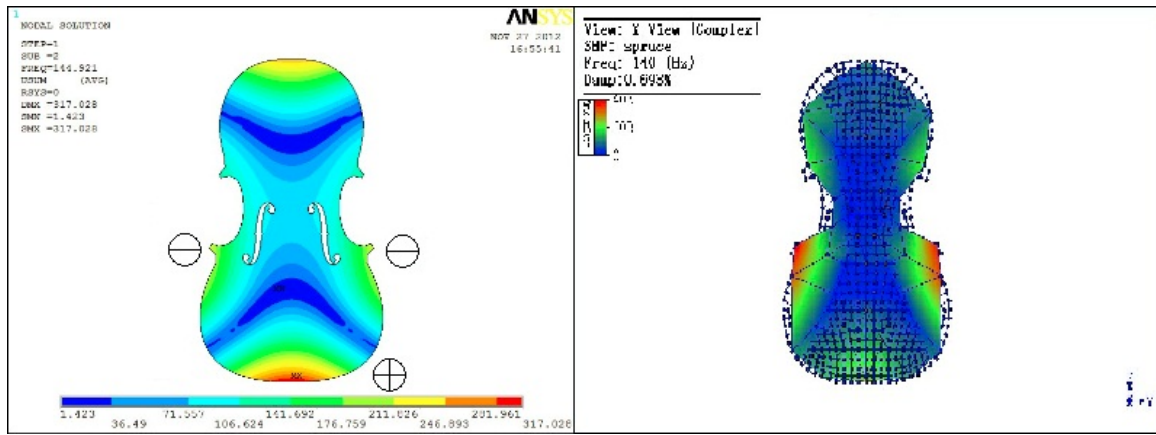
Fig. 4.5 Comparison of Mode 2 of the spruce plate by the FEM and the Modal Analysis
