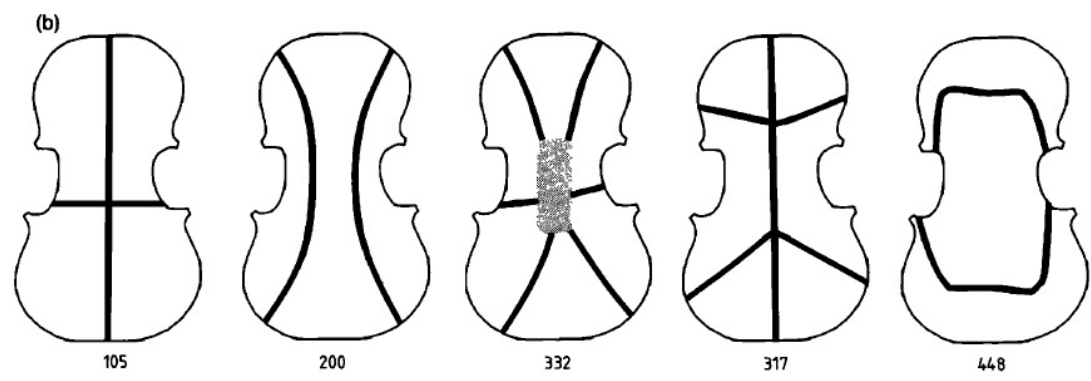
Fig. 5.2 The first six modes of the spruce plate by the FEM (Molin) [5]
