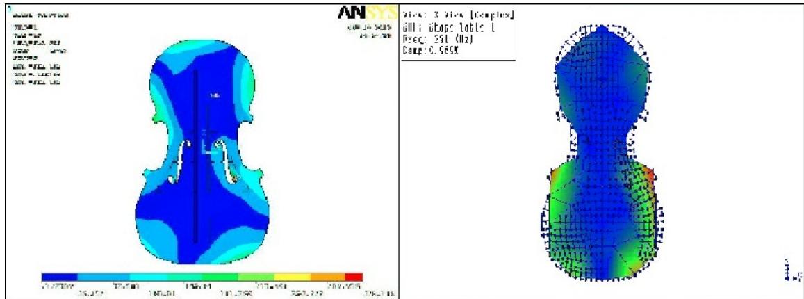
Fig. 4.21 Comparison of Mode 4 of the composite plate #1 by the FEM and the Modal Analysis
