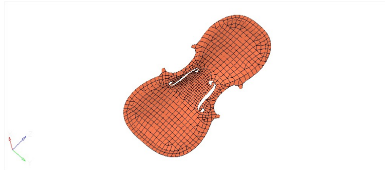
Fig. 3.4 Meshing of the spruce top plate
