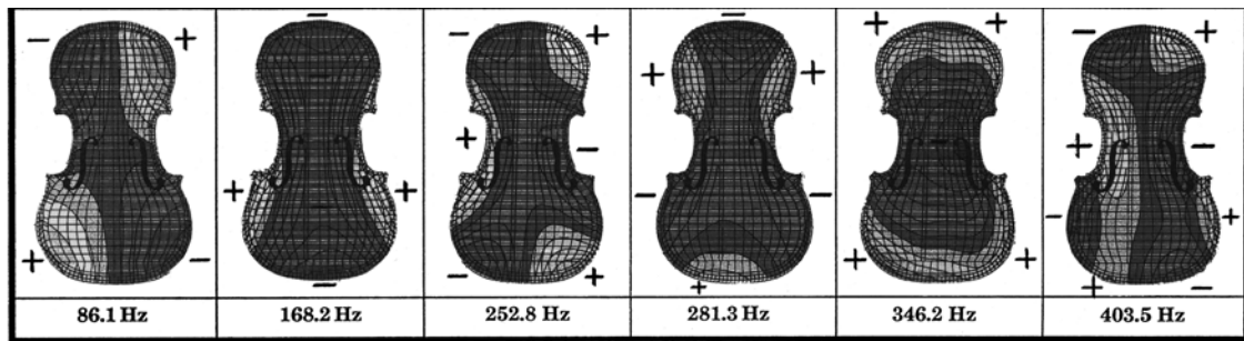
Fig. 5.1 The first six modes of the spruce plate by the FEM (Bretos) [4]
