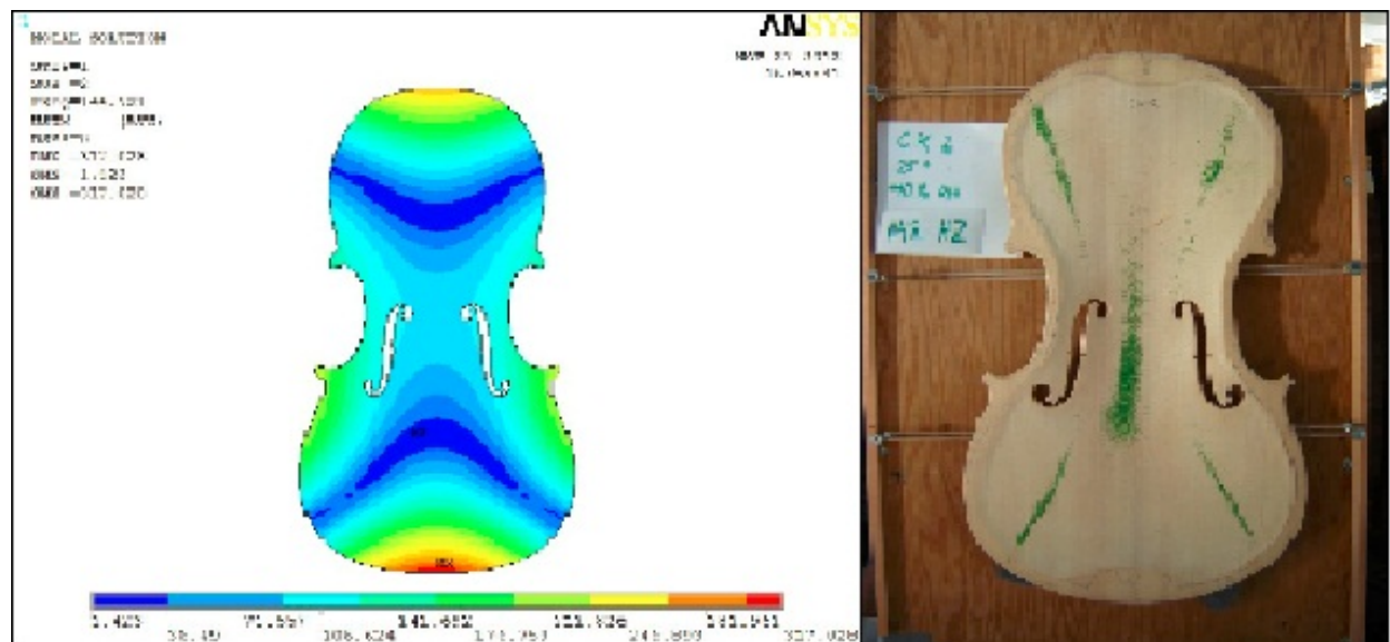
Fig. 4.2 Mode 2 of the spruce plate by the FEM and the Chladni Method
