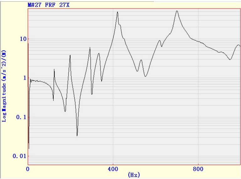
Fig. 5.7 FRF of the composite plate #1 by the Modal Analysis
