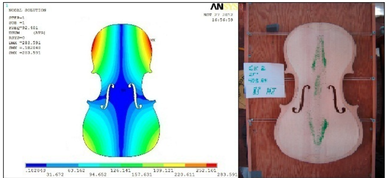
Fig. 4.1 Mode 1 of the spruce plate by the FEM and the Chladni Method
