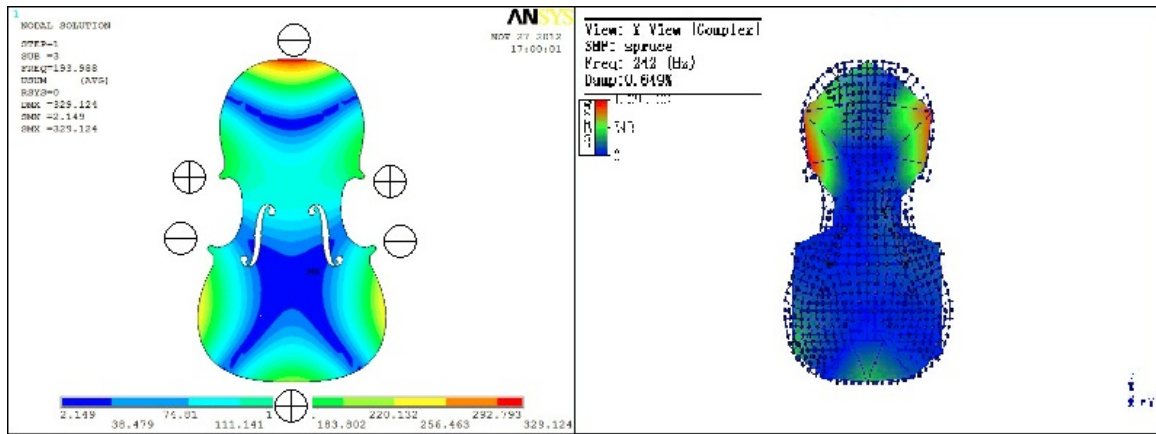
Fig. 4.6 Comparison of Mode 3 of the spruce plate by the FEM and the Modal Analysis
