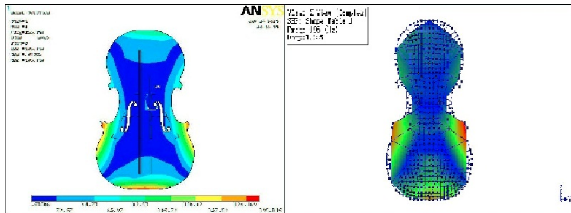
Fig. 4.19 Comparison of Mode 2 of the composite plate #1 by the FEM and the Modal Analysis
