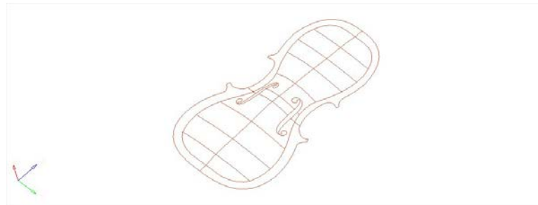
Fig. 2.4 A violin top plate
