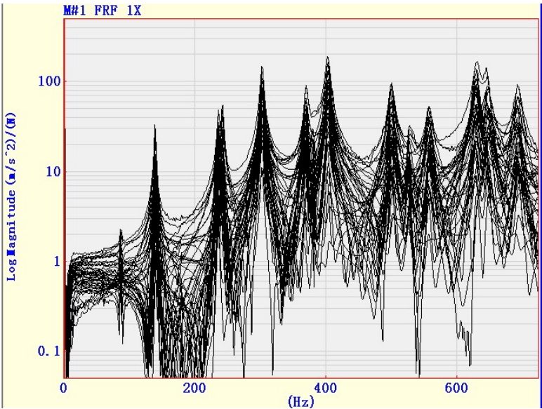
Fig. 3.15 Overlapped FRFs
