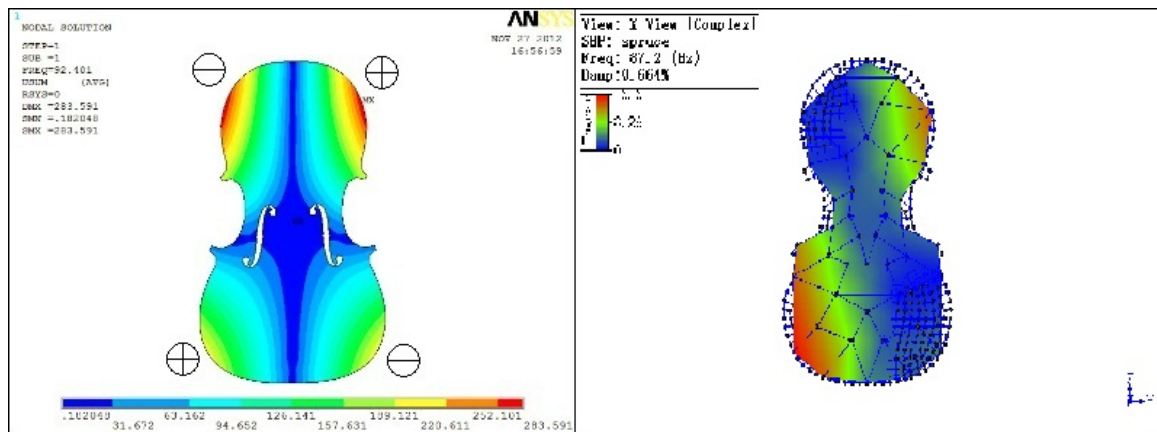
Fig. 4.4 Comparison of Mode 1 of the spruce plate by the FEM and the Modal Analysis
