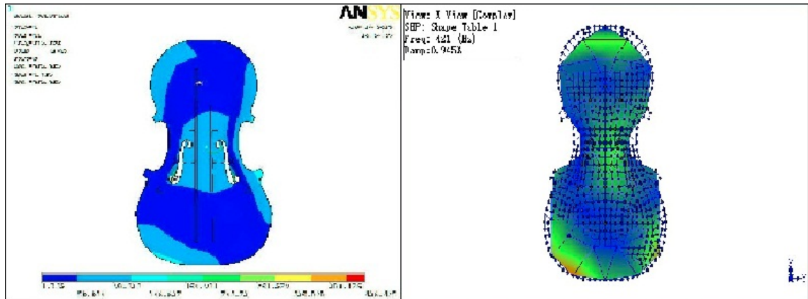
Fig. 4.22 Comparison of Mode 5 of the composite plate #1 by the FEM and the Modal Analysis
