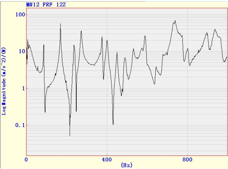
Fig. 5.9 FRF of the composite plate #2 by the Modal Analysis
