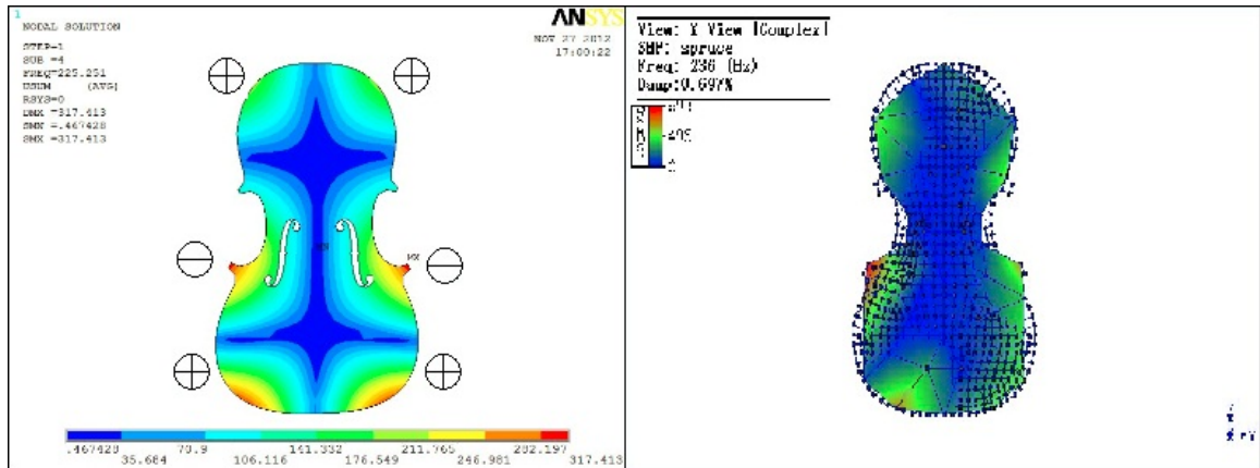
Fig. 4.7 Comparison of Mode 4 of the spruce plate by the FEM and the Modal Analysis
