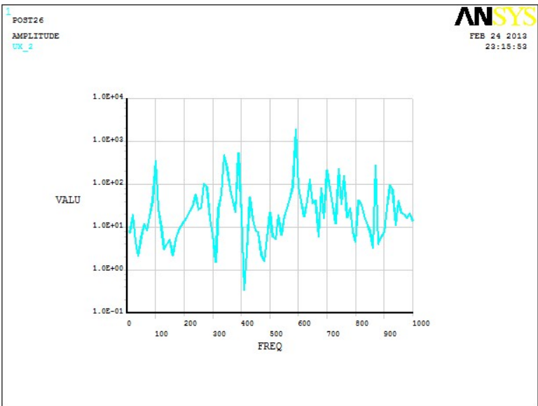
Fig. 5.8 FRF of the composite plate #2 by the FEM
