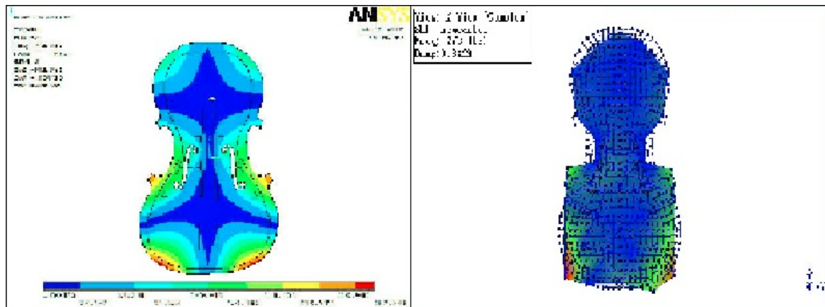
Fig. 4.29 Comparison of Mode 5 of the composite plate #2 by the FEM and the Modal Analysis
