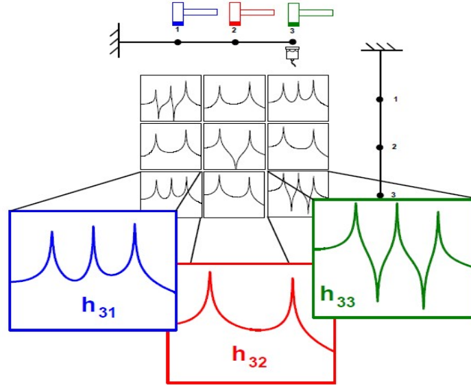
Fig. 3.6 Typical setup for a roving impact hammer test on a cantilever beam [3]
