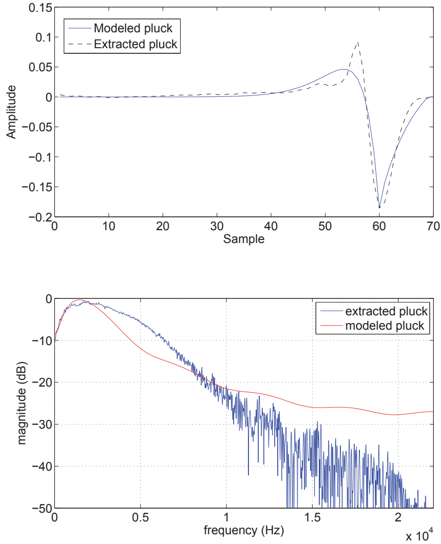
Fig. 4.29 Extracted excitation and modeled excitation. Top pane illustrates the extracted excitation and the modeled excitation in the time domain. \alpha(1|0) = 18 , \epsilon(1|0) = 9 . The bottom pane illustrates the magnitude responses of the extracted and modeled excitations.
