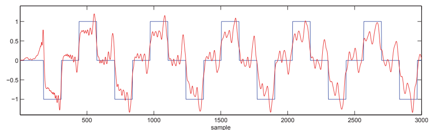
Fig. 4.8 Recorded signal y(n) and the impulse response v_{N_{pu}}(n) .
