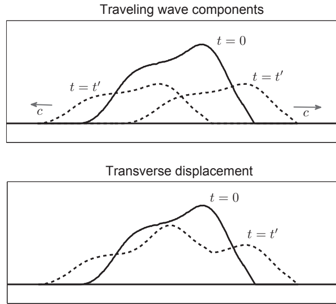
Fig. 4.1 Traveling wave components and the transverse displacement. The waveforms shown in the top pane are the right-going and the left-going traveling wave components at time t = 0 and t = t' . The waveforms shown in the bottom pane are the transverse displacements at time t = 0 and t = t' , sums of the two traveling wave components shown in the top pane.
