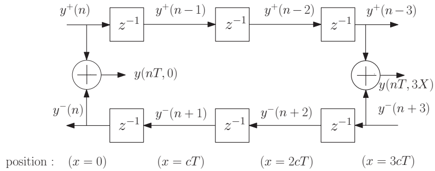
Fig. 4.2 DWG simulation of the ideal, lossless waveguide after [2]
