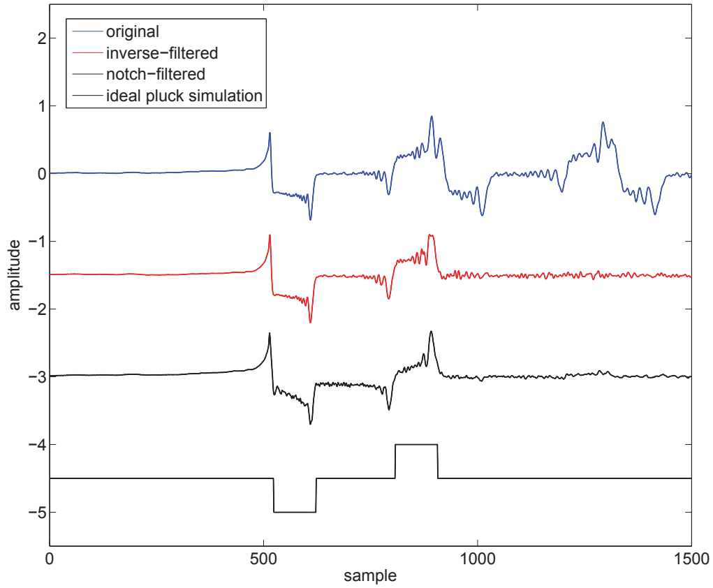
Fig. 4.19 1st: original signal. 2nd: inverse-filtered original signal. 3rd: notch-filtered original signal. 4th: the first period of the ideal plucked string SDL model.
