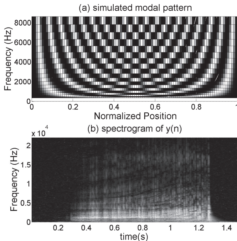
Fig. 2.7 (a) Simulated modal pattern of simply supported rectangular medium-density fiber (MDF) plate (Width: 0.95m, height: 0.25m, thickness: 0.02m) excited by a rolling object traveling from one end to the other end of the longer side, while centered on the other axis. (b) Spectrogram of y(n) . Upwardly varying notches can be seen.
