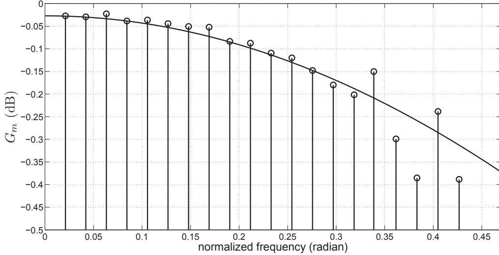
Fig. 4.17 Example of a loop gain filter. f_0 = 147.85 Hz and f_s = 44100 Hz. The hop size is 1024 samples. Circles represent measured loop gains from partial amplitude trajectories, and a single curve represents the magnitude response of H_{gain}(z) , given the filter order N = 1 , M = 1 .
