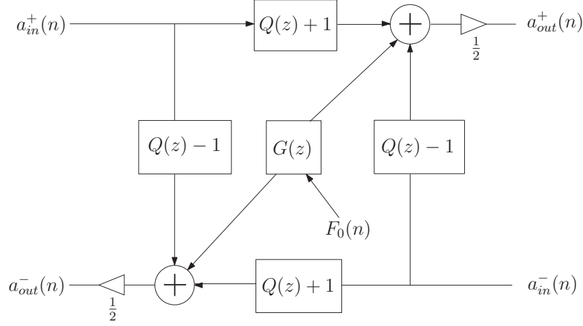
Fig. 4.31 Scattering junction at the excitation point.
