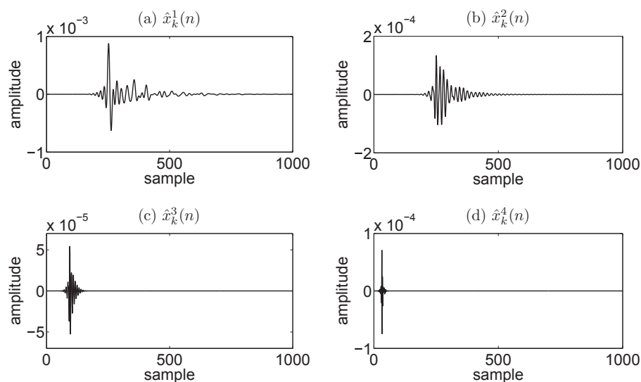
Fig. 2.10 Synthesized subband outputs ( \hat{x}_k^{(l)}(n) ): (a) \hat{x}_k^{(1)}(n) , (b) \hat{x}_k^{(2)}(n) , (c) \hat{x}_k^{(3)}(n) , (d) \hat{x}_k^{(4)}(n) .
