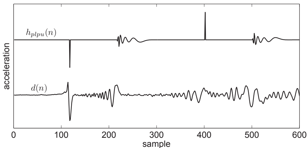
Fig. 4.24 h_{plpu}(n) and d(n) . Amplitudes (acceleration) are normalized for the comparison.
