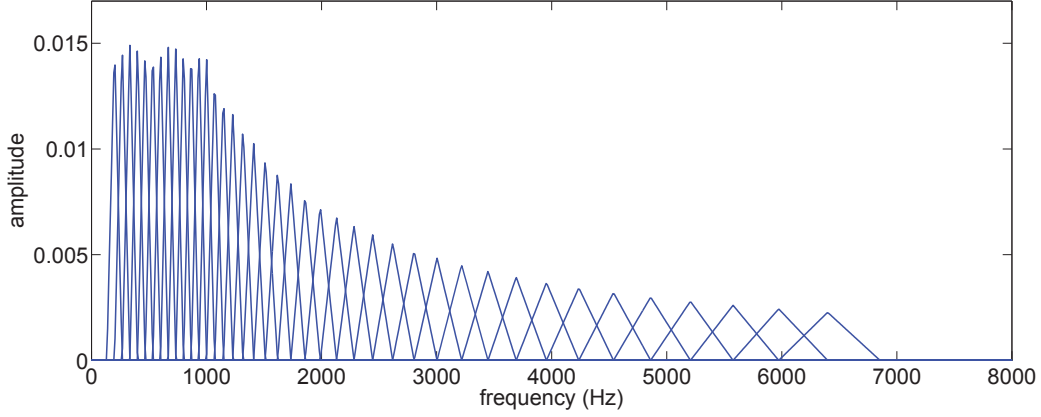
Fig. 3.8 Triangular mel-scale filter bank from Auditory toolbox [1].
