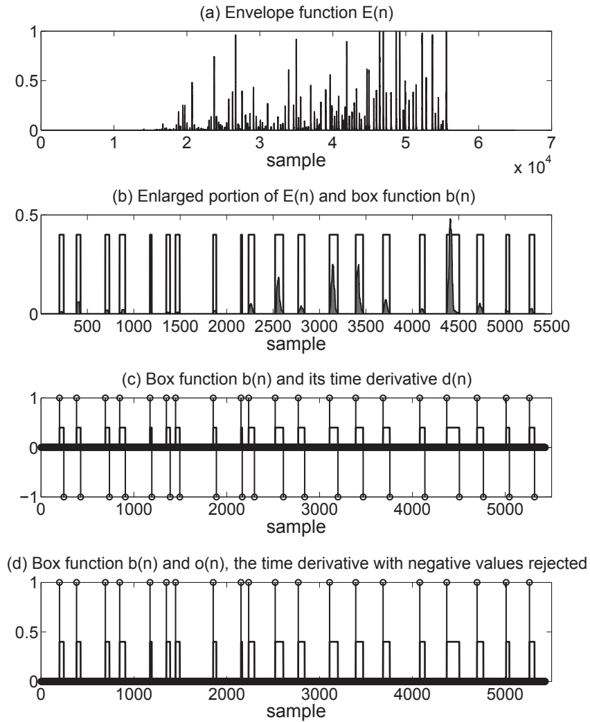
Fig. 2.2 (a) Envelope function E(n) of given rolling sound y(n) . (b) Enlarged portion of E(n) in (a) and its associated box function b(n) (Eq. 2.2). (c) Box function b(n) from (b) and d(n) , a time derivative of b(n) (vertical lines) (Eq. 2.2), here \alpha = 1 . (d) Box function b(n) from (b) and o(n) (vertical lines).
