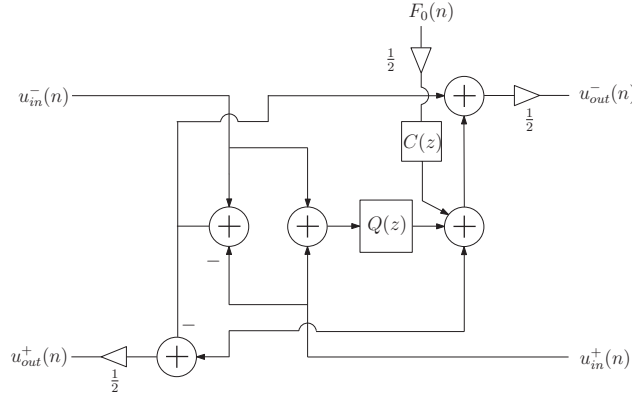
Fig. 4.30 Diagram of the plucking scattering junction, from [3] (slightly modified).
