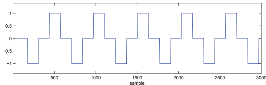
Fig. 4.7 The impulse response of the DW string model v_{N_{pu}}(n) obtained by integrating a_{N_{pu}}(n) .
