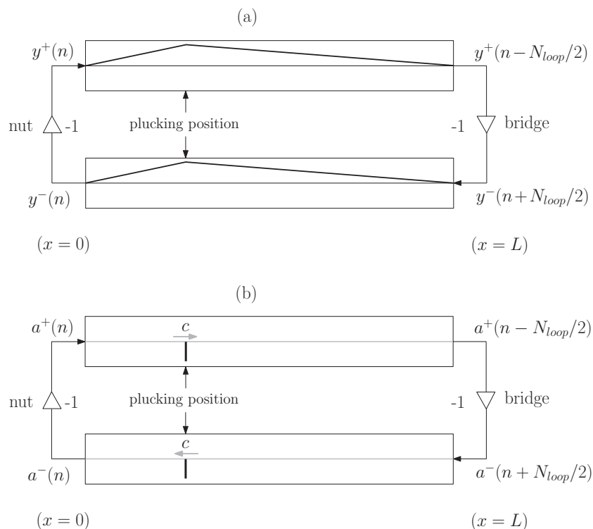
Fig. 4.3 Ideal plucked string digital waveguide models. (a) A simulation using wave variables of displacement y(n) . The initial condition y(0, x) is characterized by the shapes loaded in the delay lines. (b) A simulation using wave variables of acceleration a(n) . The initial condition a(0, x) is characterized by the impulses loaded in the delay lines. All figures are after [2].
