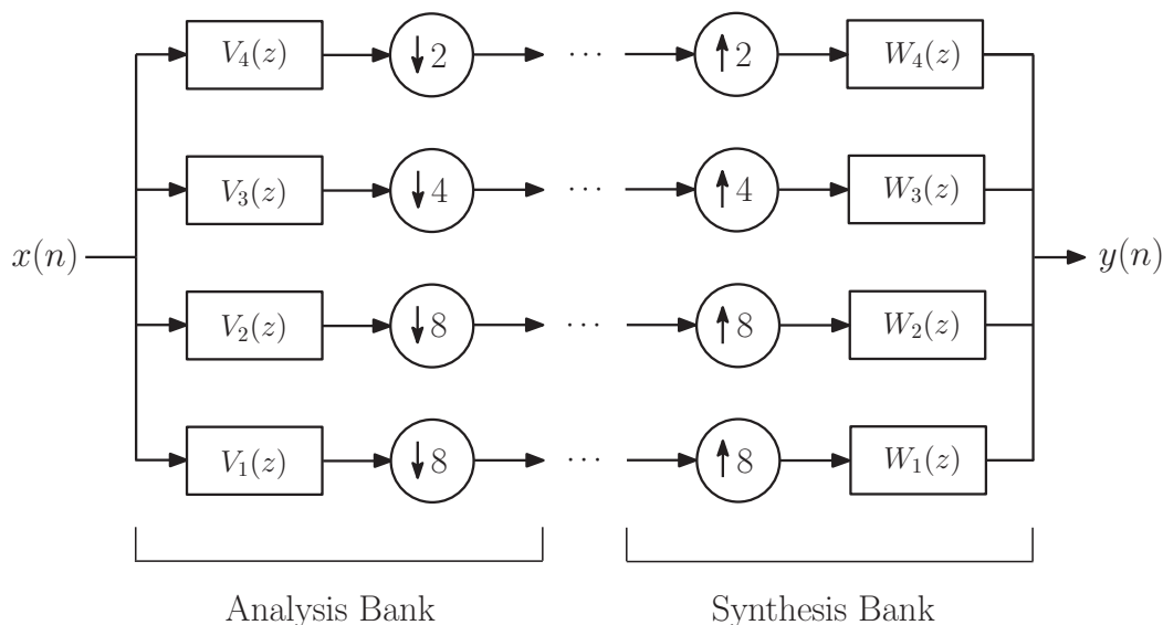
Fig. 2.6 Non-uniform 4-band filter.
