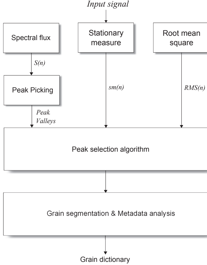
Fig. 3.2 Overview of granular analysis system. S(n) , sm(n) and RMS(n) are defined in Eqs. 3.2, 3.7 and 3.5, respectively.
