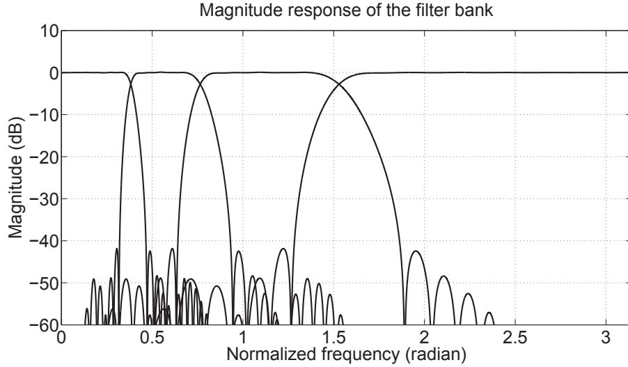
Fig. 2.5 Magnitude response of the filter bank.
