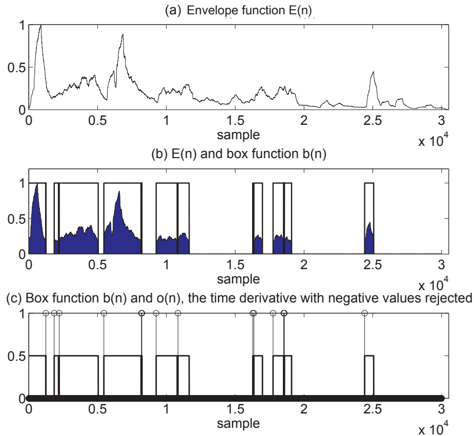
Fig. 2.13 (a) Envelope function E(n) of a rolling sound generated by rolling a steel ball on a steel plate. (b) E(n) in (a) and its associated box function b(n) . (c) Box function b(n) from (b) and o(n) .
