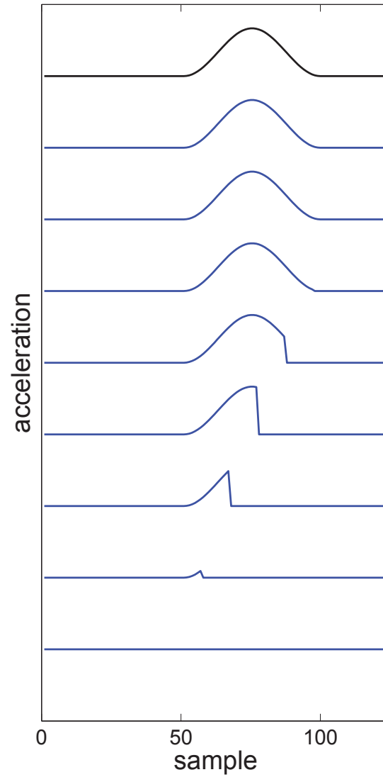
Fig. 4.23 Updates of the RLS filter \mathbf{w}(n) , temporally updated from the bottom to the top. The black one at the very top is the original signal.
