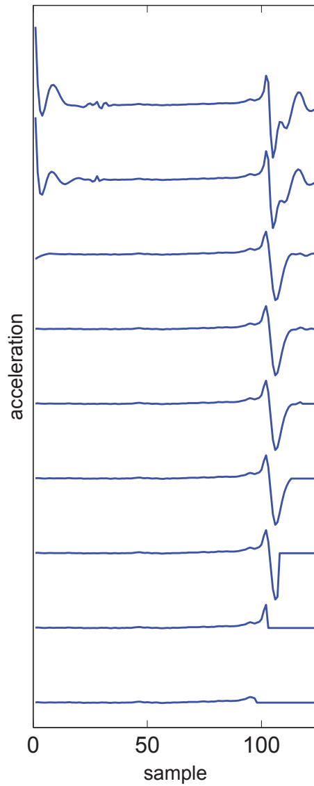
Fig. 4.25 Updates of the RLS filter \mathbf{w}(n) , temporally updated from the bottom to the top.
