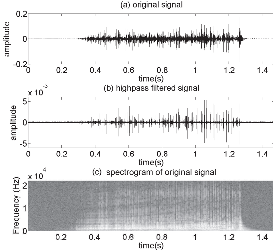
Fig. 2.1 Top: Original rolling sound y(n) . Middle: High-pass filtered rolling sound y_{hp}(n) . Bottom: Spectrogram of y(n) .
