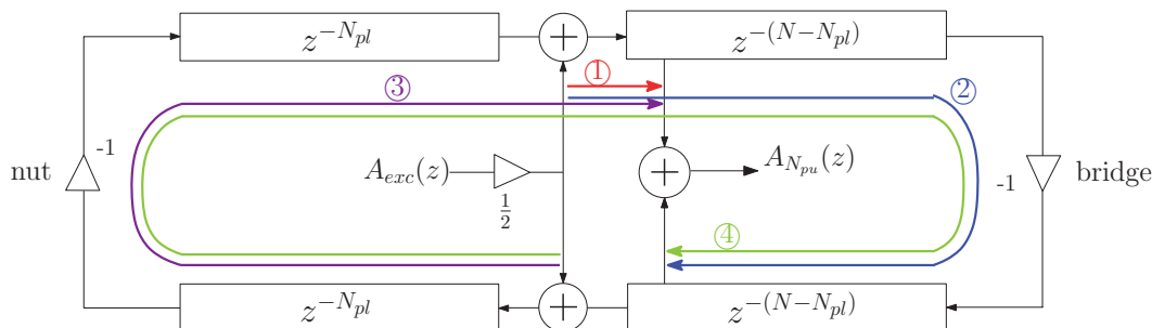
Fig. 4.14 Paths of the traveling impulses in the digital waveguide model of the ideal plucked string. The circled numbers indicate the paths of pulses in the order of arrival at the pickup position, corresponding to those in Fig.(4.15).
