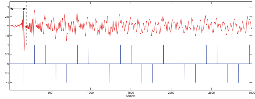
Fig. 4.9 Top: differentiated recorded signal y'(n) . The portion under the arrow is \tilde{a}_{exc}(n) . Bottom: a_{L_p}(n)
