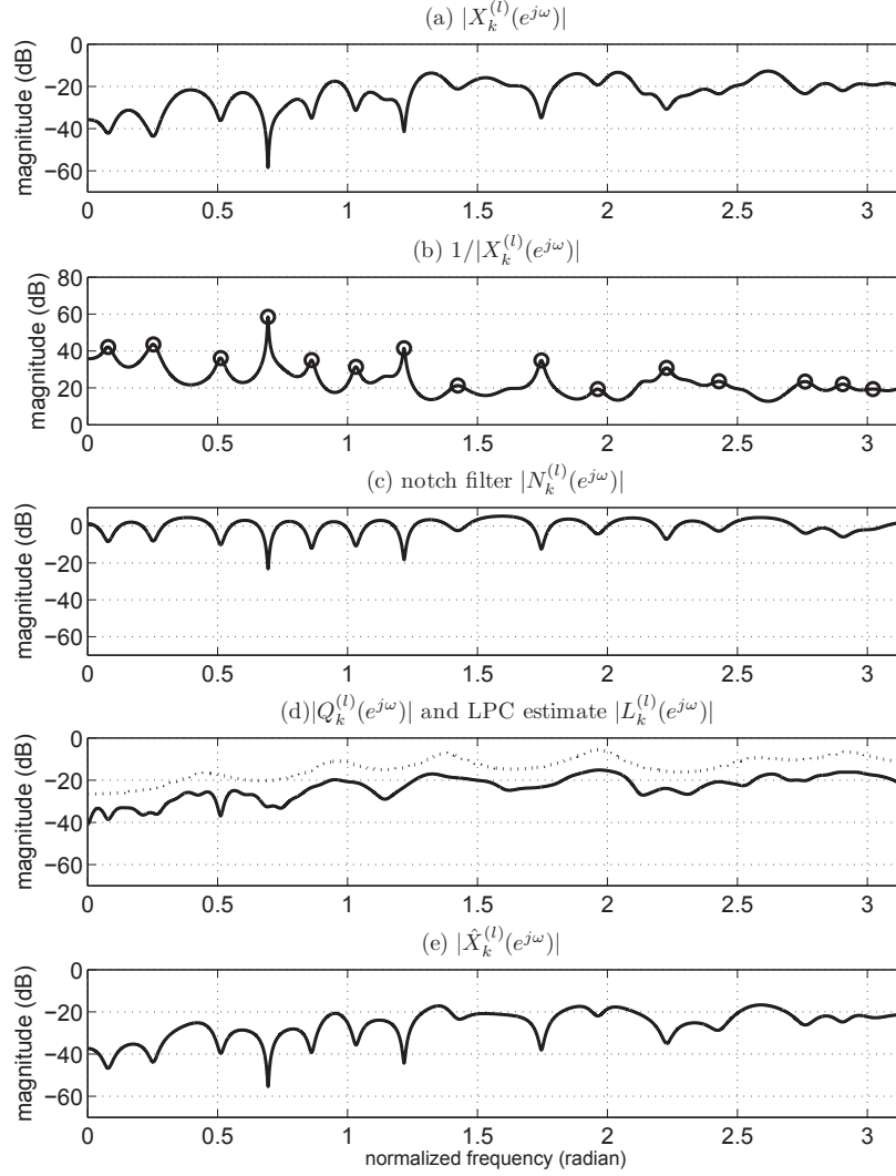
Fig. 2.8 (a) Magnitude of X_k^{(l)}(e^{j\omega}) . (b) Magnitude of 1/X_k^{(l)}(e^{j\omega}) . Circle marks denote detected peaks. (c) Magnitude response of the notch filter N_k^{(l)}(e^{j\omega}) . (d) Magnitudes of Q_k^{(l)}(e^{j\omega}) (solid) and its LP estimate L_k^{(l)}(e^{j\omega}) (dashed). (e) Magnitude of \hat{X}_k^{(l)}(e^{j\omega}) . In all figures, x -axes denote normalized radian frequencies.
