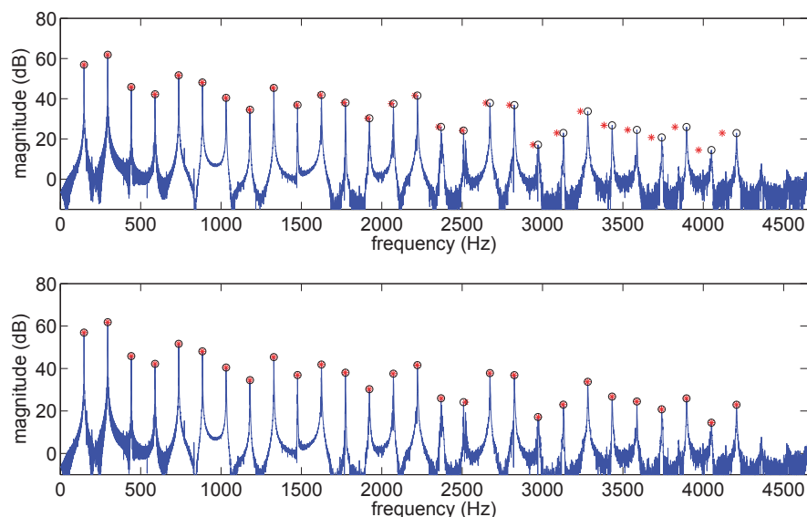
Fig. 4.18 Comparison of the spectrum of a recorded plucked string sound and the theoretical harmonics. Blue line is the magnitude response of the recorded plucked string (the low open D string of an electric guitar) sound. Black circles represent the peaks of magnitude responses. Red stars(*) are theoretical harmonics. Top: theoretical harmonics are just the multiples of the fundamental frequency. Bottom: theoretical harmonics are adjusted according to the formula of Eq. 4.42 given the estimated B .
