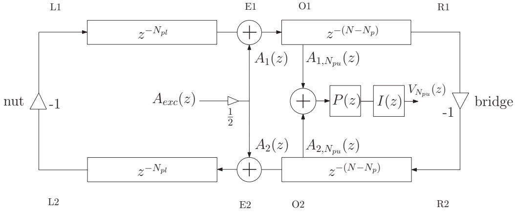
Fig. 4.5 Acceleration wave variable-based digital waveguide plucked string model with rigid terminations.
