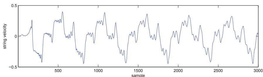
Fig. 4.4 Beginning of a plucked string sound observed through electromagnetic pickup.
