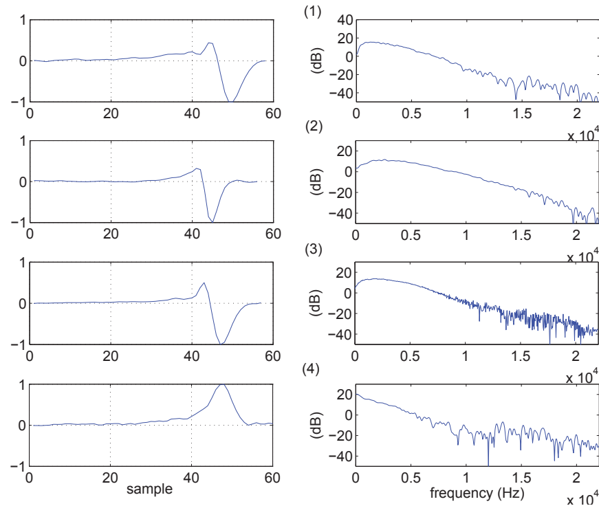
Fig. 4.26 Examples of extracted excitations. Figures on the left side are extracted excitations and those on the right side are the spectra of the extracted excitations. Amplitudes of extracted excitations are normalized for the comparison.
