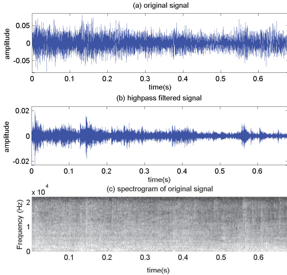
Fig. 2.11 Top : Original rolling sound. A steel ball rolling on a steel plate. Middle : High-pass filtered rolling sound. Bottom : Spectrogram of the original sound.
