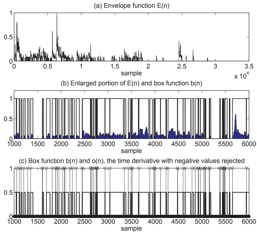
Fig. 2.12 (a) Envelope function E(n) of a rolling sound generated by rolling a steel ball on a steel plate. (b) Enlarged portion of E(n) in (a) and its associated box function b(n) . (c) Box function b(n) from (b) and o(n) .
