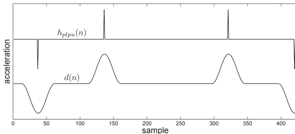
Fig. 4.22 h_{ptpu}(n) and d(n) of the synthesized plucked string sound using an ideal DWG model and a Hann window.
