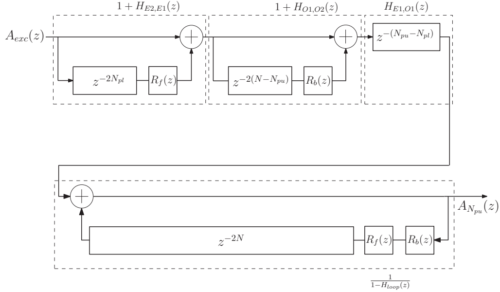
Fig. 4.13 SDL model of the plucked string.
