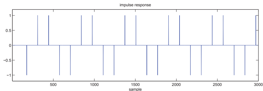
Fig. 4.6 The impulse response of the DW string model a_{N_{pu}}(n) in acceleration prior to entering the pickup.
