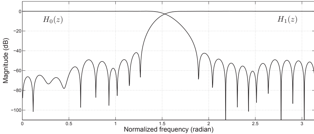
Fig. 2.3 Magnitude responses of a two channel QMF.
