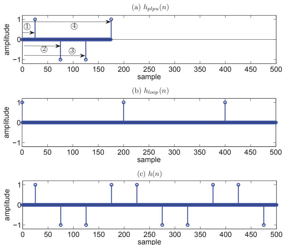
Fig. 4.15 Impulse responses of H_{plpu}(z) , H_{loop}(z) and H(z)
