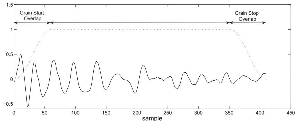
Fig. 3.9 Window used for gap filling. ‘Grain Start Overlap’ and ‘Grain Stop Overlap’ and the length of the grain determine the overall length of the window.
