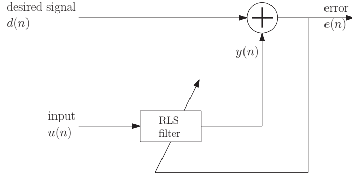
Fig. 4.21 RLS filter
