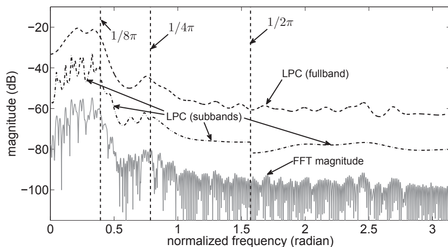
Fig. 2.9 Magnitudes of X_k(z) and its syntheses. Gray line is the magnitude plot of X_k(e^{j\omega}) and black dotted line is the full band LPC estimate with order 45. Black dash-dotted lines are the magnitude responses of the LPC estimates of the subbands' signal from the lowest subband to the highest subband, respectively (zero estimates are not considered). LPC orders are 25, 10, 5, 5, from the lowest to the highest, respectively.
