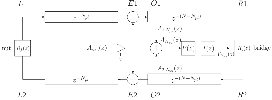
Fig. 4.12 Digital waveguide structure of the non-ideal plucked string.
