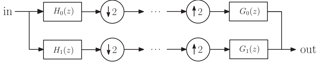
Fig. 2.4 Two channel QMF bank.
