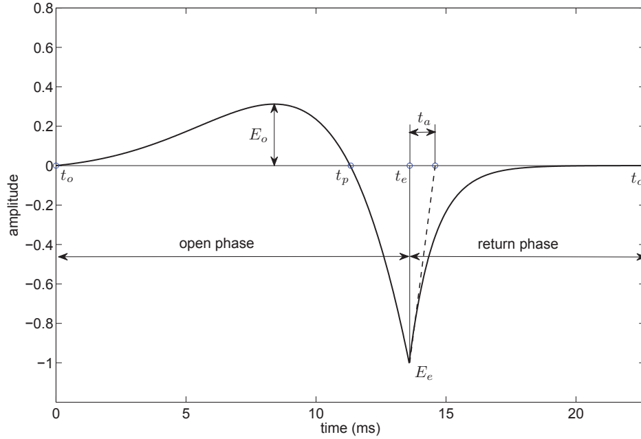
Fig. 4.28 LF model
