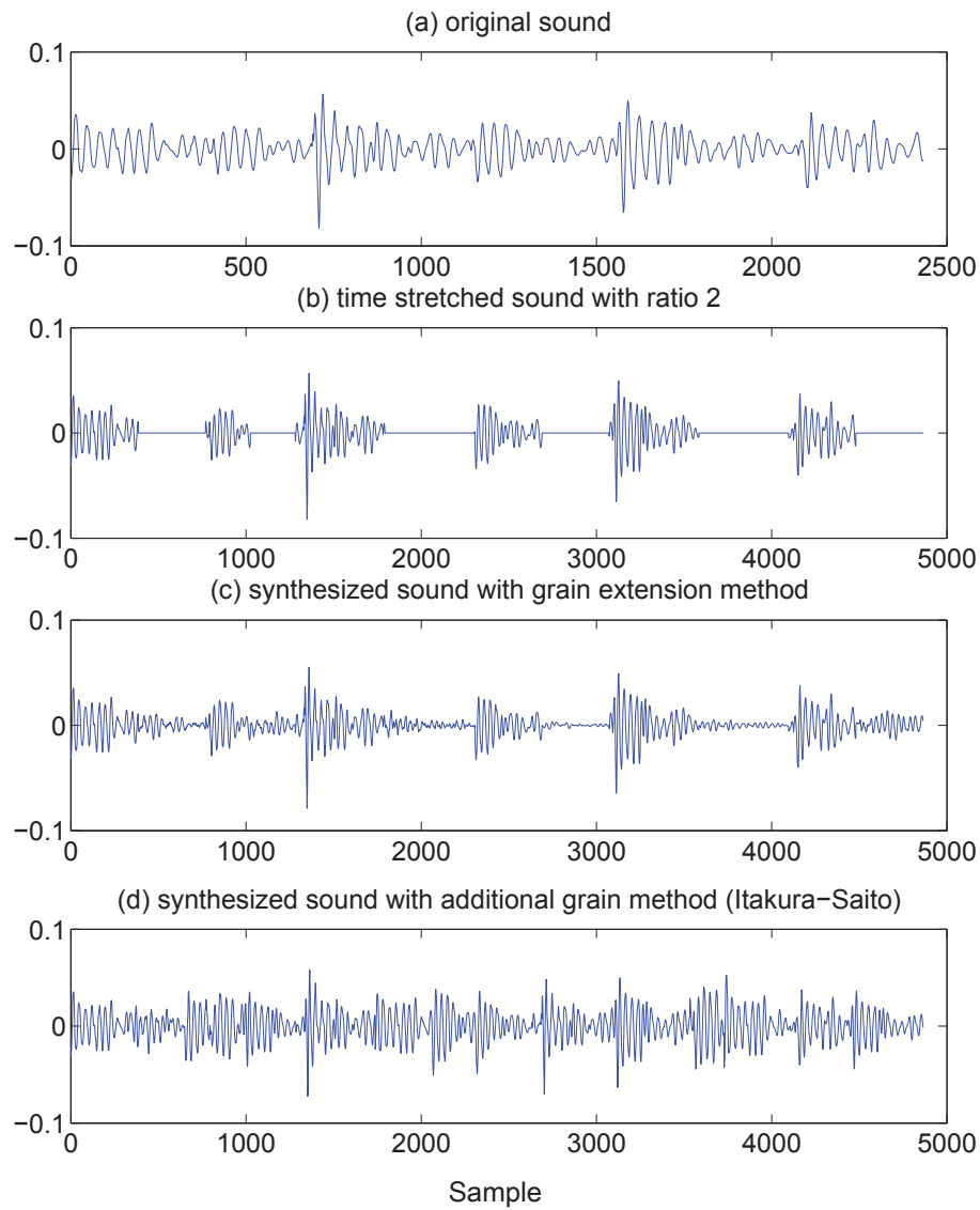
Fig. 3.10 (a) Original sound. (b) Original sound stretched with the time stretch factor \alpha = 2 . (c) Gap filling with the grain extension method. (d) Gap filling with the additional grain method.
