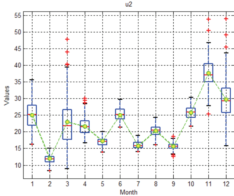
Figure 4-31: Comparison between Simulated and Empirical \mu_2 (Roxas City)
