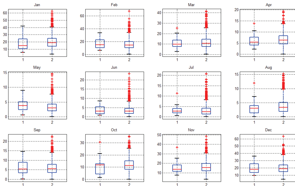
Figure 4-35: Monthly Std Deviations of Daily Rainfalls (mm) for Sooke Reservoir 1 – Observed, 2 - Simulated
