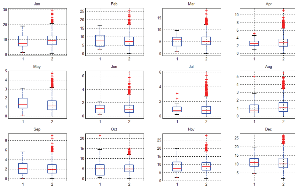
Figure 4-34: Monthly Means of Daily Rainfalls (mm) for Sooke Reservoir 1 – Observed, 2 - Simulated
