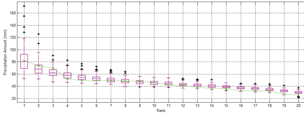
Figure 4-72: CGCM - Ranked AMP Boxplots vs Observed Series (1961-1980)
