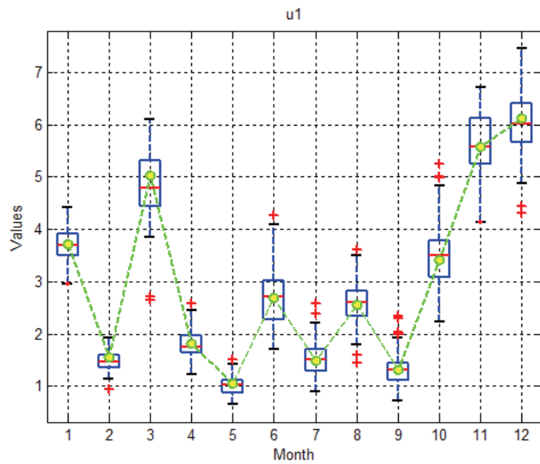
Figure 4-30: Comparison between Simulated and Empirical \mu_1 (Roxas City)
