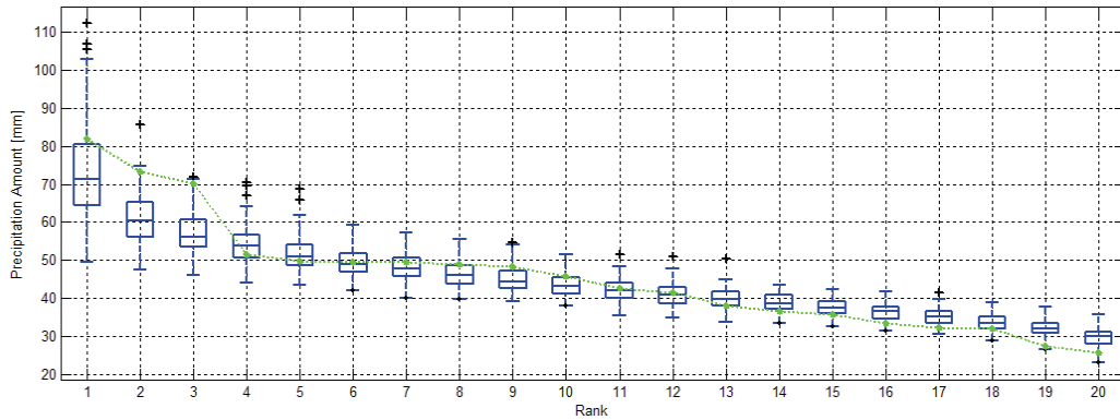
Figure 4-73: HadCM3 - Ranked AMP Boxplots vs Observed Series (1961-1980)
