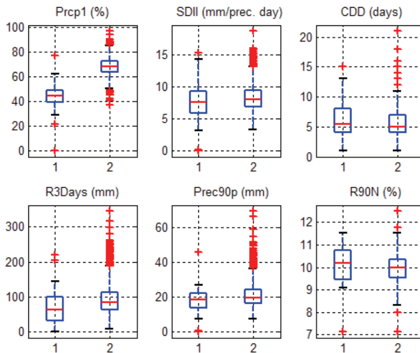
Figure 4-46: Indices for December to February (Roxas City): 1 – Observed, 2 - Simulated
