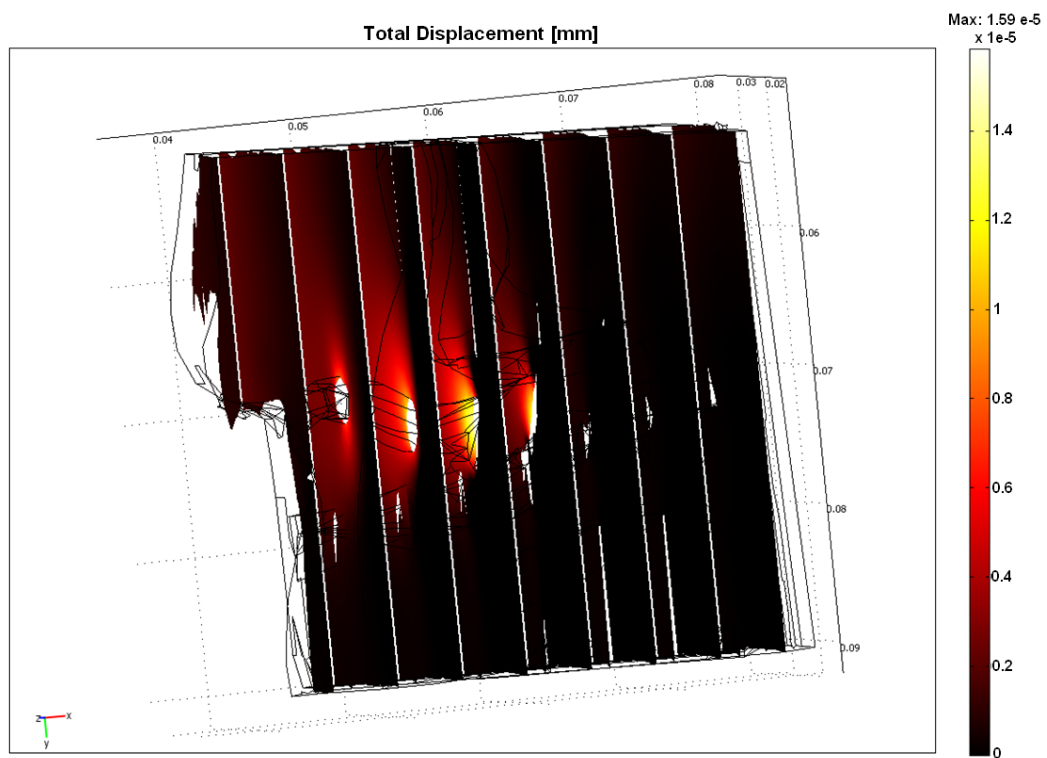
Figure 5.2 Displacement results of ear-canal model. Larger displacements are focused on the canal boundary.
