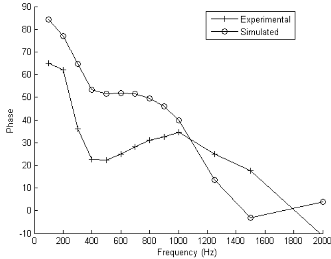
Figure 5.13 Admittance phase comparison.
