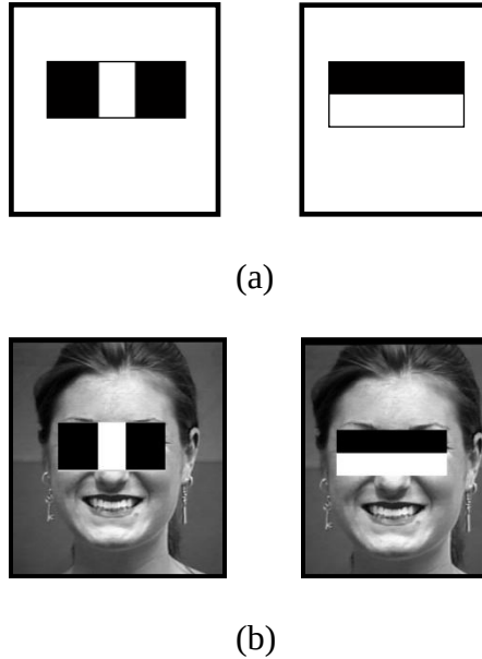
Figure 3-7: (a) First two ranked Haar-like feature used for Viola-Jones face detector (b) Haar-like features overlapped on a face image. Face image © Jeffrey Cohn.
