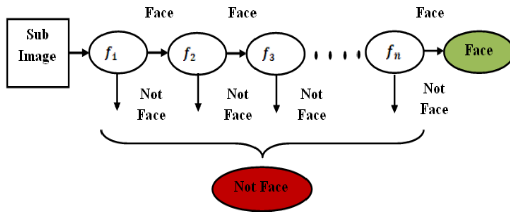
Figure 3-9: Cascade classifier: The sub-region in the image which contains the presence of all the features is classified as “Face”, and others are classified as “Not Face”.
