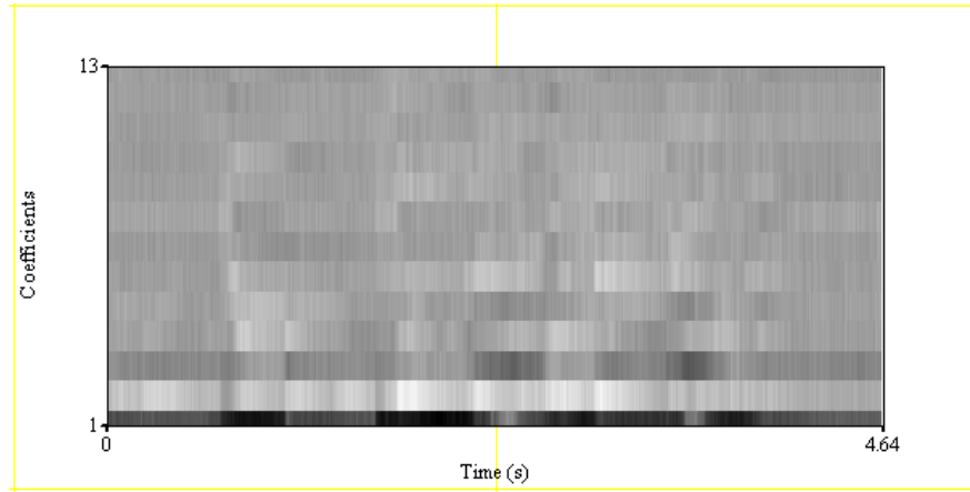
Figure 3-4: 13 MFCC of the speech signal represented in Figure 3-2.
