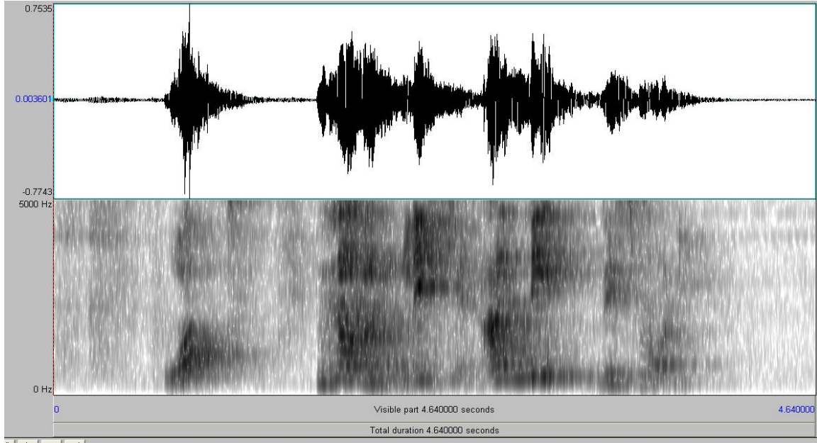
Figure 3-5: Speech signal and its spectrogram.
