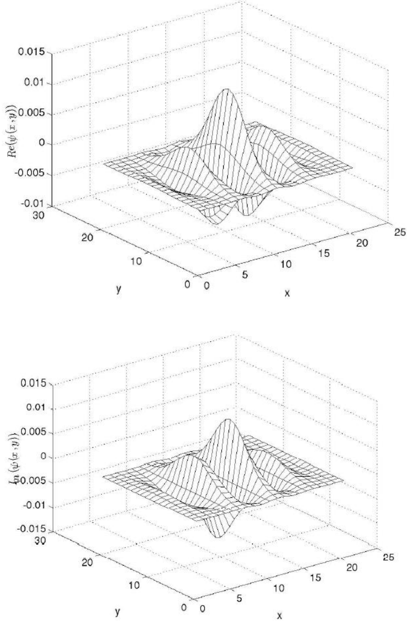
Figure 3-11: 2-d Gabor filter in spatial domain with real (top) and imaginary (bottom) components, f_0 = 0.2 , \gamma = \eta = 1 .
