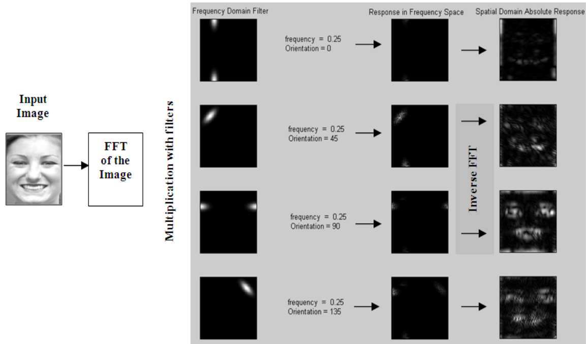
Figure 3-13: Frequency domain filtering process. Face image © Jeffrey Cohn.
