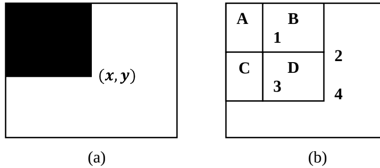
Figure 3-8: Integral image from Viola-Jones face detector. (a) Pixel location (x, y) , contains the sum of pixels in the black shaded region. (b) The sum of pixels in D is
