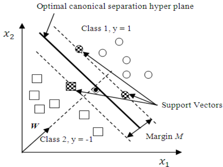
Figure 4-1: Illustration of two dimensional SVM model with separating plane represented by bold line and the two parallel planes with support vectors in the dotted lines.
