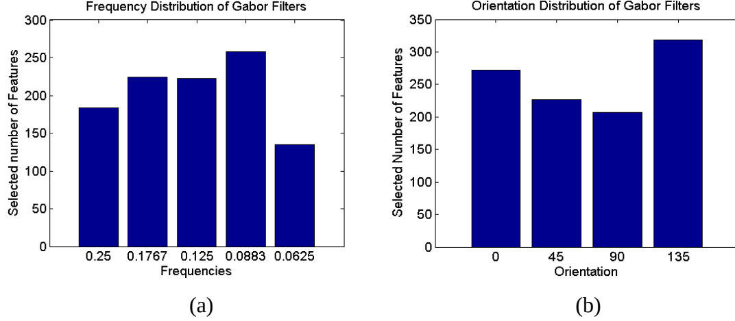
Figure 4-5: Distribution of the Gabor features selected in terms of frequencies and orientations
