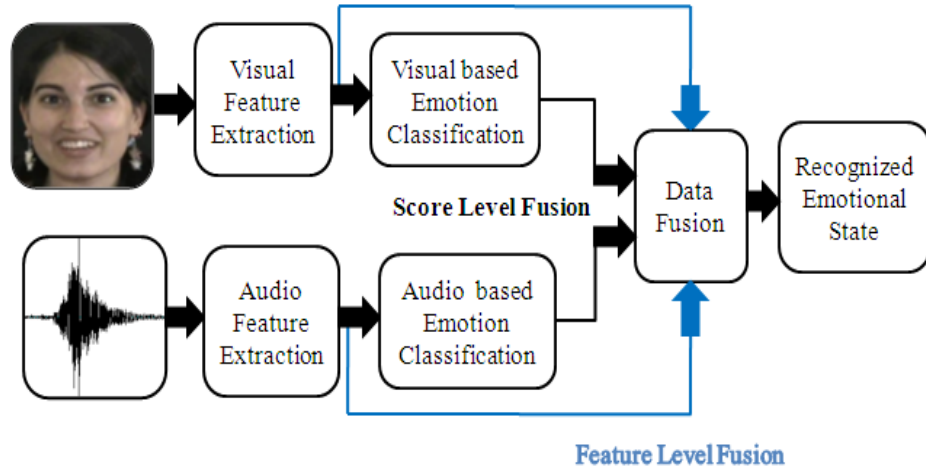
Figure 1-2: Bimodal emotion recognition system.
