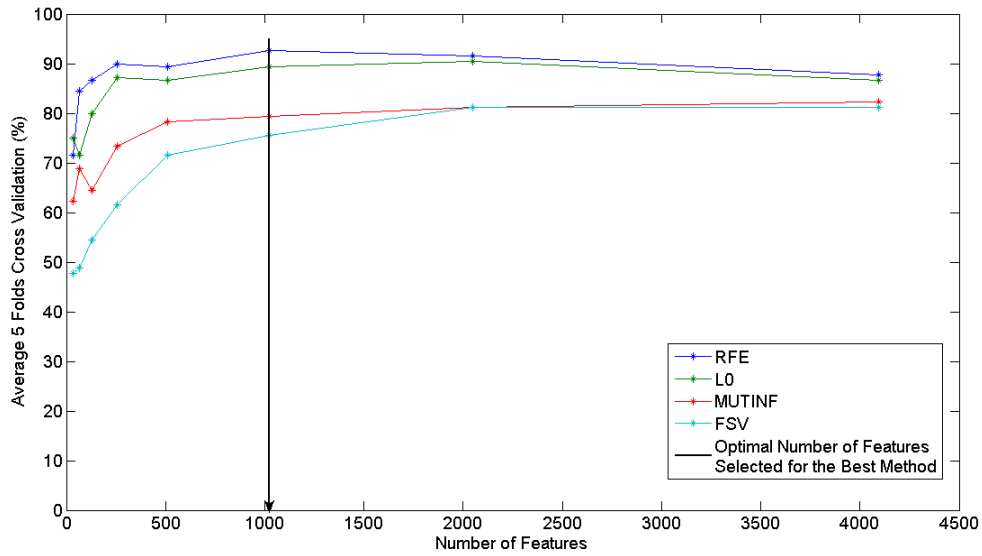
Figure 4-3(b): Evaluation of best visual feature selection method with optimal number of features.
