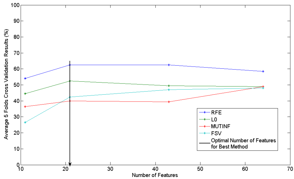
Figure 4-3 (a): Evaluation of best audio feature selection method with optimal number of features.
