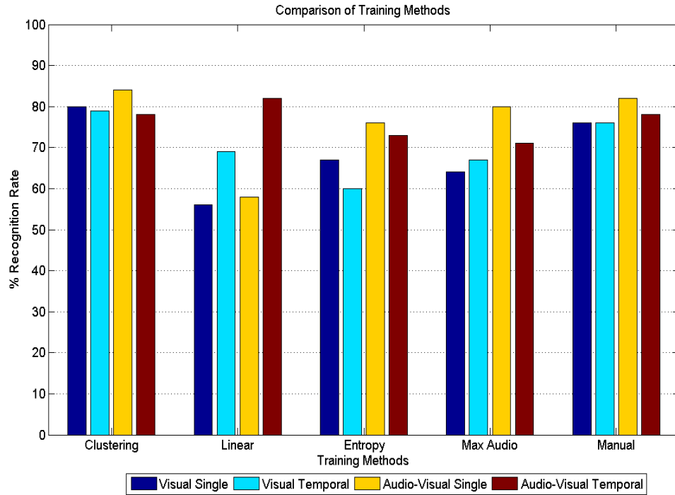
Figure 5-7: Comparison of Training Methods
