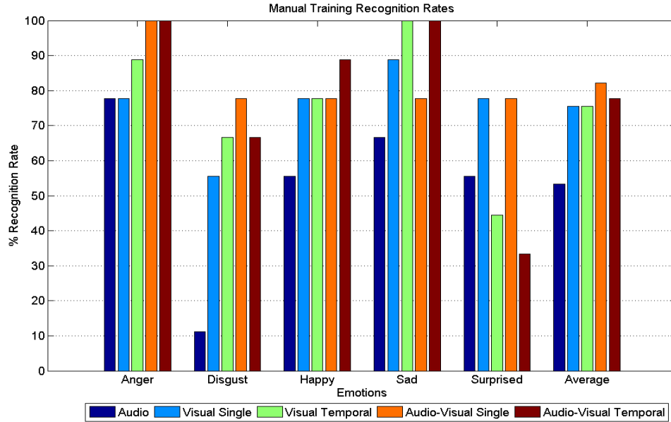
Figure 5-9: (% Correct) Recognition Rates for Manual Training Approach
