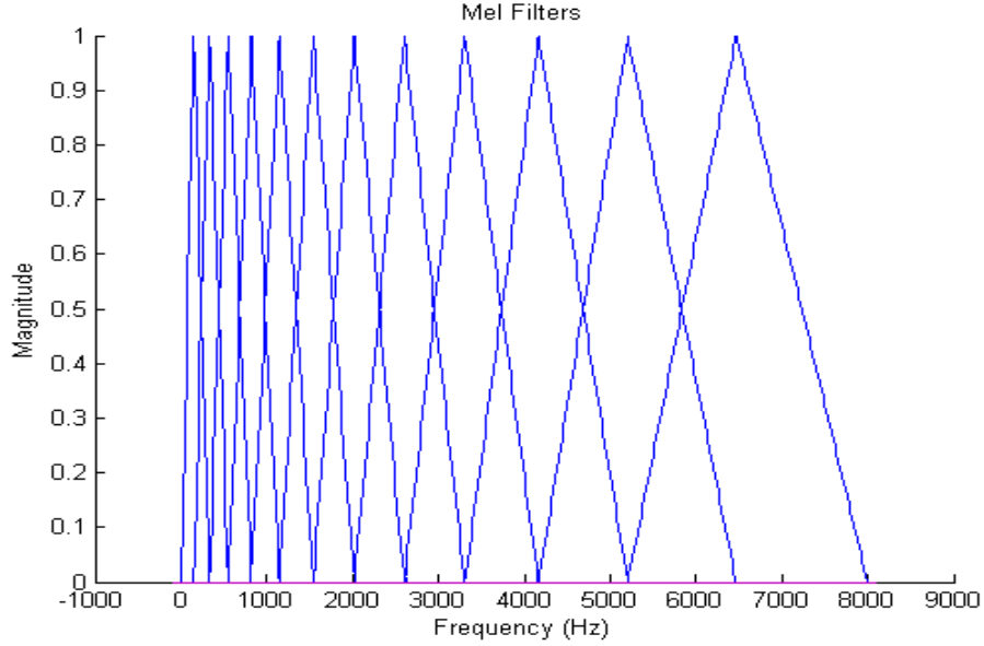
Figure 3-3: Bank of triangular filters used for Mel-Cepstrum analysis, given by:
