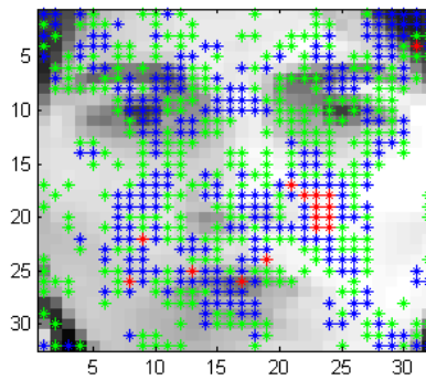
Figure 4-4(b): Spatial locations of Gabor features selected using RFE for all emotion classes
