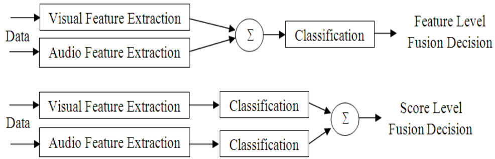
Figure 5-6: Feature-Level (above) and Score-Level Fusion (below) Techniques
