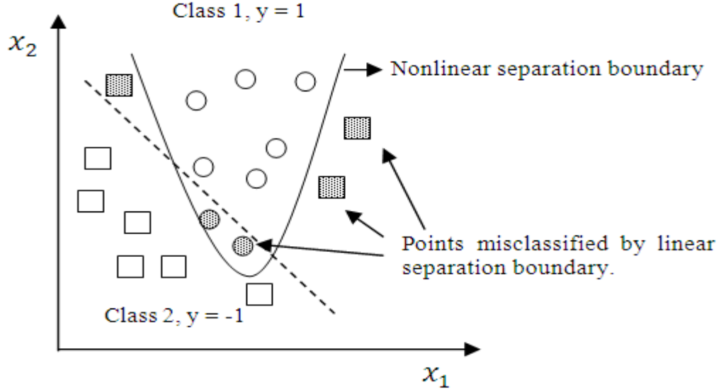
Figure 4-2: Non-linear SVM (Following [44]).
