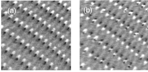
FIG. 5. MFM images of particle array with particle size of 1.2 \mu\text{m} \times 200 \text{ nm} . (a) remanent state after saturation; (b) in the presence of external field of 60 Oe along long axis. tip: 50-nm CoPtCr, tip-sample separation: 80 nm; in vacuum.
