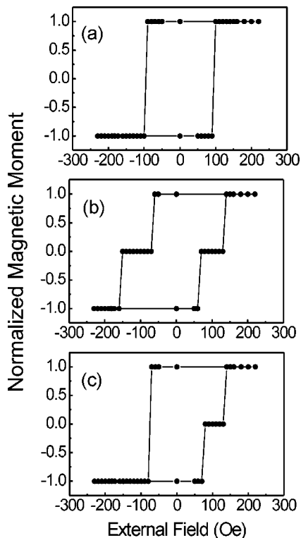
FIG. 9. Remanent hysteresis of three different individual particles in Fig. 8.
