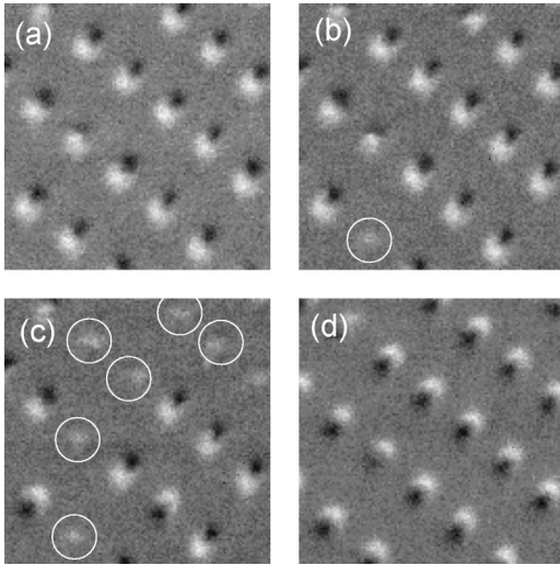
FIG. 8. Reversal as a function of external magnetic field after saturation at -250 Oe, (a) 50 Oe, (b) 70 Oe, (c) 90 Oe, (d) 180 Oe. Particle size: 800 nm \times 200 nm; circled: low moment states.
