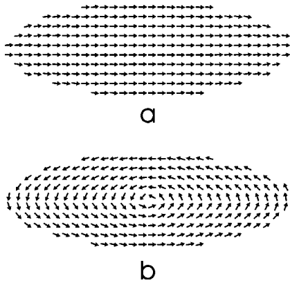
FIG. 11. Two different state in an elliptical particle. (a) single domain; (b) one vortex. Particle size 600 \text{ nm} \times 200 \text{ nm} \times 30 \text{ nm} ; unit size: 10^3 \text{ nm}^3 .
