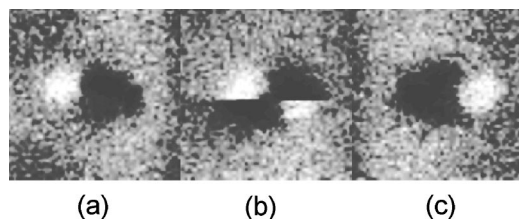
FIG. 3. (a)–(c) Three consecutive scans of the same 500\text{ nm} \times 200\text{ nm} particle; The tip is a 60-nm permalloy coated probe, and the images are acquired in air using the tapping/lift mode with a lift height of 80 nm on a DI Multimode Nanoscope.
