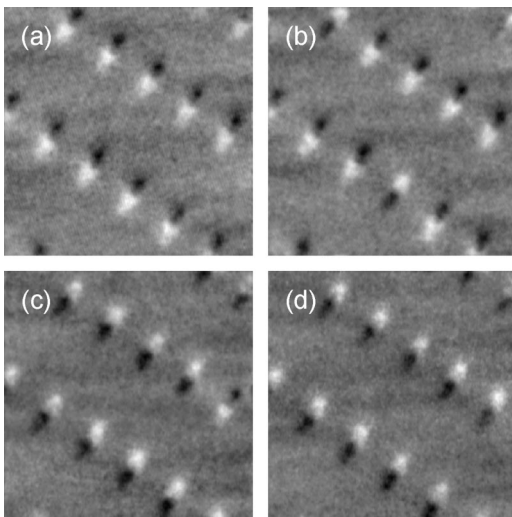
FIG. 6. Magnetization reversal as a function of external magnetic field. Imaged in the remanent states after the field ramped along particle long axis. (a) -200 Oe; (b) 75 Oe; (c) 90 Oe; (d) 101 Oe. Particle size: 1.2 \mu\text{m} \times 200 \text{ nm} , tip: 50-nm CoPtCr, lift height 120 nm.
