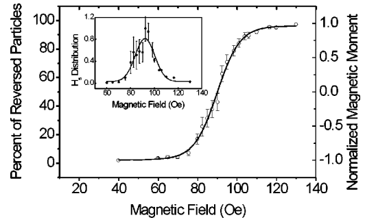
FIG. 7. (a) Percentage of reversal as function of field. Particle aspect ratio 7:1, width 200 nm; inset: switching field histogram.
