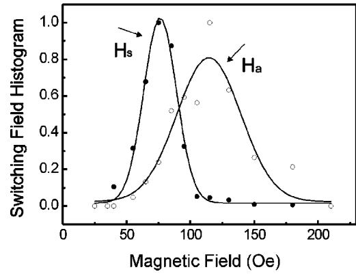
FIG. 10. Switching field histogram of the particle array with particle size of 800 nm \times 200 nm.
