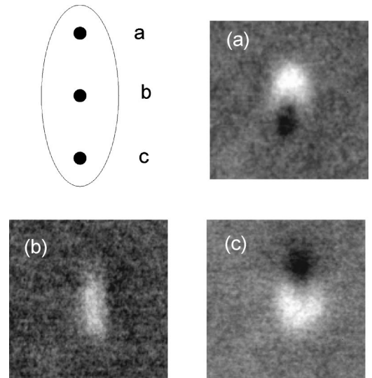
FIG. 12. Local tip stray field induced magnetization reversal. Tip located at different position above the particle can lead to different magnetic states: (a), (b), and (c). Tip: 50-nm CoPtCr, constant height mode in vacuum, particle size 600 \text{ nm} \times 150 \text{ nm} .
