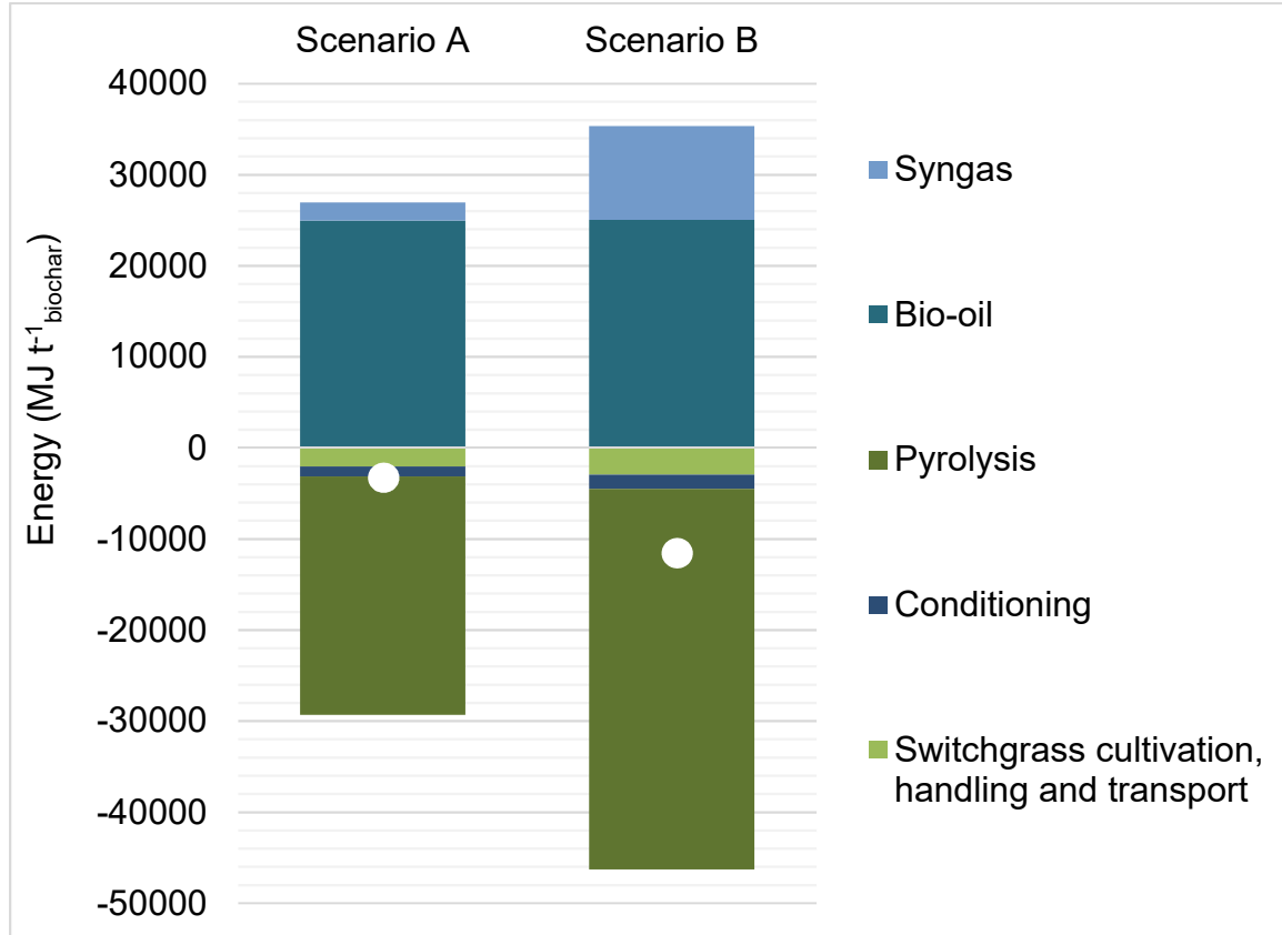
Figure 6.2: Energy balance of scenarios A and B ( \text{MJ t}^{-1} \text{ biochar} )
