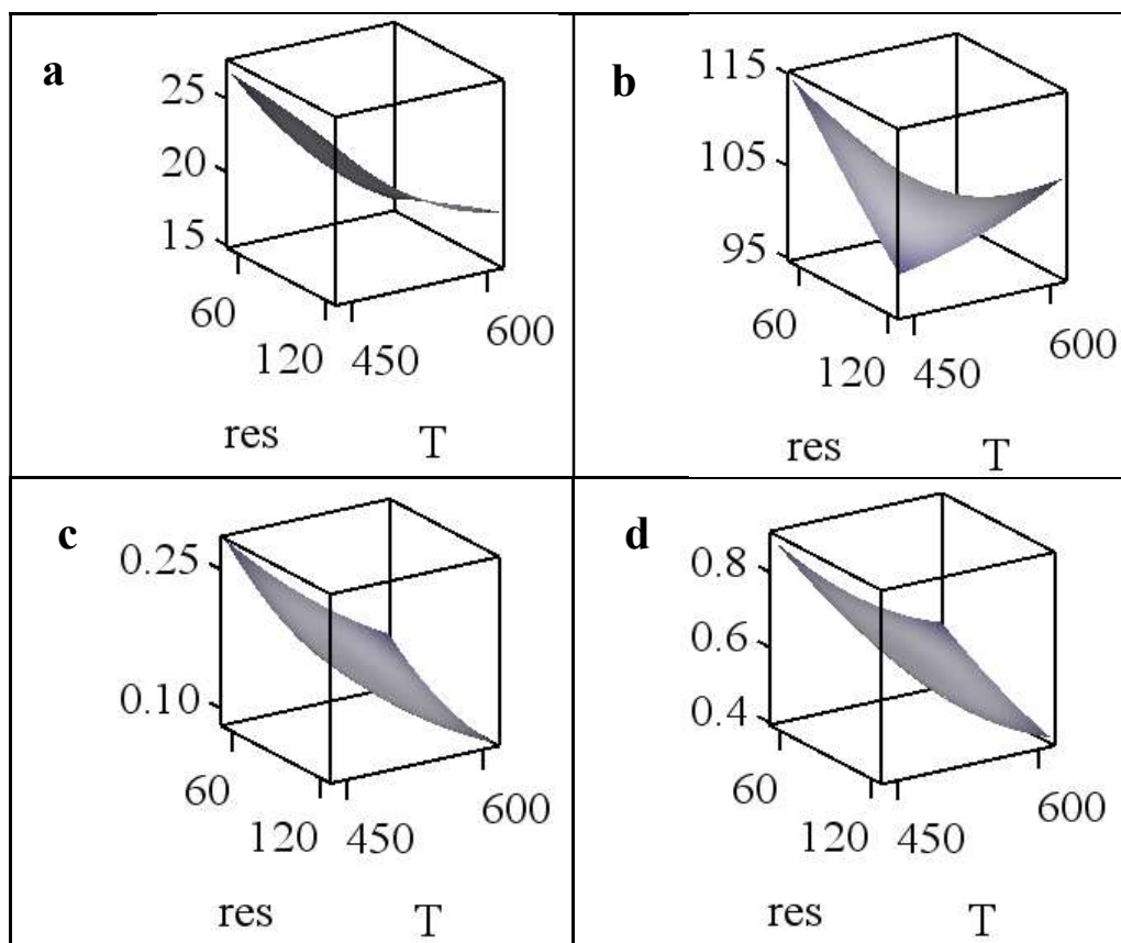
a) biochar yield; b) C/N ratio; c) O/C org ratio; d) H/C org ratio. res : residence time of biomass in the reactor; T : pyrolysis temperature. Nitrogen flowrate was fixed at 3.1 L min -1
