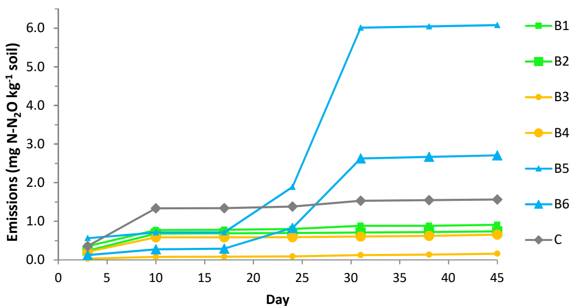
Figure 5.3: Cumulative emissions of N 2 O (mg N-N 2 O kg -1 soil) after the 45-days incubation period in the silt loam – Mean value of three replicates
