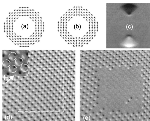
FIG. 2. Magnetic moment orientation of (a) vortex state and (b) onion state by micromagnetic simulations (see Ref. 10); (c) the z component of the stray field of (b) in a plane 40 nm above the ring; (d) MFM image at an external field of 60 Oe after a field of 300 Oe is applied; (e) MFM image at a field of 60 Oe after scanning the square area indicated in (d) at remanence. Scan area: 15 \mu m. Inset of (d) shows a smaller scan area, allowing comparison with (a) and (c). The arrow in (d) indicates the direction of the applied field. Tip: 30 nm CoPtCr; f_0 = 97.8 kHz; tip sample separation: 100 \pm 20 nm. Constant height images in vacuum. Inset in (d) shows an image in small scan size, and the white box in (d) is the 10 \mu m scan area at remanence.
