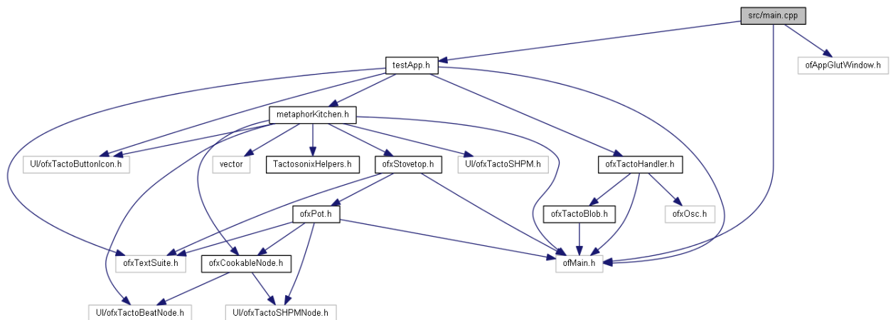
Fig. A.1 Dependency graph for main.cpp, the entry point for TactoSonix. Note the presence of the metaphorKitchen class, which most importantly includes a Stacked Half-Pie Menu (class ofxTactoSHPM ) and a stovetop (class ofxStoveTop ). This graph shows how TactoSonix was designed to allow for the implementation of multiple metaphors.
