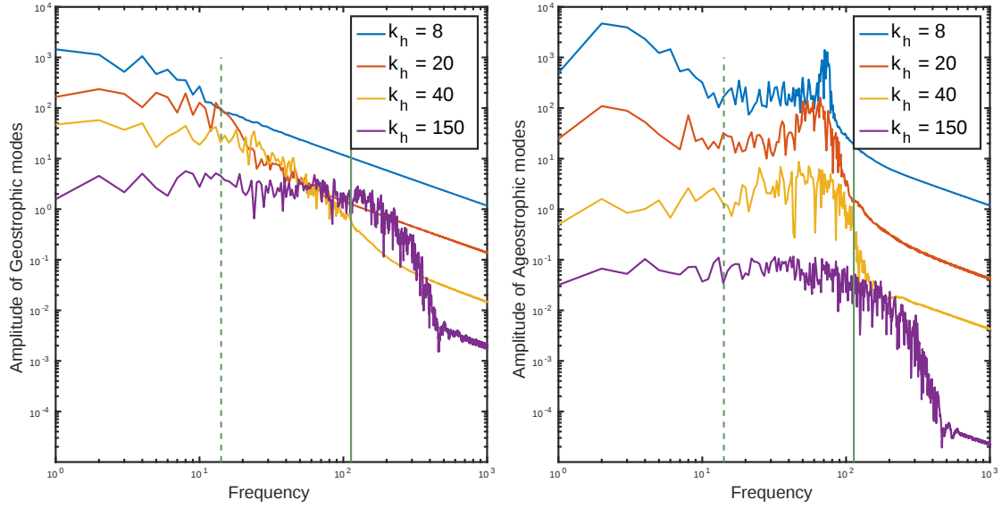
Figure 3–9: The frequency spectra of geostrophic (left) and ageostrophic (right) modes. The simulation is run at Ro = 0.03 , and 16000 points are sampled from t = 0 to t = 4\tau . The dashed and the solid vertical lines represent f and N , respectively. For clarity the ageostrophic spectra of k_h = 40 , k_h = 20 and k_h = 8 are vertically offset by one, two and three decades, respectively.
