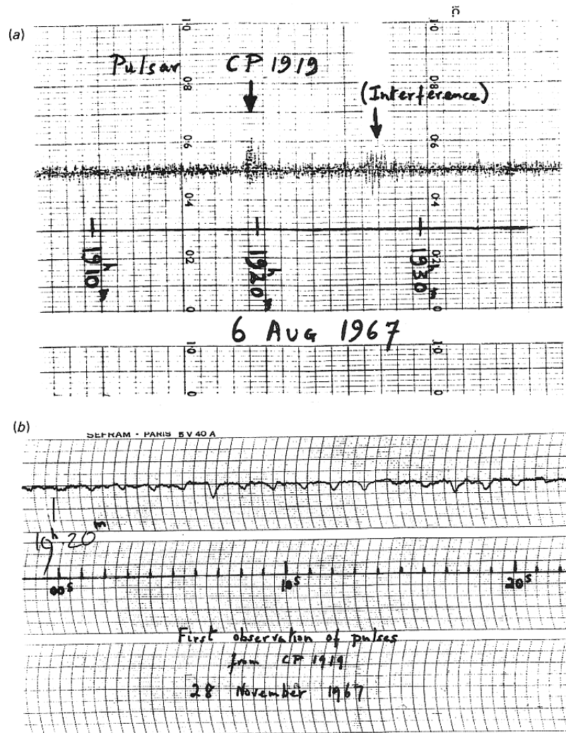
Figure 2-1: The discovery of the first pulsar. The ‘scruff’ found by Jocelyn Bell (top, marked “CP 1919”, and the first pulses observed from a pulsar (bottom) [81].
