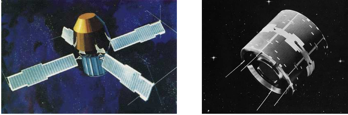
Figure 1–3: Left: the SAS-2 satellite was launched in 1972, and performed gamma ray observations for approximately seven months. Figure from [102]. Right: the COS-B satellite was launched in 1975, and operated for approximately seven years. Figure from [99].
