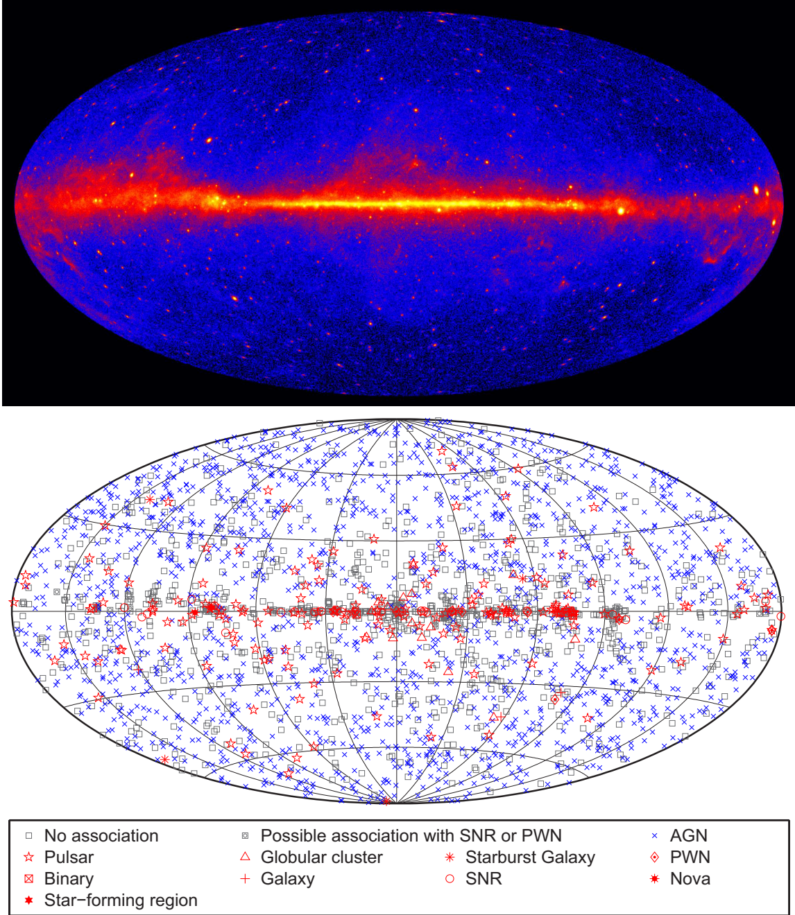
Figure 1–7: Top: a detailed view of the HE gamma-ray sky produced by Fermi LAT. Figure from [62]. Bottom: the locations of the 3033 sources listed in the Fermi Large Area Telescope third source catalogue in galactic coordinates. Figure from [32].
