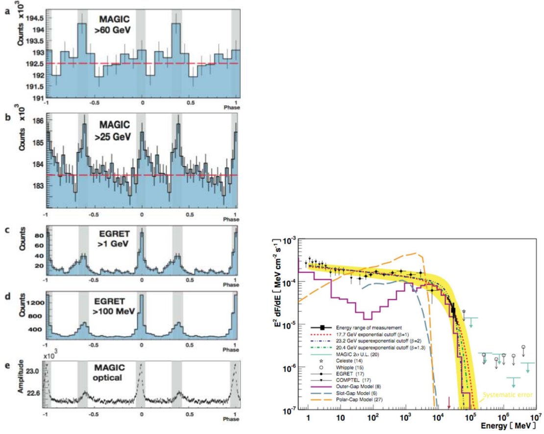
Figure 3-4: The MAGIC collaboration announced the detection of the Crab pulsar in 2008, the first detection of a pulsar by an IACT. Left: the pulse profiles of the Crab as measured by MAGIC above 25 and 60 GeV. The pulse profiles of the Crab as measured by EGRET aboard the CGRO are also shown, as is the optical profile as measured by MAGIC. Right: the spectrum of the Crab pulsar measured by various instruments, including the MAGIC spectral points. The spectrum is fit with an outer gap model, and presented a challenge for slot gap and polar cap models. Figures from [37].
