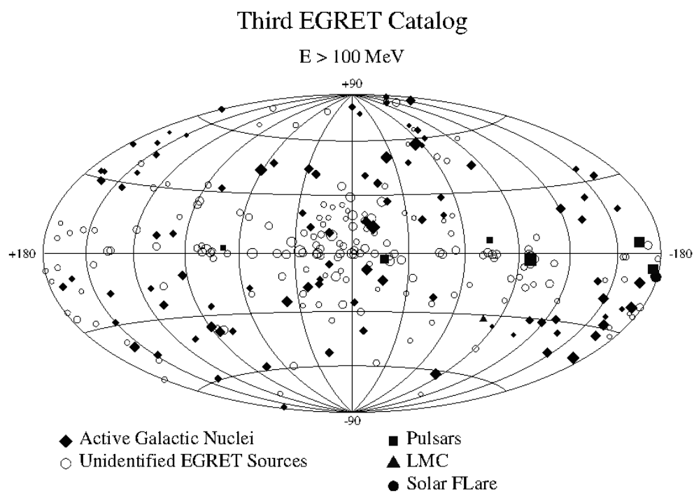
Figure 1–6: Top: the first map of the full sky in HE gamma rays, produced by EGRET. Bottom: the locations of the 271 sources in the third EGRET catalogue in galactic coordinates. Figures from [118].
