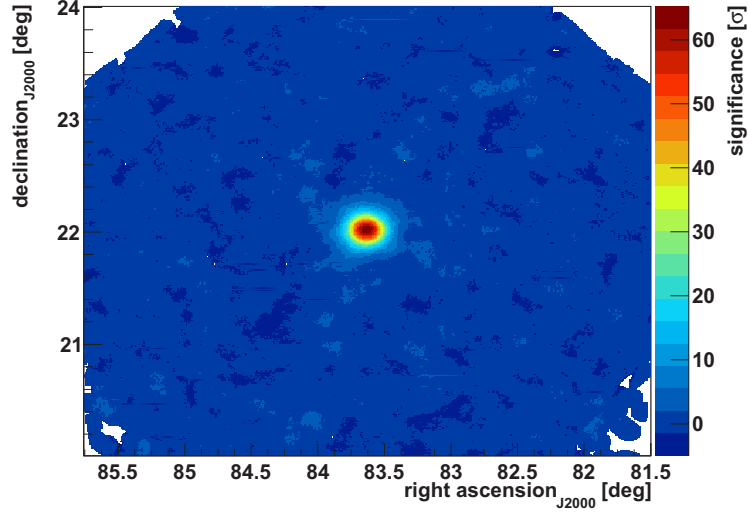
Figure 5–9: A correlated significance skymap produced with six hours of VERITAS Crab nebula data.
