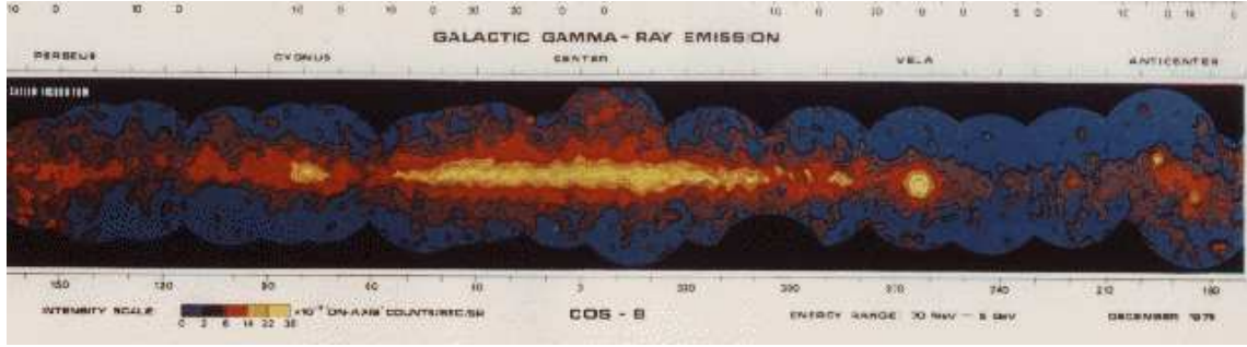
Figure 1–4: The first map of the galactic plane in gamma rays, produced by COS-B. Figure from [100].
