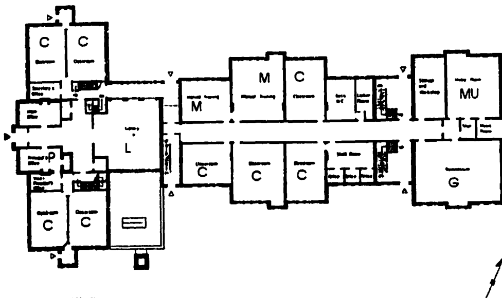
GROUND-FLOOR PLAN
