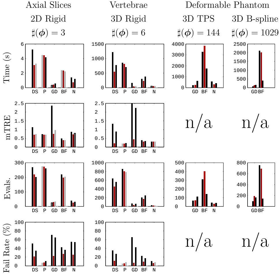
Figure 4.21 Comparison of registration results for realistic registration problems with different scale factors. Due to its poor performance the NSCL case was not used for these experiments. The optimizers are identified as DS – downhill simplex, P – Powell's, GD – gradient descent, BFGS – Broyden-Fletcher-Goldfarb-Shanno, N – Newton-Raphson. For each optimizer, the bars represent, from left to right, the result using the scale factors x10, x1, and x0.1. Case x1, the optimal scale factor, is identified in red. If the results of the other cases differ in a statistically significant way from case x1 they are shown in black. Ambiguous results (see Section 3.2.1) are shown with black outline, and results that are not significantly different from case x1 are shown in gray. mTRE is in mm for all cases. mTRE is analyzed separately for the deformable transform case, and failure rate does not apply.
