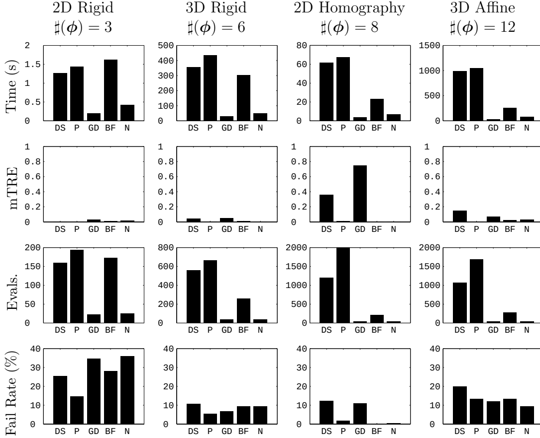
Figure 4.28 Comparison of registration results for transforms with different numbers of parameters using the mutual information cost function. The optimizers are identified as DS – downhill simplex, P – Powell's, GD – gradient descent, BFGS – Broyden-Fletcher-Goldfarb-Shanno, N – Newton-Raphson. mTRE is in mm for all cases except the homography, where it is in pixels. The datasets used were: 2D Rigid – Sagittal Brain Slice; 3D Rigid and Affine – Brainweb; 2D Homography – Agra Fort. Note that the vertical scale is not the same in all cases.
