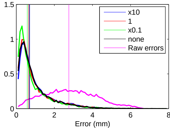
Figure 4.20 Distributions of errors remaining after registration of the deformed Sagittal Brain Image using the 2D B-spline transform with the gradient descent optimizer. The image difference measure used was mutual information. This result is selected as being typical of the results of this experiment. The graph shows the distribution of errors over a 50 \times 50 grid of points in the image extent. Point errors for all 25 runs have been combined into one histogram for each set of scale factors. Vertical lines show the median error. With all scale factors, reasonably successful registration has been achieved, as shown by the distinct leftward shift in the distribution. Case x0.1 produces a slightly, but statistically significantly smaller median error.
