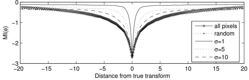
(b) Mutual Information values using different derivative scales (1% of pixels)
