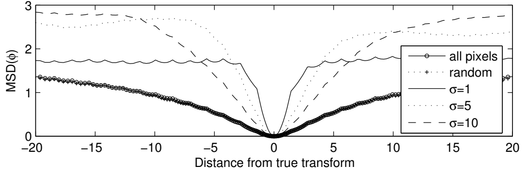
(a) Mean Squared Difference values using different derivative scales (1% of pixels)
