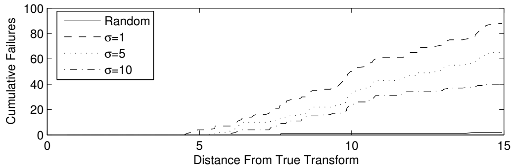
(c) Registrations of Graffiti images using Powell's method and the Tr(\mathbf{C}) criterion
