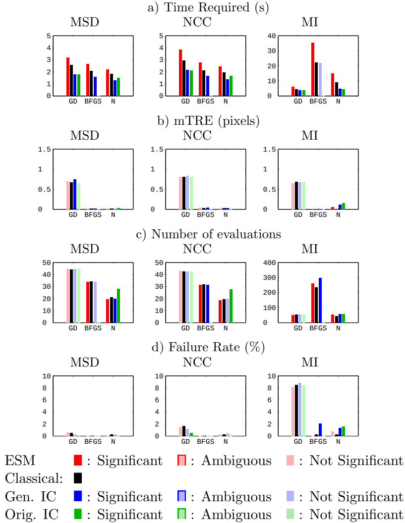
Figure 7.3 Experimental results for synthetic homographies, case 1: Starting normal distances from the true position. The optimization algorithms are Gradient Descent (GD), Broyden-Fletcher-Goldfarb-Shanno (BFGS) and Newton-Raphson (N). For each algorithm, bars are shown for the following methods from left to right: 1: ESM (Red) 2: Classical Forwards Additive (Black) 3: Generalized IC (Blue) and 4: Original IC (Green). Dark bars are statistically significantly different from classical, light bars are not significantly different and outline bars are ambiguous (see Section 3.2.1). No original IC method was implemented for the BFGS optimizer.
