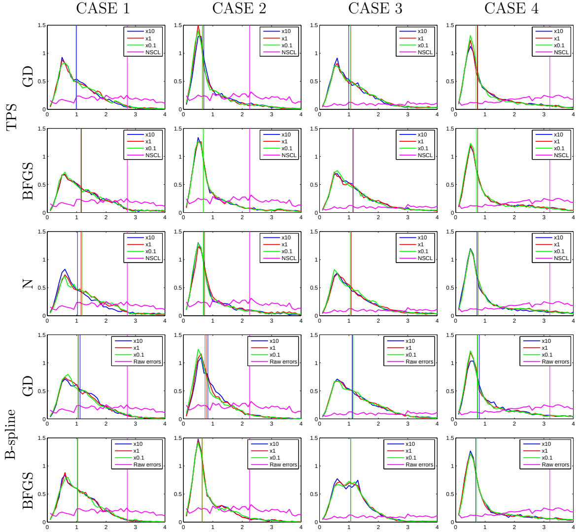
Figure D.2 The graphs show the distribution of errors over a 50 \times 50 \times 50 grid of points evenly spaced over the image extent. The image difference measure used was MSD. This result is selected as being typical of the results of this experiment. The graph shows the distribution of distances between points in a warped mesh of the balloon part of the phantom, and the mesh of the balloon created from the target volume. The vertical lines show the median of the error. Cases are (1) partially inflated to deflated, (2) partially inflated to fully inflated, (3) fully inflated to deflated, (4) fully inflated to partially inflated. For case 3, the median error for the raw data is off the graph, at 5.19mm.
