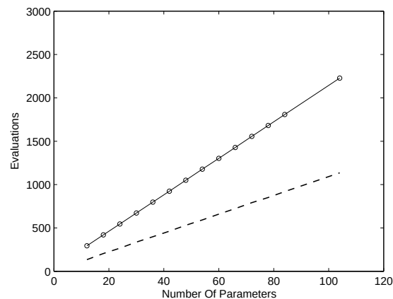
Figure 4.27 Number of evaluations required to converge when started at the minimum. For gradient based methods only one evaluation is required.
