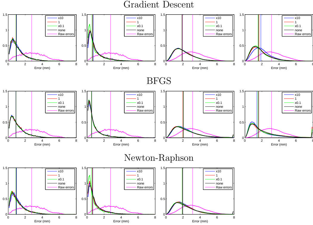
Figure D.1 Distributions of errors remaining after registration of the deformed Sagittal Brain Image using the 2D B-spline and TPS transforms, and the synthetically deformed Phantom image using the 3D B-spline and TPS transforms. The image difference measure used was mutual information, results for other cost functions are similar. The graphs show the distribution of errors over a 50 \times 50 grid ( 50 \times 50 \times 50 grid in 3D) of points in the image extent. Point errors for all 25 runs have been combined into one histogram for each set of scale factors. Vertical lines show the median error. With all scale factors, reasonably successful registration has been achieved, as shown by the distinct leftward shift in the distribution. Overall case 0.1x produces a slightly, but statistically significantly smaller median error. The 2D B-spline registration with gradient descent also appears as Figure D.1
