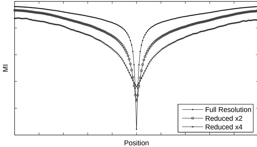
Figure 3.3 Mutual information cost function at three levels of a Gaussian scale space pyramid. The line with small dots was produced using the full resolution images, the line with circles by reduction by a factor of 2, and the line with crosses by reduction by a factor of 4. Note how the derivatives of the function become less extreme, and how the point of inflection moves further from the optimum at lower resolutions.
