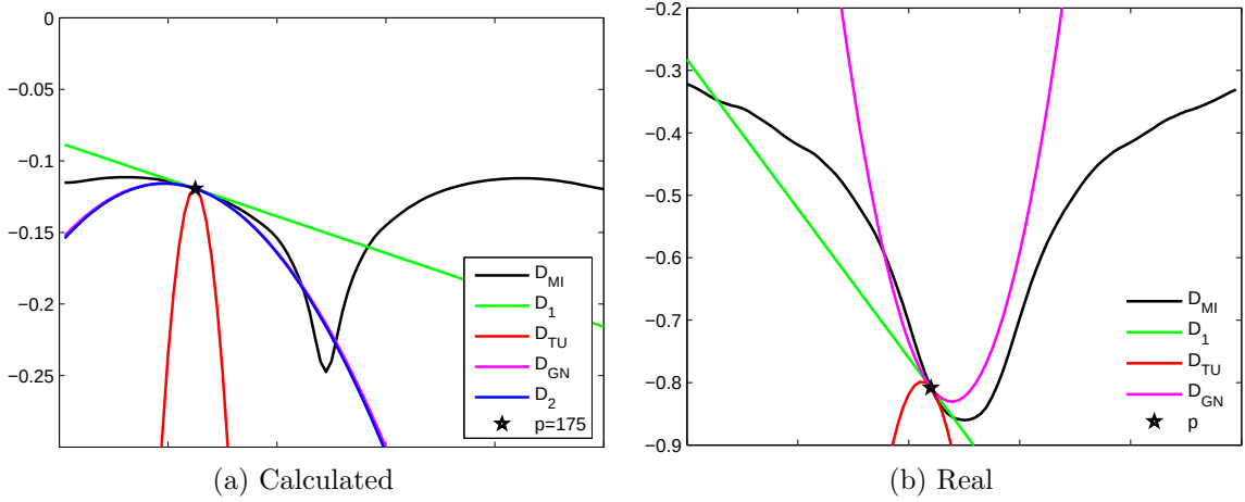
Figure 4.15 The actual function, D_{MI} , and approximations using the full Taylor series approximation, D_2 , generalized Gauss-Newton Hessian approximation, D_{GN} , the Thévenaz-Unser approximation to the Hessian, D_{TU} , and a linear approximation from the gradient, D_1 . The calculated case (left) shows the comparison on a function whose Hessian can be calculated exactly. The real case (right) shows the approximations generated from a real image.
