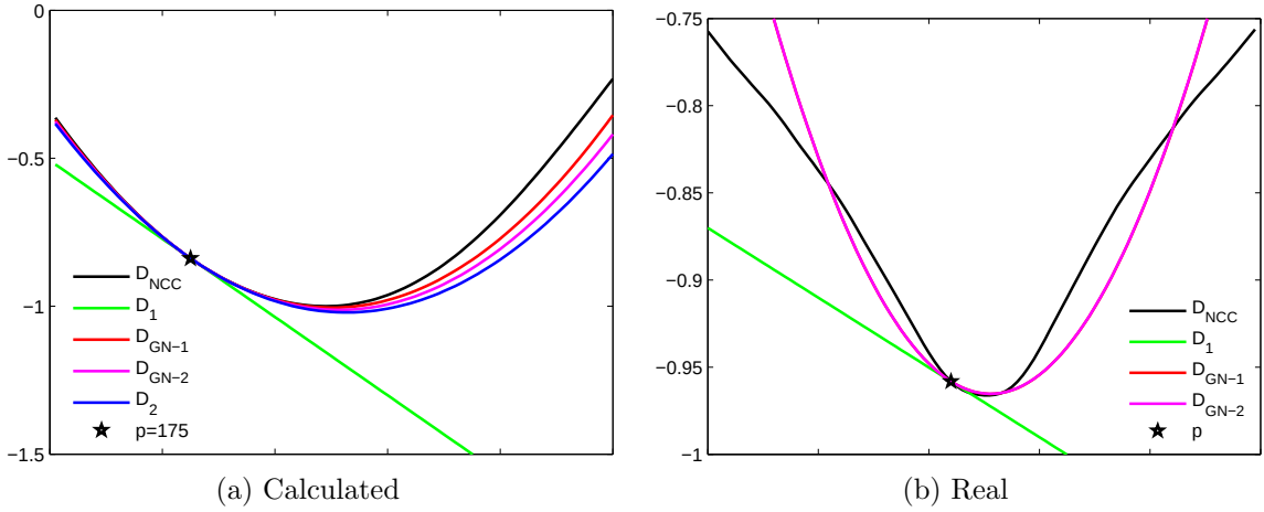
Figure 4.12 The actual function, D_{NCC} , the full second order Taylor series approximation, D_2 , the approximation based on the complete Gauss-Newton Hessian approximation, D_{GN-2} , the approximation based on the simplified Gauss-Newton Hessian approximation, D_{GN-1} , and a linear approximation, D_1 , for Normalized Correlation. The calculated case (left) shows the comparison to a full, exactly computed Taylor series. The real case (right) shows the Gauss-Newton Hessian approximations for a real image.
