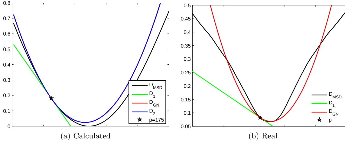
Figure 4.10 The actual function, D_{MSD} , the full Taylor series approximation, D_2 , the Gauss-Newton approximation, D_{GN} , and a linear approximation, D_1 , for Mean Squared Difference. The calculated case (left) shows the comparison to a full, exactly computed Taylor series. The real case (right) shows the estimate of the cost function computed using the Gauss-Newton Hessian approximation for a real image.
