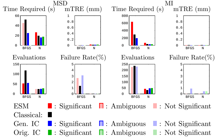
Figure 7.6 Experimental results for synthetic rigid 3D transforms for MSD (left) and MI (right). The optimization algorithms are Broyden-Fletcher-Goldfarb-Shanno (BFGS) and Newton-Raphson (N). For each algorithm, bars are shown for the following methods from left to right: 1: ESM (Red) 2: Classical Forwards Additive (Black) 3: Generalized IC (Blue) and 4: Original IC (Green). Dark bars are statistically significantly different from classical, light bars are not significantly different and out-line bars are ambiguous (see Section 3.2.1). No original IC method was implemented for the BFGS optimizer.
