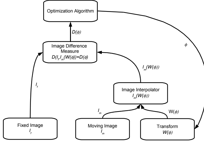
Figure 2.1 A conceptual view of the standard, pair-wise registration approach. Registration consists of optimizing an image difference measure between a fixed image, and a warped (interpolated) moving image. The details of optimization algorithms, image difference measures and interpolators are reasonably independent and may be studied separately. Figure based on [109].
