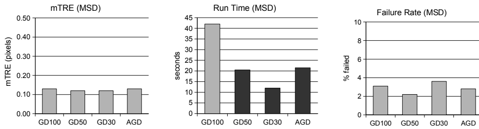
(a) Graphical summary of results for the MSD Measure
