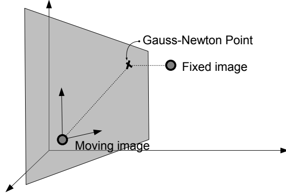
Figure 4.8 The Gauss-Newton step. The derivative of the moving image with respect to the transformation parameters creates a hyperplane in the space of possible images. The Gauss-Newton step is the point on this hyperplane closest in a Euclidean sense to the fixed image.
