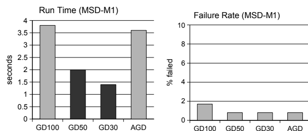
(b) Results for the MSD measure on medical images (M1)
