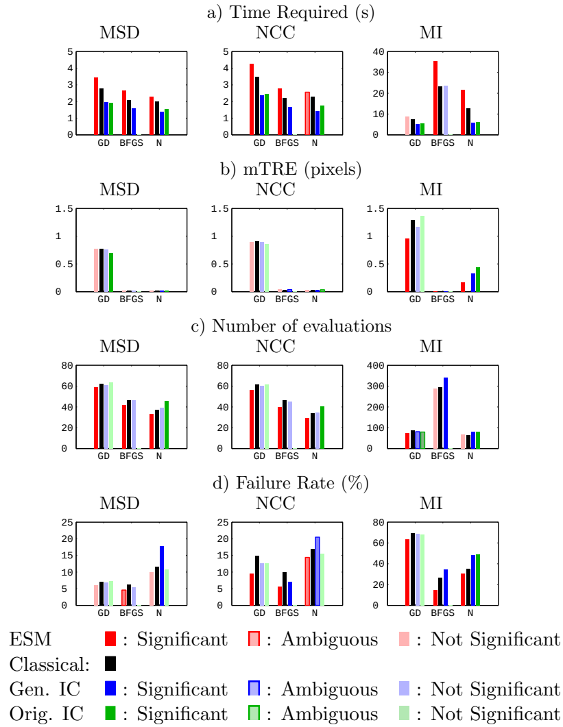
Figure 7.4 Experimental results for synthetic homographies, case 2: Starting far from the correct transform. The optimization algorithms are Gradient Descent (GD), Broyden-Fletcher-Goldfarb-Shanno (BFGS) and Newton-Raphson (N). For each algorithm, bars are shown for the following methods from left to right: 1: ESM (Red) 2: Classical Forwards Additive (Black) 3: Generalized IC (Blue) and 4: Original IC (Green). Dark bars are statistically significantly different from classical, light bars are not significantly different and outline bars are ambiguous (see Section 3.2.1). No original IC method was implemented for the BFGS optimizer.
