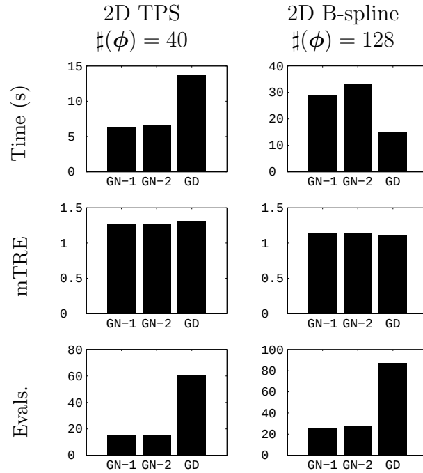
Figure 4.13 Registration performance using a Newton-Raphson optimization technique with both approximate Hessian calculation methods for the NCC measure. Results are also compared against using gradient descent (GD). The two Hessian approximations, \mathcal{H}_{GN-1}D_{NCC} and \mathcal{H}_{GN-2}D_{NCC} , give nearly identical results, so the simpler one \mathcal{H}_{GN-1}D_{NCC} is preferred. (The mTRE is given in mm.)
