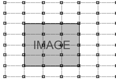
Figure 3.2 Example of a B-spline grid. This example has 4 \times 5 control points over the region of the image, but these must be padded with 3 extra rows and columns outside the region of interest. The transformation shown here is only well defined up to the edge of the image.
