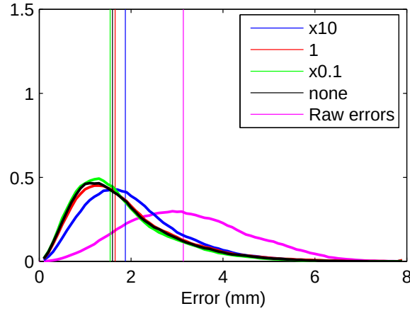
Figure 4.22 Distributions of errors remaining after registration of the Deformable Phantom, Case partially inflated to fully inflated using the 3D B-spline transform with the gradient descent optimizer. The image difference measure used was MSD. This result is selected as being typical of the results of this experiment. The graph shows the distribution of distances between points in a warped mesh of the balloon part of the phantom, and the mesh of the balloon created from the target volume. Vertical lines show the median error. With all scale factors, reasonably successful registration has been achieved, as shown by the distinct leftward shift in the distribution. Case x0.1 produces a slightly, but statistically significantly smaller median error.
