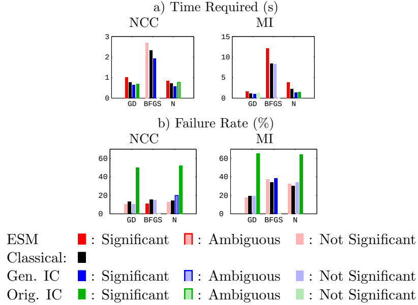
Figure 7.8 Experimental results for registrations of real homographies using NCC (left) and MI (right). The optimization algorithms are Gradient Descent (GD), Broyden-Fletcher-Goldfarb-Shanno (BFGS) and Newton-Raphson (N). For each algorithm, bars are shown for the following methods from left to right: 1: ESM (Red) 2: Classical Forwards Additive (Black) 3: Generalized IC (Blue) and 4: Original IC (Green). Dark bars are statistically significantly different from classical, light bars are not significantly different and outline bars are ambiguous (see Section 3.2.1). No original IC method was implemented for the BFGS optimizer.
