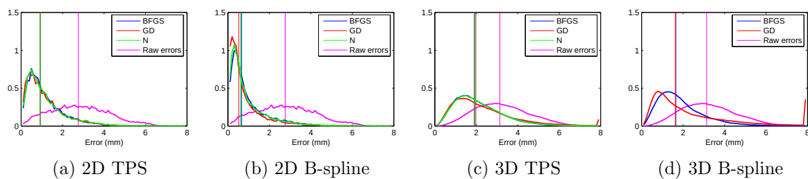
Figure 4.31 Error distributions for results of deformable registration using the MI cost function. The graph shows the distribution of errors over a 50 \times 50 grid ( 50 \times 50 \times 50 in 3D) of points in the image extent. Point errors for all 25 runs have been combined into one histogram for each optimizer. Vertical lines show the median error. All optimizers, achieved a reasonably successful registration, as shown by the distinct leftward shift in the distributions. Datasets used are: 2D TPS and B-spline – Sagittal Brain Slice; 3D TPS and B-spline Deformable Phantom.
