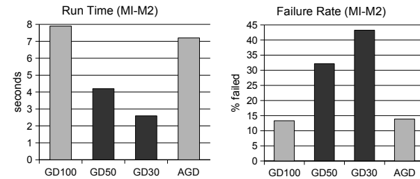
(c) Results for the MI measure on medical images (M2)
