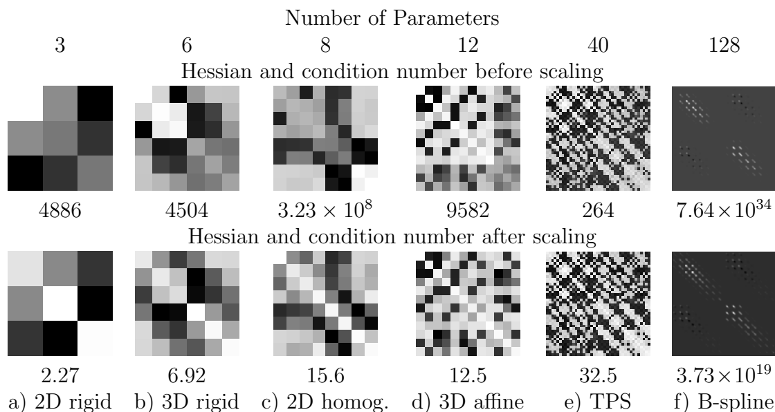
Figure 4.17 These images show the Hessians and their condition numbers for various image transformations both before and after scaling with the matrix, \mathbf{S} . The Hessian values have been logarithmically scaled to fit in the range of image intensities. Note how the condition numbers have been reduced significantly by the parameter scaling. This appears as a stronger, and more even, diagonal components after scaling for the matrix based transforms (a-d). The density of the off-diagonal elements in the TPS transform (e), and the near singularity of the B-spline Hessian (f) reduce the effectiveness of scaling for these cases. The intensities of the pre and post scaling Hessian images are scaled differently and should not be considered comparable.
