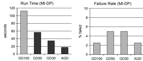
(a) Results for the MI measure on digital photo images (DP)
