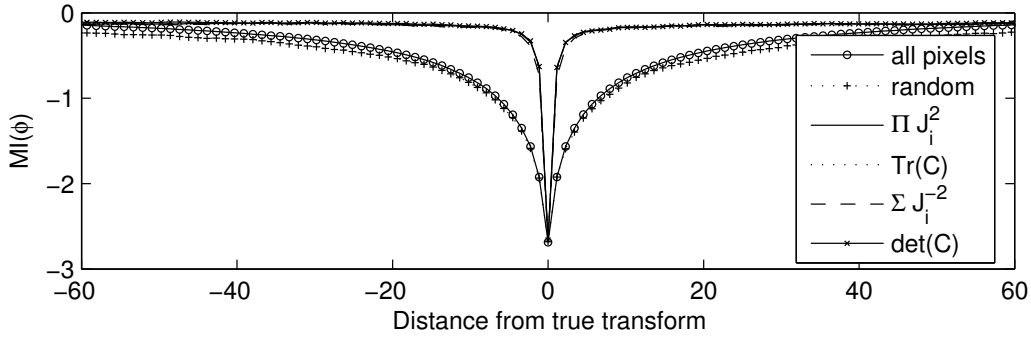
(b) Mutual Information values using different pixel selection criteria (1% of pixels)
