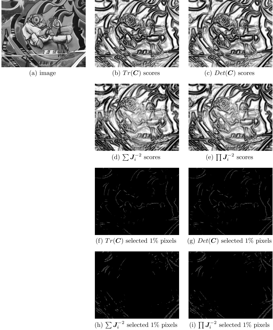
Figure 6.2 Pixel scores and selected pixels for each selection criterion. For images b-e, darker is better. For images f-i, selected 1% of pixels are shown in white.
