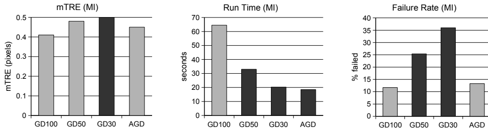
(b) Graphical summary of results for the MI Measure
