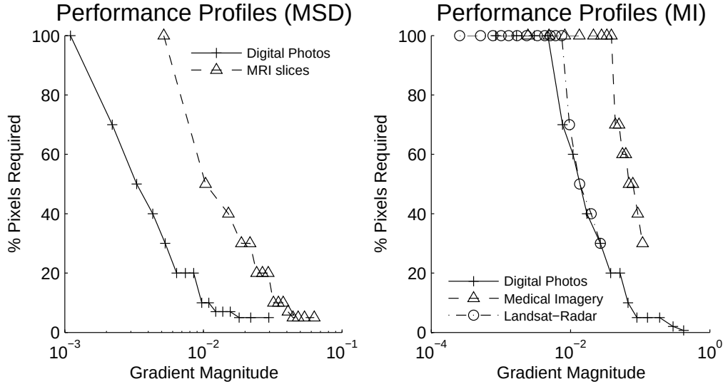
Figure 5.3 Performance profiles: The percentage of computation required to achieve E_p = 90\% . The graph on the left is for the mean squared difference measure (MSD) and the one on the right is for the mutual information measure (MI).
