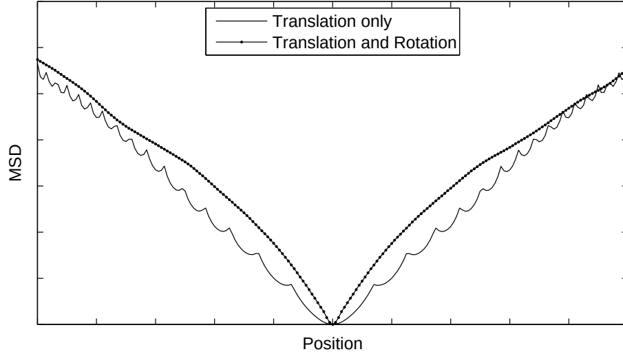
Figure 3.1 Mean squared difference cost function of an image compared to a transformed version of itself using linear interpolation. The plain line shows the case where the moving image is transformed using translation only, while the dotted line shows the case of a transformation involving both angular and translational components. Interpolation artifacts are clearly visible in the translational case, but when there is some angular shift involved these disappear. The translation ranges from \pm 16 pixels in both x and y directions. For the dotted line, the angle also varies over \pm 0.28 radians.
