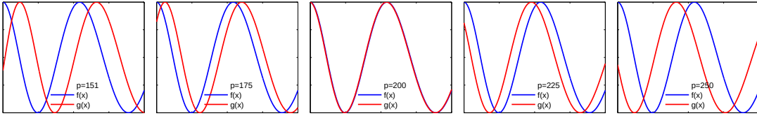
Figure 4.9 The simple functions used for testing the MSD Gauss-Newton approximation. The fixed and moving one-dimensional images are shown for values of the parameter, p , ranging from 151 to 250. Correct registration of the functions occurs at p = 200 .
