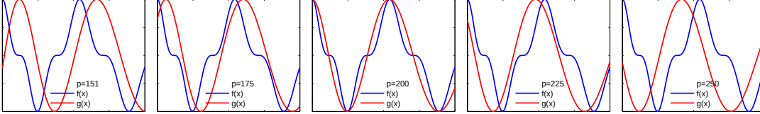
Figure 4.14 The simple functions used for testing the MI Gauss-Newton approximation. The fixed and moving one-dimensional images are shown for values of the parameter, p , ranging from 151 to 250. Correct registration of the functions occurs at p = 200 .
