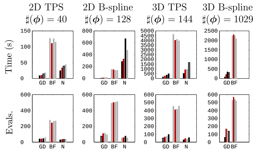
Figure 4.19 Comparison of registration results for different scale factors for transforms with different numbers of parameters using the mutual information cost function. The optimizers are identified as GD –gradient descent, BFGS – Broyden-Fletcher-Goldfarb-Shanno, N – Newton-Raphson. For each optimizer, the bars represent, from left to right, the result using the scale factors x10, x1, x0.1 and NSCL. Case x1, the optimal scale factor, is identified in red. If the results of the other cases differ in a statistically significant way from case x1 they are shown in black. Ambiguous results (see Section 3.2.1) are shown with black outline, and results that are not significantly different from case x1 are shown in gray. The datasets used were: 2D TPS and B-spline – Sagittal Brain Slice; 3D TPS and B-spline Deformable Phantom. Note that the vertical scale is not the same in all cases.
