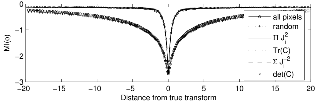
(b) Mutual Information values using different pixel selection criteria (1% of pixels)
