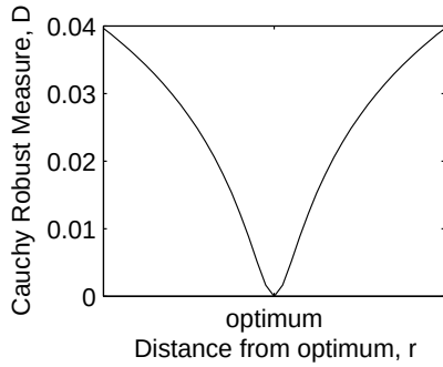
Figure 4.23 The Cauchy robust cost function [179]. The figure on the left illustrates the shape of the Cauchy robust cost function (Equation on right). Note that the shape is quasiconvex, but not convex, like the MI image difference measure. Here i indexes the grid of points, and r_i(\phi) is the distance moved by the transformed point. The parameter, b , was set to 0.1 for this test.
