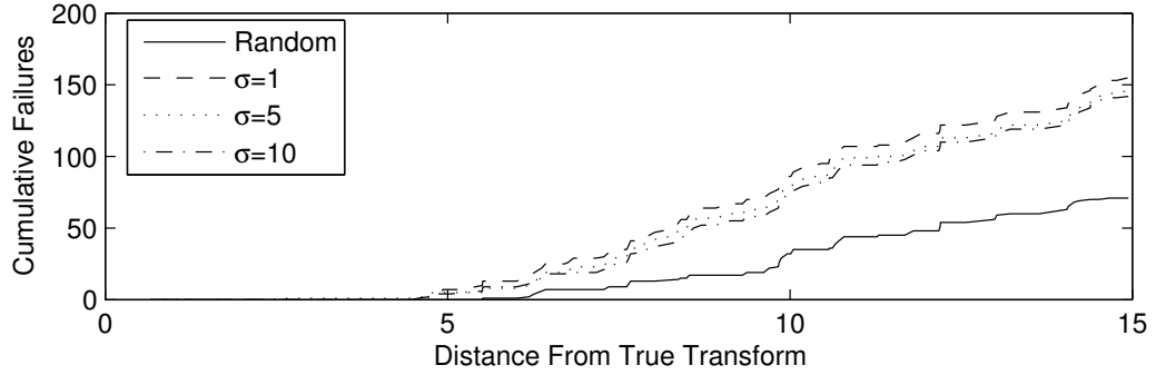
(b) Results for Image Set 2 {6.8d, 6.8e, 6.8f} using gradient descent and Tr(\mathbf{C}) criterion
