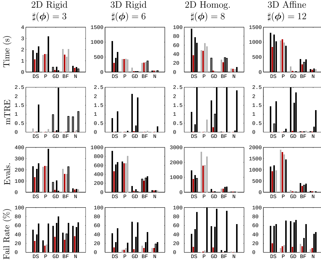
Figure 4.18 Comparison of registration results for transforms with different numbers of parameters using the mutual information cost function. The optimizers are identified as DS – downhill simplex, P – Powell’s, GD – gradient descent, BFGS – Broyden-Fletcher-Goldfarb-Shanno, N – Newton-Raphson. For each optimizer, the bars represent, from left to right, the result using the scale factors x10, x1, x0.1 and NSCL. Case x1, the optimal scale factor, is identified in red. If the results of the other cases differ in a statistically significant way from case x1 they are shown in black. Ambiguous results (see Section 3.2.1) are shown with black outline, and results that are not significantly different from case x1 are shown in gray. The datasets used were: 2D Rigid – Sagittal Brain Slice; 3D Rigid and Affine – Brainweb; 2D Homography – Agra Fort. mTRE is in mm for all cases except the homography, where it is in pixels. Note that the vertical scale is not the same in all cases.
