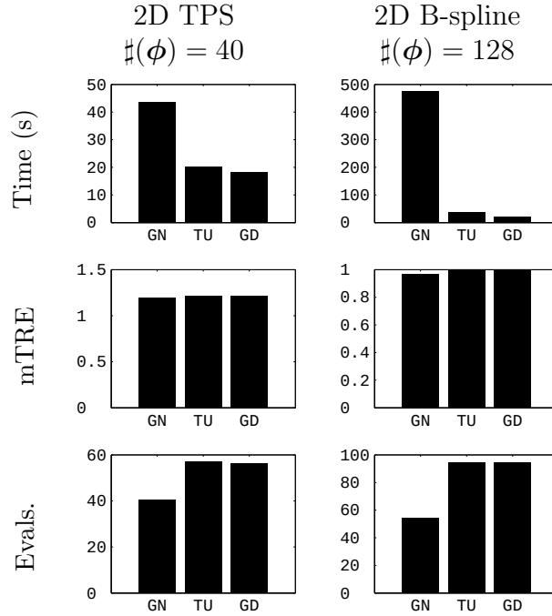
Figure 4.16 Registration performance using a Newton-Raphson optimization technique with both approximate Hessian calculation methods for the MI measure. Results are also compared against using gradient descent. The two Hessian approximations, \mathcal{H}_{GN}D_{MI} and \mathcal{H}_{TU}D_{MI} , give very different results. The shorter truncation of the Taylor series, \mathcal{H}_{TU}D_{MI} , does not result in significantly different performance from gradient descent. The longer, generalized Gauss-Newton approximation \mathcal{H}_{GN}D_{MI} is preferred. (The mTRE is given in mm.)
