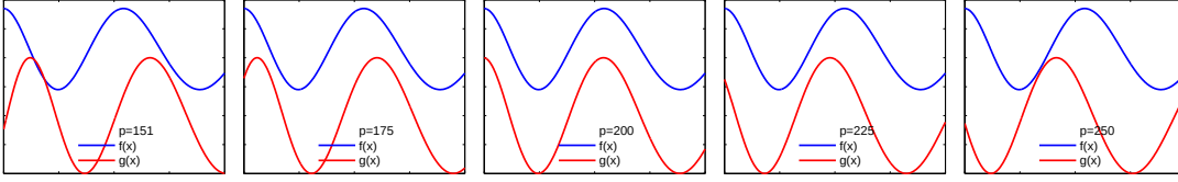
Figure 4.11 The simple functions used for testing the NCC Gauss-Newton approximation. The fixed and moving one-dimensional images are shown for values of the parameter, p , ranging from 151 to 250. Correct registration of the functions occurs at p = 200 .
