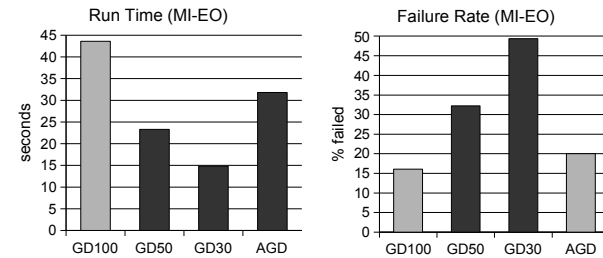
(b) Results for the MI measure on earth observation images (EO)
