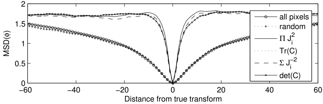
(a) Mean Squared Difference values using different pixel selection criteria (1% of pixels)
