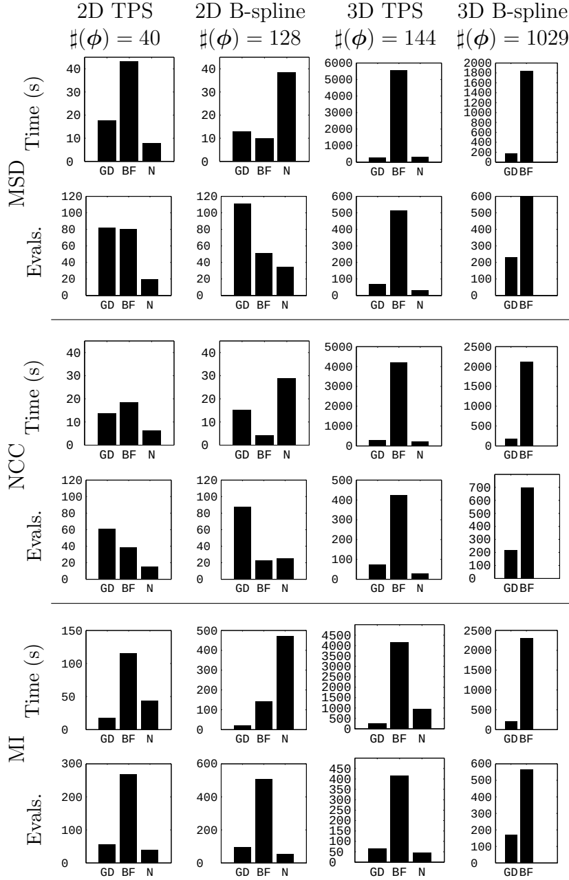
Figure 4.30 Comparison of time and number of evaluations for deformable transforms with different numbers of parameters showing all cost functions on matrix based transforms. Optimizers shown are the Newton-Raphson (N), Broyden-Fletcher-Goldfarb-Shanno (BFGS) and gradient descent (GD). Note that the vertical scale is not the same in all cases. Datasets used were: 2D TPS and B-spline – Sagittal Brain Slice; 3D TPS and B-spline Deformable Phantom.
