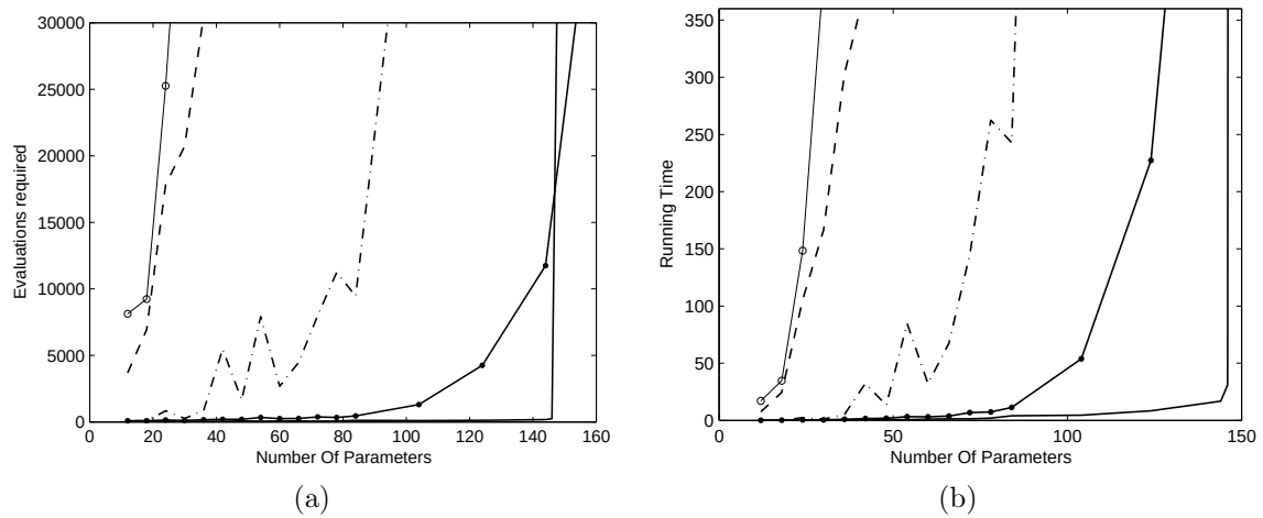
Figure 4.24 Number of evaluations and time required for optimizing a simple cost function as the number of parameters changes. a) Number of evaluations required for convergence for various numbers of parameters, similar starting positions. b) Time required for convergence.
