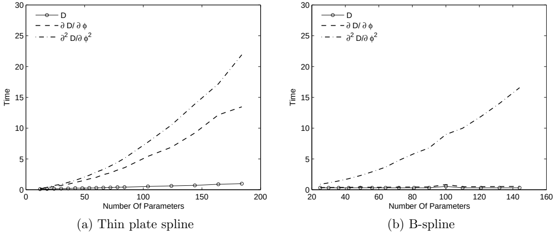
Figure 4.26 Time required to compute D , \nabla D and \mathcal{H}D on a 240 \times 256 image. a) Thin plate spline b) B-spline. Note the difference in complexity of computing the gradient.
