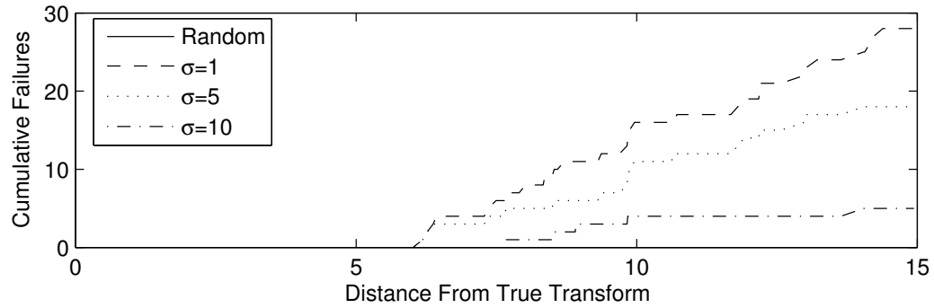
(a) Registering Graffiti b) to a) using gradient descent and the Tr(\mathbf{C}) criterion
