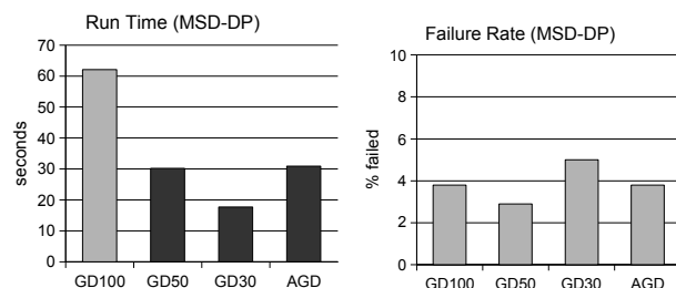
(a) Results for the MSD measure on digital photo images (DP)
