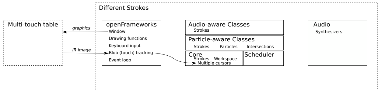
Figure 4.13 System diagram illustrating the new features added to Different Strokes to support multi-touch interaction.
