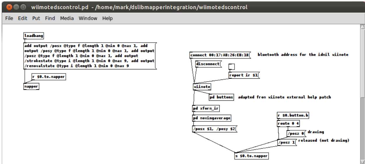
Figure 6.5 The main part of the Pure Data patch, showing the mapper and wiimote objects. The wiimote IR data and button presses are propagated to DS through libmapper . The declaration of the libmapper output signals can be seen in the input to the mapper object, on the left.
