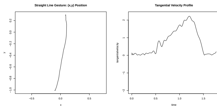
Figure 5.12 A gesture trace in (x, y) screen space, and its associated tangential velocity profile (participant c13fbc, straight line task, static friction condition).
