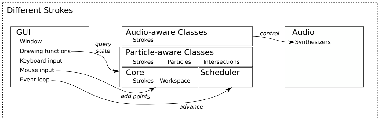
Figure 4.5 The main components of the DS code are the graphics subsystem (GUI), the simulation subsystem, and the audio subsystem. Arrows indicate the interactions between the components. The simulation is made up of layers of classes that each add extra functionality to the one below.
