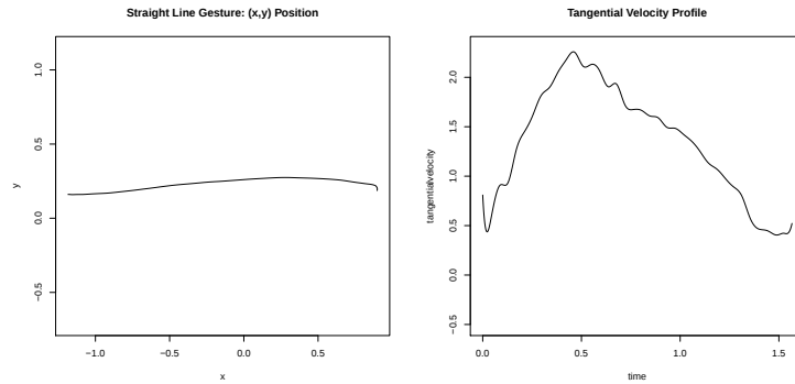
Figure 5.13 A gesture trace in (x, y) screen space, and its associated tangential velocity profile (participant 8b5d2e, straight line task, cursor inertia condition).
