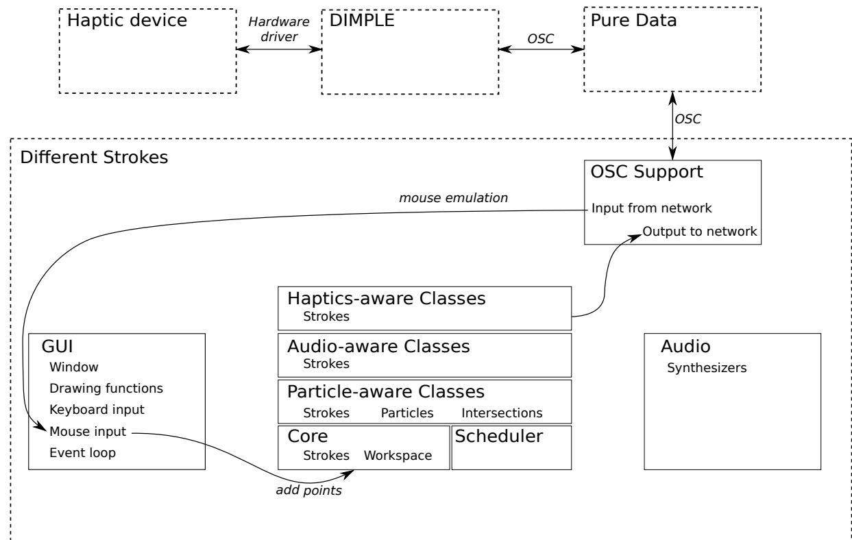
Figure 5.2 A system diagram for DIMPLE integration into Different Strokes to support haptic input devices.
