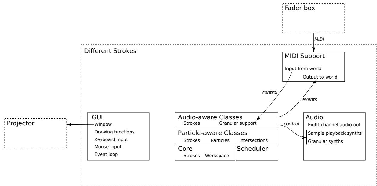
Figure 4.11 System diagram illustrating the new features added to Different Strokes for the d_verse project.
