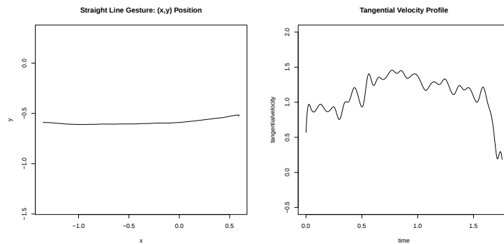
Figure 5.14 A gesture trace in (x, y) screen space, and its associated tangential velocity profile (participant c13fbc, straight line task, modulated cursor inertia condition).
