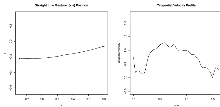
Figure 5.11 A gesture trace in (x, y) screen space, and its associated tangential velocity profile (participant 2d891a, straight line task, dynamic friction condition).
