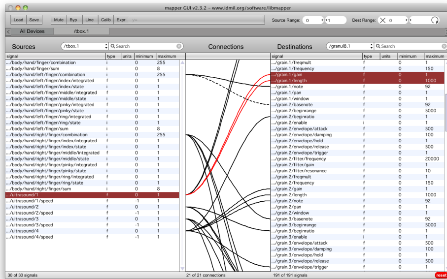
Figure 6.1 A screenshot of a libmapper GUI, showing the input and output signals for two devices. Output signals for a tbox are listed along the left, and input signals for a granul8 software synthesizer instance are listed along the right. Connections between the signals are represented as curved lines from left to right. The properties of a given connection appear at the top of the screen when it is selected.
