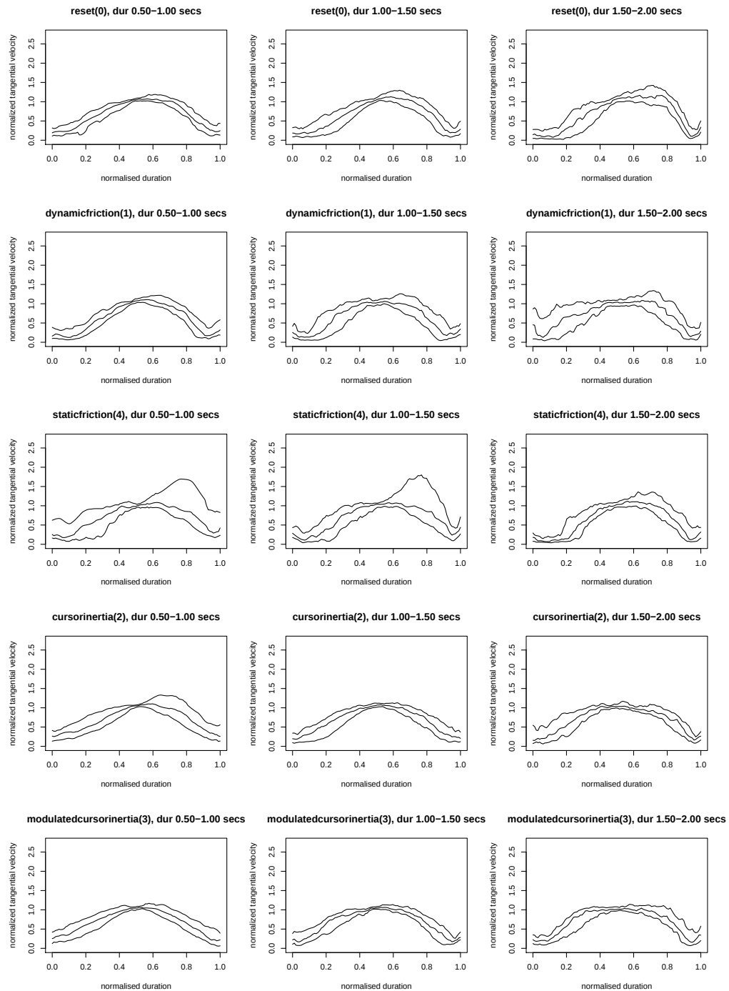
Figure 5.16 Velocity distributions for all five haptic conditions, over the duration intervals 0.5–1.0 seconds, 1.0–1.5 seconds, and 1.5–2.0 seconds. Each plot shows the first quartile, median, and third quartile for the distribution of velocities at a given point in time over the population of strokes. The stroke duration and velocity are normalized.
