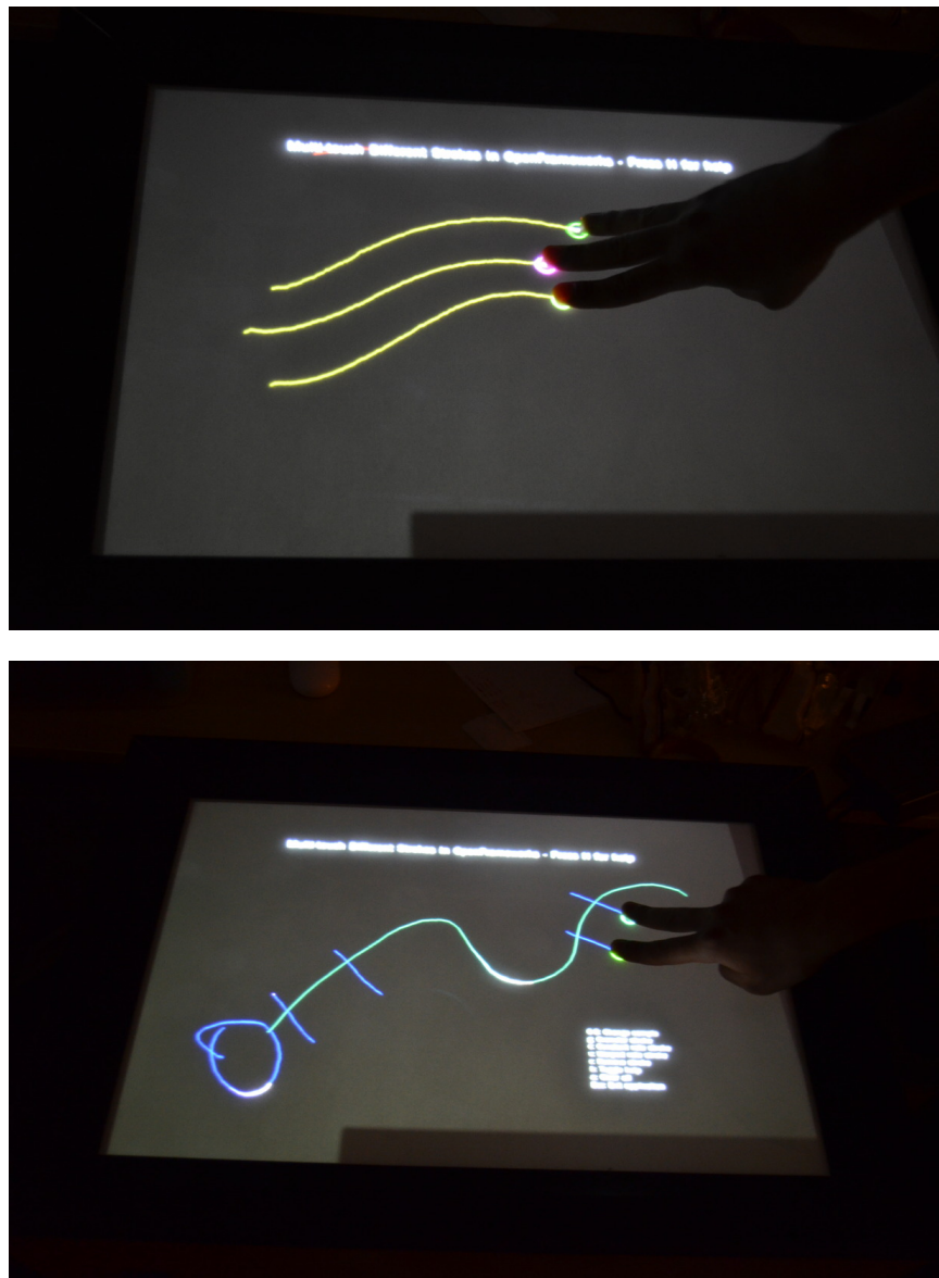
Figure 4.15 Photos of Different Strokes running on the TactoSonix multi-touch table.
