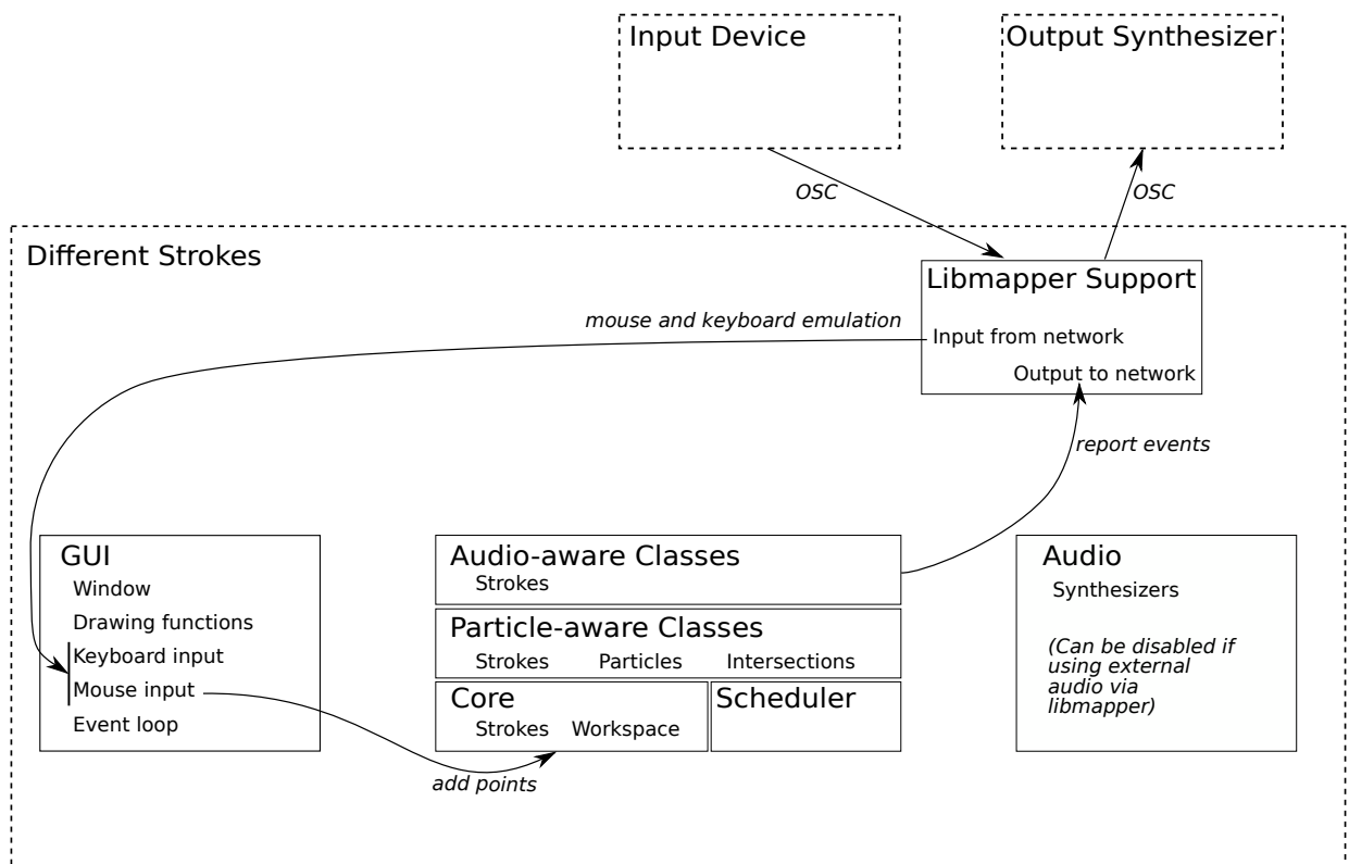
Figure 6.2 A system diagram for libmapper integration into Different Strokes .
