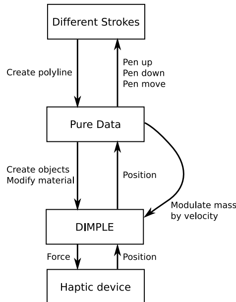
Figure 5.4 Information flow between the DS and DIMPLE applications.
