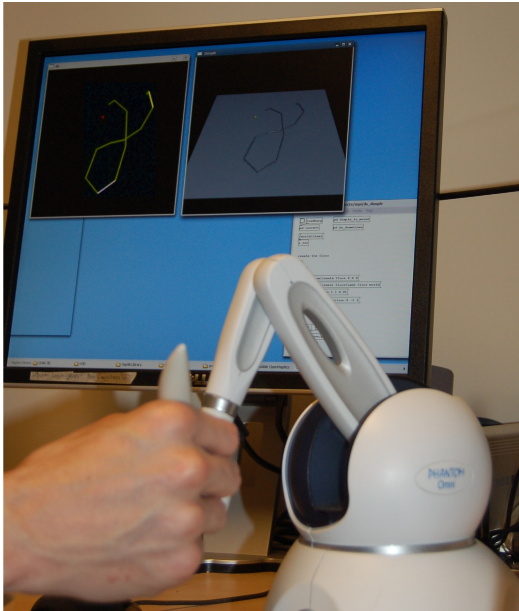
Figure 5.1 The prototype's physical setup (Zadel et al., 2009). The user holds a Sensable Phantom Omni device and manipulates it, feeling the forces controlled by the software. The image on the screen shows the three software applications used in the implementation: Different Strokes (at the left), DIMPLe (in the middle), and Pure Data (lower right). Note the flat square polygon in the DIMPLe window: this acts as a writing surface that the user can feel through the haptic device.
