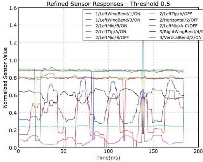
Fig. 3.5 Ballagumi Significant Signal Responses - Moving the Apex
