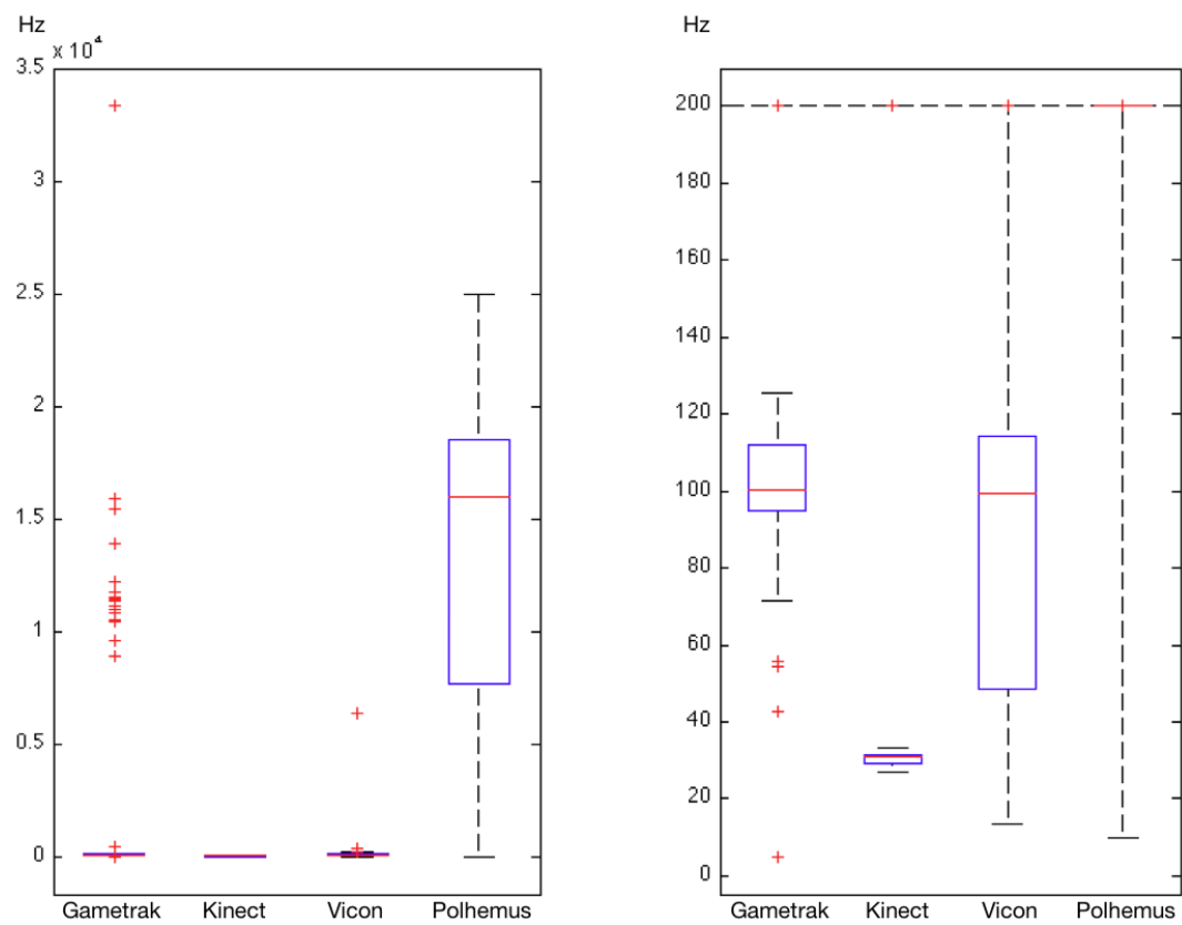
Fig. 4.16 Update rate for the four position trackers
