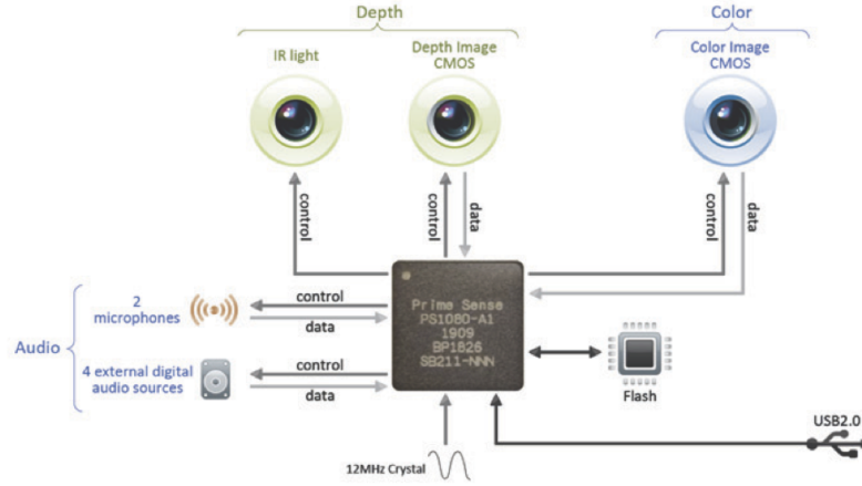
Fig. 4.1 PrimeSensor™ block diagram (Primesense 2011)
