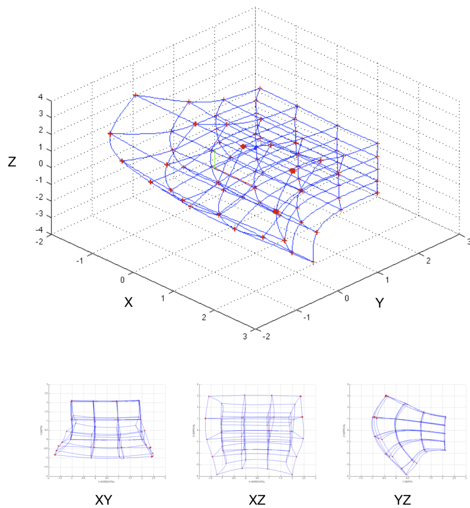
Fig. 4.11 Polhemus 240/8 reported space
