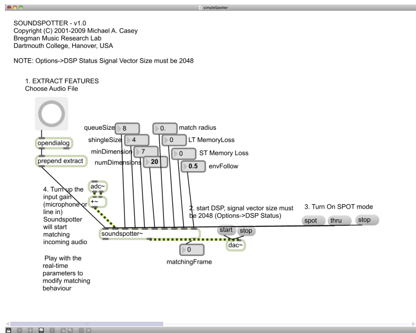
Fig. 3.2 SoundSpotter GUI
