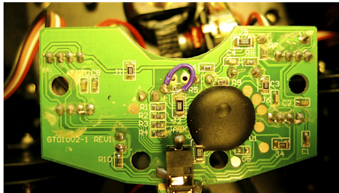
Fig. 4.8 Gametrak modification
