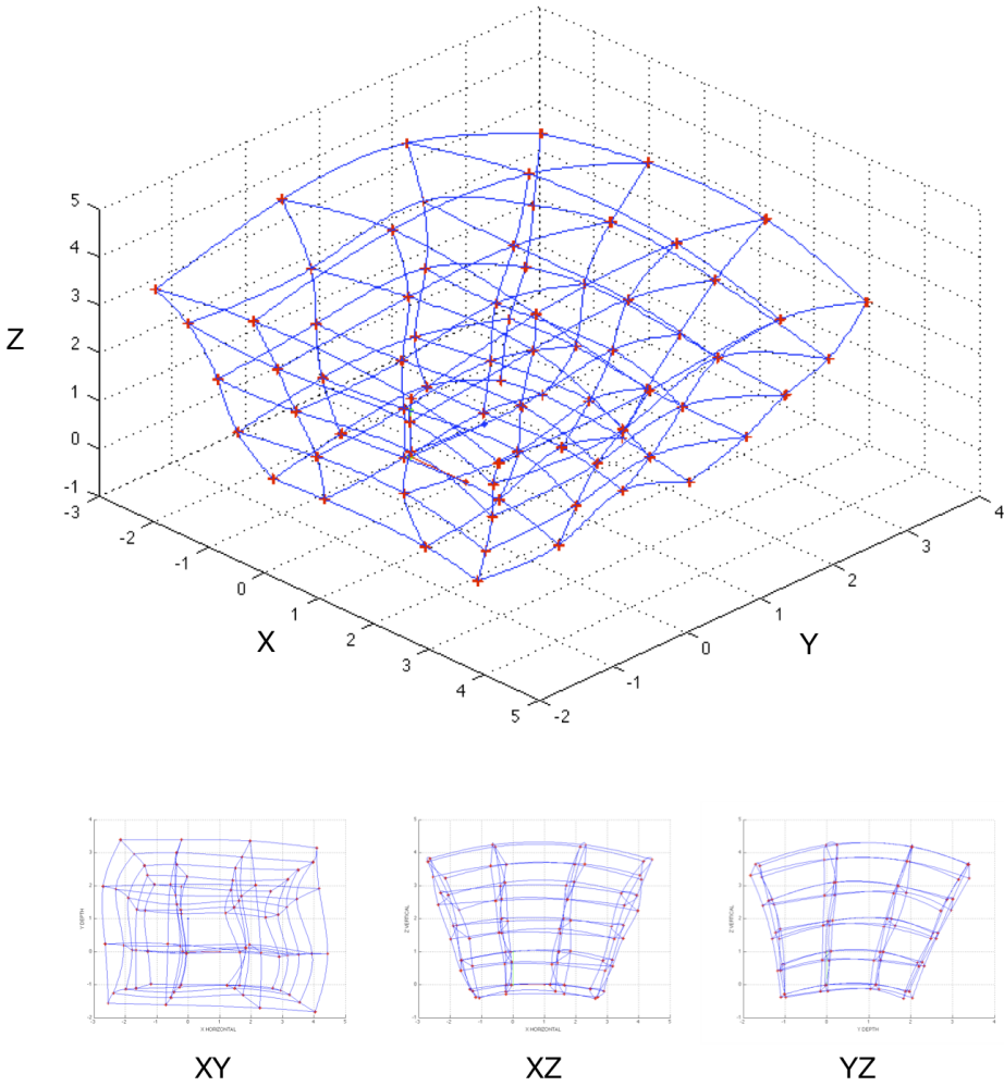
Fig. 4.12 In2Games Gametrak reported space
