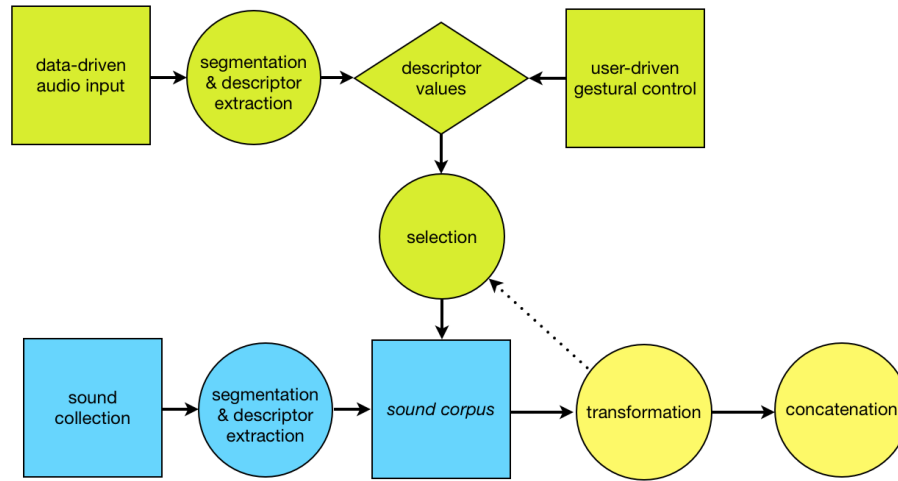
Fig. 3.1 CBCS schematic diagram, adapted from (Schwarz et al. 2006)
