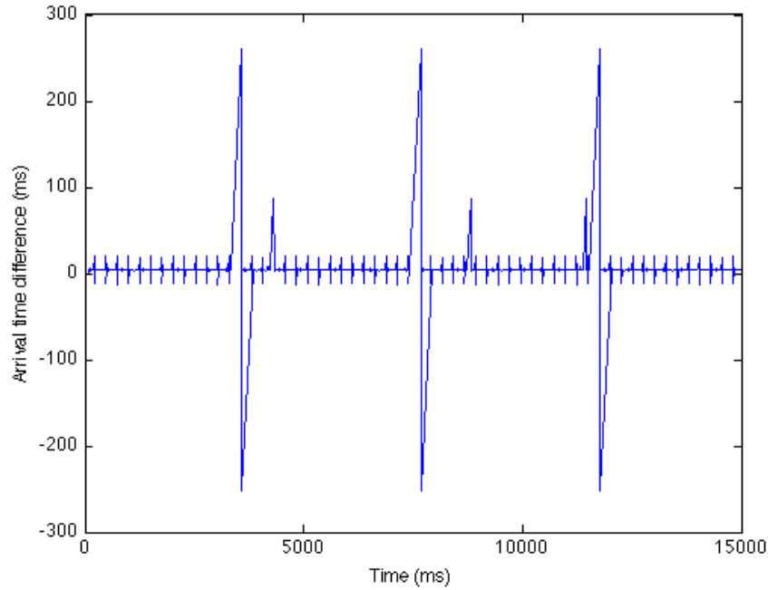
Fig. 4.17 Arrival time difference of the Polhemus data
