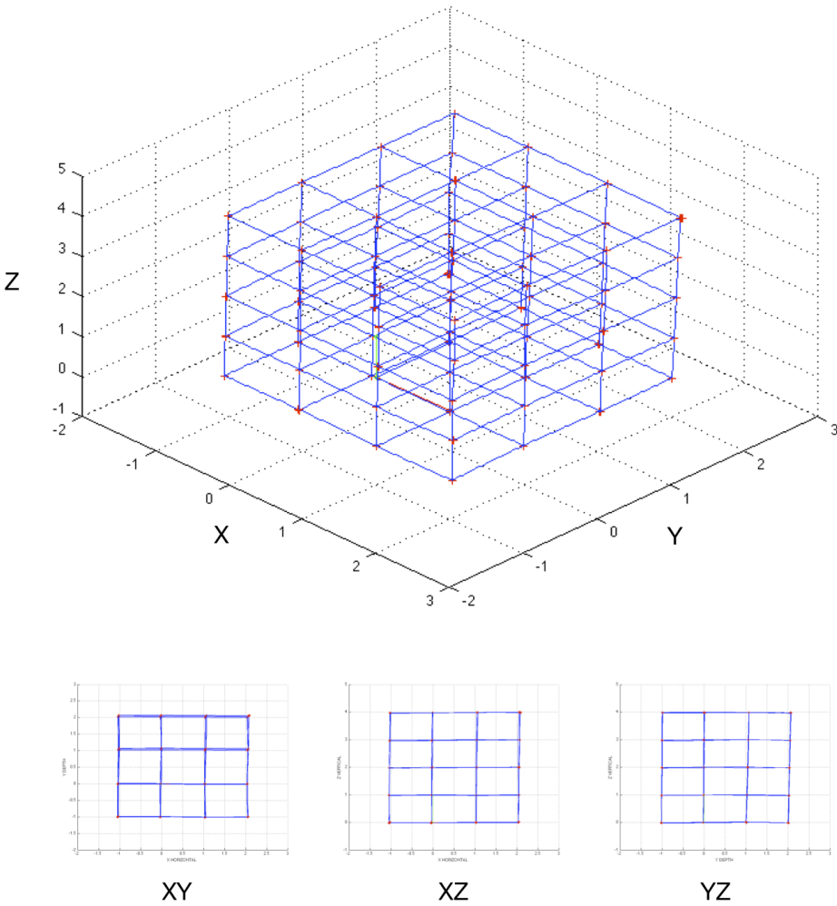
Fig. 4.9 Vicon 460 reported space
