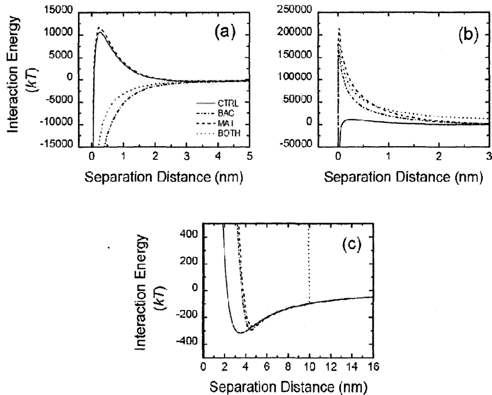
Figure 4.6: representative calculated interaction energy plotted as a function of separation distance for E. coli approaching a flat PVC surface using (a) the xDLVO model; (b) the Steric model; and (c) the Steric model replotted on a different scale to highlight the presence of the secondary energy well. Measured zeta potentials (Table 4.1), calculated surface tension components (Table 4.1) and calculated Hamaker constants (Table 4.2) were used to determine interaction energies.
