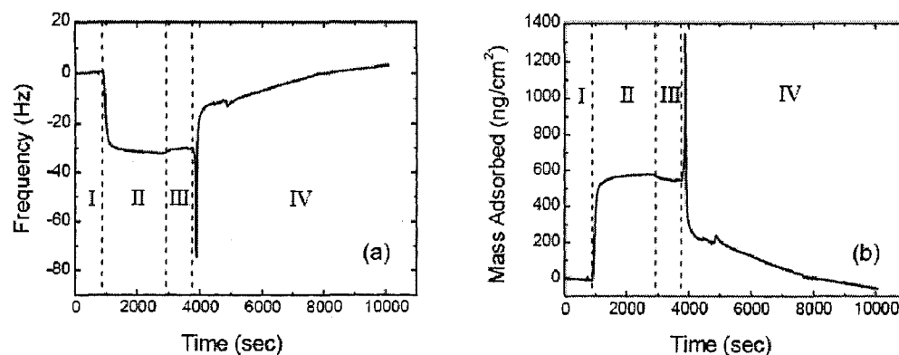
Figure 4.2: QCM data of PAC adsorption on PVC. Mass deposition (B) as calculated using Sauerbrey's equation for rigid films, from QCM frequency response (A) during PAC adsorption to PVC coated crystals. (I) Baseline was achieved in PBS. (II) PAC supplemented PBS was flowed through the system (100 \mu g/mL), (III) PBS is injected; (IV) 0.1% Hellmanex is injected.
