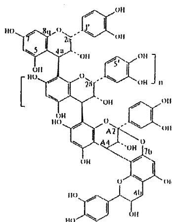
Figure 2.4: Chemical structure of PAC. The compound consists of epicatechin subunits linked through A and B type linkages. Adapted from Foo et al.[6].
