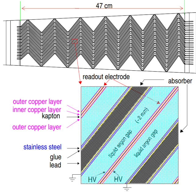
Figure 3.7 – Schematic of the EMCAL showing accordion-like geometry [105].
