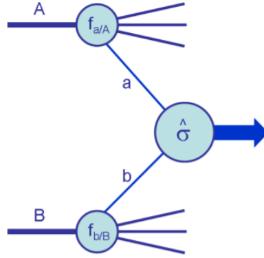
Figure 2.5 – An illustration of two partons from hadrons interacting in a collision [74].
