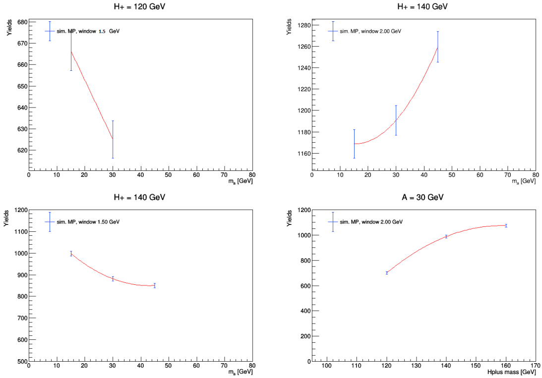
Figure 6.4 – Signal Interpolation: Plots showing the interpolation of yields between simulated mass points using cubic splines for H^+ = 140, 120 GeV masses assuming BR(H \rightarrow AW) = 1 and BR(A \rightarrow \mu\mu) = 3 \times 10^{-4} . These figures show that the splines are well-behaved and the simulated mass points provide the appropriate knots to create a smooth interpolation.
