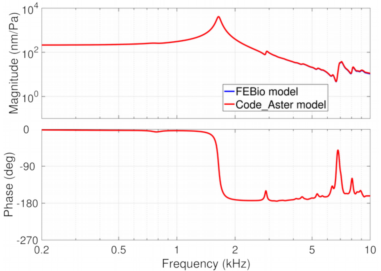
Fig. 5–2: Comparison of frequency responses of umbo in FEBio and Code_Aster. The red lines almost completely obscure the blue lines.
