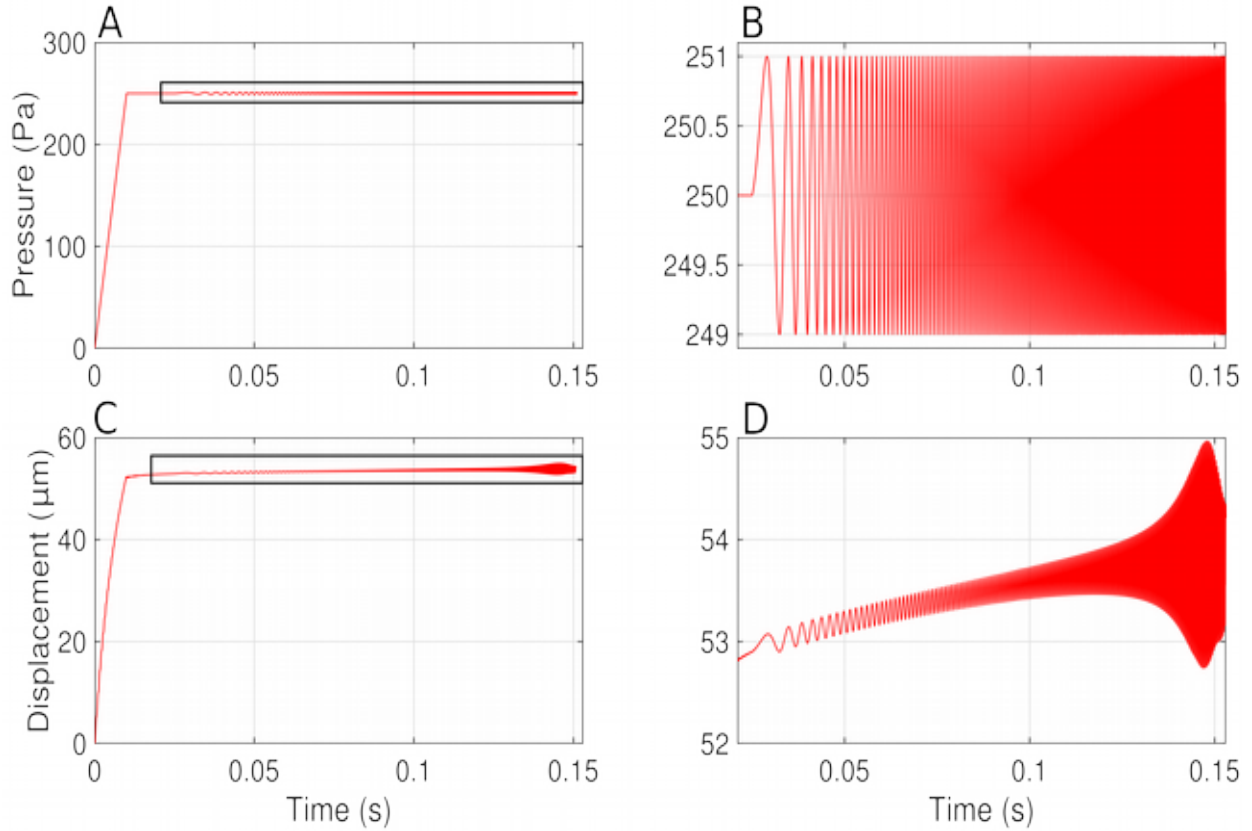
Fig. 5–22: Results for a quasi-static pressure combined with a chirp (0.12 to 3 kHz) using FEBio. A: Input pressure signal. B: Magnified view corresponding to the rectangle in A to show the acoustic stimulus. C: Umbo displacement as a function of time. D: Magnified view corresponding to the rectangle in C.
