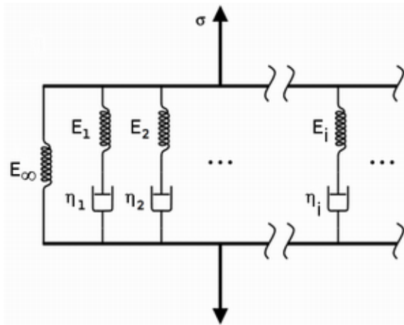
Fig. 3–4: Schematic of the Generalized Maxwell Model (Source: https://en.wikipedia.org/wiki/Generalized_Maxwell_model as of 2017 June 29)
