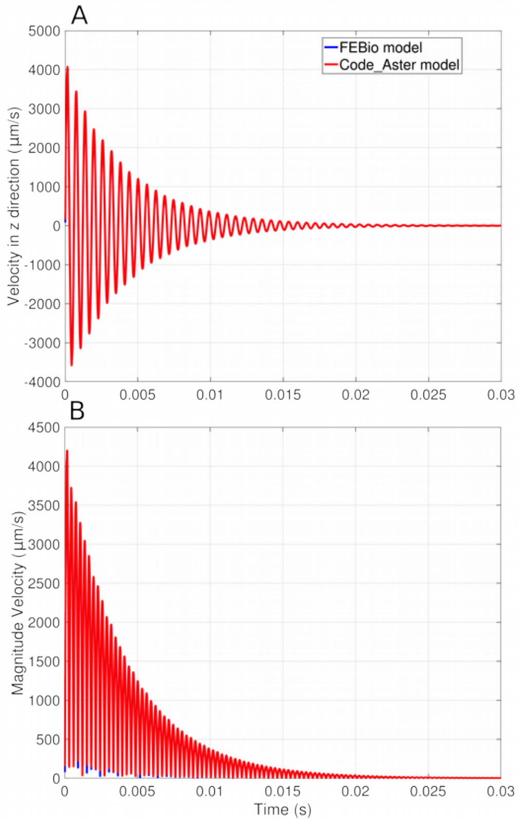
Fig. 5–1: Comparison of umbo velocity in FEBio and Code_Aster. A: Comparison of velocity in z direction . B: Comparison of magnitude velocity. The red lines almost completely obscure the blue lines.
