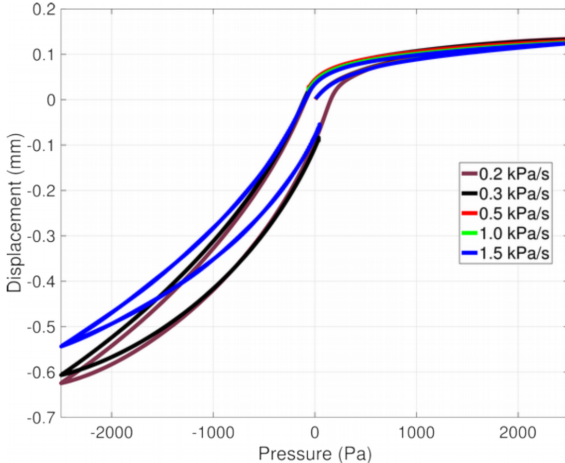
Fig. 5–14: Model umbo displacement as function of pressure at different ultra-low frequencies when the coefficient of the time constant 2.3 s is increased from 0.07 to 0.6.
