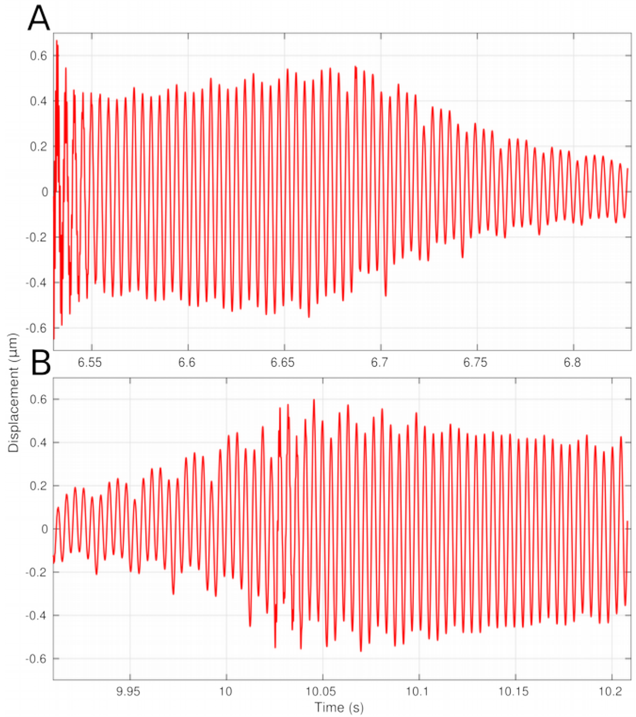
Fig. 5–17: Model umbo vibration after removing the displacement induced by quasi-static pressure sweep. A: Umbo vibration in the ascending branch. B: Umbo vibration in the descending branch.
