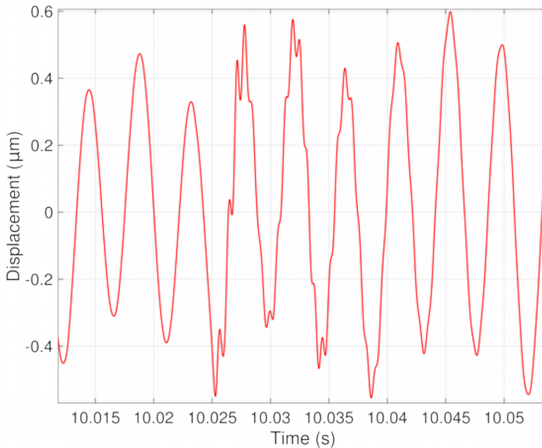
Fig. 5–18: Magnified view of model umbo vibration in the descending branch (Fig. 5–17B).
