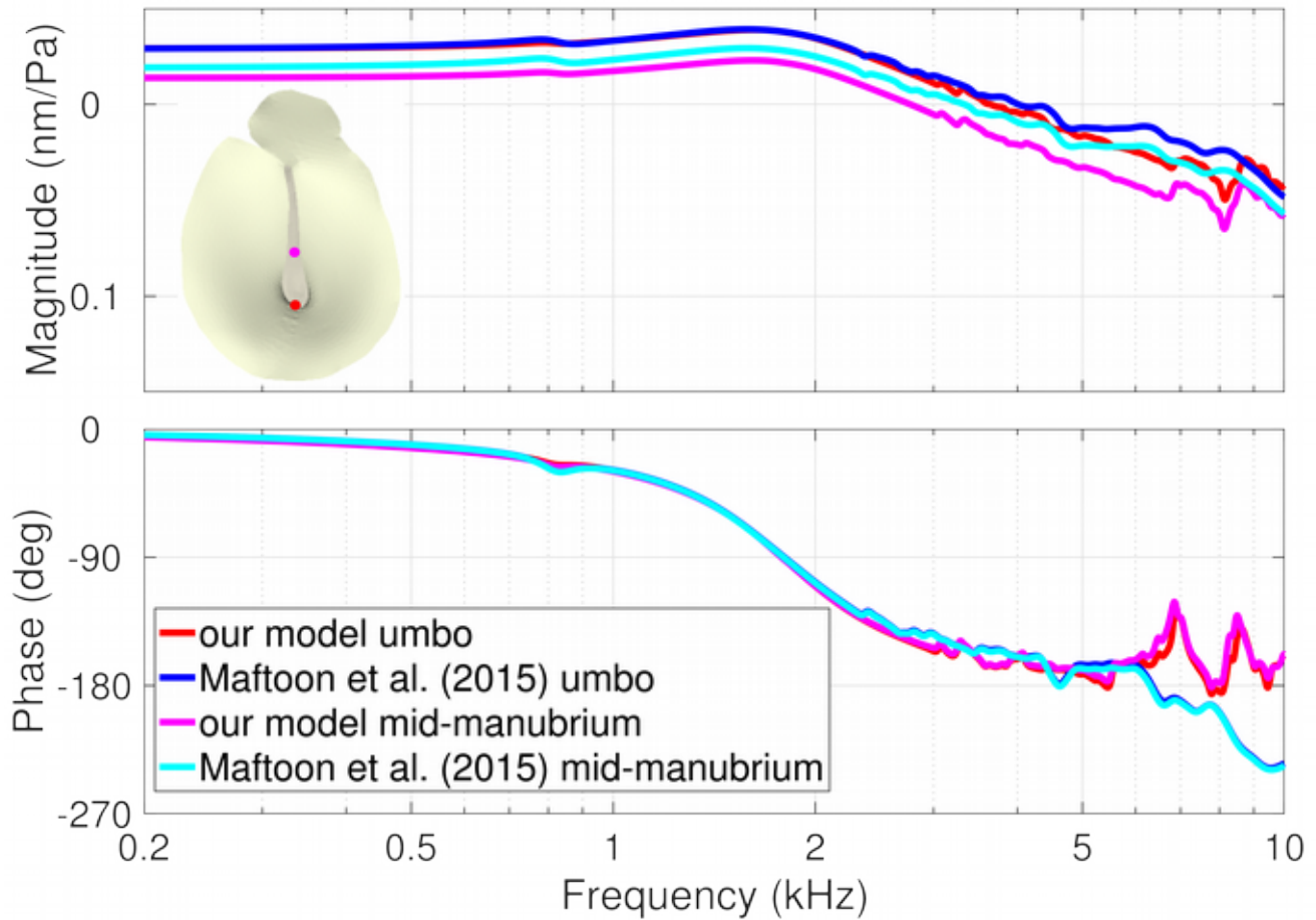
Fig. 5–9: Comparison of our gerbil model response with Maftoon’s model at umbo and at mid-manubrium.
