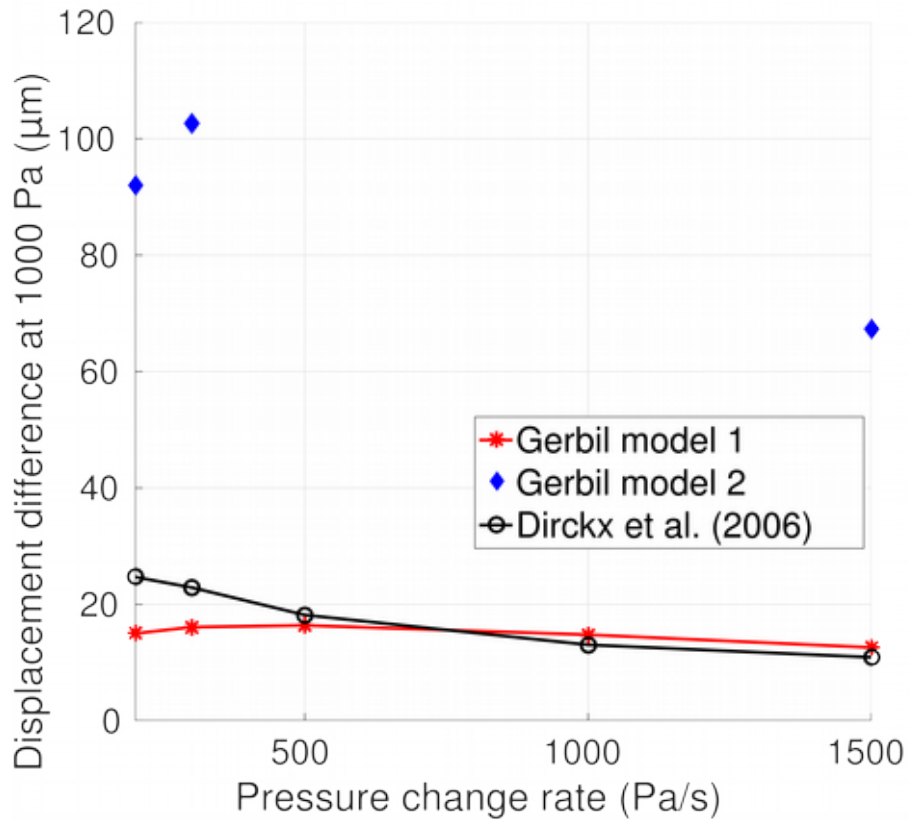
Fig. 5–15: Umbo hysteresis as a function of pressure-change rate, measured in the two gerbil models and in the experiment by Dirckx et al. (2006).
