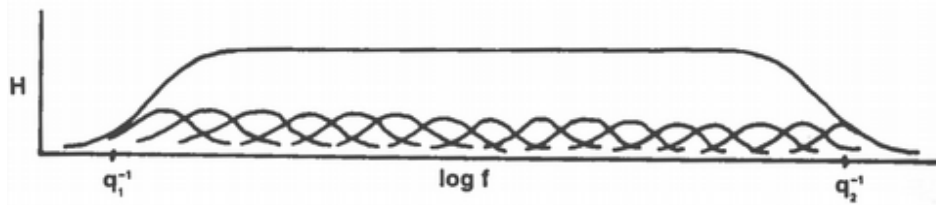
Fig. 4-4: Typical hysteresis-log frequency relationship for living soft tissues. The small bell-shaped curves correspond to the contributions of one Prony series term ( g_i, \tau_i ). The sum is almost flat over a wide range of frequencies. (Source: Fung, 2013, p. 288)
