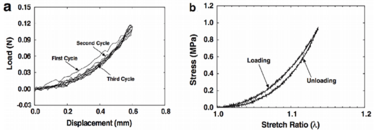
Fig. 3–5: Experimental measurements on TM specimens. a: Load-displacement curves for three cycles obtained from uniaxial tensile tests for one TM specimen. b: Curves of stress vs. stretch ratio for the same TM specimen after steady state (Source: Cheng et al., 2007)
