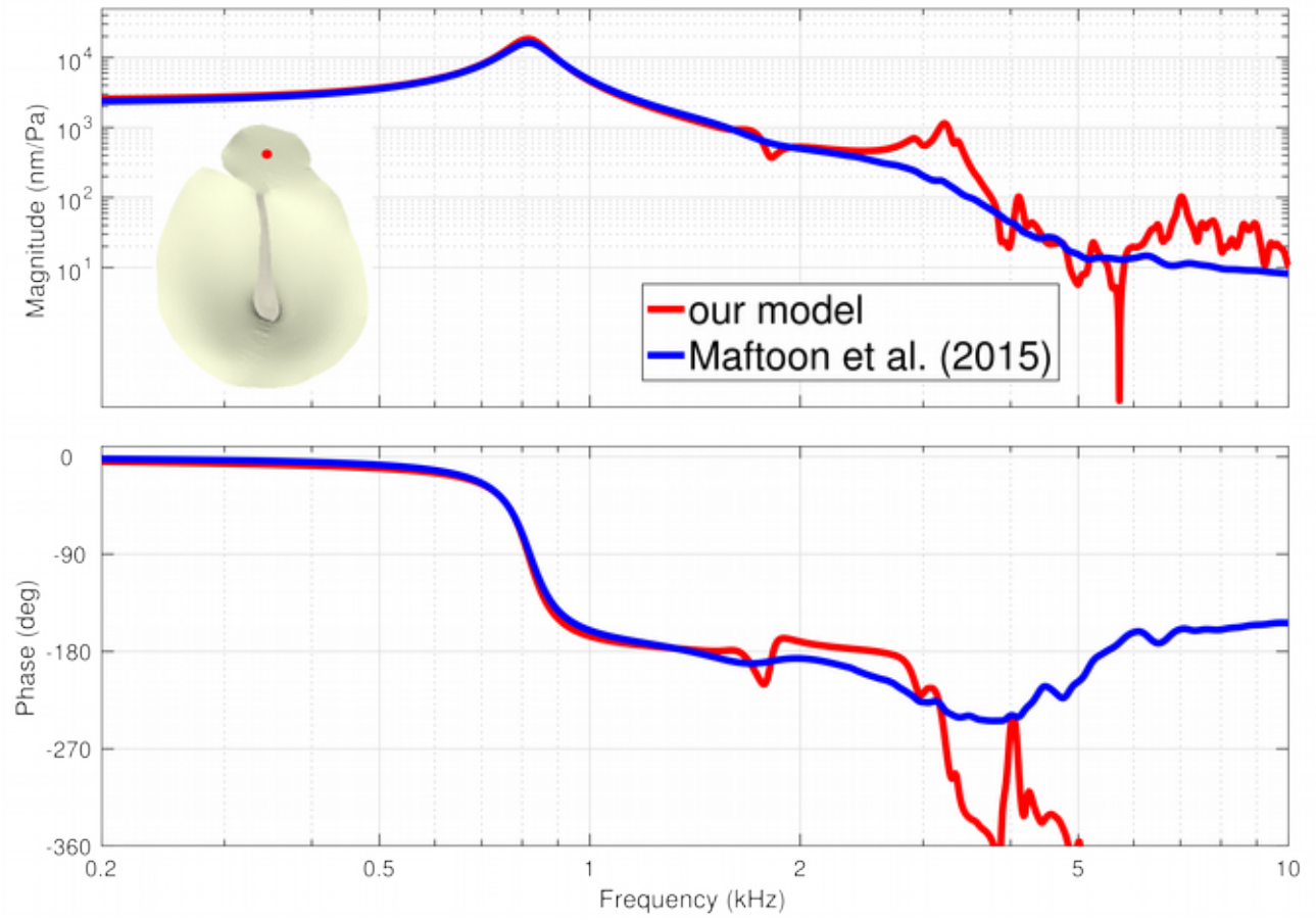
Fig. 5–4: Comparison of our gerbil PF model response with Maftoon’s model response.
