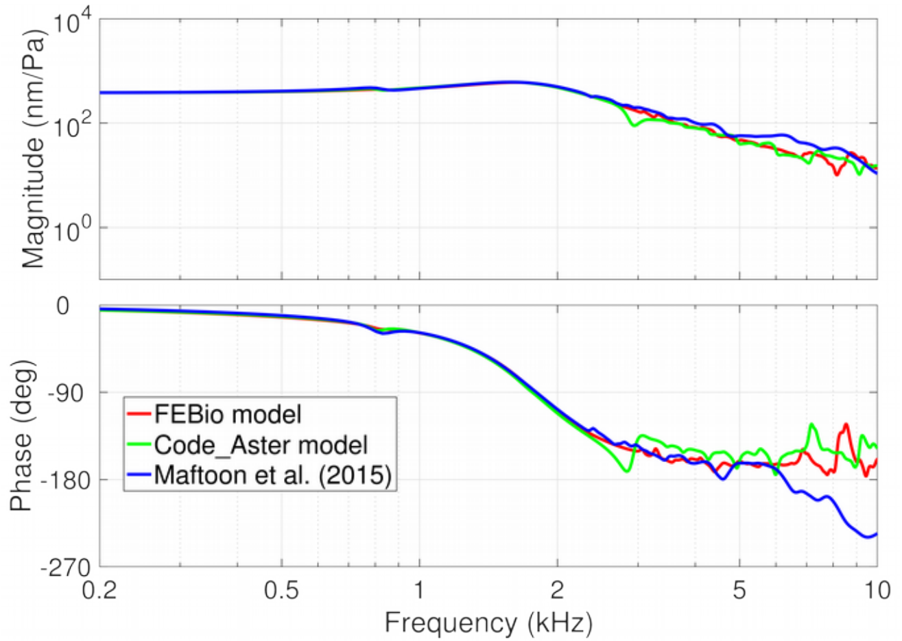
Fig. 5–7: Comparison of the umbo response of FEBio and Code_Aster models with the umbo response of Maftoon’s model.
