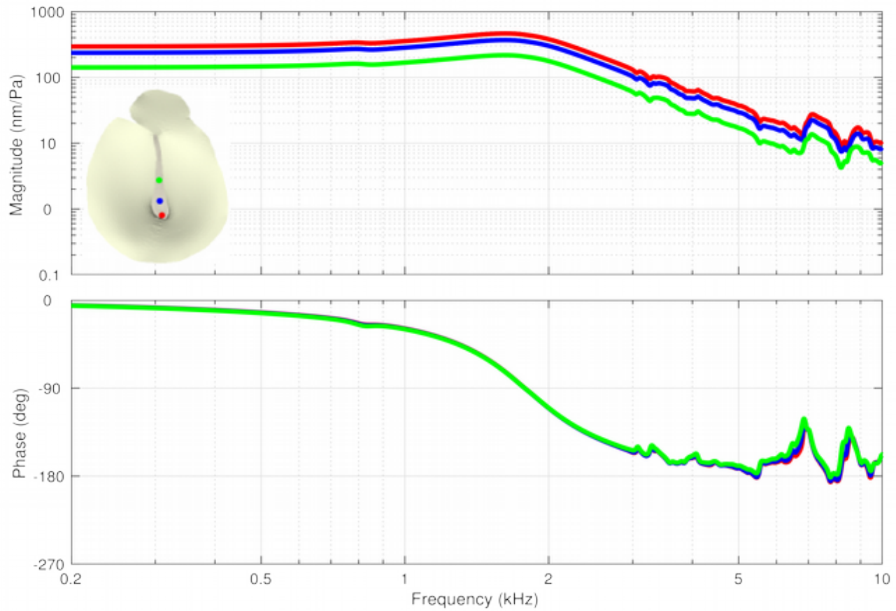
Fig. 5–8: Model responses at three locations along the manubrium. The colours of the curves correspond to the colours of the dots in the inset.
