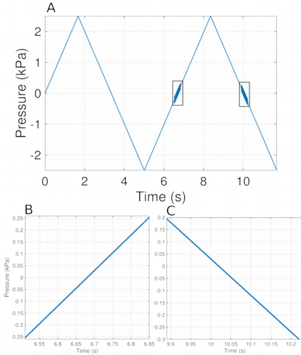
Fig. 4–6: Illustration of the loading condition for quasi-static pressure-change rate at 1.5 kPa/s with a superimposed pure tone of 226 Hz. A: Pressure as a function of time with magnification of the acoustic stimulus (a factor of 100 was applied on the acoustic stimulus for better visualization). B: A closer view of the left-hand rectangle in A. C: A closer view of the right-hand rectangle in A.
