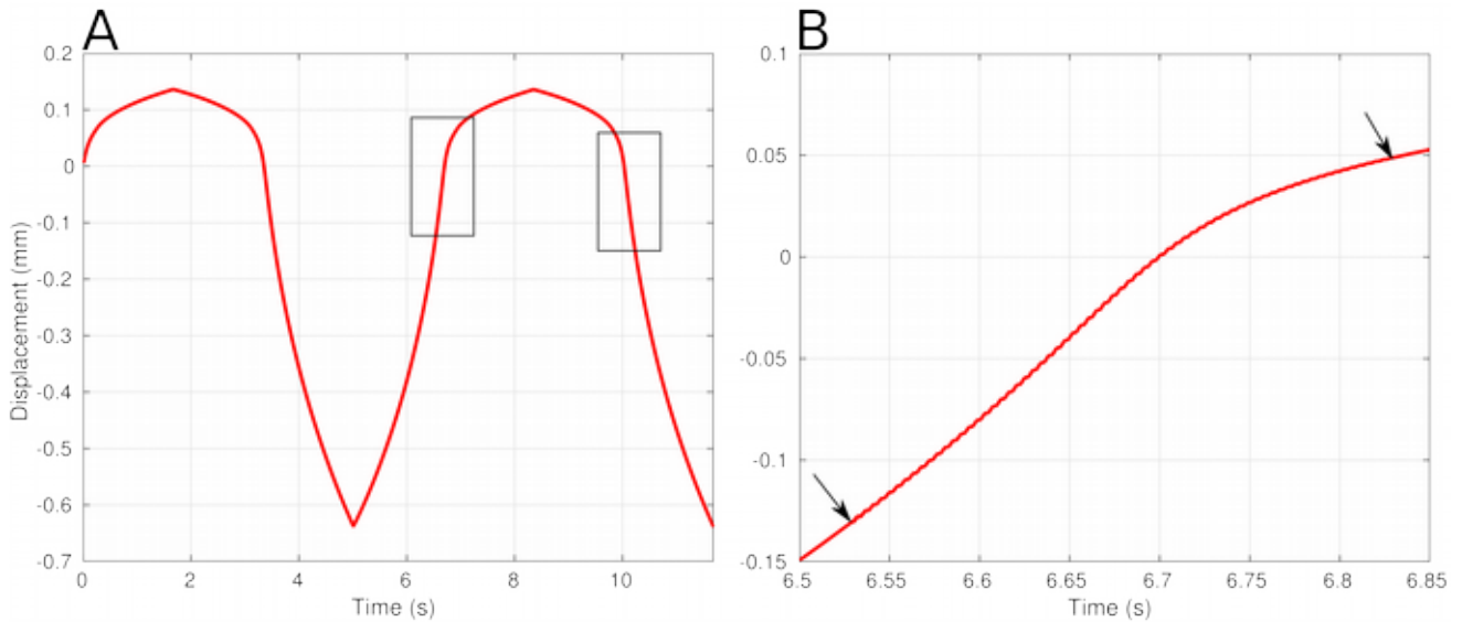
Fig. 5–16: Response of the model to a 226-Hz pure tone during large sweeps of quasi-static pressure. A: Model umbo displacement as function of time. Rectangles indicate areas where the acoustic stimulus was applied. B: Magnified view of the left square in A to highlight the acoustic induced displacements during the ascending branch. Arrows indicate the start and end of the vibrations.
