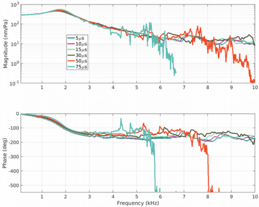
Fig. 4–5: Effect of size of time step on simulated umbo frequency response.
