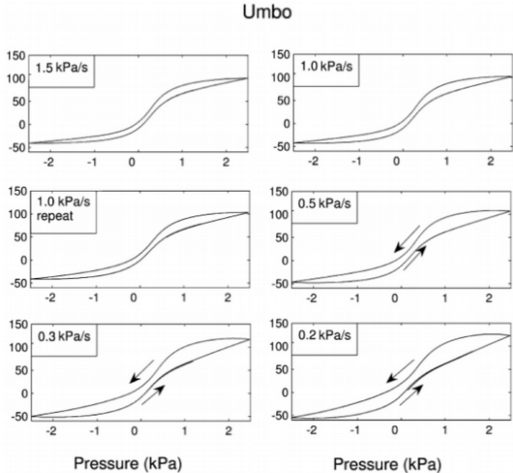
Fig. 3–7: Umbo displacement as a function of pressure at different ultra-low frequencies obtained in one ear (Dirckx et al., 2006)
