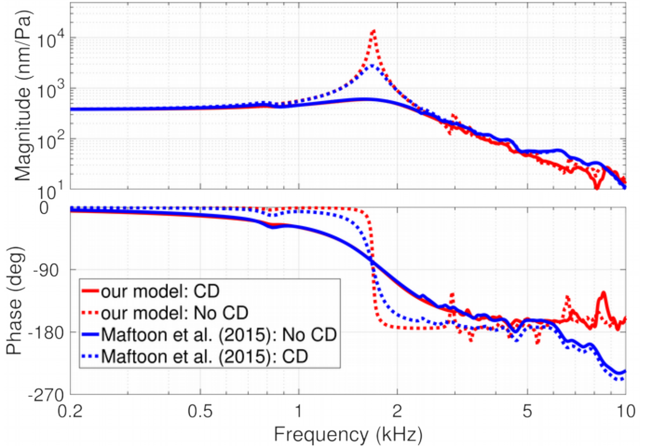
Fig. 5–6: Comparison of our model umbo response with that of Maftoon's model with cochlear damping (CD) and with no cochlear damping (No CD).
