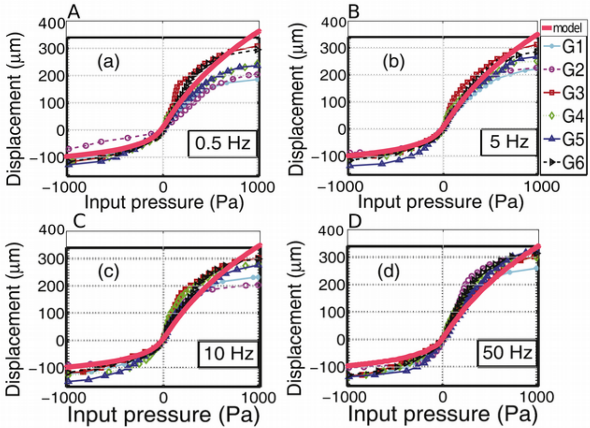
Fig. 5–20: Comparison of displacement of gerbil umbo at different frequencies with experimental data of Salih et al. (2016). (a) 0.5 Hz, (b) 5 Hz, (c) 10 Hz and (d) 50 Hz.
