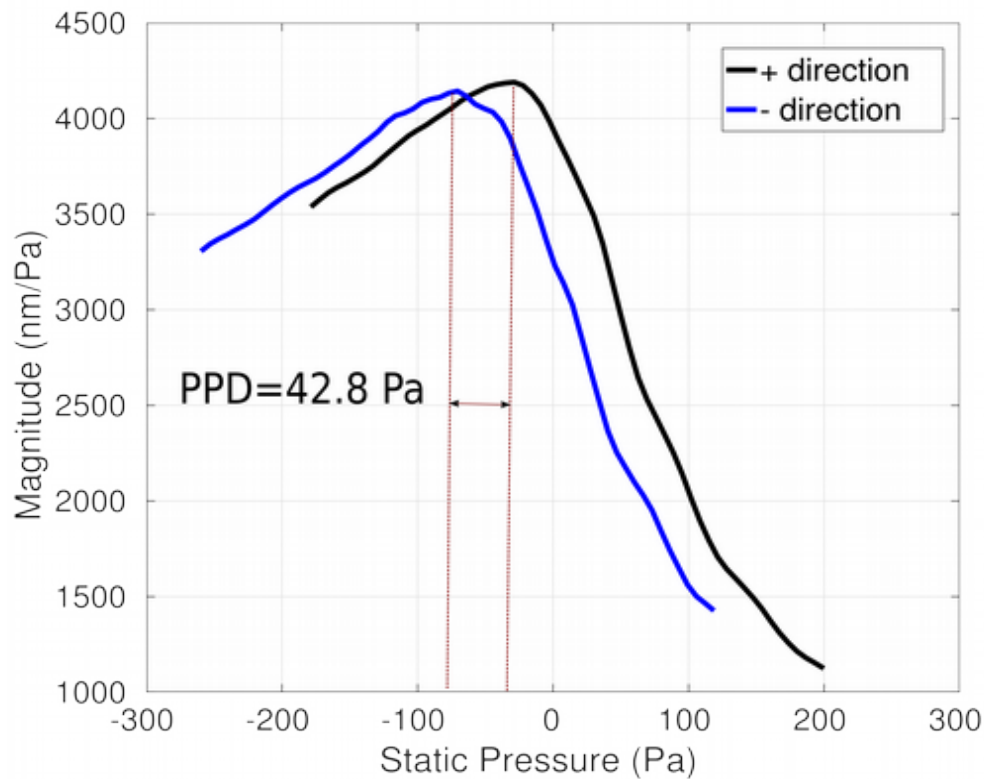
Fig. 5–19: Umbo magnitude displacement normalized by sound pressure as function of static pressure in both directions. PPD refers to the peak pressure difference defined in section 3.3.4.1, that is, the separation between the two pressure peaks obtained during the increasing and decreasing parts of the pressure cycle. “+ direction” stands for positive direction (from -2.5 kPa to +2.5 kPa) and “– direction” is for negative direction (from +2.5 kPa to -2.5 kPa).
