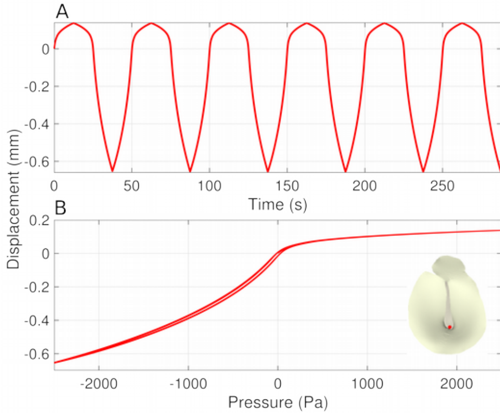
Fig. 5–11: Simulated umbo response to about 6 cycles of triangular waves of pressure for a pressure-change rate of 200 Pa/s. A: Umbo displacement as a function of time. B: Umbo displacement as a function of pressure for all cycles.
