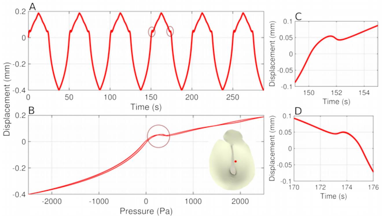
Fig. 5–12: Simulated anterior PT response to about 6 cycles of triangular waves of pressure for a pressure-change rate of 200 Pa/s. A: Displacement as a function of time. B: Displacement as a function of pressure for all cycles. Circles highlight some regions of buckling. C: Magnified view of the left circle in A. D: Magnified view of the right circle in A.
