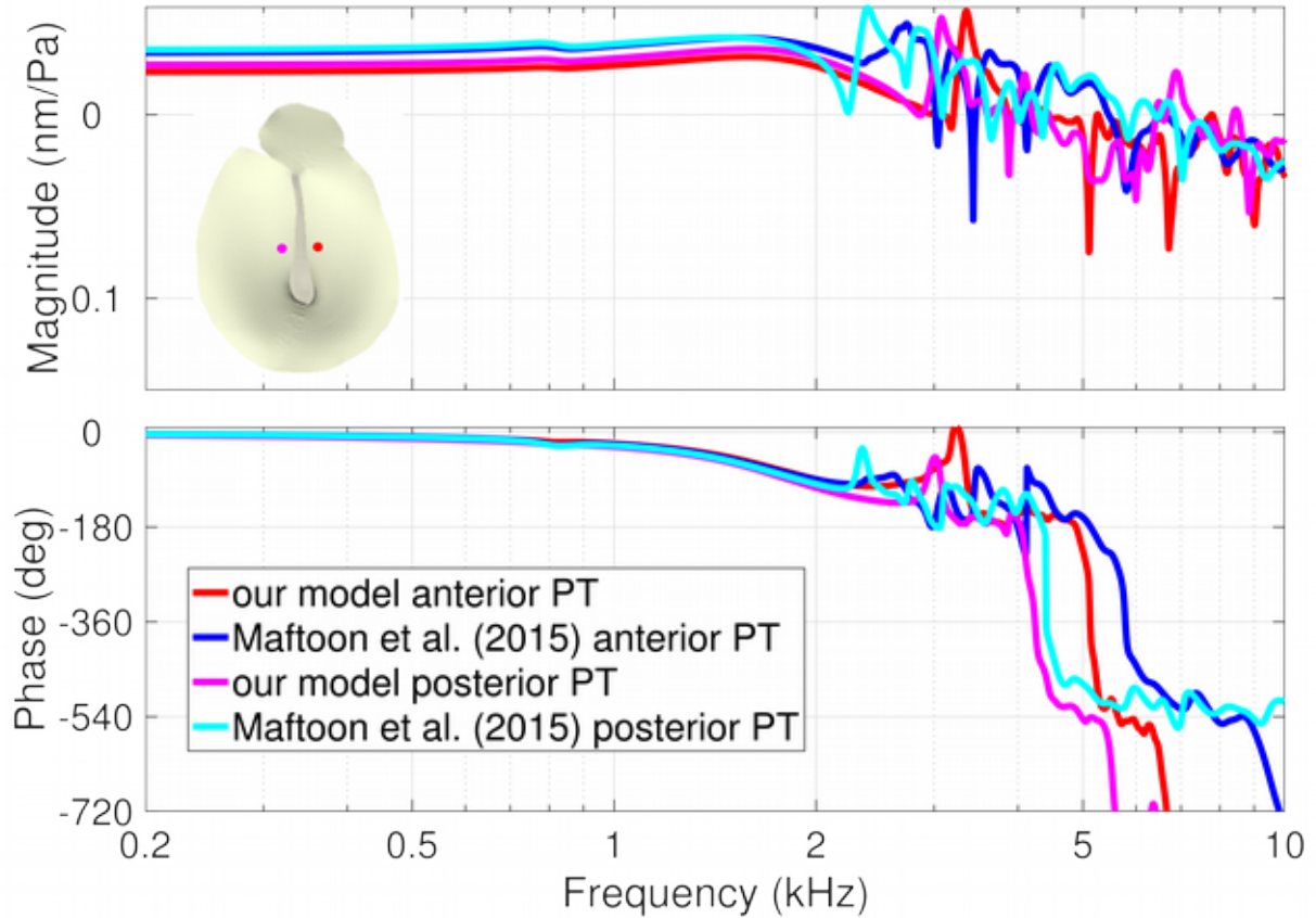
Fig. 5–10: Comparison of our gerbil model response with Maftoon’s model (2015) response at a point in anterior PT and a point in posterior PT
