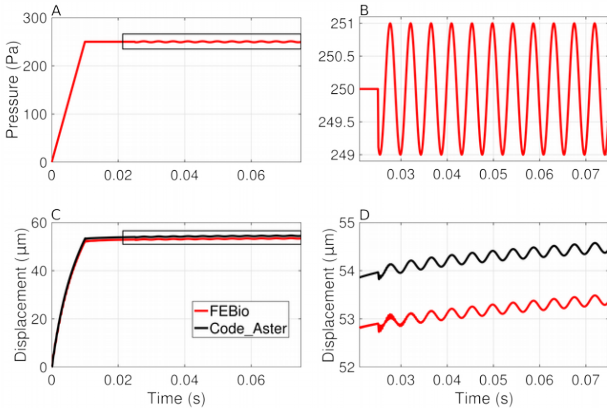
Fig. 5–21: Results for a quasi-static pressure combined with a 226-Hz pure tone using FEBio and Code_Aster. A: Input pressure signal. B: Magnified view corresponding to the rectangle in A to show the acoustic stimulus. C: Umbo displacement as a function of time. D: Magnified view corresponding to the rectangle in C.
