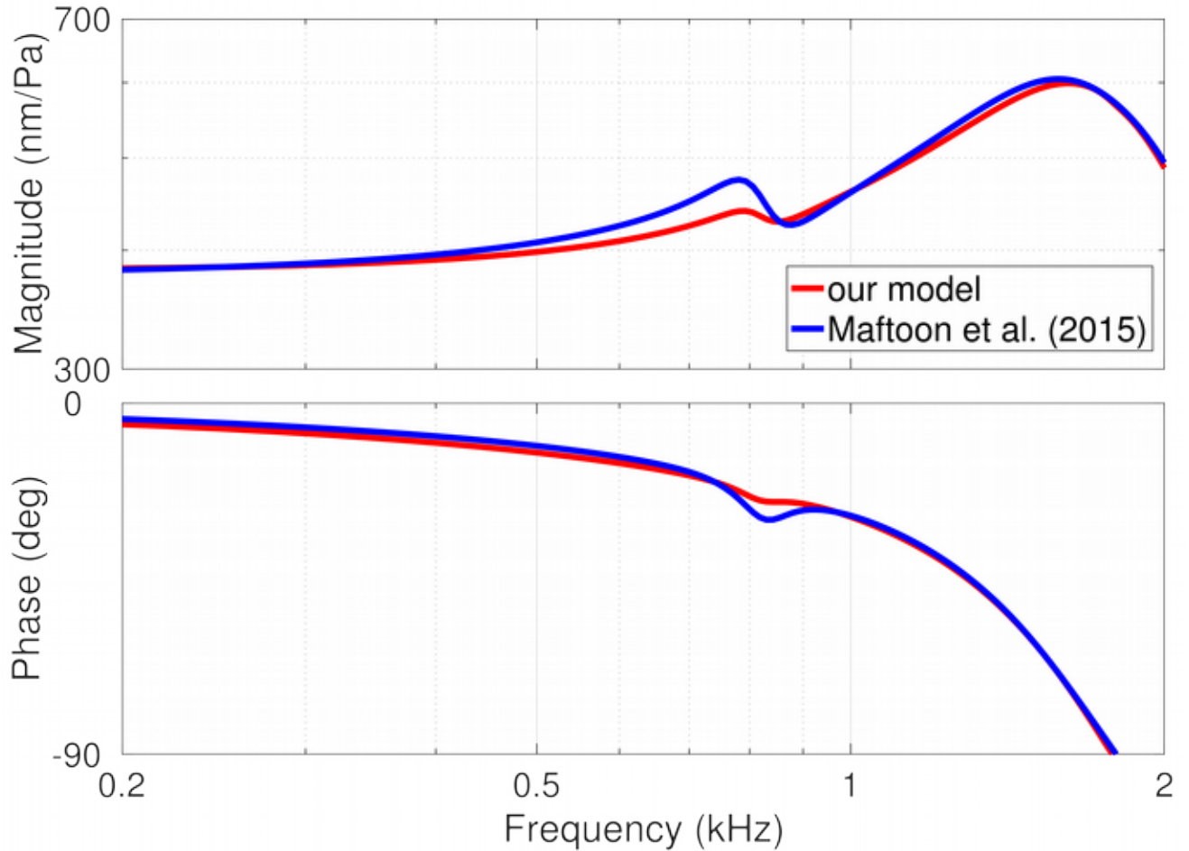
Fig. 5-5: A magnified view of part of Fig 5-3 to clearly show the effect of the flat PF on the umbo response, namely, a maximum and minimum and in the displacement magnitude that corresponds to the resonance frequency of the PF.
