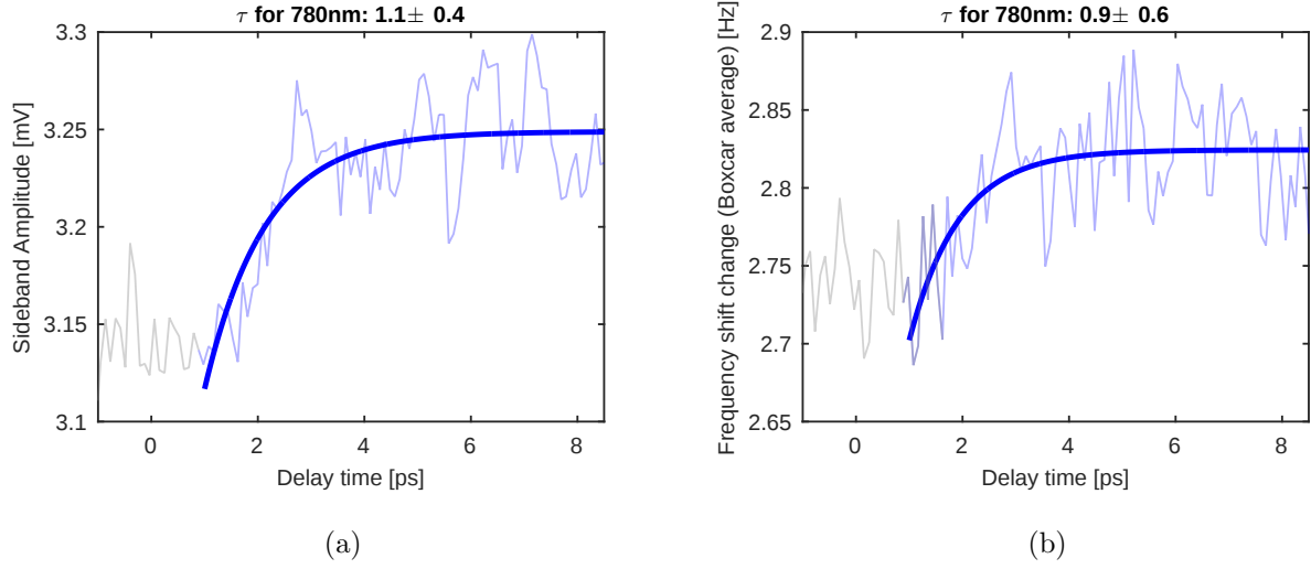
Figure 6.7: Photocarrier decay measured in LT-GaAs without \delta F feedback. A 780 nm pump laser and a 610 nm probe laser is used. Decay time recording using the direct side band detection (a) compared to the boxcar averaging in the time domain (b) is shown. The decay is fitted to an exponential decay with a time constant of \tau = 1.1 \pm 0.4 ps for a) and \tau = 0.9 \pm 0.6 ps for b)
