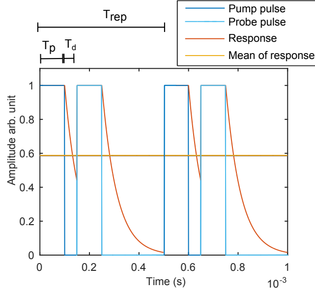
Figure 6.2: Simulation of stimulated pulse train and potential response with an exponential decay.
