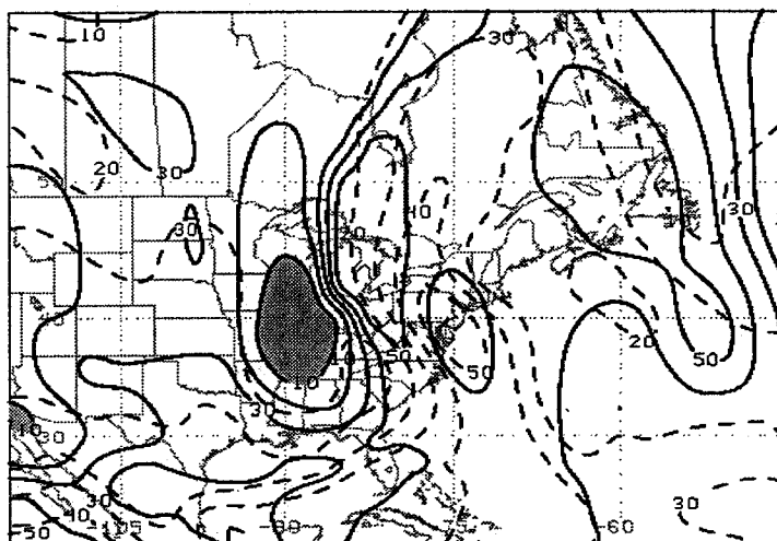
11 00 UTC 16 Oct 1954
