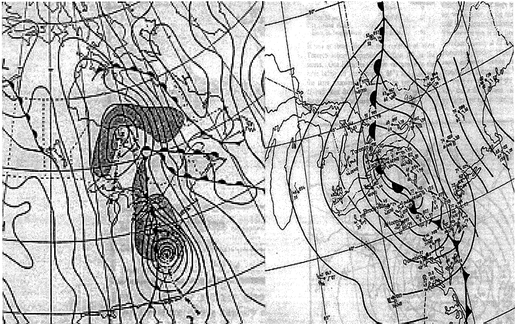
Fig. 1.3.1. (a) surface map at 1830 UTC 15 October from Knox (1955); (b) surface map at 0030 UTC 16 October from Knox (1955).
