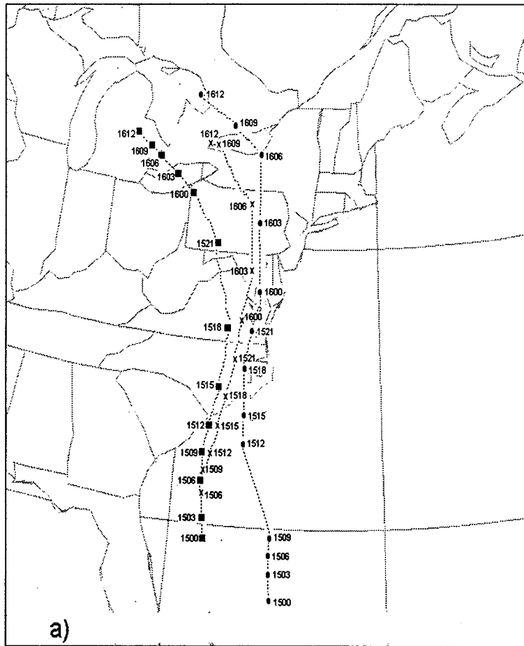
Fig. 5.8.1. (a) Tracks of Hazel in MC2 simulations (CONT in solid circles, BOG36 in solid squares, BOG12 in 'X'); (b) Tracks of Hazel in Observations (X) (Knox 1955) and control model simulation by Anthes (1990) (solid circles) from Anthes (1990).
