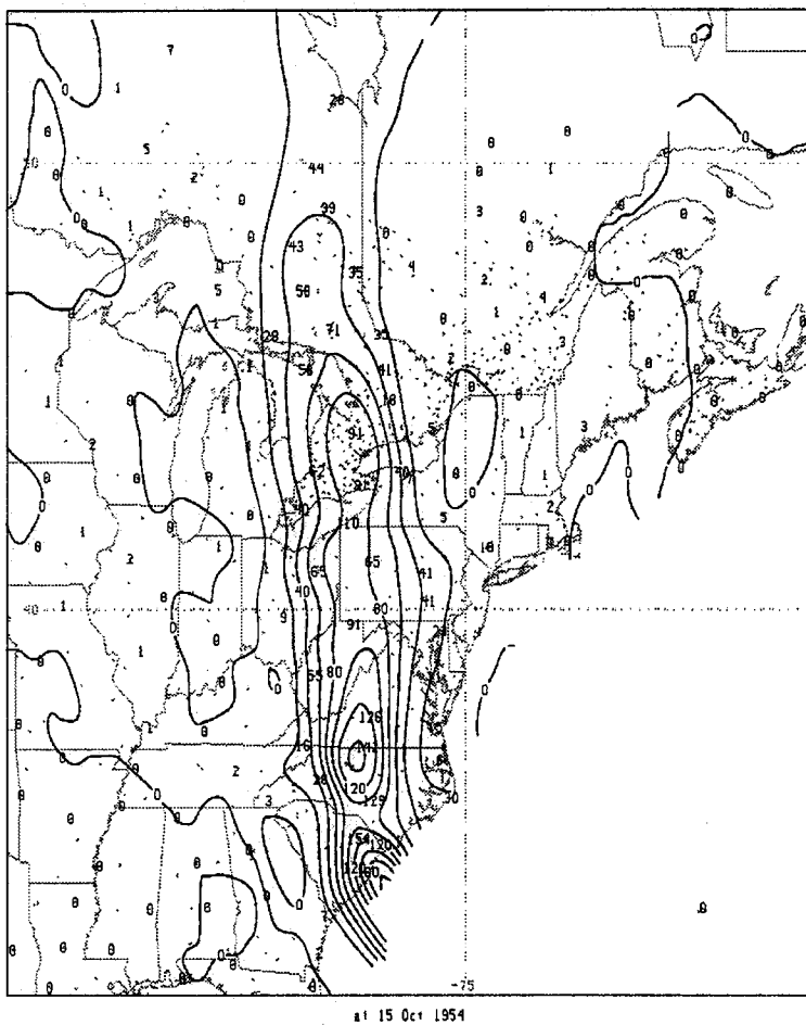
Fig. 3.6.1. (a) Storm total precipitation (solid, contour interval of 20 mm). Values plotted at select stations, dots indicate reporting stations; (b) Sea level pressure (solid, contour interval of 4 hPa) from Knox (1955).
