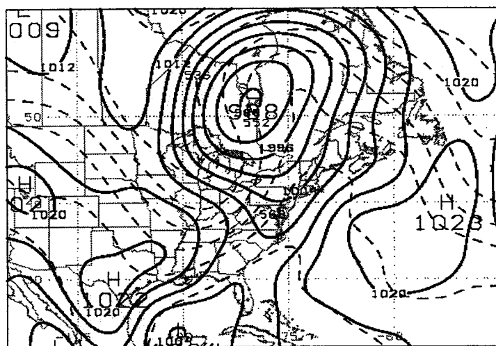
k 00 UTC 15 Oct 1995
