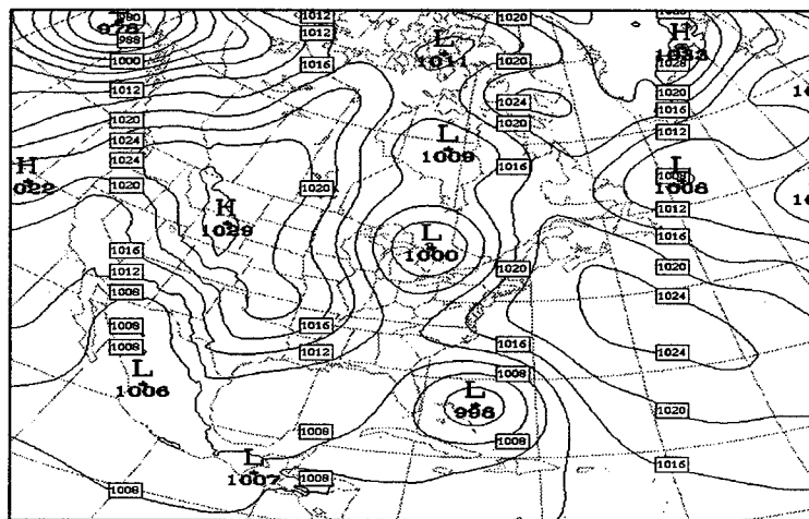
a) 00 UTC 15 Oct
