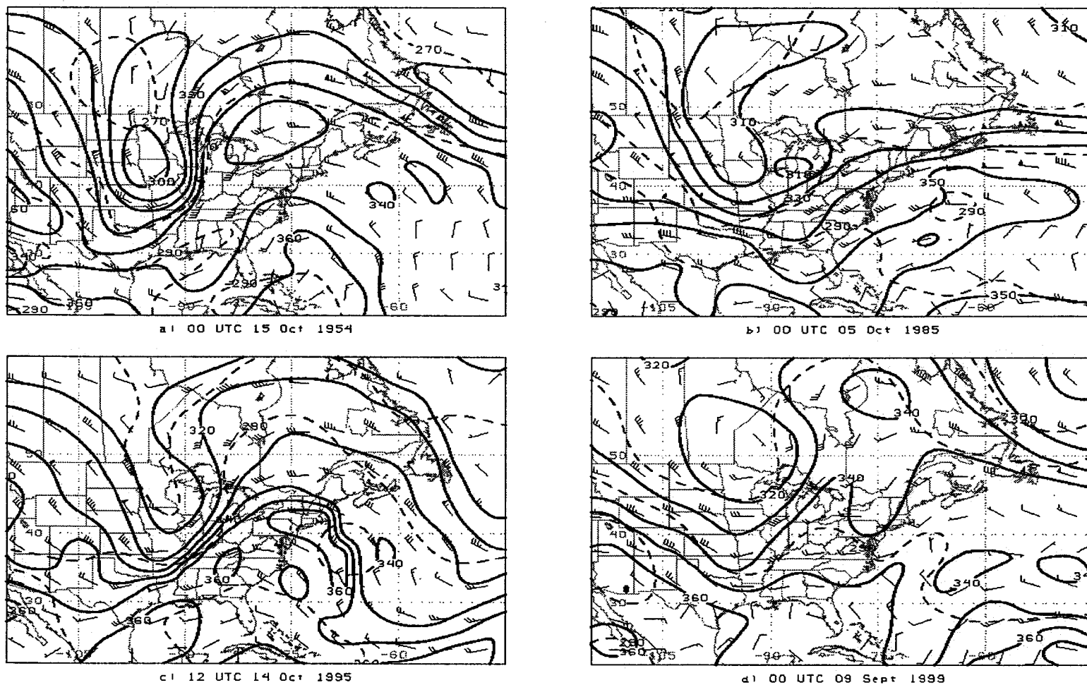
Fig. 4.4.1. Dynamic tropopause potential temperature (solid, contour interval of 10 K), winds on the dynamic tropopause ( \text{m s}^{-1} ), and 850 hPa potential temperature (dashed, contour interval of 10 K). For (a) Hazel; (b) 1985 analogue; (c) 1995 analogue; (d) 1999 analogue.
