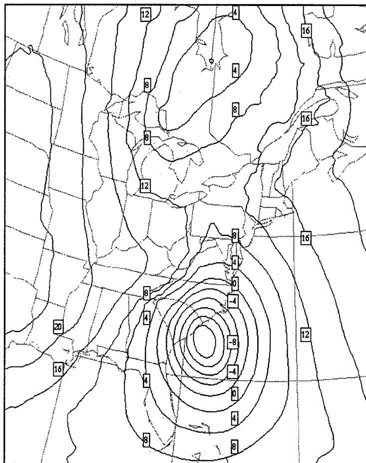
a) 15 UTC 15 Oct
