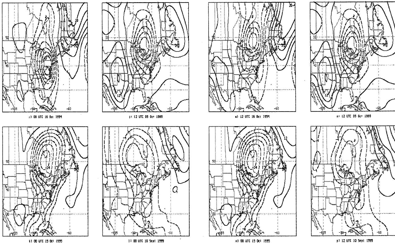
Fig. 4.2.1. (Continued) For: (i) and (m) Hazel; (j) and (n) 1985 analogue; (k) and (o) 1995 analogue; (l) and (p) 1999 analogue.
