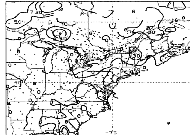
d) 9-10 Sept 1999
