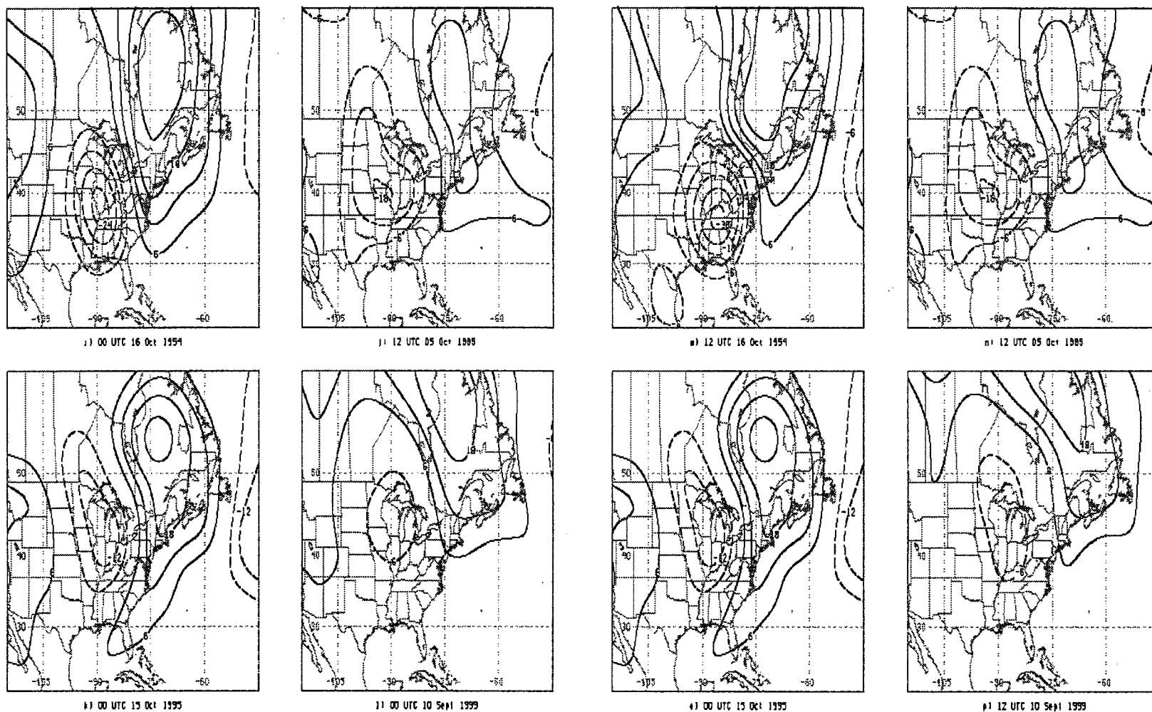
Fig. 4.2.2. (Continued) For: (i) and (m) Hazel; (j) and (n) 1985 analogue; (k) and (o) 1995 analogue; (l) and (p) 1999 analogue.
