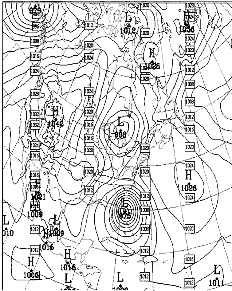
a) 03 UTC 15 Oct
