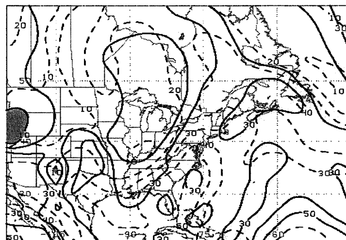
11 00 UTC 10 Sept 1999
