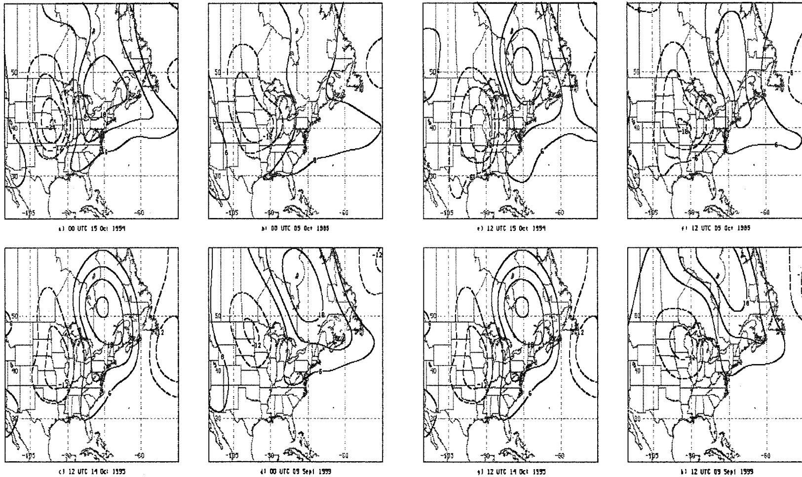
Fig. 4.2.2. 1000-500 hPa thickness anomalies (positive anomalies in solid, negative anomalies in dashed, contour interval of 6 dam). Zero contour is omitted. For: (a) and (e) Hazel; (b) and (f) 1985 analogue; (c) and (g) 1995 analogue; (d) and (h) 1999 analogue.
