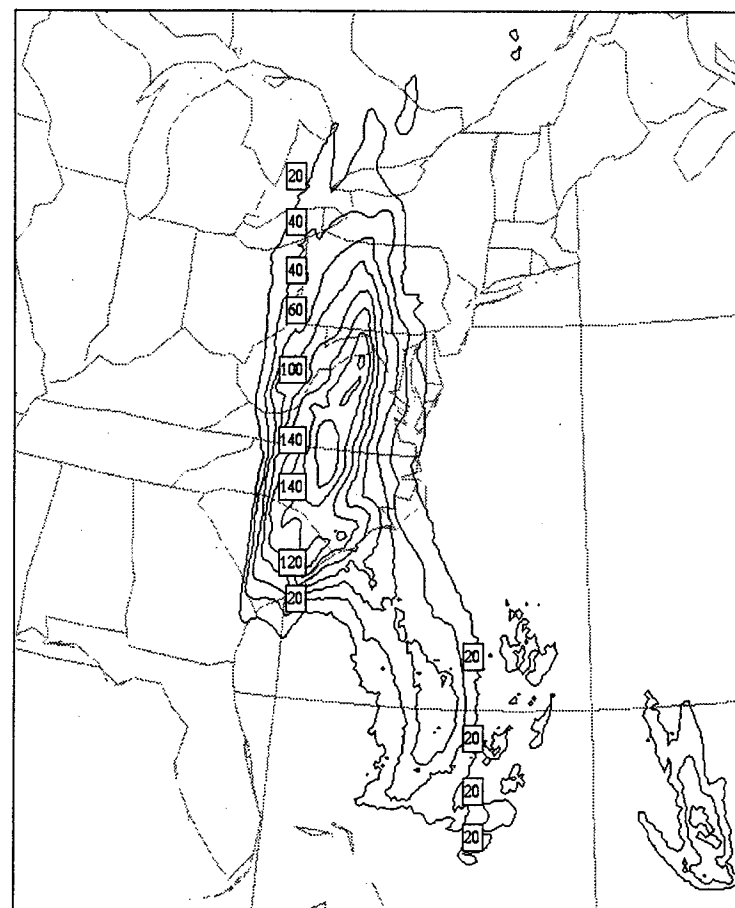
b) 15-16 October
