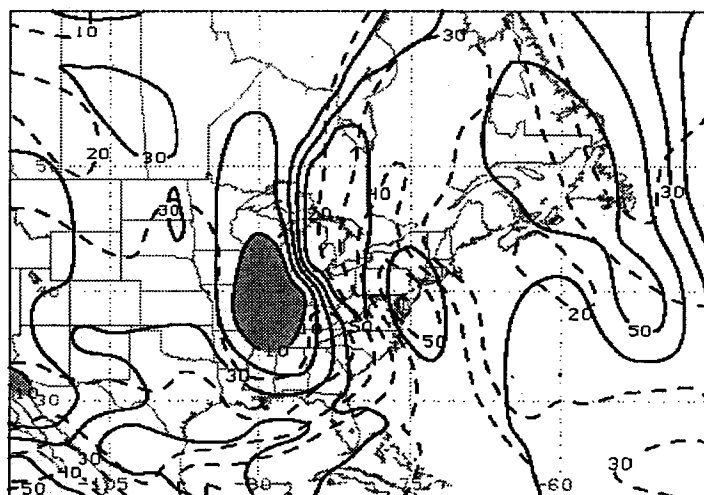
c) 00 UTC 16 Oct 1954
