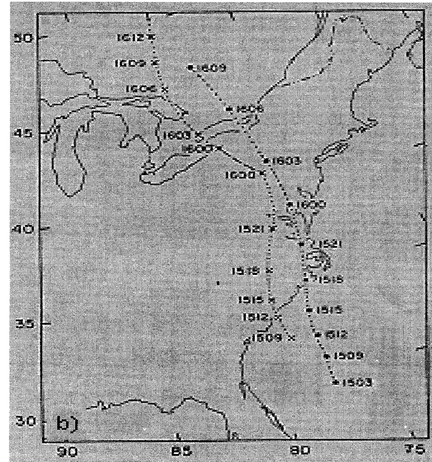
Fig. 5.8.1. (a) Tracks of Hazel in MC2 simulations (CONT in solid circles, BOG36 in solid squares, BOG12 in 'X'); (b) Tracks of Hazel in Observations (X) (Knox 1955) and control model simulation by Anthes (1990) (solid circles) from Anthes (1990).
