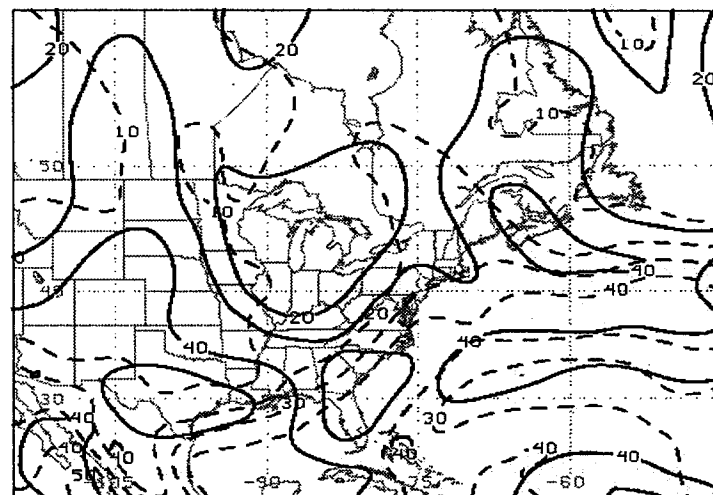
11 12 UTC 05 Oct 1985
