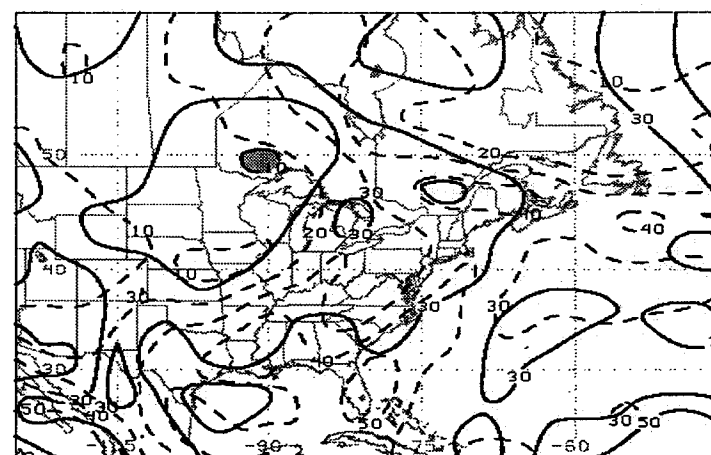
d) 00 UTC 09 Sept 1999
