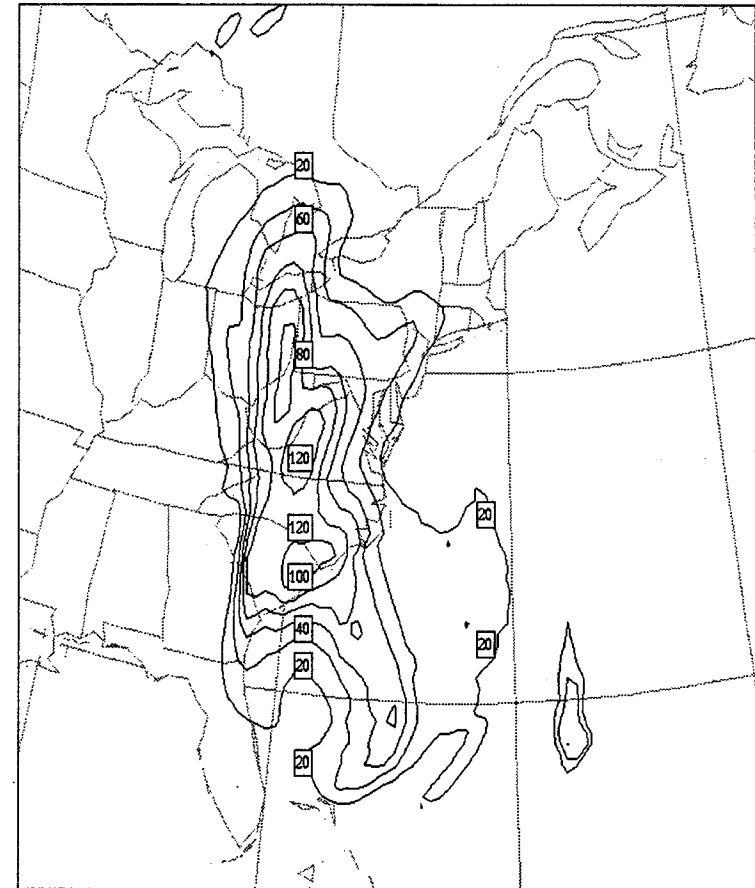
b) 15-16 October
