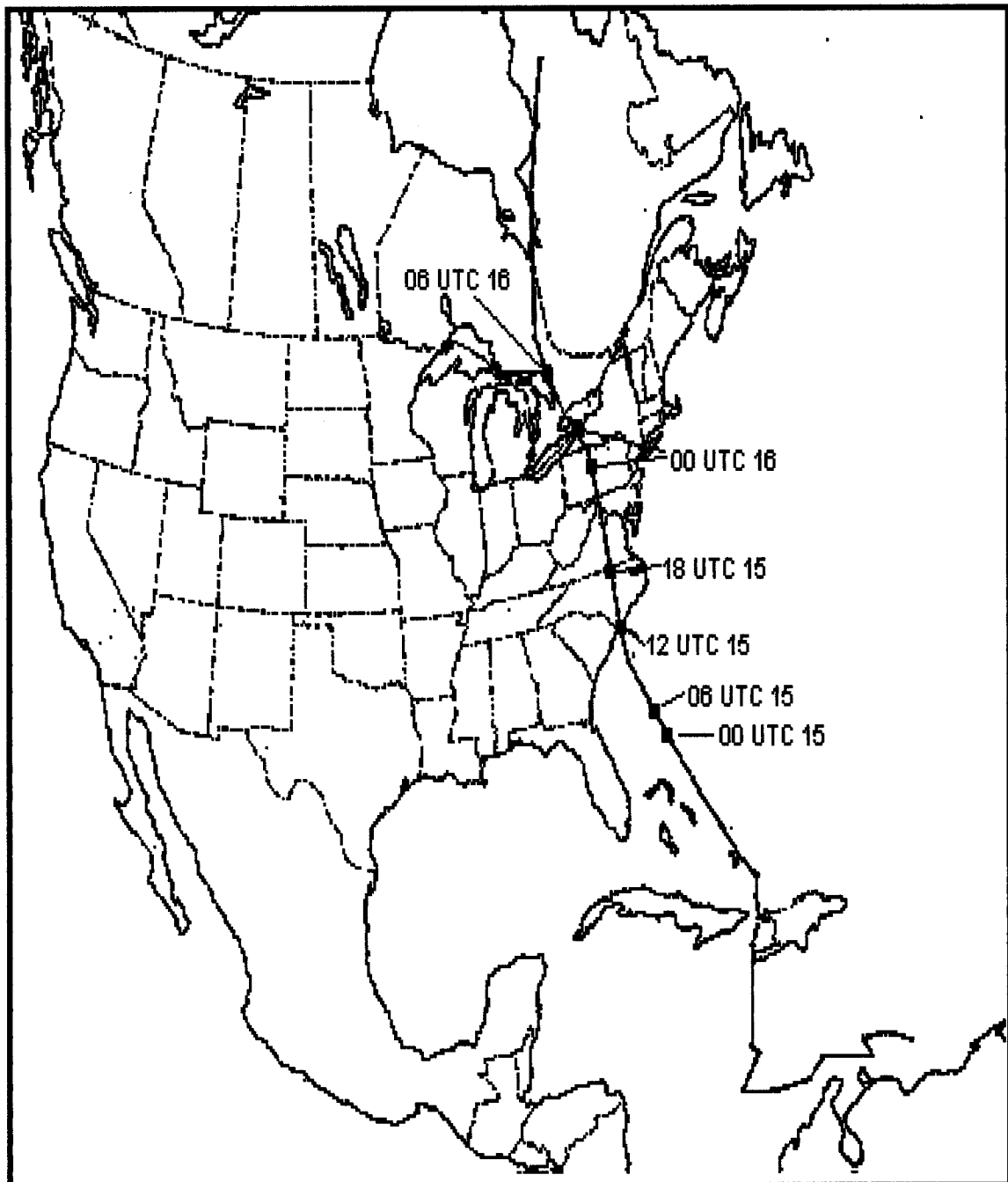
Fig. 1.3.2. Path of the storm Hazel, 6 October – 17 October 1954, adapted from Mason et al. (1955) .
