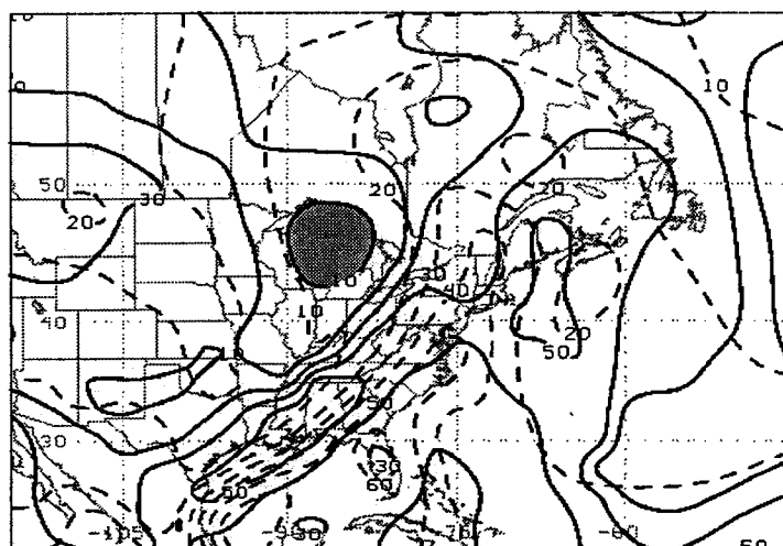
11 00 UTC 15 Oct 1995
