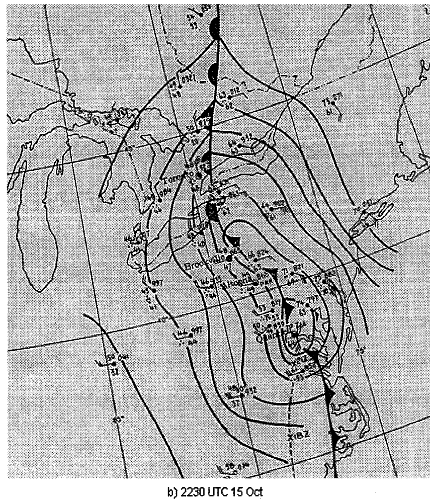
Fig. 3.6.1. (a) Storm total precipitation (solid, contour interval of 20 mm). Values plotted at select stations, dots indicate reporting stations; (b) Sea level pressure (solid, contour interval of 4 hPa) from Knox (1955).
