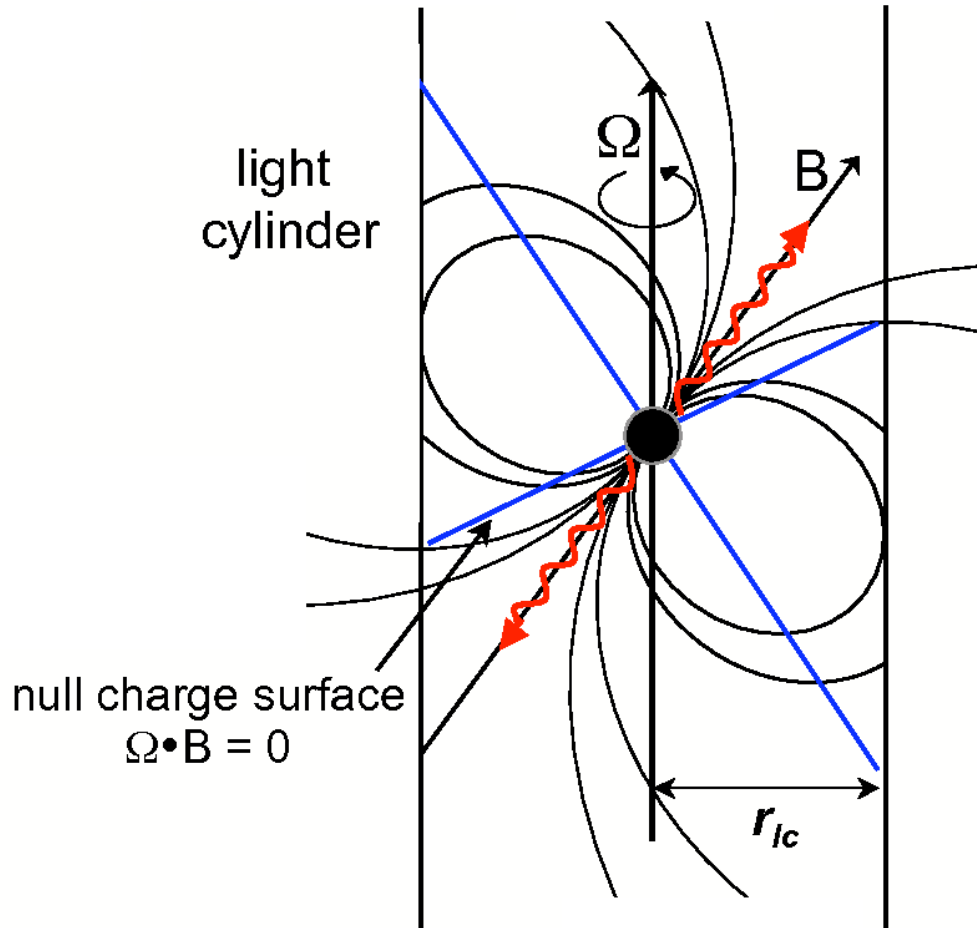
Figure 1.2: Schematic of a pulsar and its magnetosphere. In this case the rotation and magnetic axes are misaligned. The light cylinder radius is shown. The null charge density lines ( \Omega \cdot B = 0 ) separate the regions of positive and negative charges. Radiation beams inclined to the rotation axis will then result in periodic signals if they are intercepted by our line of sight and the star will be detected as a pulsar.
