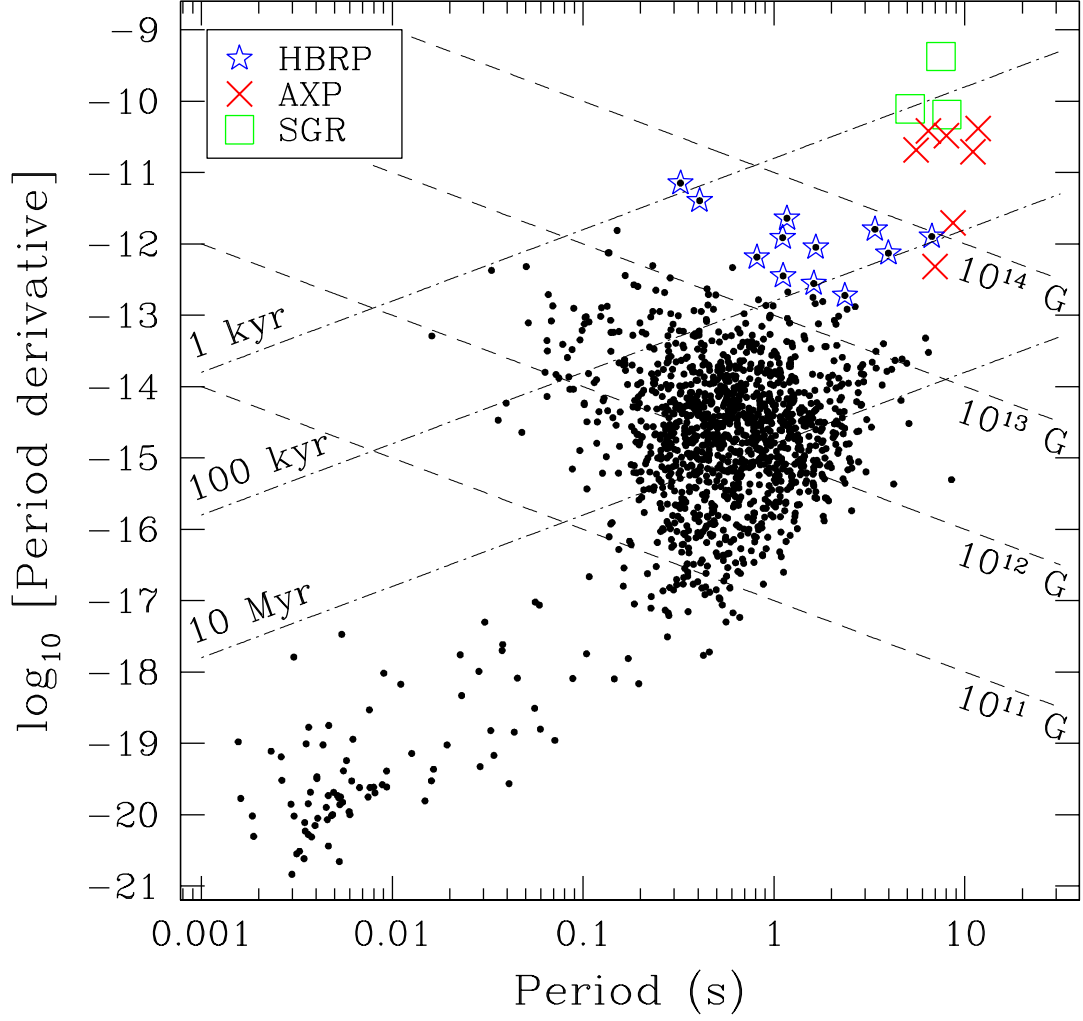
Figure 4.1: P - \dot{P} diagram showing high magnetic field radio pulsars (HBRPs) with estimated magnetic fields > 2 \times 10^{13} \text{ G} as a reference. Magnetars are also shown as labeled.
