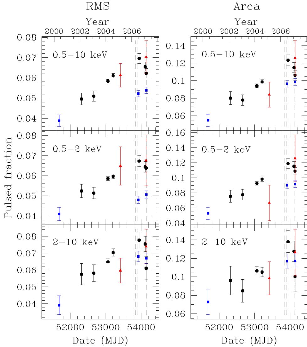
Figure 5.3: RMS ( left ) and area ( right ) pulsed fractions in the 0.5–10 keV ( top ), 0.5–2 keV ( center ) and 2–10 keV ( bottom ) ranges. Values shown correspond to those measured with XMM-Newton (black circles), Chandra (blue squares) and Swift (red triangles). The dashed lines indicate the three burst epochs.
