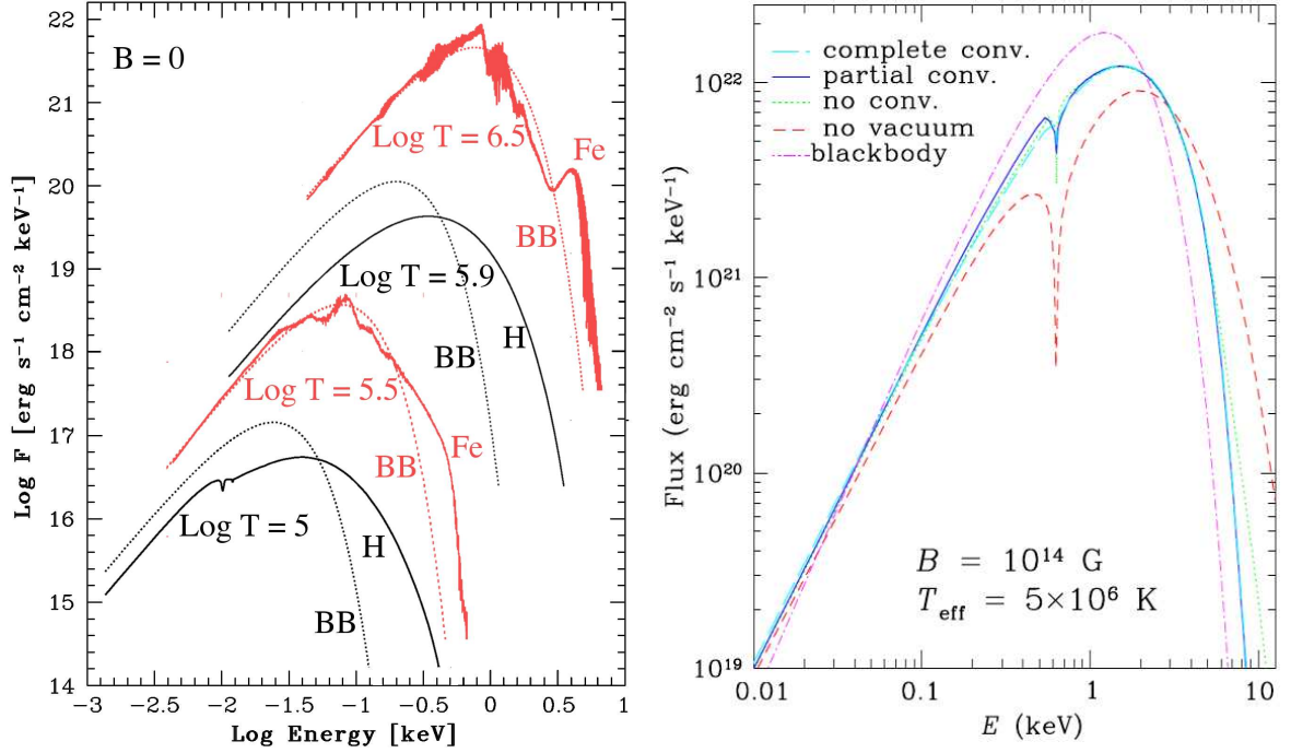
Figure 1.5: Sample emergent spectra from the atmosphere of a NS at various temperatures, compositions and magnetic fields. Left: H (black) and Fe (red) atmospheres at different temperatures and zero magnetic field. Dashed lines show the corresponding blackbody spectrum. The effect of a light element atmosphere is clearly visible: a high energy tail is produced and at low temperatures weak spectral features are present. Heavy elements result in a large number of spectral features and shape closer to a blackbody. This figure was produced using data by Pavlov et al. publicly available at http://www.ioffe.rssi.ru/astro/Stars/ . Right: Spectra of a fully ionized H atmosphere in the presence of a large magnetic field. A large proton cyclotron line and hard-energy tail are visible when vacuum polarization is not taken into account, which together with mode conversion results in softer spectra (though still harder than a blackbody) and less significant spectral features. Adapted from van Adelsberg & Lai (2006).
