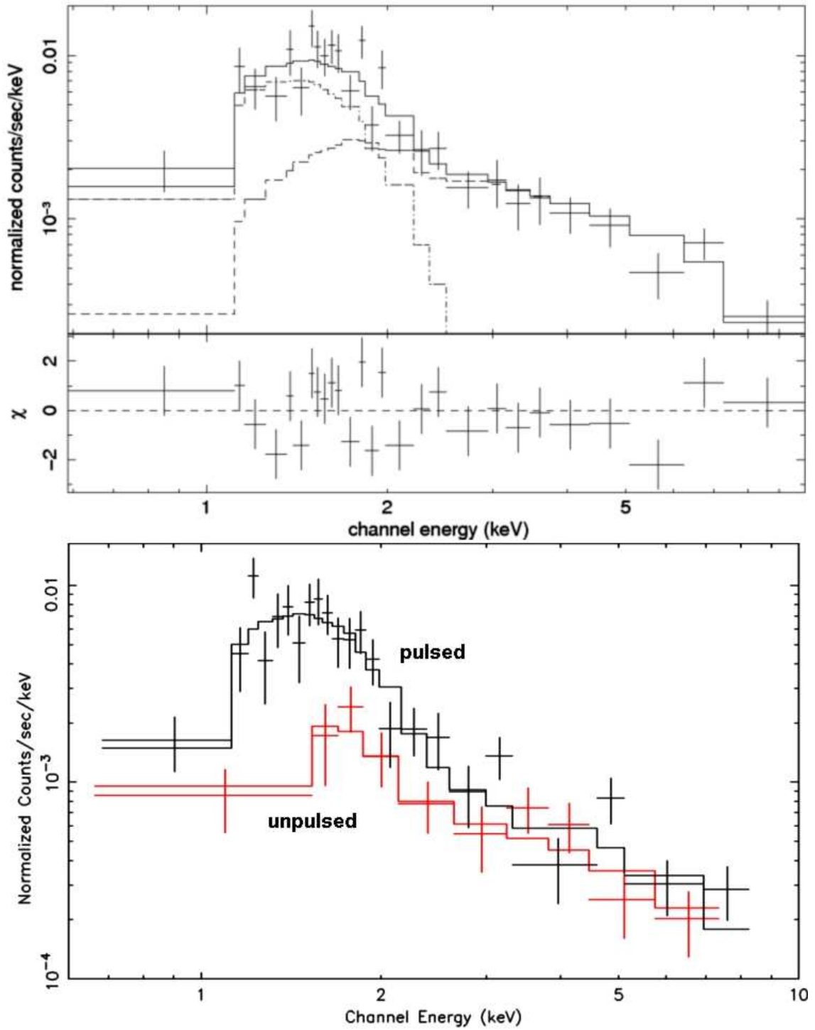
Figure 4.4: Top: Phase-averaged PN spectra showing individual spectral components (blackbody dominating at small energies). Bottom: PN spectra obtained for the pulsed ( black , phases 0.7–1.3) and unpulsed ( red , 0.3–0.7) regions of the pulse profile with their respective best-fit blackbody plus power-law model (solid curves).
