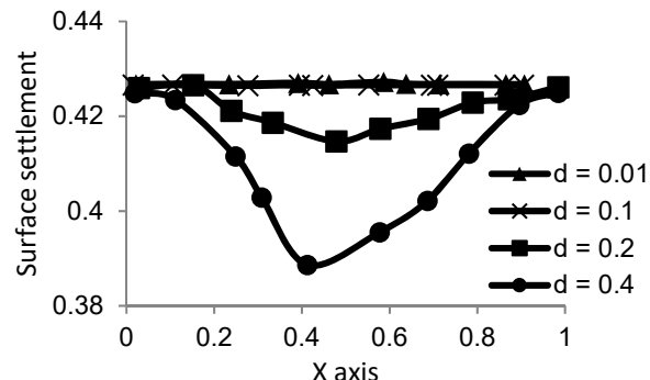
Figure 6 Effect of trapdoor displacement on surface settlement
