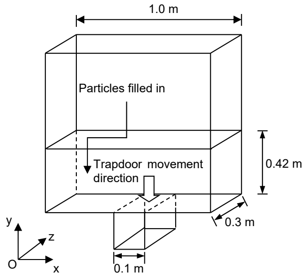
Figure 2 Schematic of the trapdoor geometry
