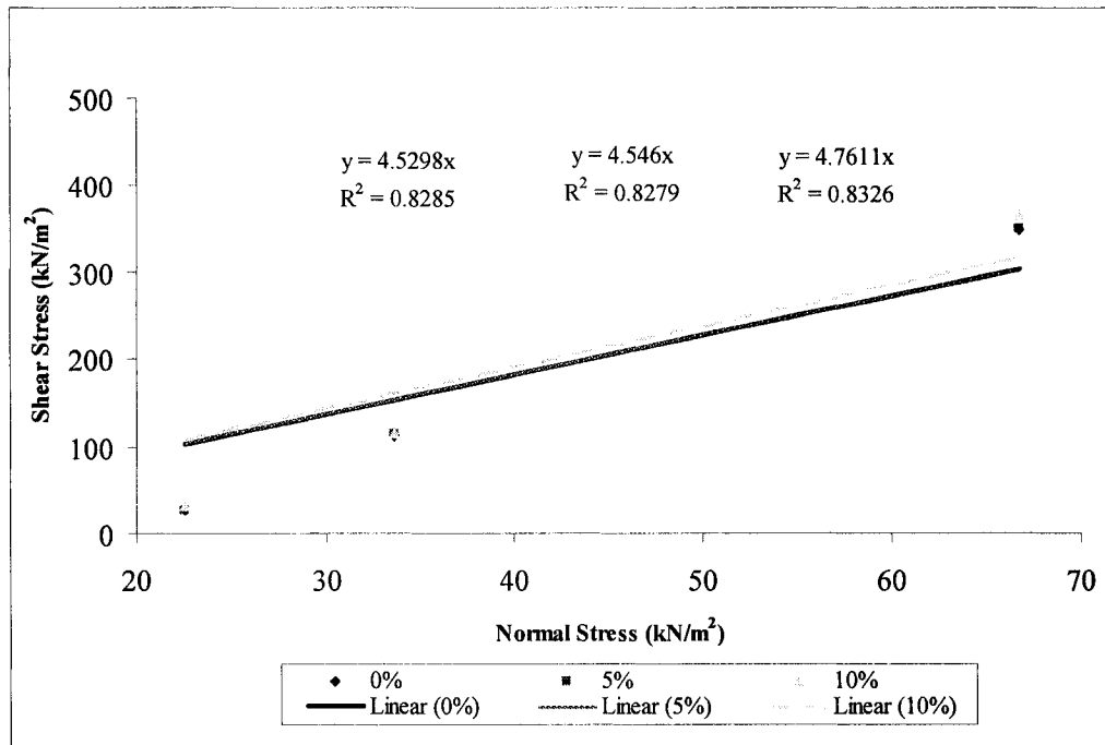
Figure 4.10: Shear Stress ( \text{kN/m}^2 ) versus Normal Stress ( \text{kN/m}^2 ) for >250 \mu\text{m} KMI zeolite at 0%, 5%, and 10% moisture content under normal loads of 22.6, 33.6, 66.8 \text{kN/m}^2 to determine angle of internal friction
