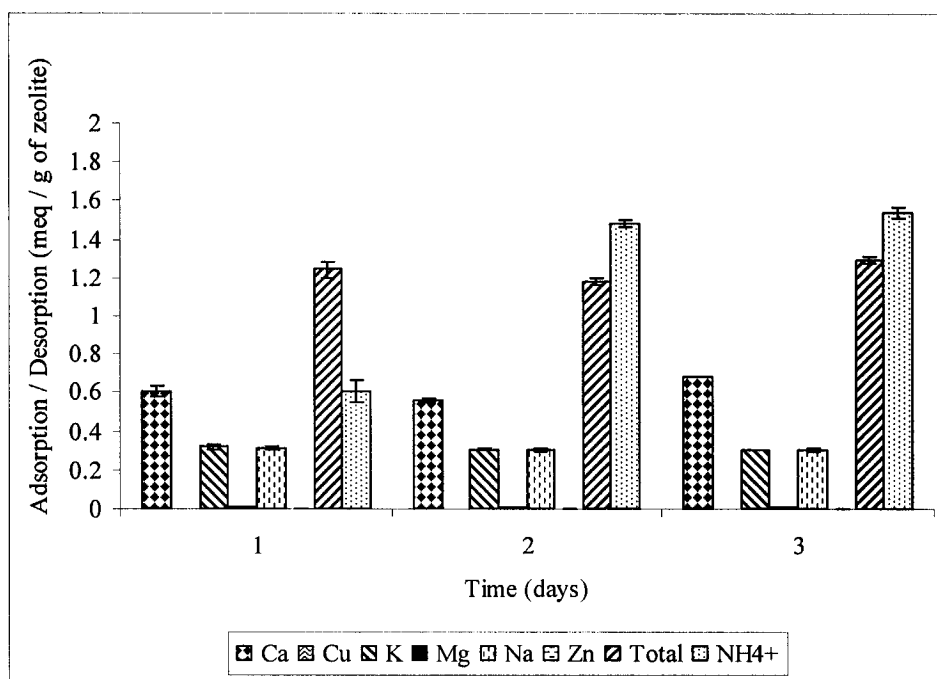
Figure 4.5: Mineral desorption (Ca, Cu, Mg, Na, Zn, and Total) versus \text{NH}_4^+ adsorption under a neutral pH at 22°C for < 250 \mu\text{m} Steel Head zeolite in a 0.05M \text{NH}_4\text{Cl} solution (meq/g of zeolite). Total refers to summation of Ca, Cu, Mg, Na and Zn mineral desorption
