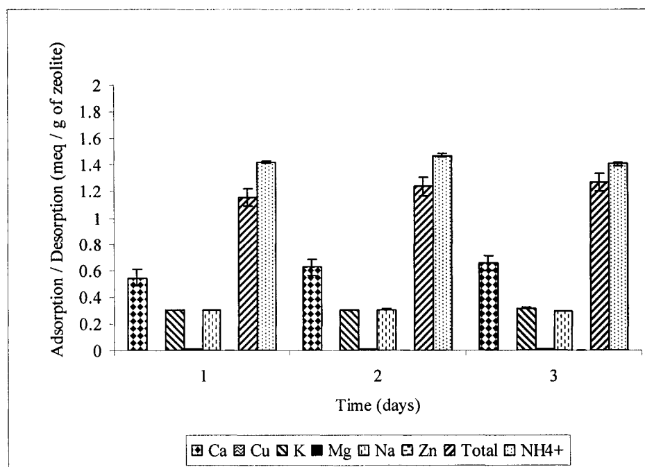
Figure 4.4: Mineral desorption (Ca, Cu, Mg, Na, Zn, and Total) versus NH 4 + adsorption under a neutral pH at 22°C for > 250 μm Steel Head zeolite in a 0.05M NH 4 Cl solution (meq/g of zeolite). Total refers to summation of Ca, Cu, Mg, Na and Zn mineral desorption
