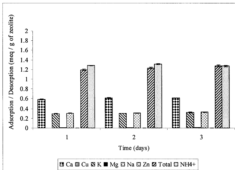
Figure 4.6: Mineral desorption (Ca, Cu, Mg, Na, Zn, and Total) versus \text{NH}_4^+ adsorption under a neutral pH at 22°C for mixed Steel Head zeolite in a 0.05M \text{NH}_4\text{Cl} solution (meq/g of zeolite). Total refers to summation of Ca, Cu, Mg, Na and Zn mineral desorption
