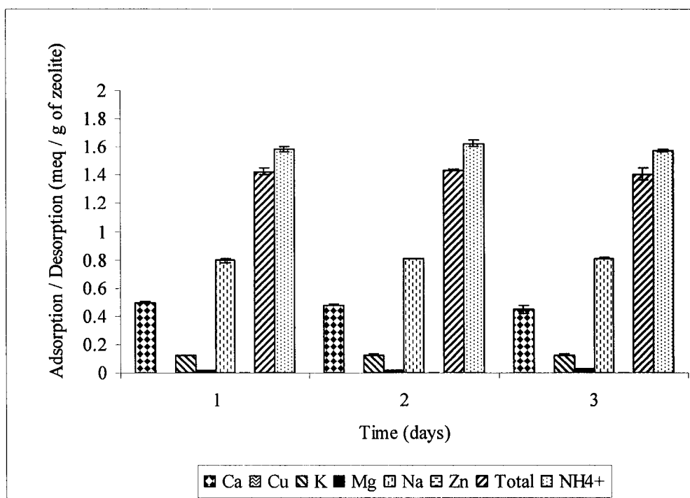
Figure 4.1: Mineral desorption (Ca, Cu, Mg, Na, Zn, and Total) versus \text{NH}_4^+ adsorption under a neutral pH at 22°C for > 250 µm KMI zeolite in a 0.05M \text{NH}_4\text{Cl} solution (meq/g of zeolite). Total refers to summation of Ca, Cu, Mg, Na and Zn mineral desorption
