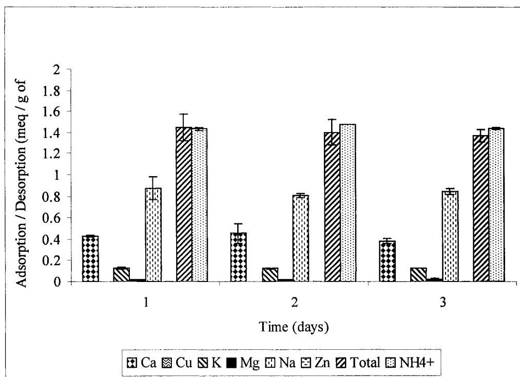
Figure 4.3: Mineral desorption (Ca, Cu, Mg, Na, Zn, and Total) versus NH 4 + adsorption under a neutral pH at 22°C for mixed KMI zeolite in a 0.05M NH 4 Cl solution (meq/g of zeolite). Total refers to summation of Ca, Cu, Mg, Na and Zn mineral desorption
