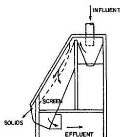
Figure 3.5: Sloping Stationary Screen (Miner et al., 2000b)
