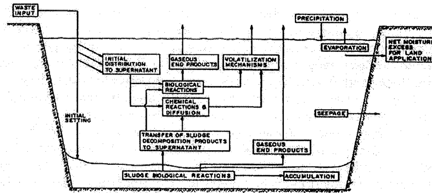
Figure 3.12: Anaerobic Lagoon Storage (Miner et al., 2000c)
