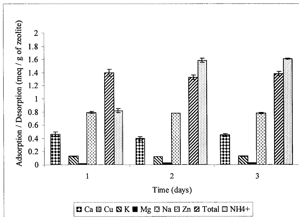
Figure 4.2: Mineral desorption (Ca, Cu, Mg, Na, Zn, and Total) versus \text{NH}_4^+ adsorption under a neutral pH at 22°C for < 250 µm KMI zeolite in a 0.05M \text{NH}_4\text{Cl} solution (meq/g of zeolite). Total refers to summation of Ca, Cu, Mg, Na and Zn mineral desorption
