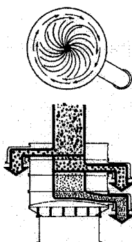
Figure 3.6: Vibrating Screen Solid-Liquid Separator (Miner et al., 2000b)
