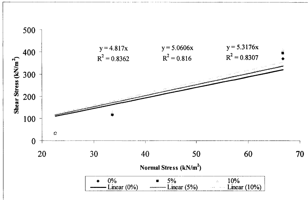
Figure 4.9: Shear Stress ( \text{kN/m}^2 ) versus Normal Stress ( \text{kN/m}^2 ) for <250 \mu\text{m} KMI zeolite at 0%, 5%, and 10% moisture content under normal loads of 22.6, 33.6, 66.8 \text{kN/m}^2 to determine angle of internal friction
