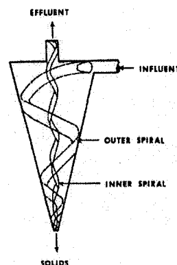
Figure 3.8: Hydro-cyclone (Zhang and Westerman, 1997)
