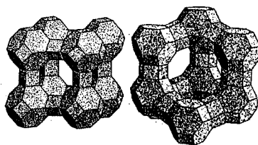
Figure 3.3: Arrangements of truncated cubo-octahedron (sodalite) units to enclose large central cavities (cages). Left = sodalite unit connected by double 4-rings of oxygen in the structure of synthetic zeolite A. Right = sodalite units connected by double 6-ring of oxygen in structure of faujasite and synthetic zeolites X and Y (Mumpton and Fishman, 1977)
