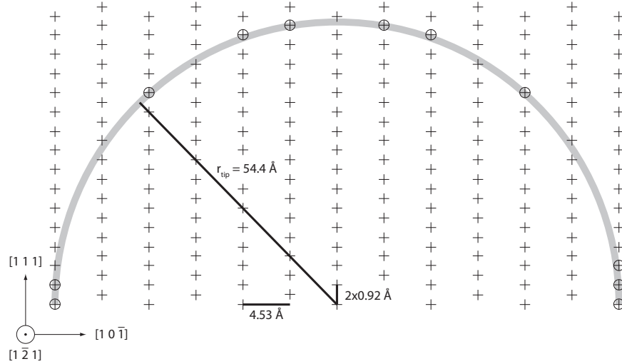
Figure 3.11 Tip atom selection for tip reconstruction for a radius of r_{tip} = 5.4 nm.
