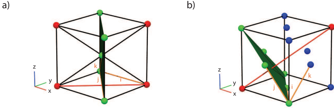
Figure A.2 a) Visualization of the bcc 110 ijk vectors (in orange). b) ijk for the fcc 111 Au model.
