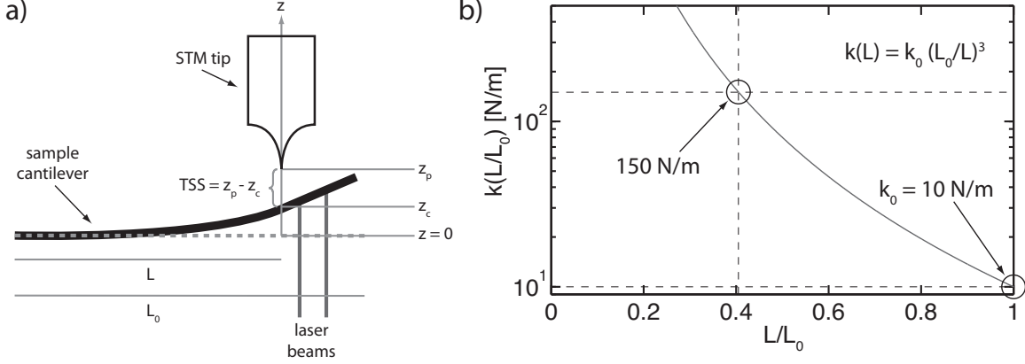
Figure 2.4 a) Distances that need to be known in order to calculate the tip sample separation (TSS). The tip sits at a distance L from the cantilever base. b) Estimation of the spring constant at the distance L from the cantilever base. A value of 150 N/m has been used for most of the experiments
