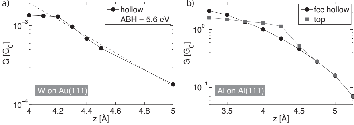
Figure 4.7 Tunneling data from simulations that includes relaxation. a) Data for W on Au(111) [40]. b) Data for Al on Al(111) [41]. Details see text.
