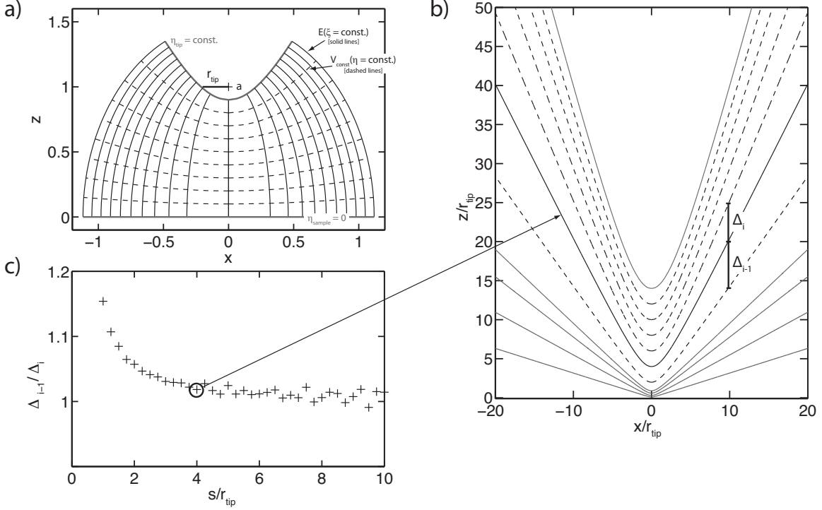
Figure B.1 a) The electric field and equipotential lines for a hyperbolic geometry. The tipshape is given by a constant \eta_{tip} , the sample by \eta_{sample} = 0 . Lines of constant \xi represent the electric field lines and lines of constant \eta equipotentials. b) The tip shape is not maintained for small tip-sample distances. The tip shape diverges at a tip-sample distance of s = 4r_{tip} . (The blue shapes are not separated by a constant distance increment. All other curves are.) c) A plot of differences of z(x=10 r_{tip}) for consecutive plots with equal spacing in s – see indication in b). The differences become very similar for distances with s \geq 4r_{tip} .
