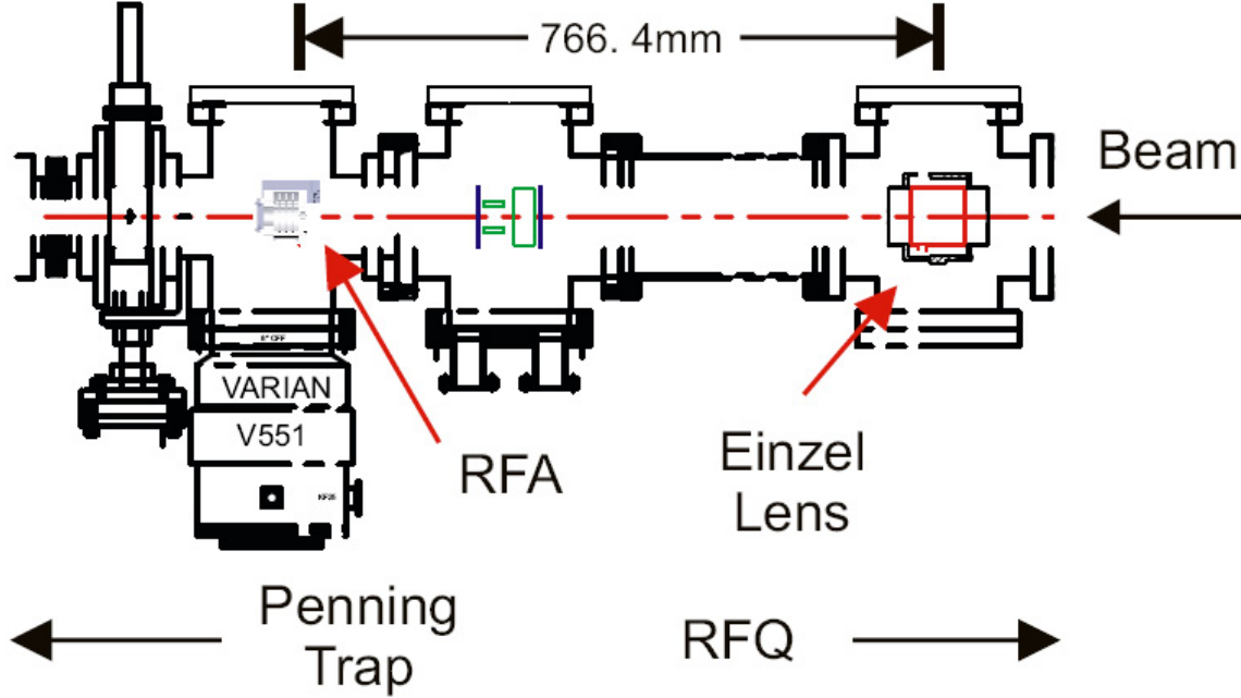
Figure 5–4: Section of TITAN beamline where the TITAN RFA was installed for experimental testing. The Einzel lens situated upstream from the RFA places an upper limit on the maximum beam divergence.
