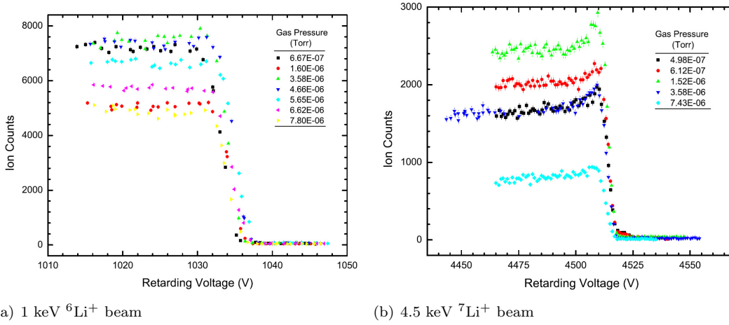
Figure 7–9: Ion counts plots for 1 keV {}^6\text{Li}^+ (left) and 4.5 keV {}^7\text{Li}^+ (right) ion beam under different RFQ buffer gas pressure as a function of the retarding voltage.
