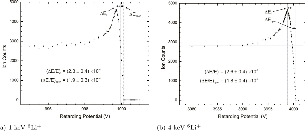
Figure 5-5: 635 wpi mesh simulation of the ion counts as a function of the retarding voltage for a monoenergetic {}^6\text{Li}^+ beam of (a) 1 keV and (b) 4 keV. The energy resolution errors introduced by the ion focusing ( \Delta E/E|_f ) and mesh openings ( \Delta E/E|_{open} ) are easily noticeable.
