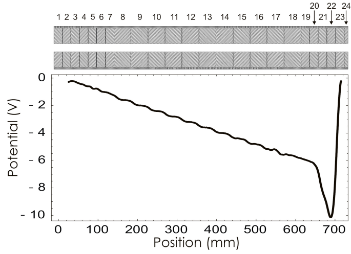
Figure 2-5: Top: Segmented electrodes of the RFQ as function of axial position. Bottom: Corresponding simulated RFQ longitudinal trapping potential. Taken from [41].
