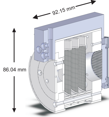
Figure 3–5: Section view of the TITAN RFA. The RFA has three meshes; a central retarding mesh and two outer meshes. The retarding mesh filters the longitudinal kinetic energy component of the incoming ions. The outer meshes provides two homogeneous electric field regions between them and the retarding mesh and minimizes secondary electrons, due to ion impacts on meshes and collector, from reaching the retarding mesh.
