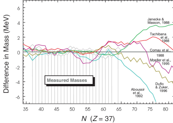
Figure 1–2: Mass difference between various theoretical models and experimental mass data obtained for rubidium isotopes. A modified ensemble averaging of the mass predictions from the theoretical models is used as the baseline [1]. Below N = 64 , the models are in good agreement with the experimental masses whereas for N > 64 , the models begin to diverge. Taken from [11]
