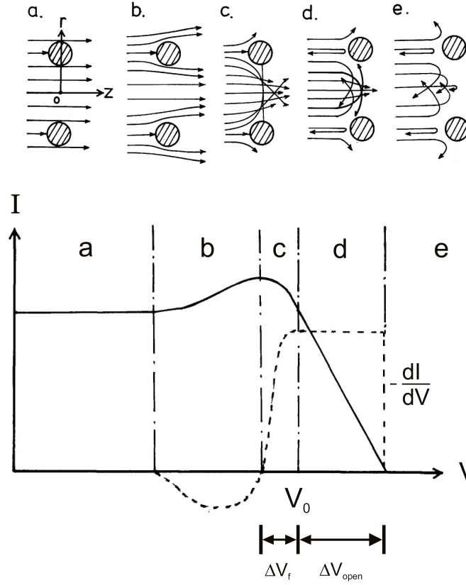
Figure 4-2: Top: Schematic views of ion trajectories with longitudinal kinetic energy qV_0 for different applied potential V on mesh. Bottom: Complementary plot of the current I as function of the applied voltage V on mesh with corresponding regions. a) V \ll V_0 : Ion trajectories are unaffected by the applied potential of the mesh. b) V < V_0 : Electrostatic ion focusing around wires of mesh starts to be noticeable as the radial component of the electric field increases. c) V \lesssim V_0 : Further focusing with increase deflections. d) V_0 < V < V_0 + \Delta V_{open} : Partial reflection of ions with decreasing equipotential surface V_0 within the mesh opening. e) V > V_0 + \Delta V_{open} : All ions are reflected. Taken from [63].
