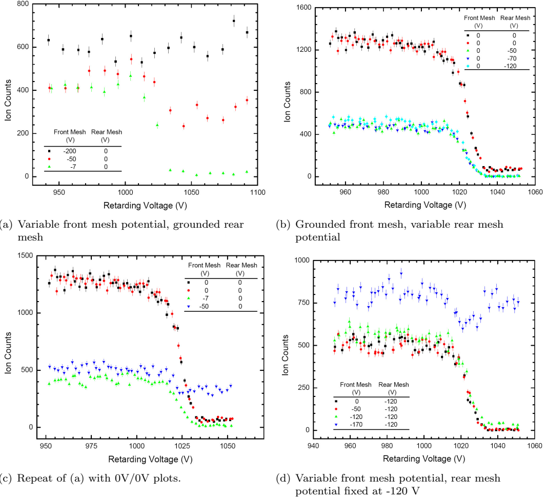
Figure 7-1: Ion counts for a 1 keV {}^6\text{Li}^+ beam under different outer meshes potentials as a function of the retarding voltage. (a) shows an increase in parasitic current as the front mesh potential is lowered. The 0V/0V plot is missing due to a software glitch which prevented saving the data. (b) Two runs using the 0V/0V configuration were taken with even and odd voltages respectively. The parasitic current is visible in both these runs for V_{\text{retard}} > 1036 V. The enhanced ion counts in both 0V/0V plots is due to the deactivation of the RFQ beamgate from 1 ms, leaving an unimpeded path for ions entering the RFQ from the TITAN ion source. (c) repeats the scans from (a) with smaller voltage steps. 0V/0V plots are the same as from (b). (d) shows the presence of the parasitic current occurring for front mesh potentials lower than the rear potential.
