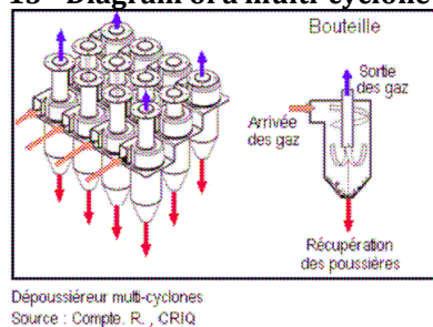
Figure 13 - Diagram of a multi-cyclone cleaner
