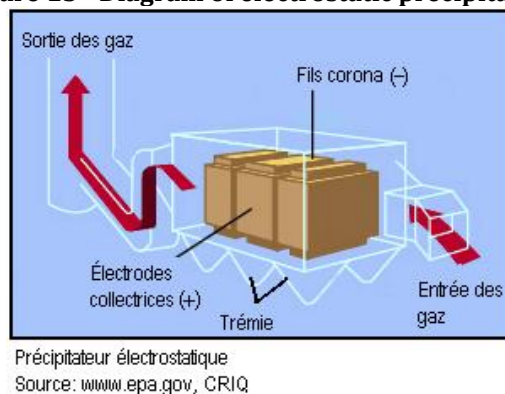
Figure 15 - Diagram of electrostatic precipitators
