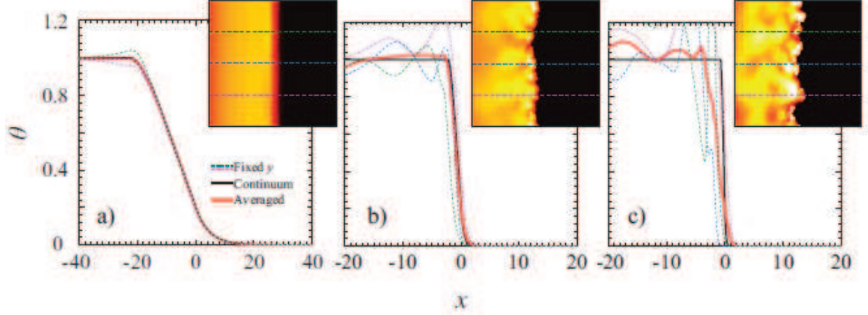
FIG. 3. Temperature profiles plotted against spatial coordinate in direction of flame propagation, i.e., \theta(x) , for ignition temperature \theta_{\text{ign}} = 0.2 and discreteness parameter (a) \tau_c = 100 , (b) \tau_c = 1 , (c) \tau_c = 0.1 . Corner inset: corresponding temperature contour plots. Thin dashed curves in temperature profile are extracted from corresponding lines shown on the temperature contours. Red line corresponds to width-averaged temperature profile, and black line corresponds to the analytic solution based on a continuum flame model.
