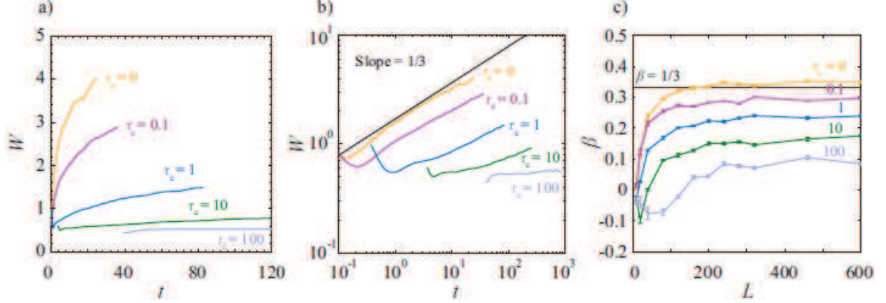
FIG. 4. Ensemble-averaged flame front roughness W as a function of time t for \theta_{\text{ign}} = 0.2 and \tau_c from 0 to 100 using (a) linear scales, and (b) logarithmic scales. Each curve is plotted for flame propagation in a 200 \times 200 domain (40000 discrete sources, beginning from the time at which at least 20 sources have been triggered). The measured \beta is plotted as a function of domain width L in (c). The reference line in (b) and (c) shows \beta = 1/3 . Error bars show the 95% confidence interval on the slope measurement.
