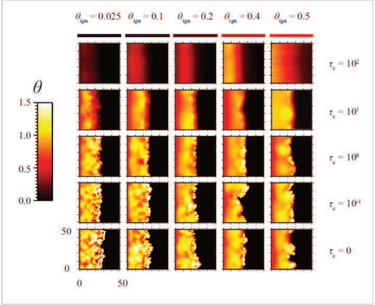
FIG. 2. Temperature fields of flames propagating rightward in systems of discrete sources. Average inter-source spacing is unity, and size of each plot window is chosen to be 50 \times 50 . Each system corresponds to a different set of nondimensional ignition temperature \theta_{\text{ign}} (increasing from left to right) and discreteness parameter \tau_c (increasing from bottom to top). The color bars above the top row correspond to the column's ignition temperature. The flame front is near the middle of each plot window.
