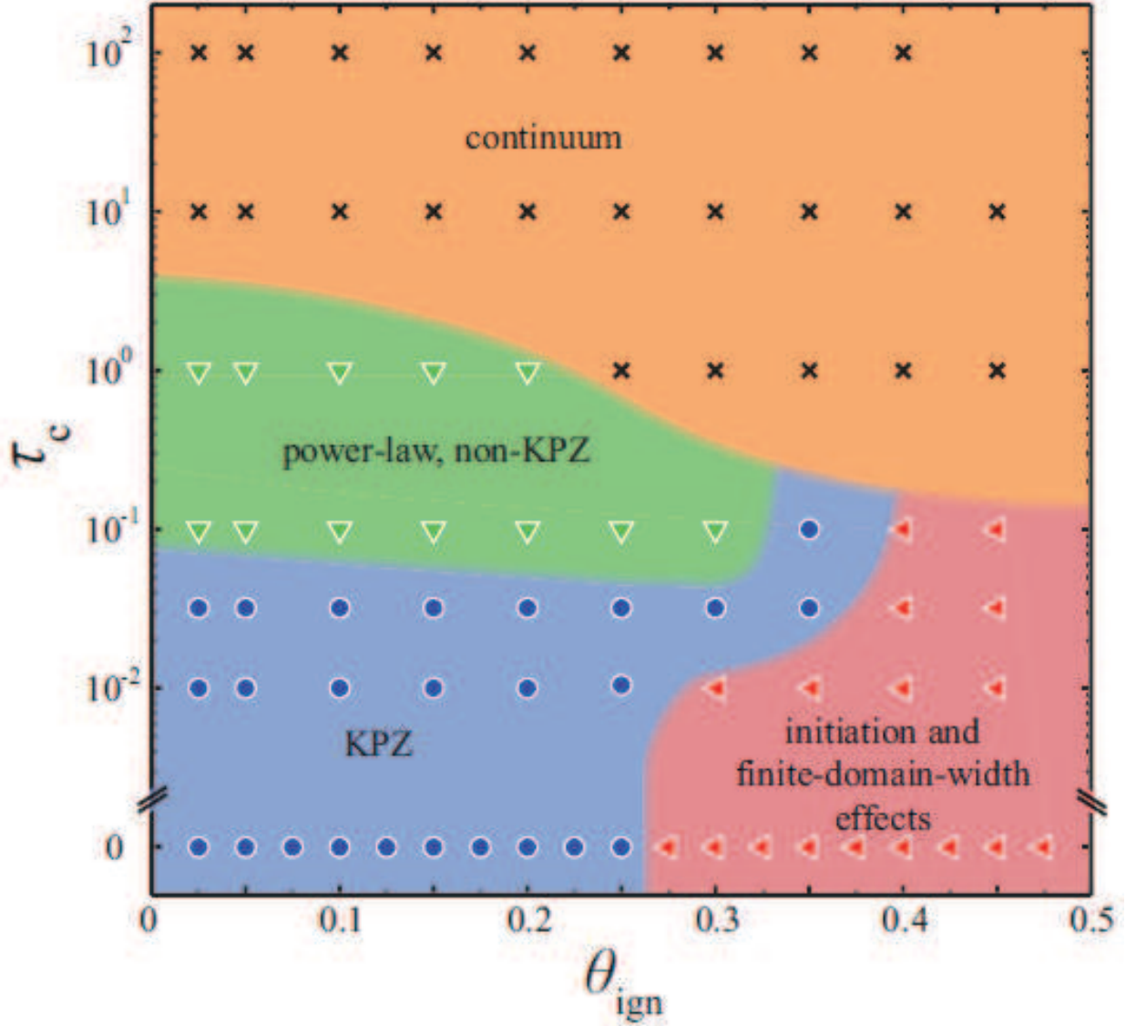
FIG. 6. Simulation results categorized according to the flame front roughening behavior and summarized as a map in \theta_{\text{ign}}\text{-}\tau_c parameter space. Each color-shaded region represents a category of front roughening behavior; each symbol represents an ensemble of simulations with a specific set of \theta_{\text{ign}} and \tau_c .
