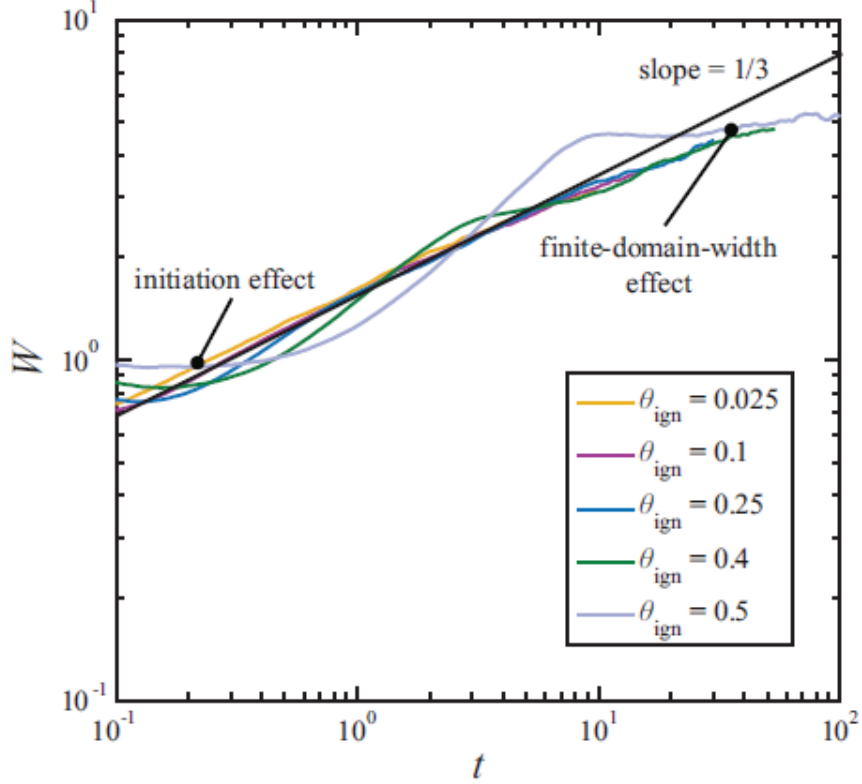
FIG. 5. Ensemble-averaged flame front roughness W as a function of time t for \tau_c = 0 and \theta_{\text{ign}} = 0.025 to 0.5 using logarithmic scales. Each curve is plotted for flame propagation in a 200 \times 200 domain (40000 discrete sources). The roughening behavior influenced by the initiation of the flame and the finite domain width are indicated on the curve of \theta_{\text{ign}} = 0.5 .
