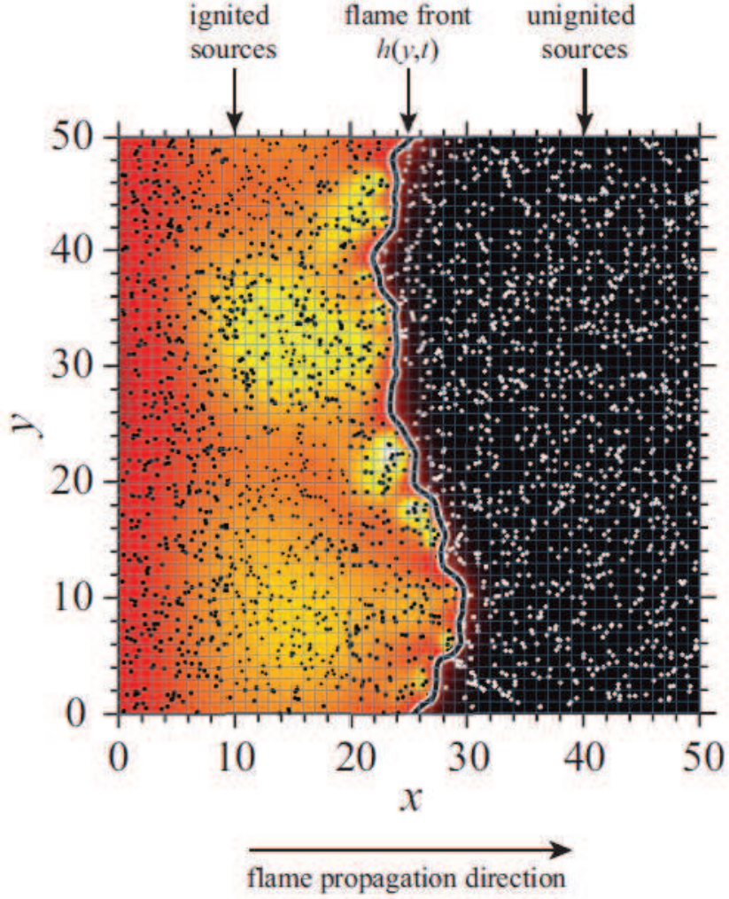
FIG. 1. Visualization of a small domain ( 50 \times 50 ) with \theta_{\text{ign}} = 0.5 , \tau_c = 1 , showing the color contours of temperature field, with the flame front (marked by the black-white line), and randomly distributed ignited (black dots) and unignited (white dots) sources. The uniform Cartesian grid over which the temperature field is calculated for front roughness measurement is illustrated as the blue lines.
