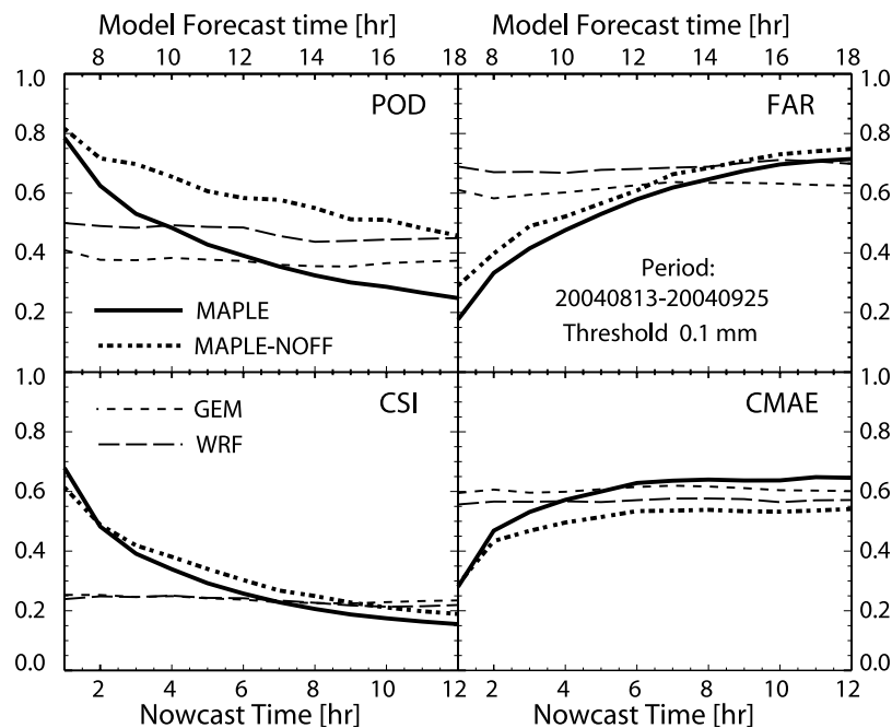
Figure 3. As in Figure 2 but for the second analysis period using two different models (long dashed for WRF and short dashed for GEM operational). The solid (MAPLE) and dotted (MAPLE-NOFF) curves correspond to two versions of 12-hour radar nowcasts; see text for description. The 12-hour forecast period is shown as the abscissa at the bottom, starting at t = 0 . The threshold for hourly precipitation is 0.1 mm.
