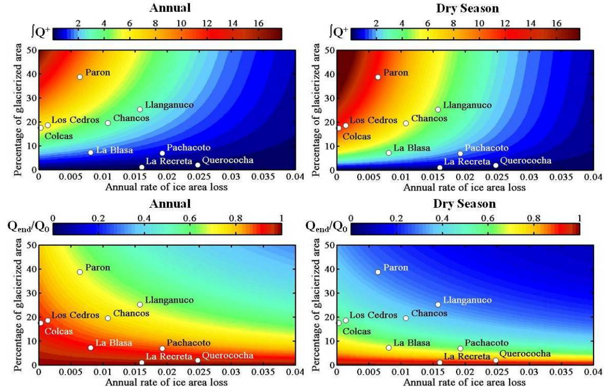
Figure 4.6. Variations of |Q^+ (top graphs) and Q_{end}/Q_0 (bottom graphs) for the “rapid retreat simulations”, as a function of percentage of glacierized area and the annual rate of ice area loss. Colors represent values of |Q^+ (indicator of the glaciers capacity to further increase the watershed flows) and of Q_{end}/Q_0 (starting and ending simulated discharge ratio). Full year simulations appear on the left and dry-season ones are reported at the right. All parameters are dimensionless.
