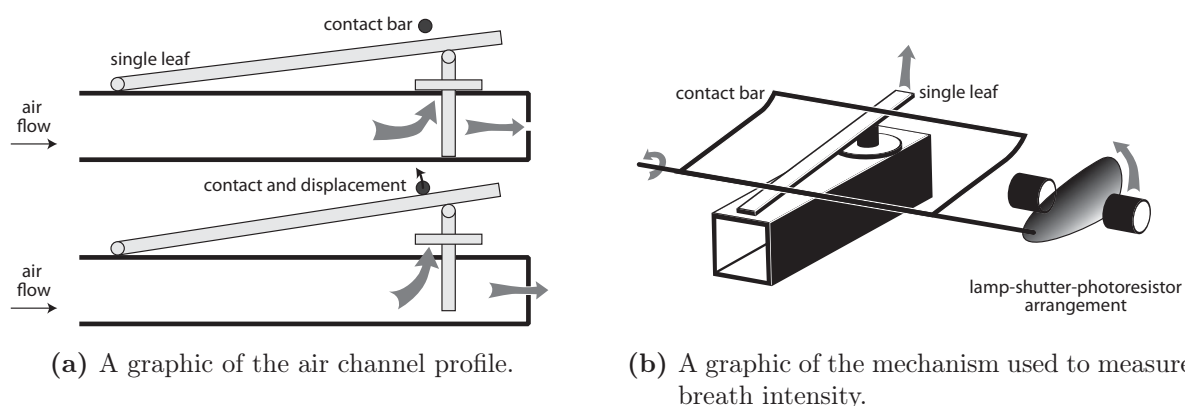
Fig. 3.1 – The mechanism to measure air pressure and note position as presented in Hillairet, Lecadre, and Wallace (1970).
