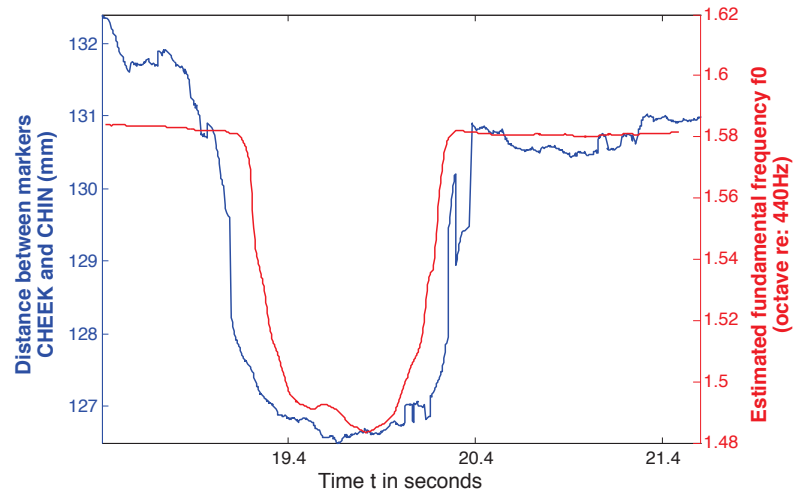
Fig. 4.2 – A graph displaying the cheek–chin distance and the estimate of fundamental frequency during a hole 8 blow bend to Eb and back.
