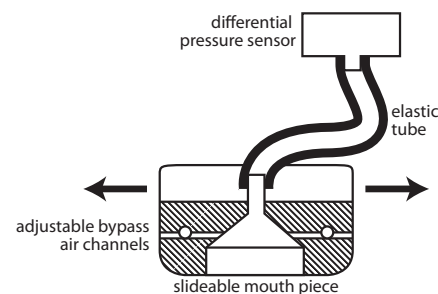
(b) A schematic of the slideable mouthpiece.
