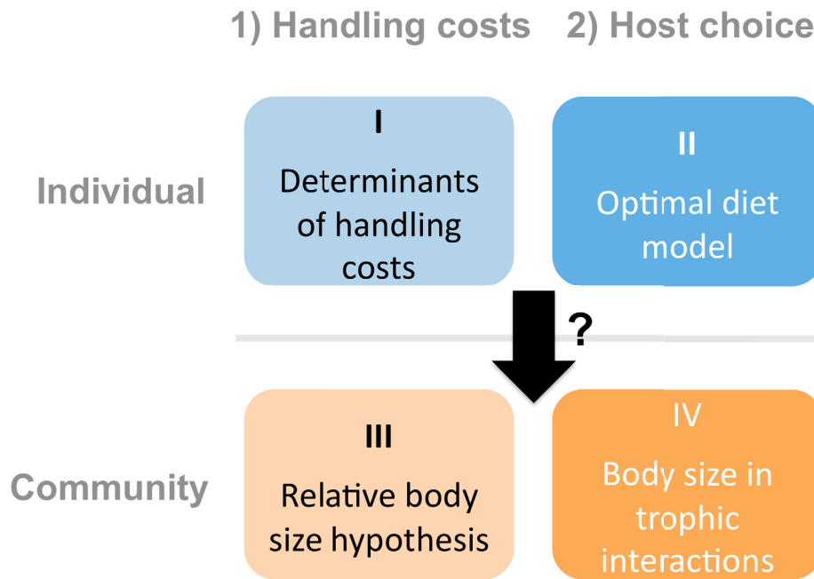
Figure 1.2.1 Diagram of the general questions addressed in this thesis. Questions about 1) determinants of handling costs and 2) host choice are addressed at the level of individuals (blue) and communities (orange). Collectively, they aim to explore the potential implications of individual foraging behaviour for higher levels of organisation, the community (black arrow).
