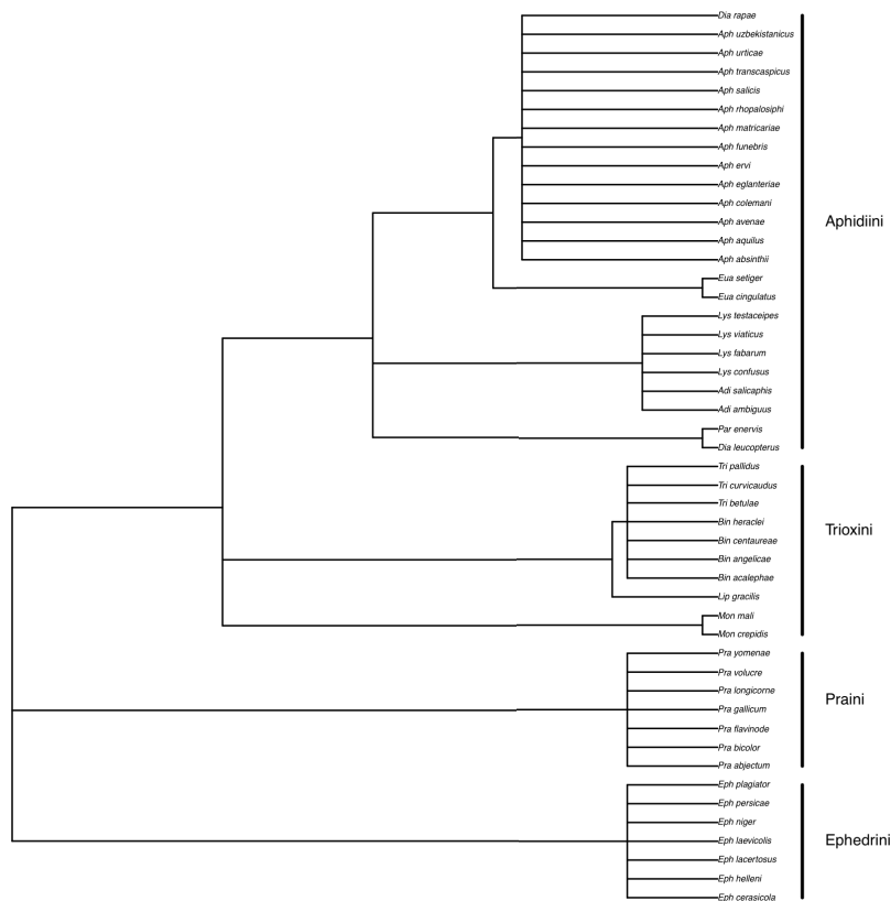
Figure 7.3.1 Topology of the phylogenetic trees for 166 species of aphids (a) and 48 species of parasitoids (b) included in analyses. High-resolution images of both phylogenies with species names are available on request.
