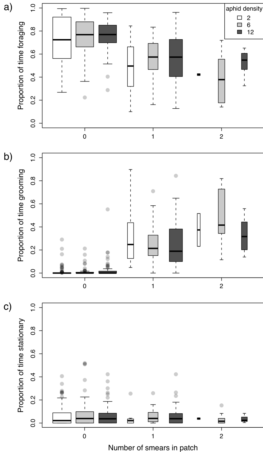
Figure 4.4.4 Parasitoid's time budget within patch visits against smearing frequency. Box plots show the proportion of time spent: a) foraging (searching & handling); b) grooming; and c) stationary in patches containing 2 (white), 6 (grey), and 12 (black) aphids.
