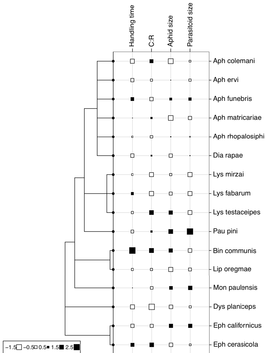
Figure 6.4.1 Trait averages for each parasitoid species plotted on the parasitoid cladogram used. Handling times are corrected for aphid instar; aphid and parasitoid size are log transformed body lengths. Traits were scaled and centred for illustrative purposes. There was no significant phylogenetic signal in any traits.
