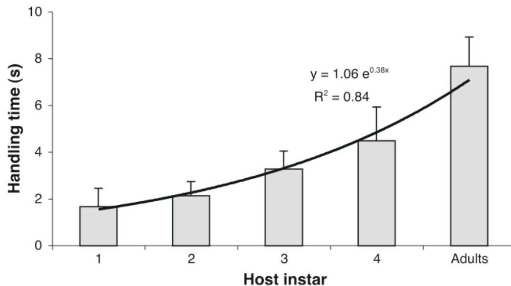
Figure 5.4.2 Influence of host instar on the handling time of A. colemani parasitizing M. persicae .
