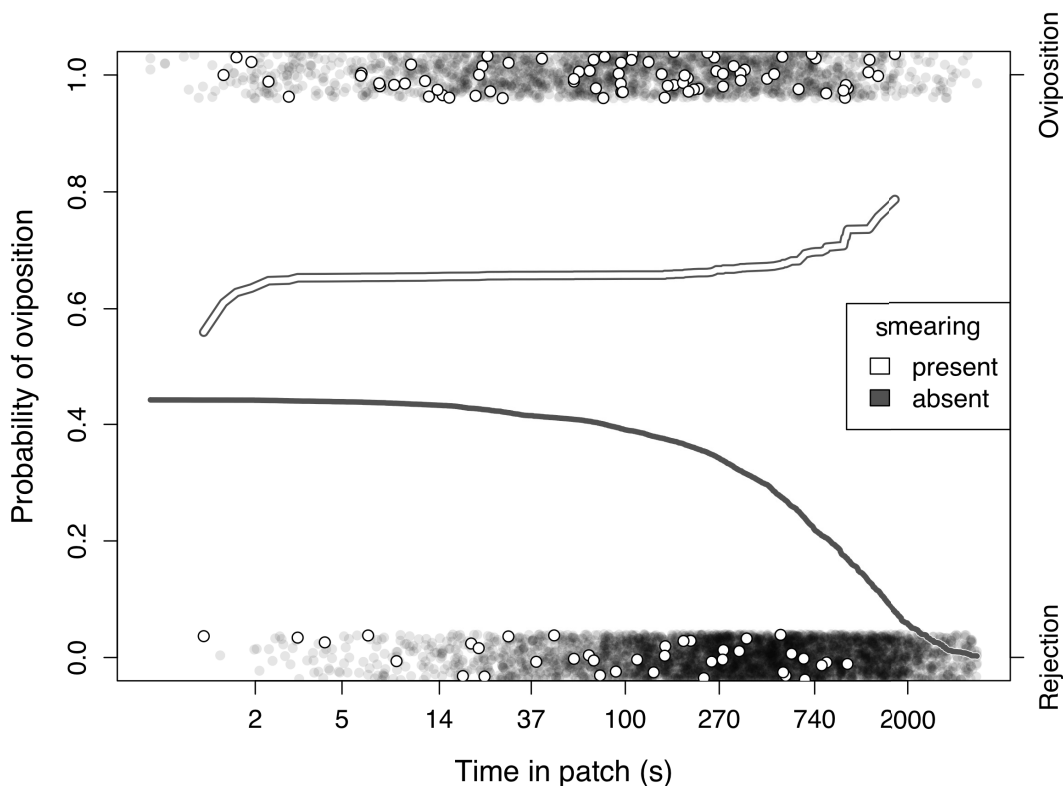
Figure 4.4.1 Encounters resulted in oviposition more frequently in the presence of smearing (white), than in its absence (grey). Lines show the fitted probabilities of oviposition and dots show the outcome of individual encounters (oviposition vs. rejection), as a function of the timing of events.
