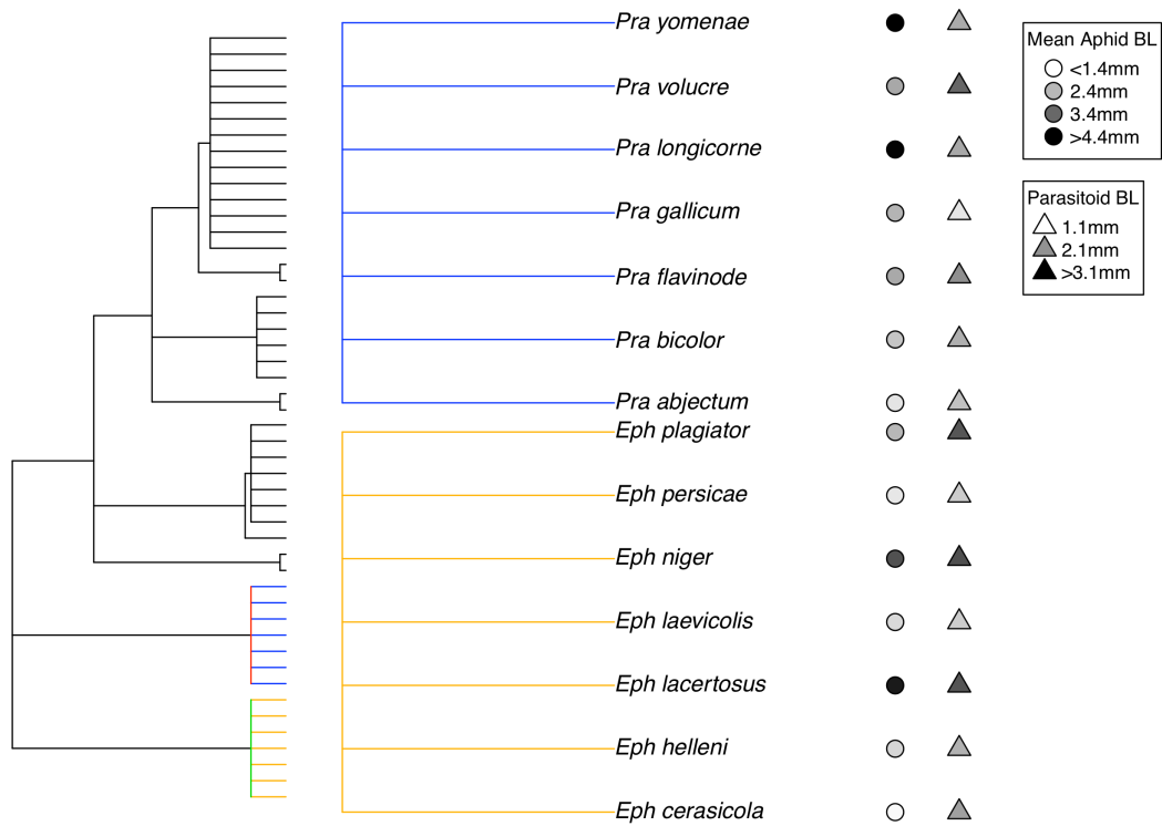
Figure 7.4.3 Phylogenetic patterns of aphid and parasitoid body sizes in feeding relationships. Body sizes of aphids (circles) and parasitoids (triangles) are shown for two clades of aphid and parasitoid phylogenies to illustrate the different phylogenetic patterns. Phylogenetic conservatism in aphid evolution (a): Closely related species of aphid share similar body sizes and are attacked by parasitoids of similar body sizes. Disruptive selection in parasitoid evolution (b): The body size of parasitoids and their respective hosts differ more within genera than between distant genera.
