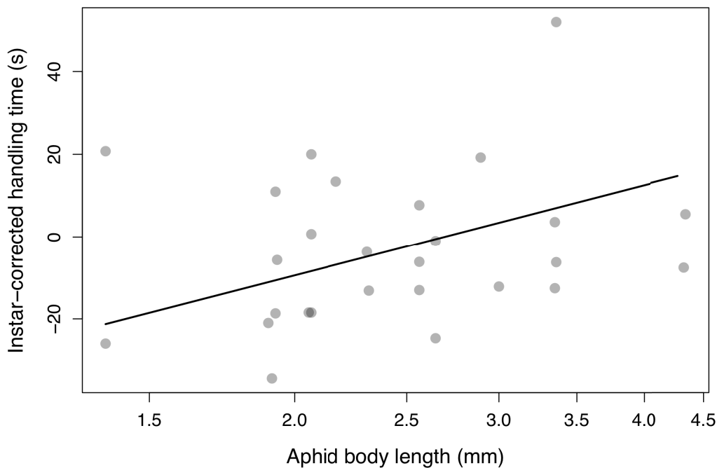
Figure 6.4.3 Aphid instar corrected handling time increased with aphid species body length (log scale) in individual aphid-parasitoid associations.
