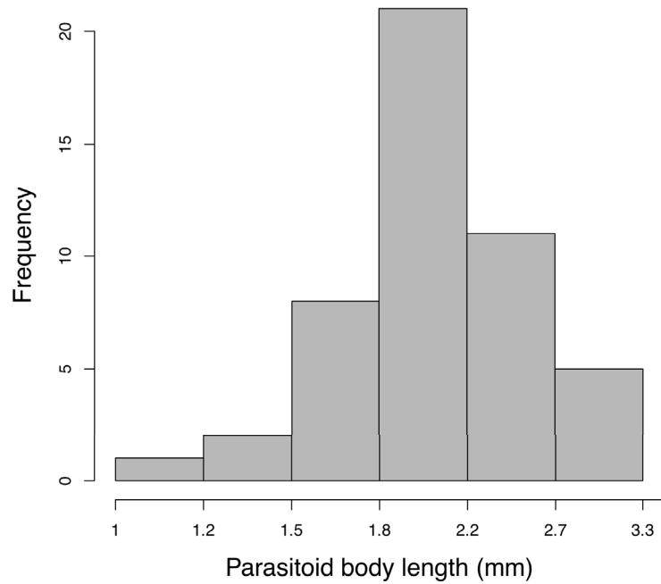
Figure 7.4.1 Frequency distributions of body lengths (log scale) for species of aphids (a) and parasitoids (b) included in the study.
