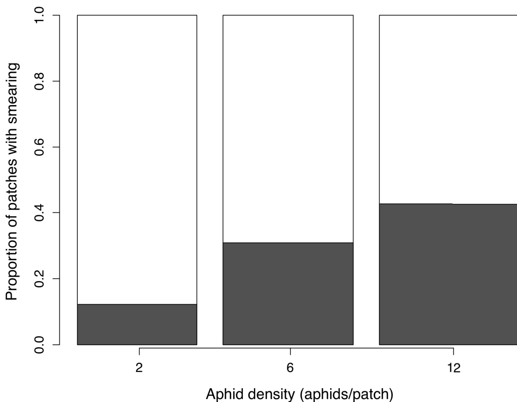
Figure 4.4.5 Occurrence of smearing in patch visits against aphid density. Dark area shows the proportion of patches in which the parasitoid was smeared. The widths of columns are proportional to the square root of sample sizes.
