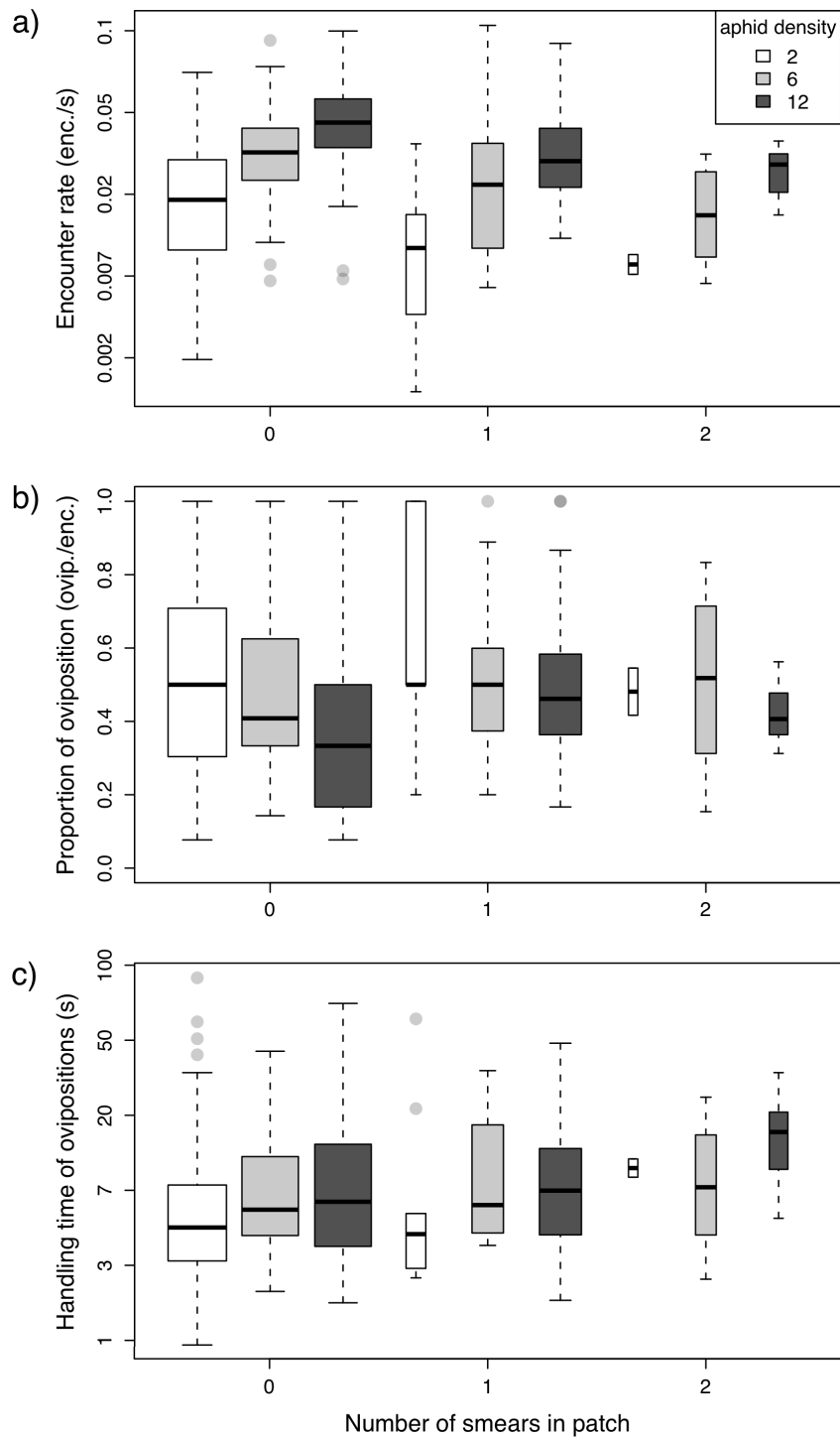
Figure 4.4.3 Components of the parasitoids' foraging success within patch visits against smearing frequency. Box plots show the distributions of: a) encounter rate; b) outcome of encounters; and c) handling time of ovipositions for patches containing 2 (white), 6 (grey), and 12 (black) aphids. Encounter rate (a) and handling time (c) are plotted on a log scale.
