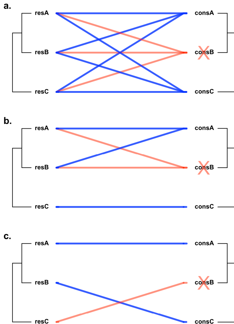
Figure 8.3.1 Trophic interactions between hypothetical resource (left) and consumer species (right) represented by connecting lines. Red lines show interactions that would cease if consumer B (consB) became extinct. When there is: a) no phylogenetic constraint, other consumers (consA, consC) can exploit resources freed; b) phylogenetic conservatism, closely related consumers (consA) can exploit freed resource; and c) disruptive selection, resource freed cannot be exploited by closely related consumers (consA).
