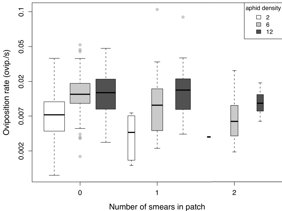
Figure 4.4.2 Parasitoid oviposition rate against smearing frequency in patches. Box plots show the distribution of oviposition rates for patches containing 2 (white), 6 (grey), and 12 (black) aphids. Boxes show the interquartile range (50% of observations), in which the horizontal bar is the median. Whiskers extend 1.5 times the interquartile range beyond the median. Dots show individual observations lying outside this interval. Box widths are proportional to the square root of sample sizes.
