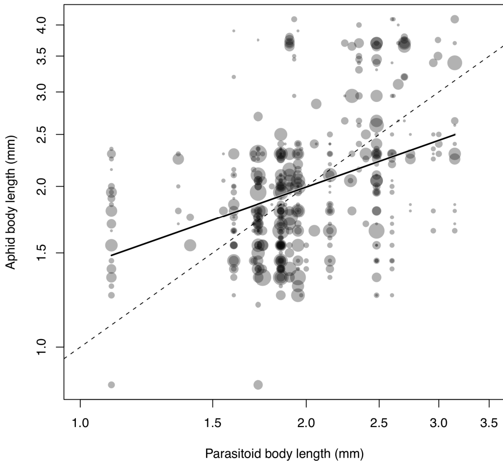
Figure 7.4.2 Relationship between aphid parasitoid size and host size use in feeding relationships (log-log scale). The solid line shows the fitted least squares linear regression (slope=0.49) and the dashed line shows the relationship for equal aphid and parasitoid body sizes (slope=1).
