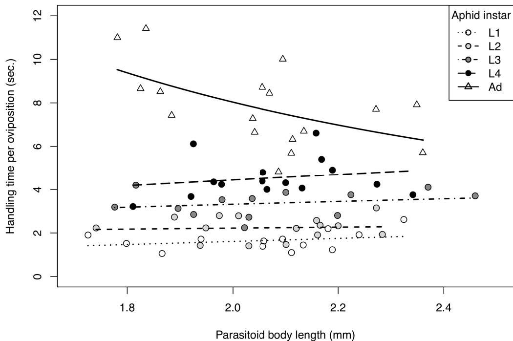
Figure 3.4.1 Handling time of Aphidius colemani as a function of parasitoid body length and instar of Myzus persicae . Handling time ( T_h ) decreased significantly with increasing parasitoid body length (BL) for adult aphids only ( T_h = 22.29 \times BL^{-1.472} ).
