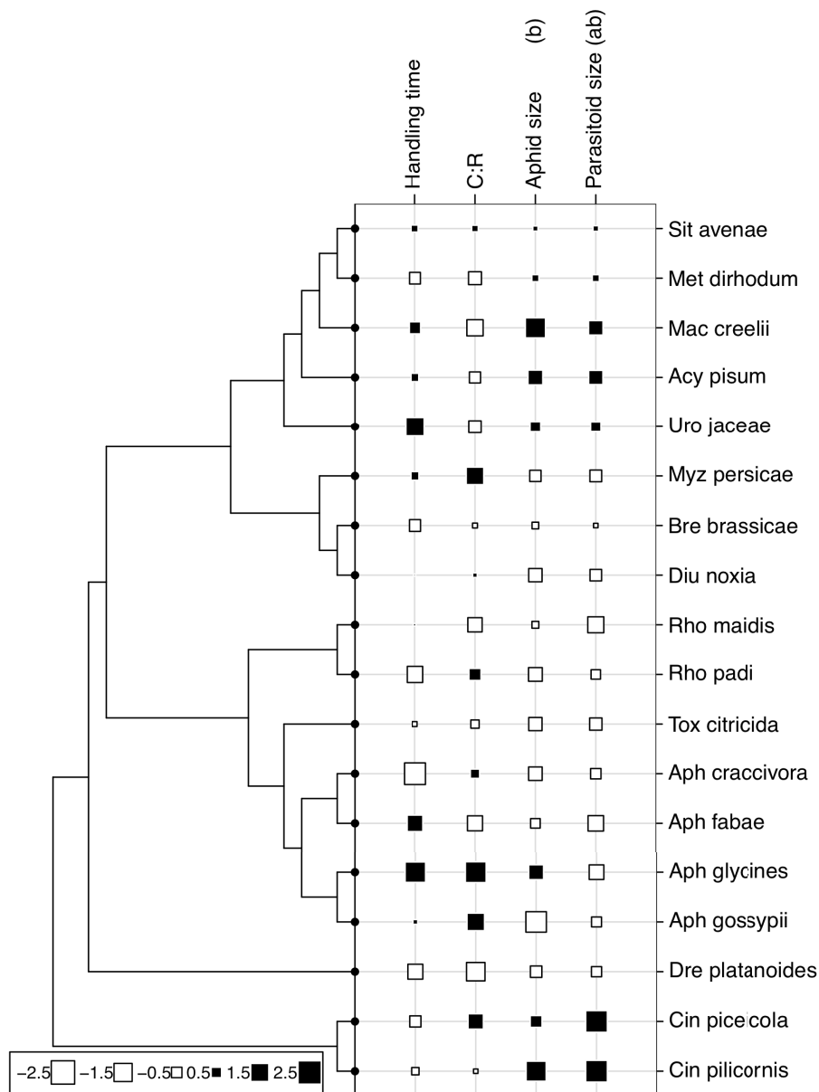
Figure 6.4.2 Trait averages for each aphid species plotted on the aphid cladogram used. Handling times shown are corrected for aphid instar; aphid and parasitoid size are log transformed body lengths. Traits were scaled and centred for illustrative purposes. Letters in brackets denote traits with significant phylogenetic signal using (a) Abouheif's test for serial independence and (b) Blomberg's K statistic.
