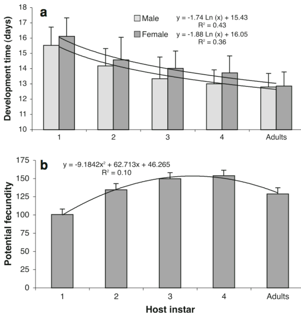
Figure 5.4.1 Influence of host instar on development time (a) and fecundity (b) of Aphidius colemani parasitizing Myzus persicae .
