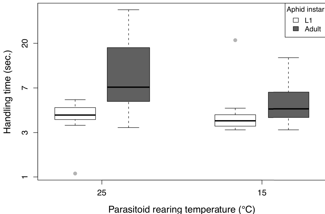
Figure 3.4.2 Handling time (log scale) of Aphidius colemani as a function rearing temperature and instar of its host, Myzus persicae . Boxes show the interquartile range, in which the horizontal line indicates the median. Vertical bars extend to 1.5 the upper and lower interquartile range, beyond which data are usually considered outliers (dots); removing these two points did not change the significance of the results.
