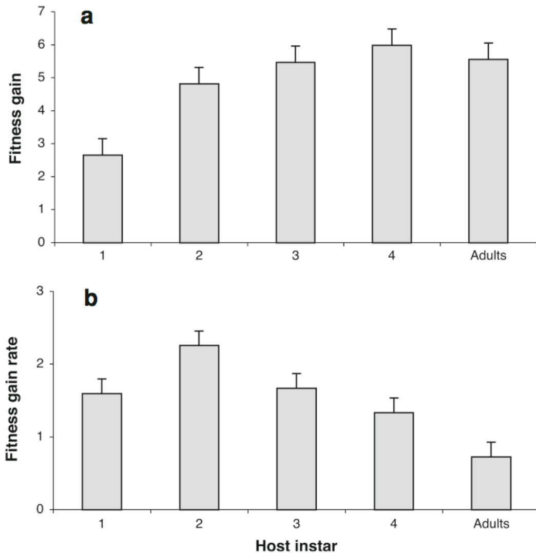
Figure 5.4.3 Host profitability as a function of host instar in A. colemani parasitizing M. persicae . Fitness gain per host estimated with life-history traits measurement (a); and fitness gain rate estimated with life-history traits measurement and handling time (b).
