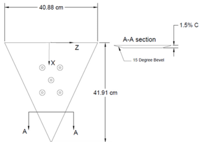
Figure 12 Reverse delta wing model
