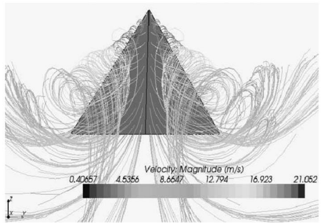
Figure 11 CFD simulation done by Altaf et al. [3]
