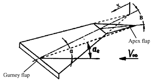
Figure 10 DW with GF and drooping apex [36]
