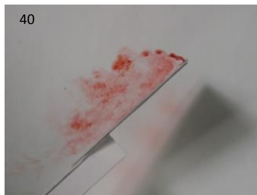
Figure 26 Dye flow visualization (middle injection) of RDW at \alpha = 10^\circ - 40^\circ
