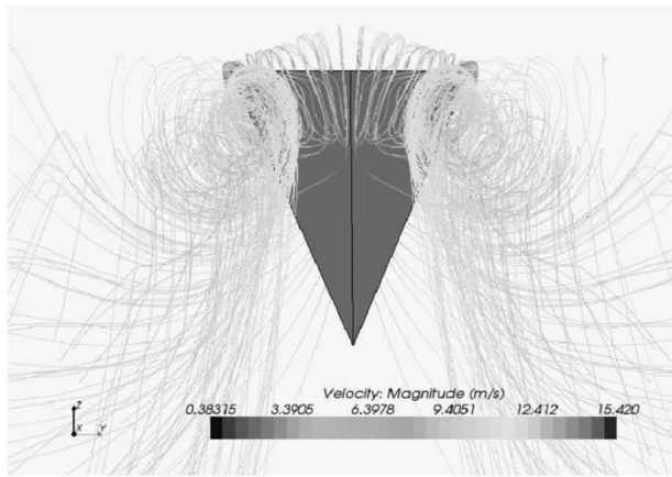
Figure 11 CFD simulation done by Altaf et al. [3]
