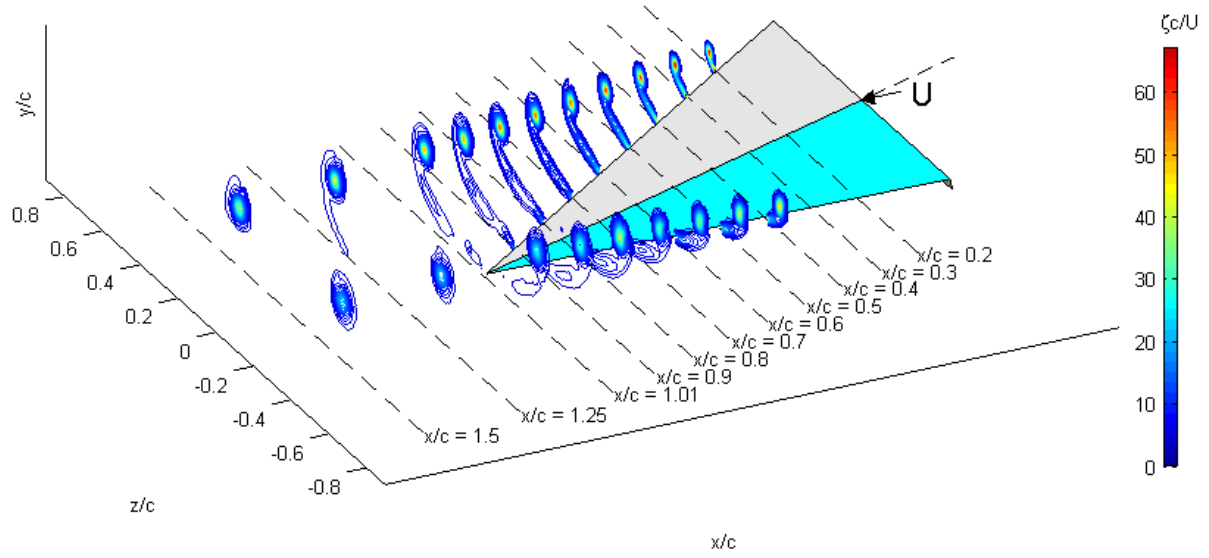
Figure 39 Iso-vorticity contour of 3% c LES in direct comparison of a BW
