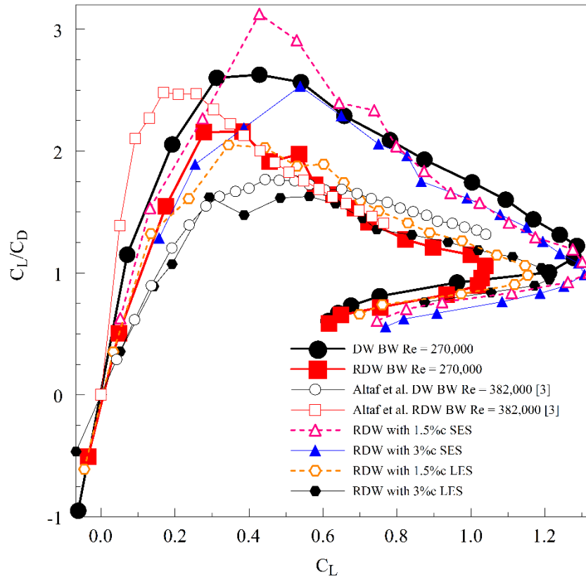
Figure 23 L/D verses lift coefficient for different wing configurations
