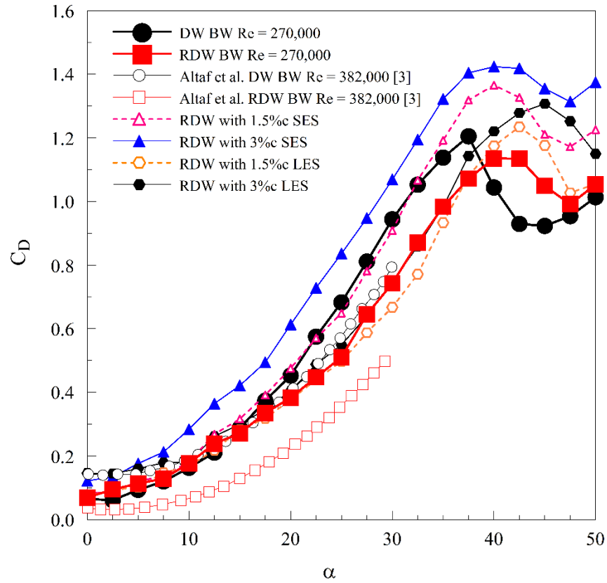
Figure 22 Drag coefficient verses angle of attack for different wing configurations
