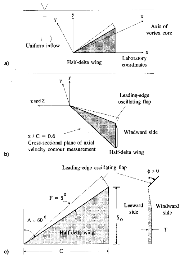
Figure 4 Leading-edge vortex flap (LEV) [25]
