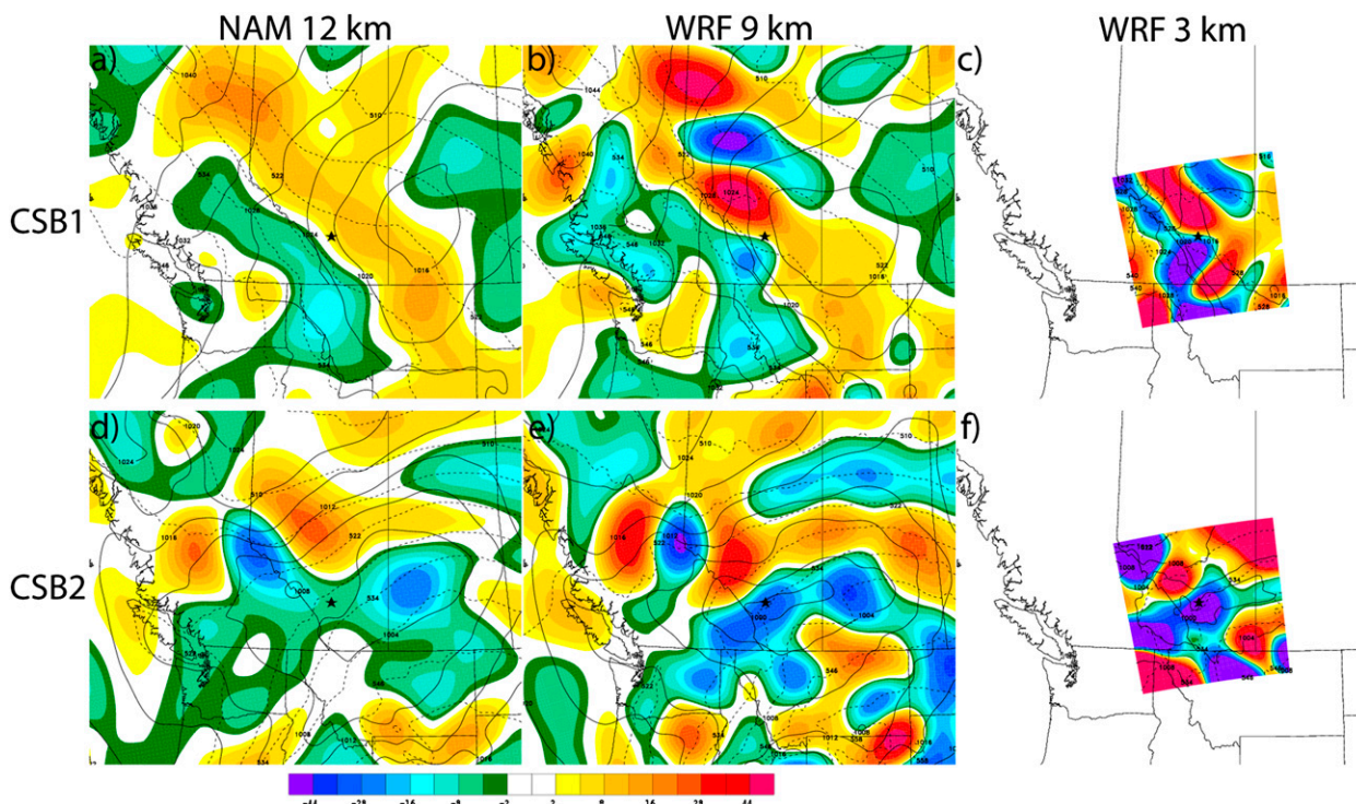
FIG. 14. As in Fig. 13, but for sea level pressure (hPa; solid contours), 1000–500-hPa thickness (dam; dashed contours), and 850–250-hPa layer-averaged \mathbf{Q} -vector divergence ( \times 10^{-18} \text{ K m}^{-2} \text{ s}^{-1} ; shaded cool colors for convergence, warm colors for divergence). The approximate location of CYYC is marked with a black star.
