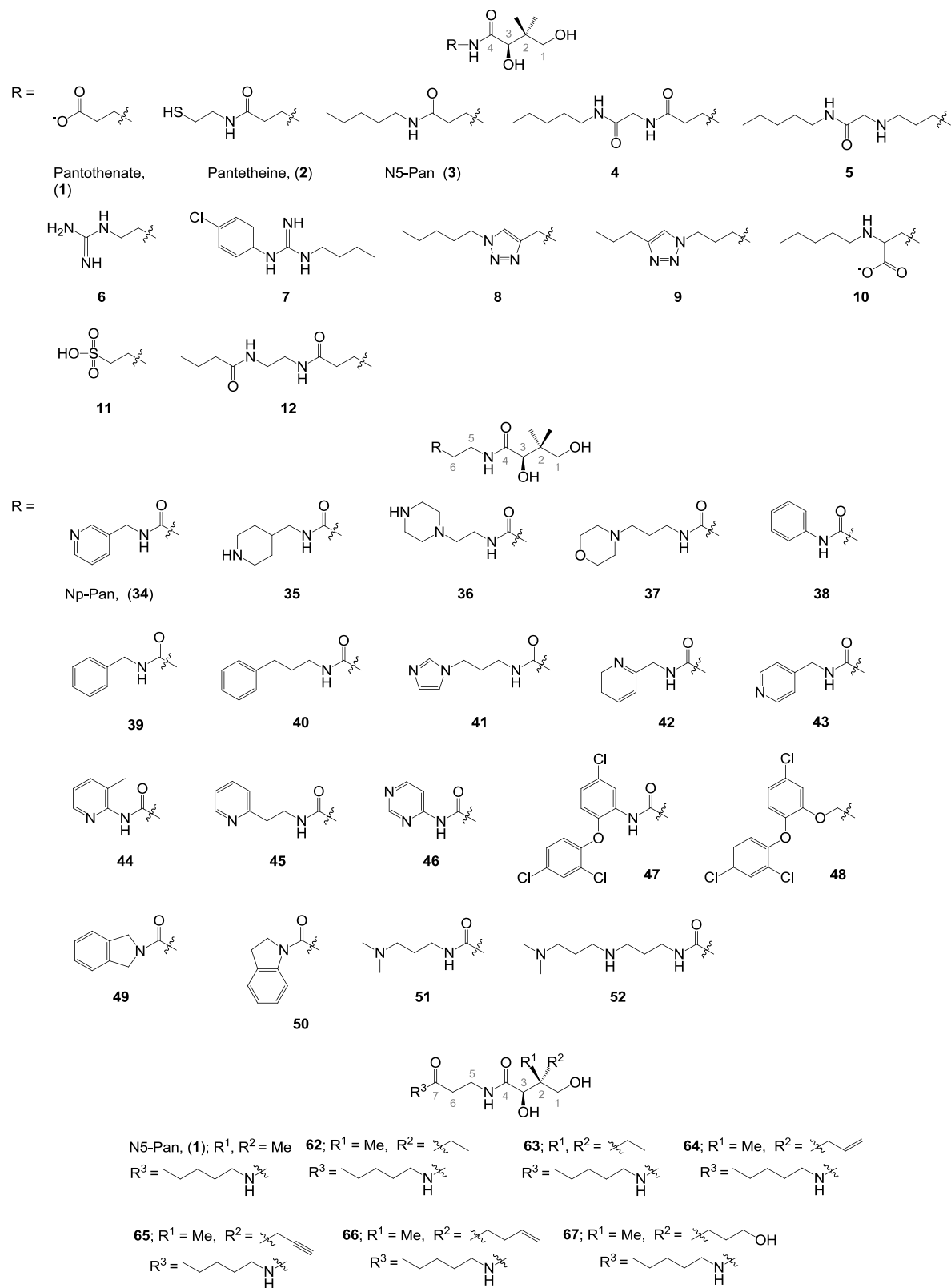
Figure 2. Pantothenate analogues described in this work.
