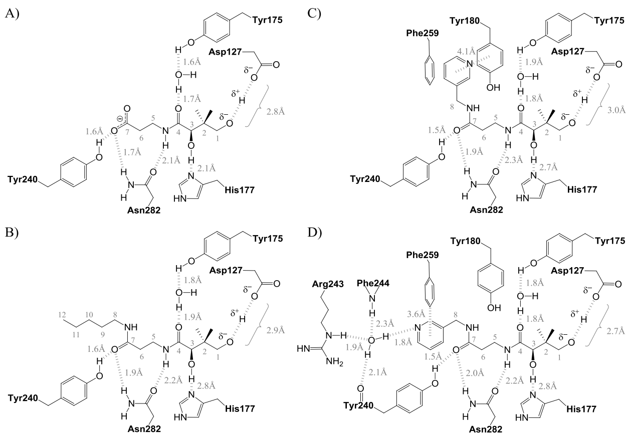
Figure 3. Highlight of the conserved active site residues involved in substrate binding; A) EcPanK (PDB 1SQ5) in complex with pantothenate ( 1 ); B) KpPanK (PDB 4F7W) in complex with 3 ; C) KpPanK (PDB 4GI7) in complex with 34 (yellow) and in a conformation where sandwich \pi - \pi stacking interactions form with Tyr180, or D) KpPanK (PDB 4GI7) in complex with 34 (turquoise) in a conformation where T-shaped \pi - \pi interactions form with Phe259 and water-mediated hydrogen bonding between the pyridyl nitrogen and Arg243, Phe244, and Tyr240.
