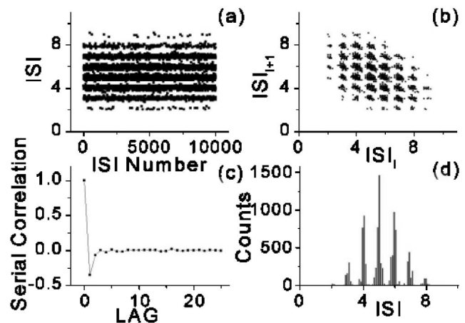
FIG. 1. Analysis of 10000 consecutive interspike intervals from a P -unit of the weakly electric fish A. leptorhynchus (data courtesy of Mark Nelson, Beckmann Institute, Illinois, USA; we focus on such “nonbursty” units). Time is in EOD cycles; the EOD frequency is 755 Hz. The firing rate is 145 Hz which corresponds to P = 0.192 . (a) Raster plot of ISI duration versus ISI number, (b) return map, (c) serial correlation, and (d) histogram.
