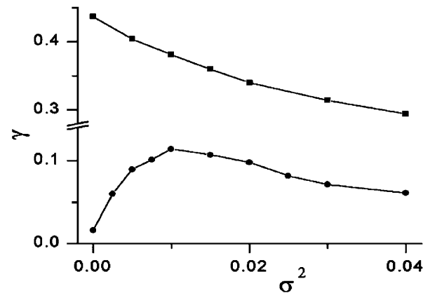
FIG. 4. Coding fraction \gamma vs synaptic noise variance \sigma^2 on a small plateau (5:1, upper curve) and a large plateau (2:1, lower curve) of Fig. 3. The AFM signal S(t) is a lowpass-filtered Gaussian noise of variance \sigma_{\text{sig}}^2 (fourth-order pole with cutoff frequency f_c equal to one-tenth of the EOD frequency [6]). This signal modulates the amplitude of the carrier, i.e., A(t) = A[1 + \xi(t) + S(t)] . An optimal Wiener filter h(t) was obtained [6] by minimizing the mean square error \epsilon = [\int_{-f_c}^{f_c} S_{nn}(f) df]^{1/2} , where S_{nn}(f) is the power spectrum of n(t) = S(t) - S_{\text{est}}(t) ; here S_{\text{est}}(t) is an estimated signal resulting from the convolution of the spike train with h(t) . The coding fraction is \gamma = 1 - \epsilon/\sigma_{\text{sig}} , the quality of encoding being best for \gamma = 1 . The signal variances were 0.15 (5:1) and 0.04 (2:1), yielding lower values of \gamma for the latter case. Parameters other than \sigma are the same as in Fig. 2, except for A = 1.38 mV in the 2:1 case and D = 0 in both cases.
