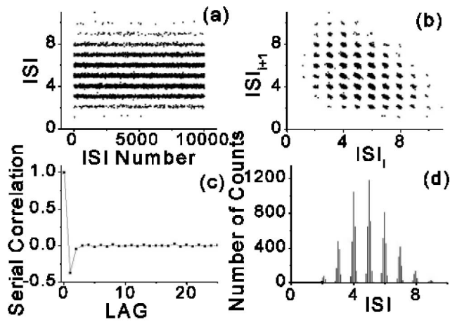
FIG. 2. Analysis of 10000 ISI's generated by the model of Eq. (4). Time is in EOD cycles. (a) Raster plot, (b) return map, (c) serial correlation, and (d) histogram. Parameters are: f = 1000 Hz, T_r = 1 ms, A = 0.3 mV, \gamma = 0.87 , w_0 = 0.03 mV, \Delta w = 0.05 mV, \tau_v = 1 ms, \tau_w = 7.75 ms, \sigma^2 = 0.0256 , \tau_\eta = 0.075 ms, and D = 1.758 \times 10^{-4} .
