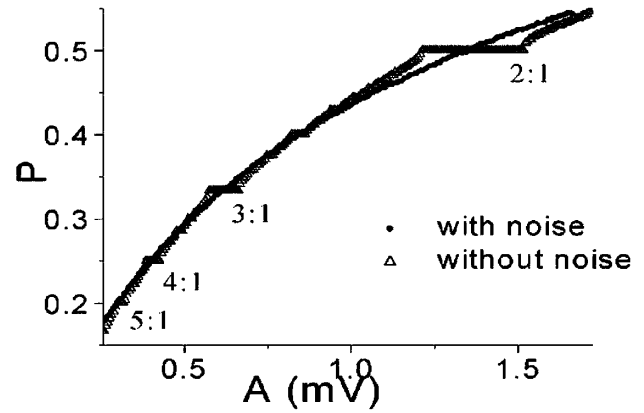
FIG. 3. Mean frequency of firing versus amplitude of the forcing in Eq. (4), without (hollow) and with (solid) P -unit noise. A devil's staircase structure is seen in the noiseless case; steps are "rounded" by noise. Each value is obtained from the mean firing rate of a 500 ms simulation.
