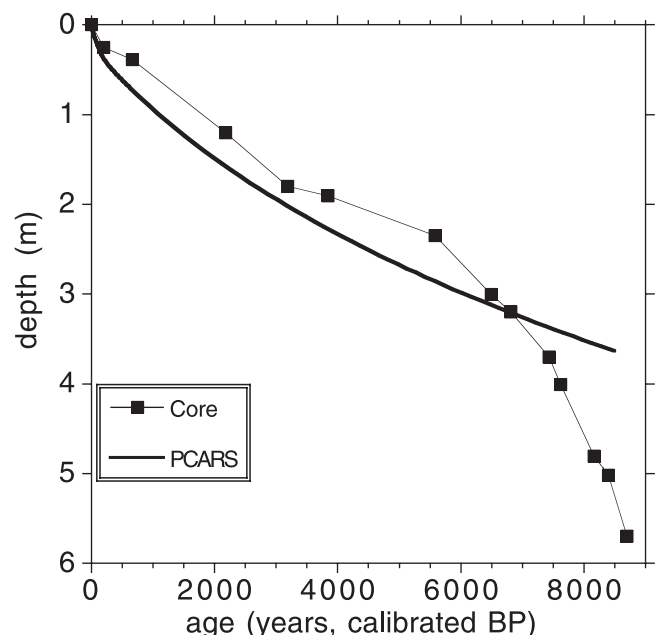
Figure 5. Age-depth profile for peat at Mer Bleue Bog in vicinity of eddy covariance tower and as simulated by PCARS. Solid line is PCARS peat profile initiation, and points are ^{14}\text{C} ages (see Frolking et al. [2001] for details). Model thus has a 3.6-m peat profile, with \sim 8500 annual peat layers; each layer has an initial mass and decomposability (see equation (8)). PCARS uses these to calculate instantaneous decomposition of each layer and then aggregates profile to calculate total decomposition, one component of site carbon balance.
