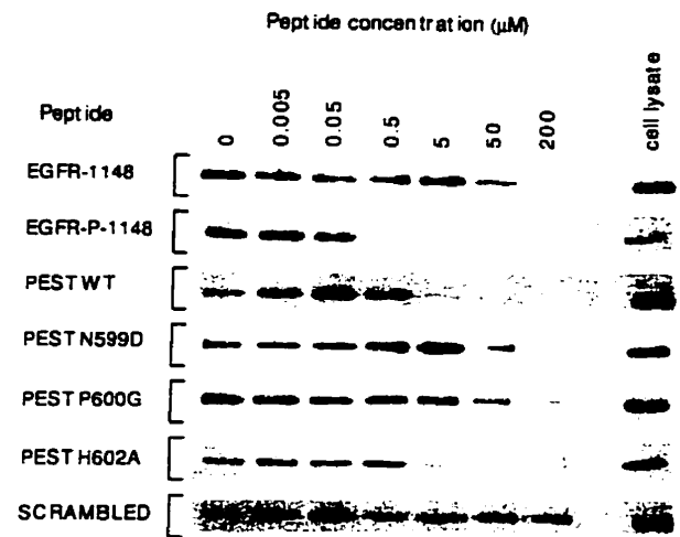
FIG. 5. Competition by peptides for HA-MPTP-PEST binding to the PTB/PI domain of SHC. 200 \mu g of total cell lysate from COS-1 cells transiently expressing HA-MPTP-PEST proteins were incubated with 100 ng of GST-SHC-1-209 fusion protein in the presence of the indicated concentrations of peptides (see "Materials and Methods"). The noncompeted, bound HA-MPTP-PEST was visualized by Western blot analysis using the anti-HA tag antibody 12CA5. The blots were then stripped and reprobed with an anti-GST antibody to assess loading (data not shown). The amino acid sequences of the synthetic peptides are as follows: EGFR-1148, 1140 QISLDNPDYQQDF 1152 ; EGFR-P-1148, 1140 QISLDNPDYQQDF 1152 ; PEST-WT, 594 PLSFTNPLHSDDWH 607 ; and Scrambled, DPSTHSHPLWLNFD. The results shown are representative of at least three independent experiments.
