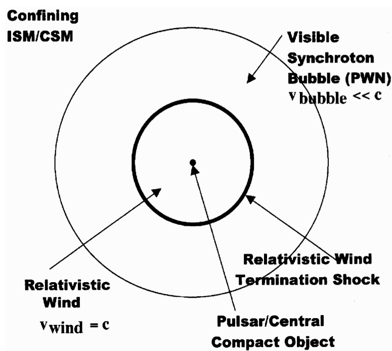
Figure 6.3: Schemataic of a PWN. Image credit — Fig. 2 from [27].
