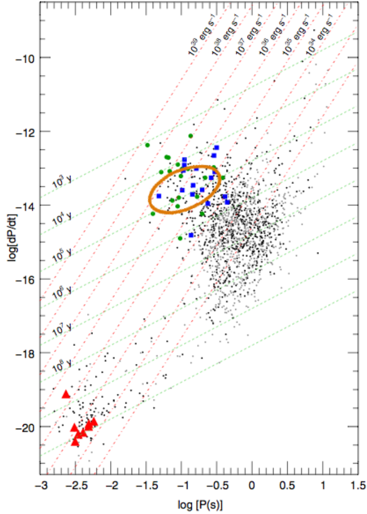
Figure B.1: The P - \dot{P} diagram from the First Fermi Pulsar Catalog with the approximate region indicated (orange ellipse) where a hypothetical young pulsar powering VHE emission near Terzan 5 would be situated. Image credit — adapted from Fig. 2 of [4].
