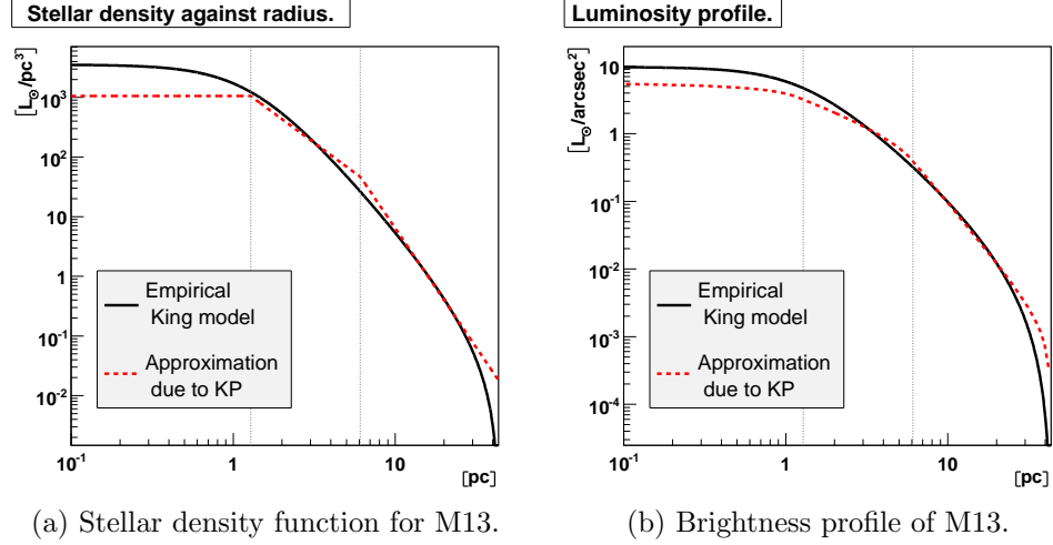
Figure 2.10: The approximation of the stellar density function due to Kuranov & Postnov [139], (a), is uniform within the core radius (left-hand vertical grey line) and a pair of power laws of differing slope outside that. The power-law break is at the half-mass radius (right-hand vertical grey line) and the model ends at the tidal radius (the upper limit of the horizontal axis): beyond this the stellar density for the cluster is zero. Meanwhile, the empirical King model, (b), is an excellent representation of the observed distribution of stars in M13 as projected onto the plane of the sky, (see Fig. 11 of [126]): here the model is calibrated using parameters from the Harris catalogue (2010 version) [95]. The empirical King model may be converted to a stellar density function using integration by parts, which yields Eq. 27 of [126]. This is plotted in (a) where it is clear that the approximation of [139] underestimates the stellar density in the core of the cluster. Conversely, the approximation for the stellar density may be projected onto the plane of the sky ( e.g. see Eq. 23 of [127]) as a luminosity/brightness profile: the underestimate of the stellar density in the inner regions of the cluster leads to a deficit by a factor of almost two in the surface brightness in the core of the cluster. For both the empirical King model and the approximation, the volume integral out to the tidal radius is within 10% of the cluster’s total luminosity.
