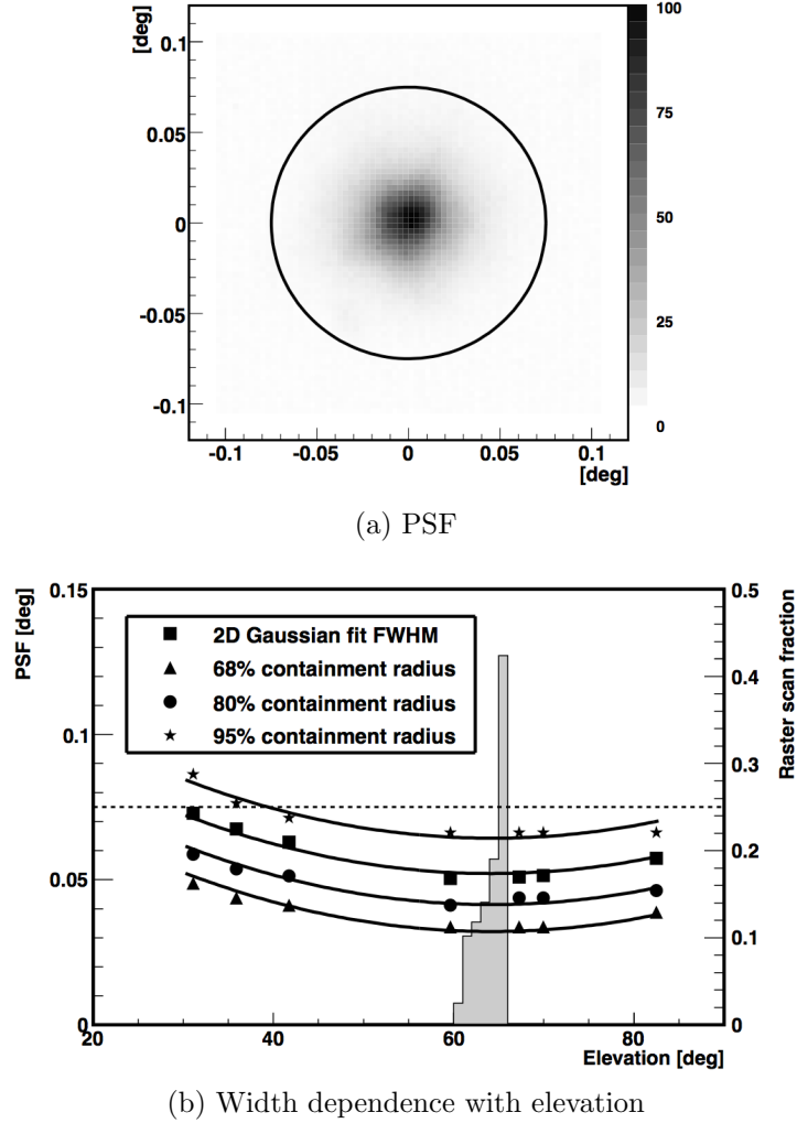
Figure 3.8: The on-axis PSF due to a bright star, from [157]. An image of the smallest PSF is shown in (a). The intensity values (grey scale) are plotted in arbitrary units. A PSF image is made by mounting a white screen at a telescope’s focal plane and photographing, (with a digital camera mounted on the OSS) the image formed by the telescope of a bright star being tracked by it. The dependence of the size of the on-axis PSF with elevation is shown in (b): the histogram indicates the number of raster-scan images taken at each elevation. The angular size of a single PMT pixel (see §3.2.2) is indicated by a circle in (a) and a dashed horizontal line in (b). Image credit — Fig. 6(b) and Fig. 7 from [157].
