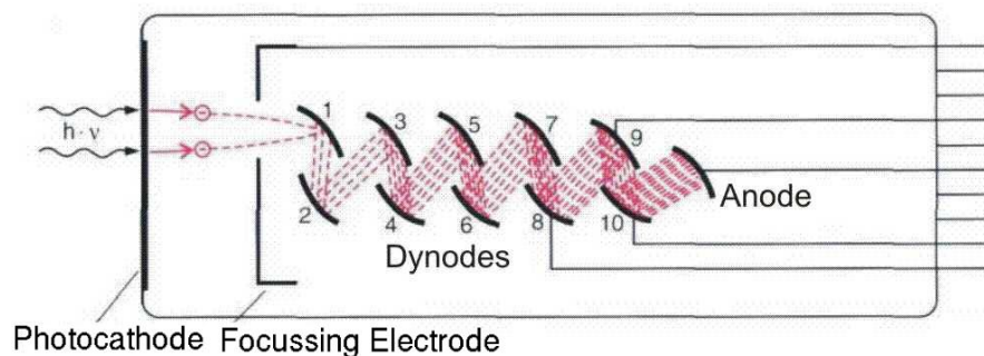
Figure 3.4: Schematic of the operation of a photo-multiplier tube. Electrons emitted at the cathode through the photoelectric effect cascade through the dynode chain to be absorbed at the anode, generating a current pulse.
