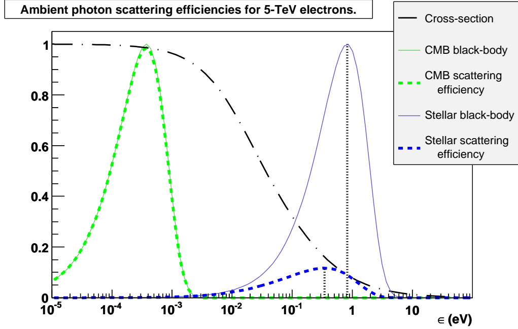
Figure 2.7: The effect of Klein-Nishina suppression on the scattering efficiency of 5 -TeV electrons from the CMB and from stellar photons. The black-body distributions due to the CMB (green, left) and stellar radiation (blue, right) at 6000 K are indicated by thin, solid lines. In both cases the distributions have been normalised for the peak to reach 1. The Klein-Nishina scattering cross-section, as a fraction of the Thomson cross-section, is the black dot-dashed line. The product of each black-body spectrum with the scattering cross-section is indicated by thick dashed lines: these curves demonstrate the efficiency with which black-body photons are scattered by 5 -TeV electrons. The CMB spectrum is scattered with nearly uniform efficiency in the Thomson limit of IC scattering: the distribution of photons that are scattered is not distorted with respect to the original black-body distribution. In comparison, the stellar photons are scattered disproportionately due to the onset of Klein-Nishina suppression: the separation of the most common stellar photon (the peak of the black-body distribution) and the most-likely scattered stellar photon (the peak of the black-body/cross-section product) is indicated by the vertical dotted lines. There is essentially zero separation in the case of the CMB for which Klein-Nishina suppression is effectively negligible. Note that at even greater electron energies the cross-section curve shifts to the left, Klein-Nishina suppression sets in at lower target photon energies and even scattering of CMB photons will be subject to this effect, for electrons an order of magnitude more energetic.
