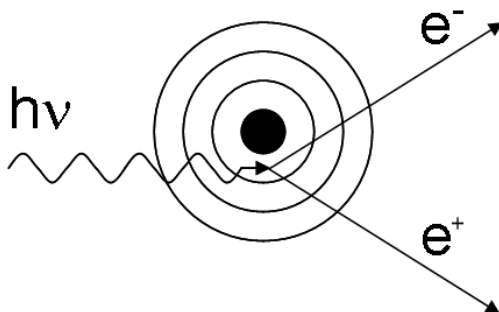
Figure 1.1: An incident gamma ray interacts with the electric field of a nucleus: a larger atomic number (more protons in the nucleus) implies a stronger electric field and greater probability of inducing pair-production. The nucleus absorbs a small amount of momentum in the interaction but its recoil is essentially negligible in comparison to the energy and momentum imparted to the pair of electrons.
