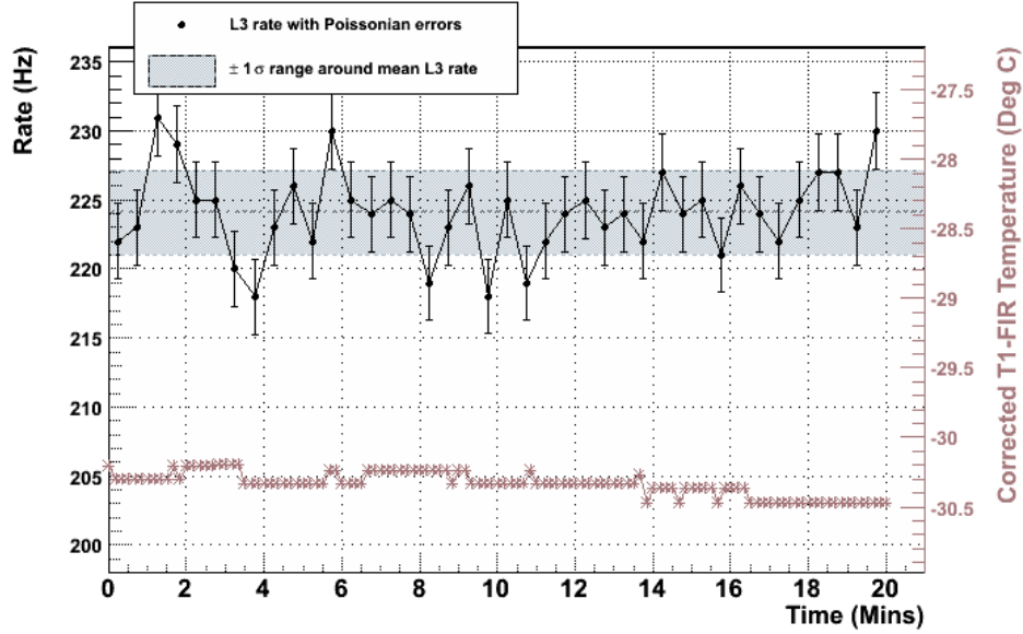
Figure 5.3: L3 rate (upper points) and sky temperature from an FIR pyrometer (lower points) versus time for a single data run (#51535). The fluctuations of the rate are not stochastic at the level of only 1.1\sigma and are therefore consistent with stability. Image credit — plotted by loggen (see main text for a description).
