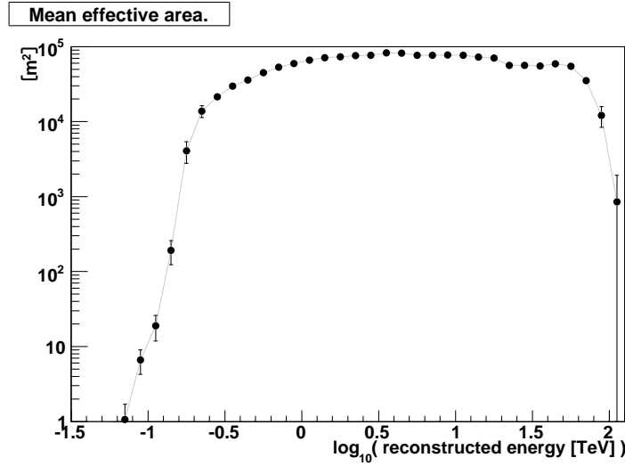
Figure 5.10: The mean effective area shown is the average of the run-wise effective area curves generated by anasum , weighted by the number of events over which each was computed. The errors indicate the range of variation of the effective area between runs: \sim 30\% below the spectral peak and much smaller above it.
