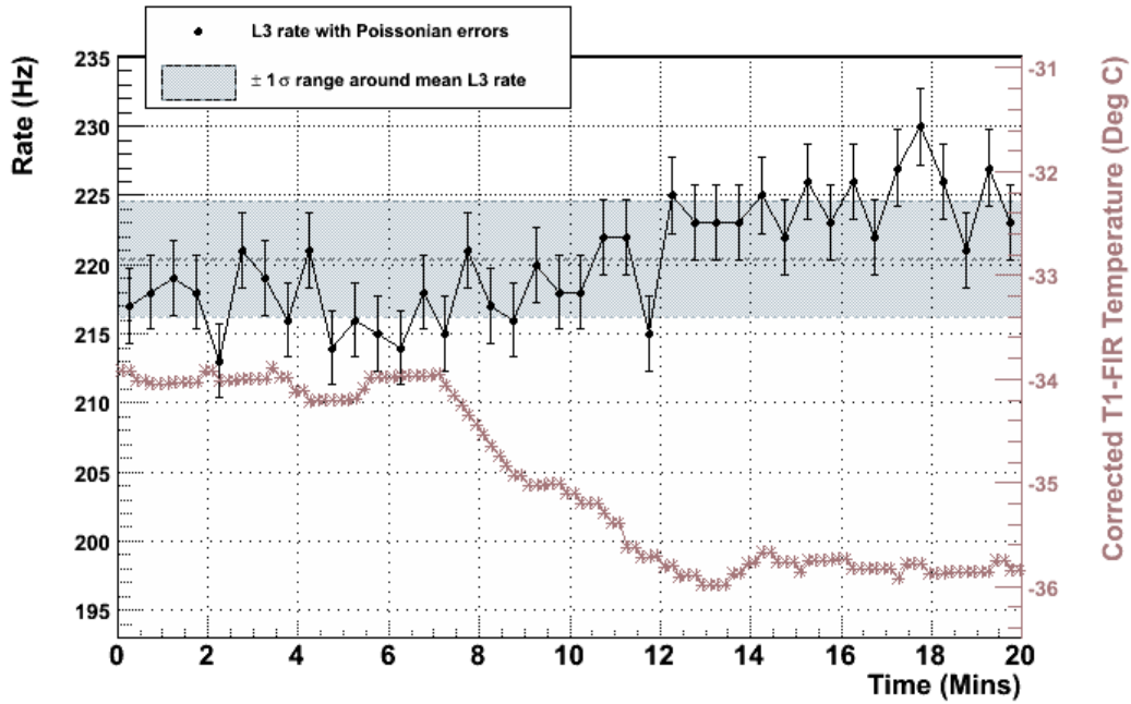
Figure 5.1: L3 rate (upper points) and sky temperature from an FIR pyrometer (lower points) versus time for a single data run (#51588). The non-statistical fluctuation of the rate is correlated with changes in the transparency of the atmosphere. Image credit — plotted by loggen (see main text for a description).
