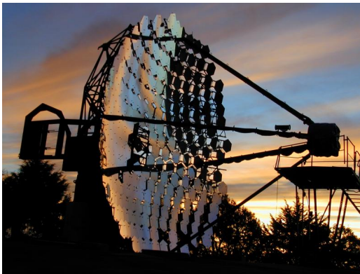
Figure 1.7: The 10-m ACT at the Fred Lawrence Whipple Observatory. Constructed in 1968, it operated with a single-pixel detector ( i.e. as an ACT without imaging capabilities) until 1982 when an imaging camera was installed. The telescope was in operation until 2011. Image credit — D. Horan.
