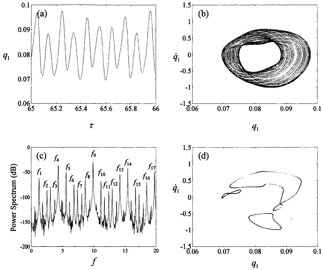
Figure 4-10 (a) Time history, (b) phase plane plot, (c) power spectral density plot and (d) Poincaré map for the system of Figure 4-6 for \mathcal{Z}=15.0 , obtained with N_u = N_v = 6 (quasiperiodic oscillation).
