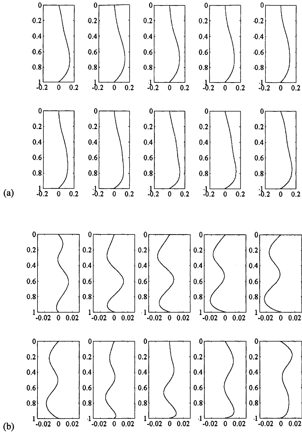
Figure 4-18 Spatial shape of the cylinder of Figure 4-6 at \mathcal{U}=14.6 , periodic oscillation (see also Figure 4-17(b)): (a) total displacement, (b) vibrations around the buckled position.
