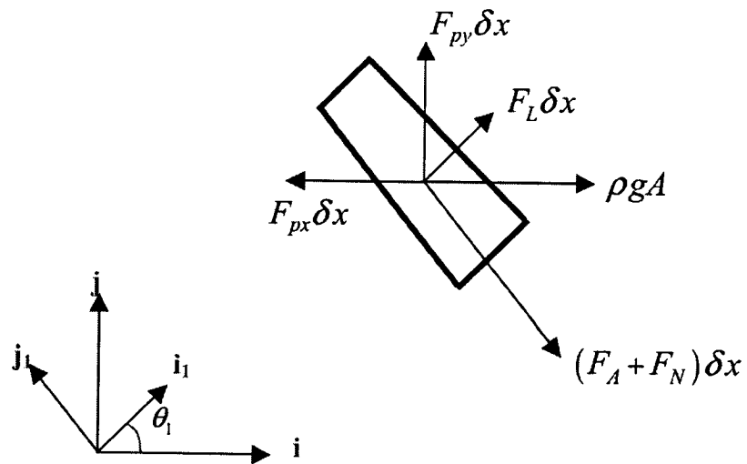
Figure 2-2 An element \delta x of the cylinder, showing the forces acting on it.
