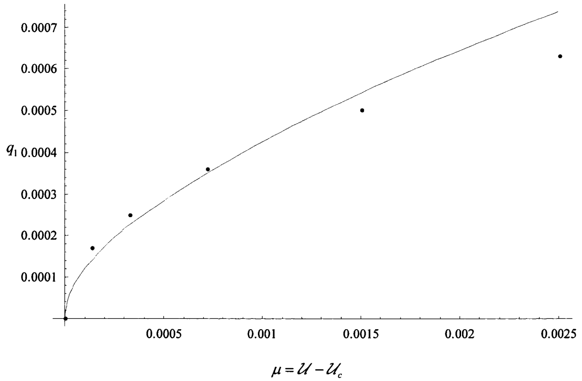
Figure 5-18 Bifurcation diagram for the clamped-hinged cylinder with the physical parameters of Table 5-2 in the vicinity of the pitchfork bifurcation point, obtained with N_u = N_v = 1 using centre manifold reduction (continuous line) and AUTO (dots).
