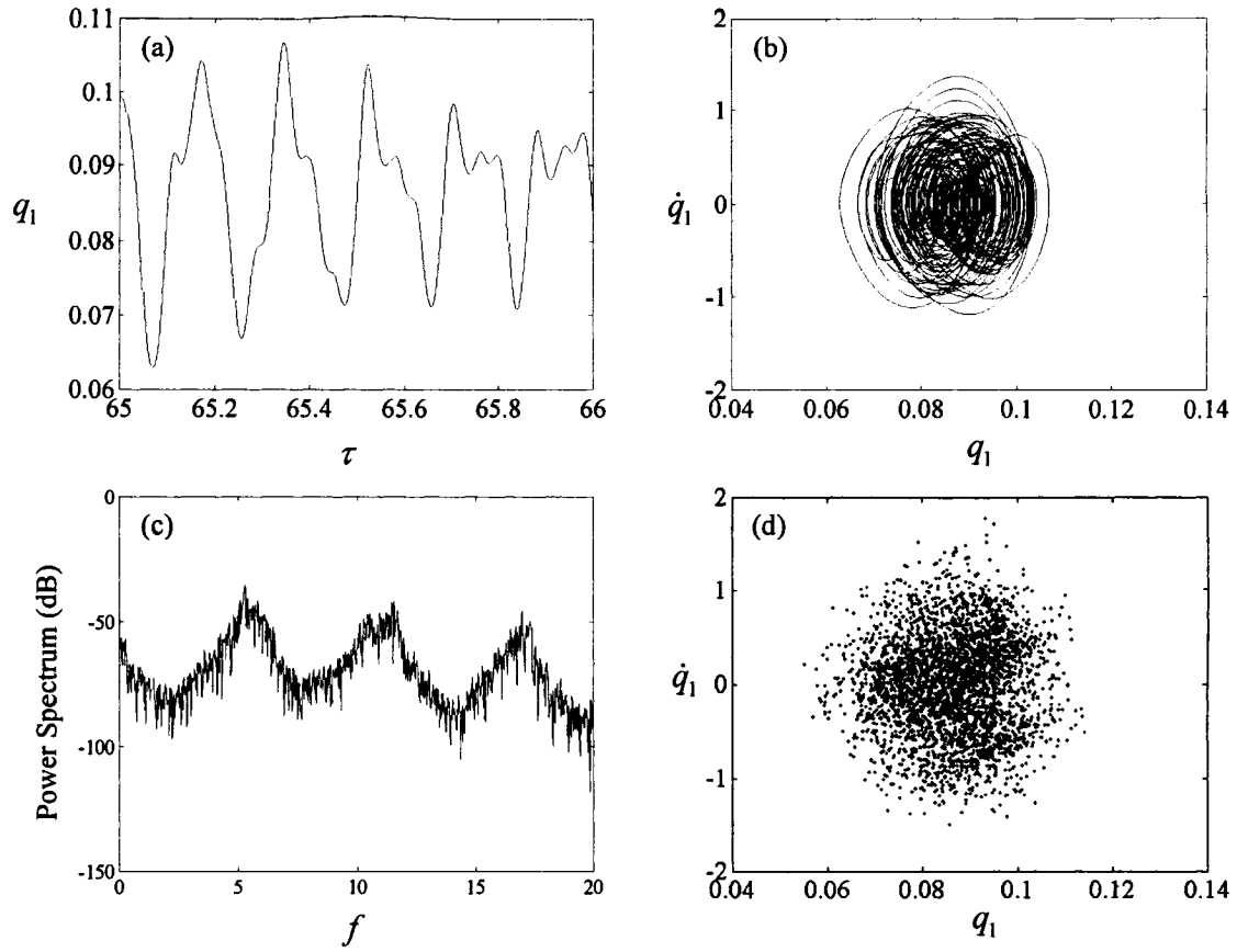
Figure 4-12 (a) Time history, (b) phase plane plot, (c) power spectral density plot and (d) Poincaré map for the system of Figure 4-6 for \mathcal{Z}=16 , obtained with N_u = N_v = 6 (chaotic oscillation).
