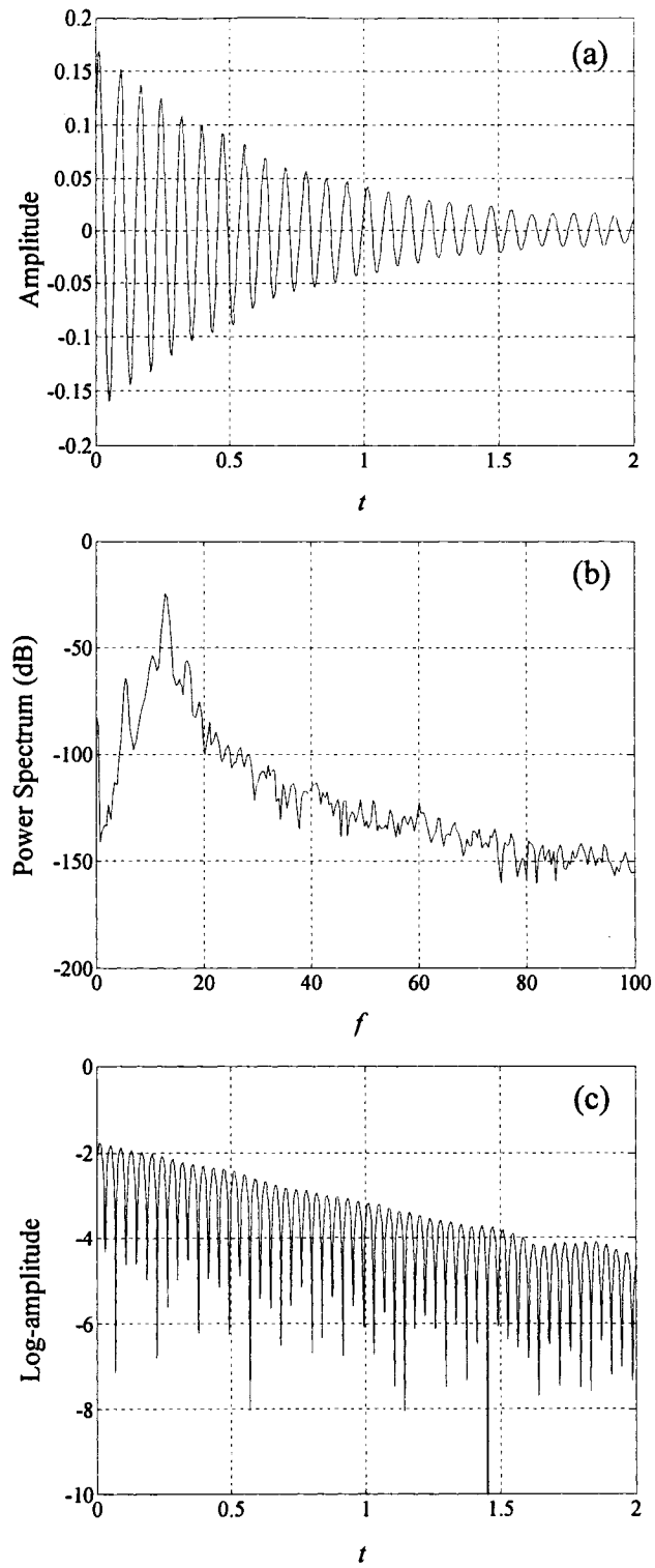
Figure C-3 (a) Time history, (b) PSD plot and (c) the log-amplitude versus time plot of the second-mode oscillation of the clamped-clamped cylinder.
