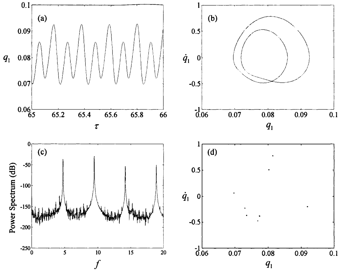
Figure 4-11 (a) Time history, (b) phase plane plot, (c) power spectral density plot and (d) Poincaré map for the system of Figure 4-6 for \mathcal{Z} = 14.6 , obtained with N_u = N_v = 7 (period-2 oscillation).
