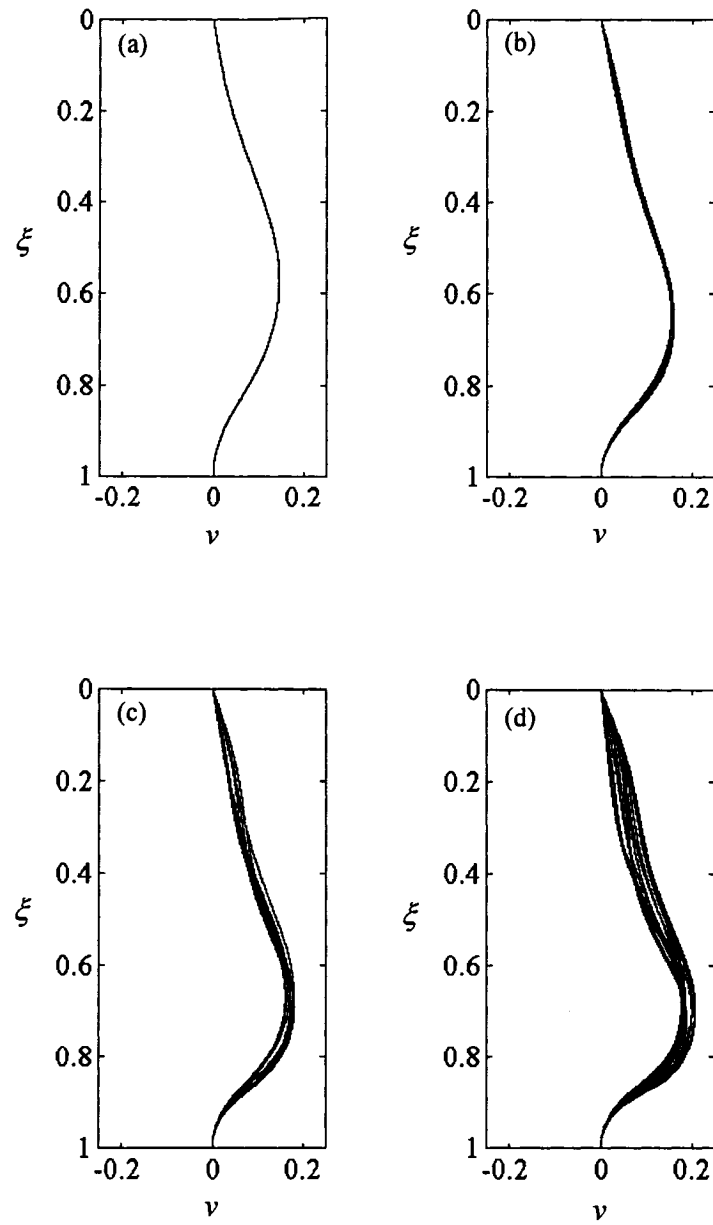
Figure 5-23 Spatial shape of the hinged-clamped cylinder of Figure 5-19 at different flow velocities: (a) U=20 , buckled position, (b) U=22.0 , periodic oscillation, (c) U=24.0 , quasiperiodic oscillation, (d) U=26.0 , chaotic oscillation.
