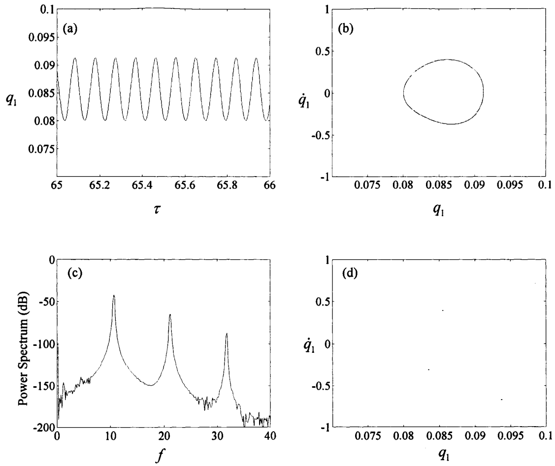
Figure 5-3 (a) Time history, (b) phase plane plot, (c) power spectral density plot and (d) Poincaré map for the system of Figure 5-2 (clamped-clamped cylinder) for \mathcal{U}=21.8 , obtained with N_u = N_v = 6 (periodic oscillation).
