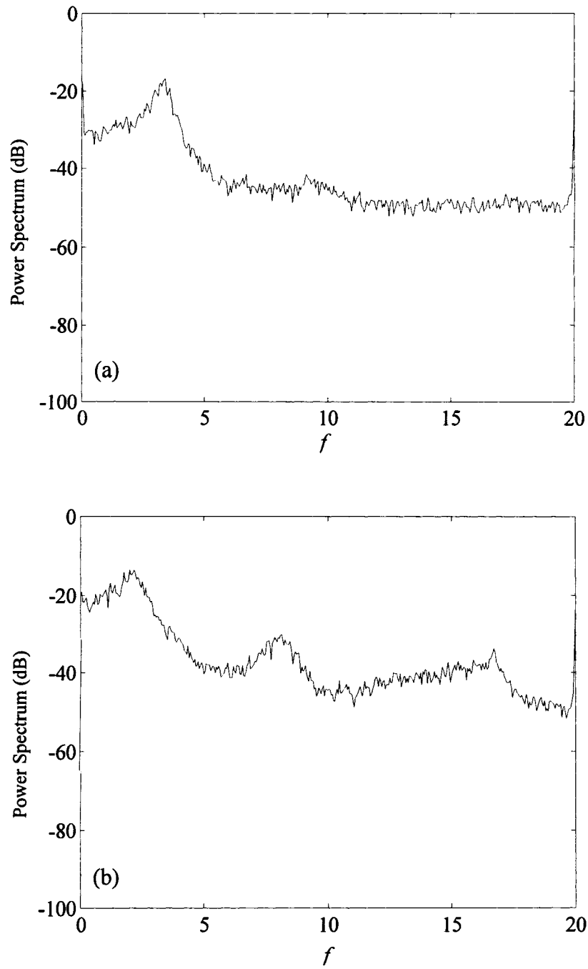
Figure 6-6 PSD plots for the second series of experiments with a clamped-clamped cylinder with no end-sliding and with parameters given in Table 6-1 at (a) L/D = 3.2 , and (b) L/D = 6.1 .
