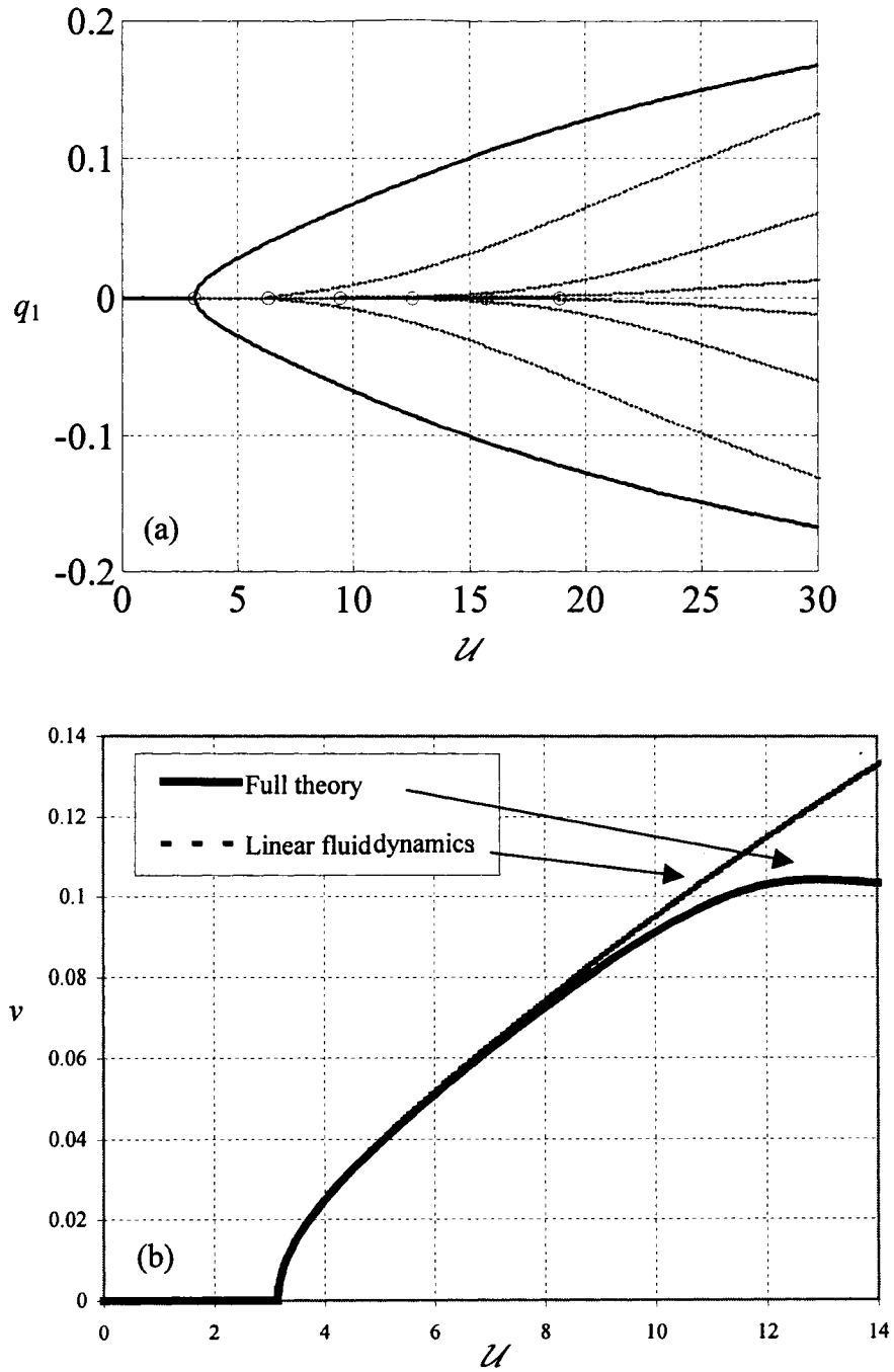
Figure 4-20 (a) Bifurcation diagram for a simply supported cylinder subjected to axial flow using a nonlinear structural model but linear fluid-related forces, for \beta = 0.47 , \delta = 1 , \gamma = 0 , c_n = c_t = 0.025 ; showing no secondary instabilities; (b) comparison between the results found using the full model and the one with linear fluid-dynamic forces.
