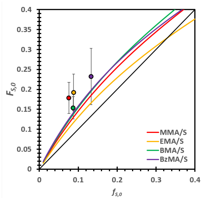
Figure 3: Final styrene composition ( F_S ) versus initial styrene feed ratio ( f_{S,0} ) in the XMA/S block (XMA/S; X = methyl (M), ethyl (E), n-butyl (B) or benzyl (Bz)) chain extensions from poly(styrene- alt -maleic anhydride) (PSMA) macroinitiator. The solid lines represent the theoretical composition of the XMA block estimated using the Mayo-Lewis 47 equation and the reactivity ratios of MMA/S ( r_{MMA} = 0.58 , r_S = 0.55 ) 45 , EMA/S ( r_{EMA} = 0.65 , r_S = 0.29 ) 46 , BMA/S ( r_{MMA} = 0.54 , r_S = 0.64 ) 46 and BzMA/S ( r_{BzMA} = 0.51 , r_S = 0.44 ) 46 . The filled circles represent the estimated styrene composition in the XMA/S block, given the macroinitiator composition and the yield of the second block. The colours of the filled circles match the solid line, which correspond to the legend in the figure.
