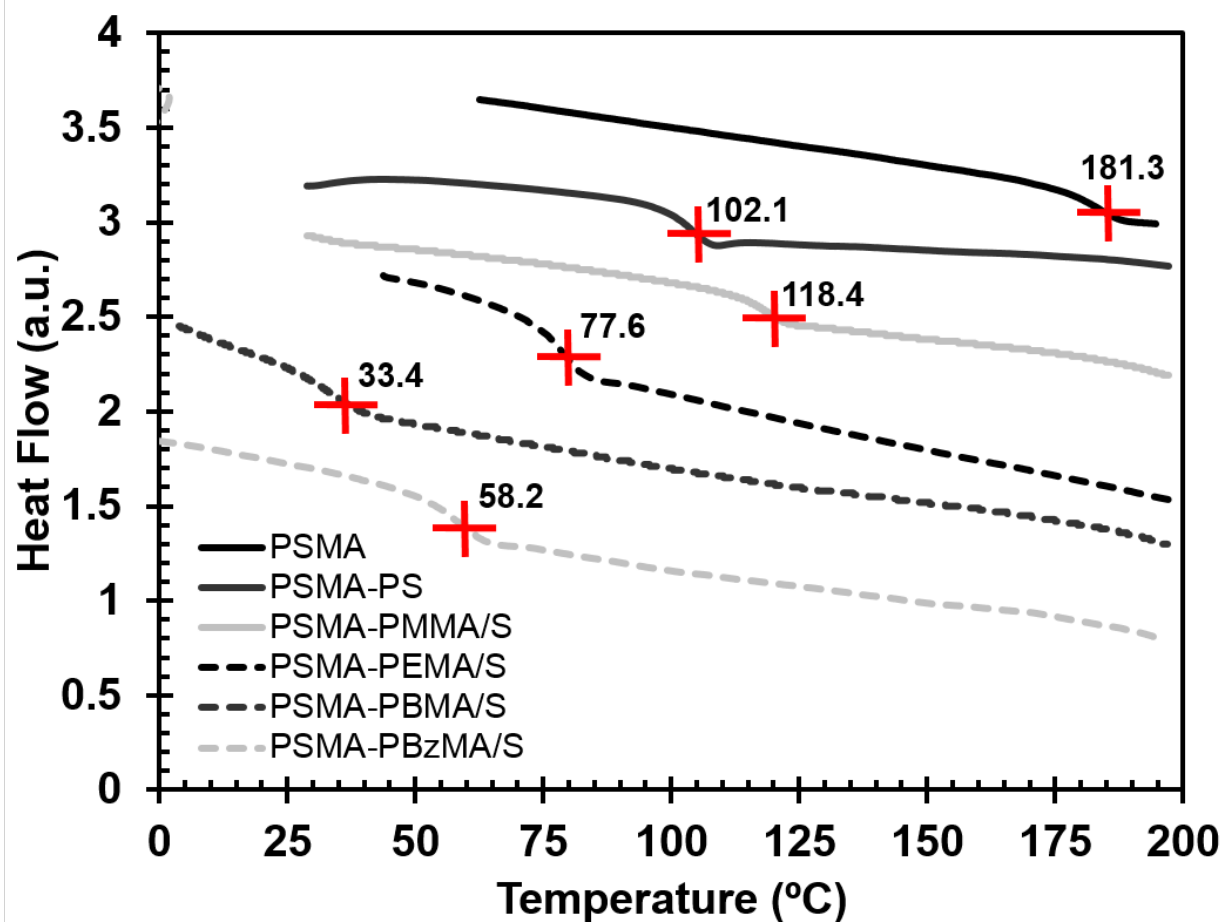
Figure 4: Differential scattering calorimetry (DSC) spectrograms for poly(styrene- alt -maleic anhydride) (PSMA) macroinitiator, PSMA-poly(styrene) (PSMA-PS) and PSMA-X-methacrylate/styrene (XMA/S; X = methyl (M), ethyl (E), n-butyl (B) or benzyl (Bz)) block copolymer. The spectrograms are from the second heat cycle in a heat/cool/heat experiment. All formulations and characterization data are summarized in Table 1 and Table 2, respectively.
