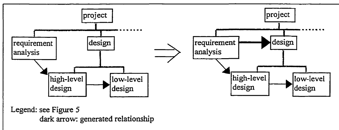
Figure 15 - Generating the relationship "activity precedes activity"
