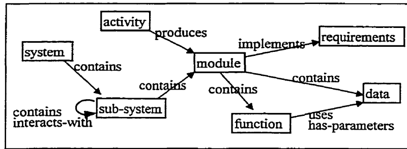
Figure 7 - An instance of the entity-relationship schema for product modeling
