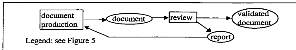
Figure 13 - Information-flow aspect of the analyst's view
