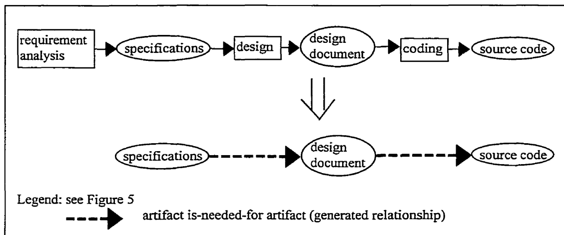
Figure 18 - Generating dependencies from information flow aspect
