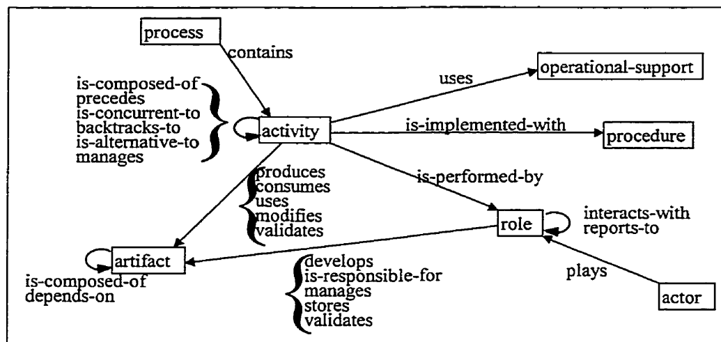
Figure 4 - An instance of the entity-relationship schema for process modeling
