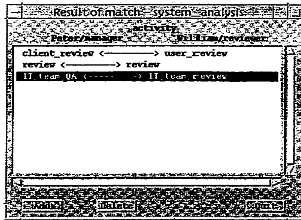
Figure 58 - Final matches for the activities between Peter's and William's views
