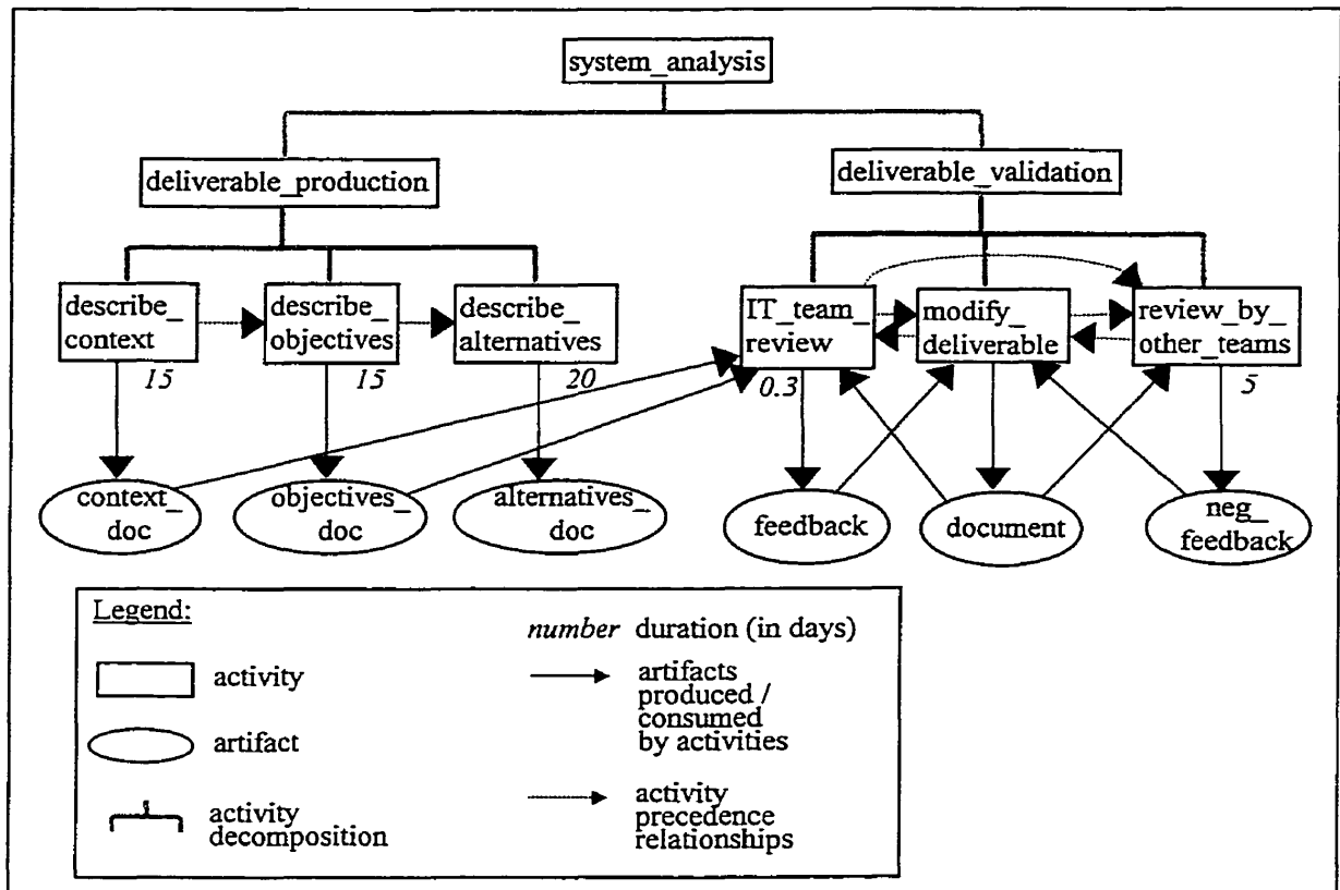
Figure 25 - Bob's partial view
