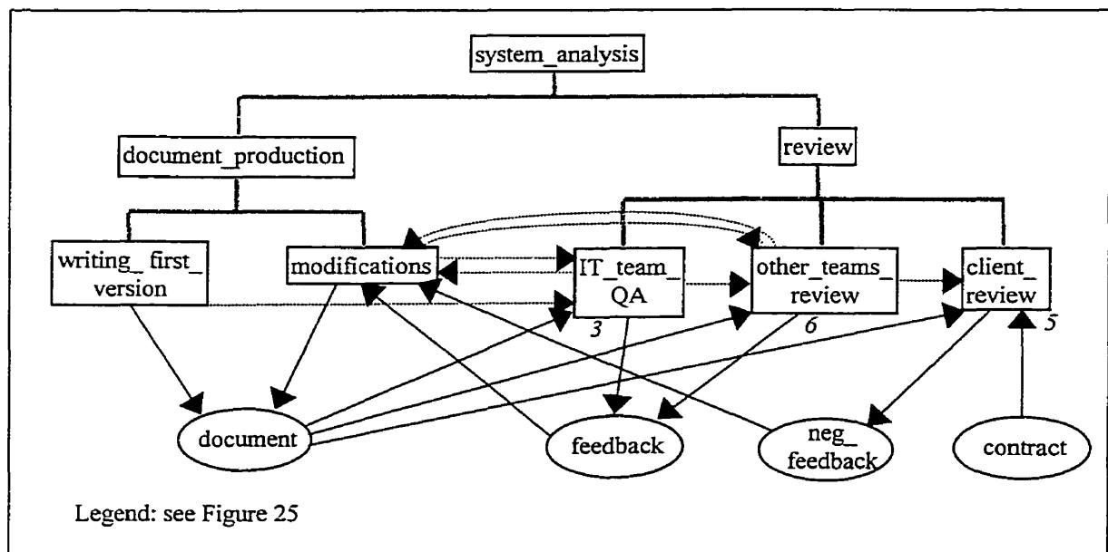
Figure 26 - Peter's partial view
