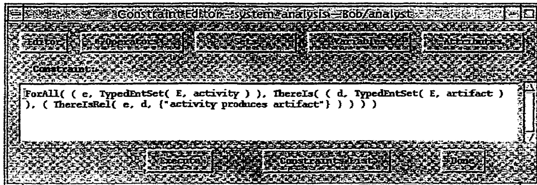
Figure 43 - Example of constraint specification
