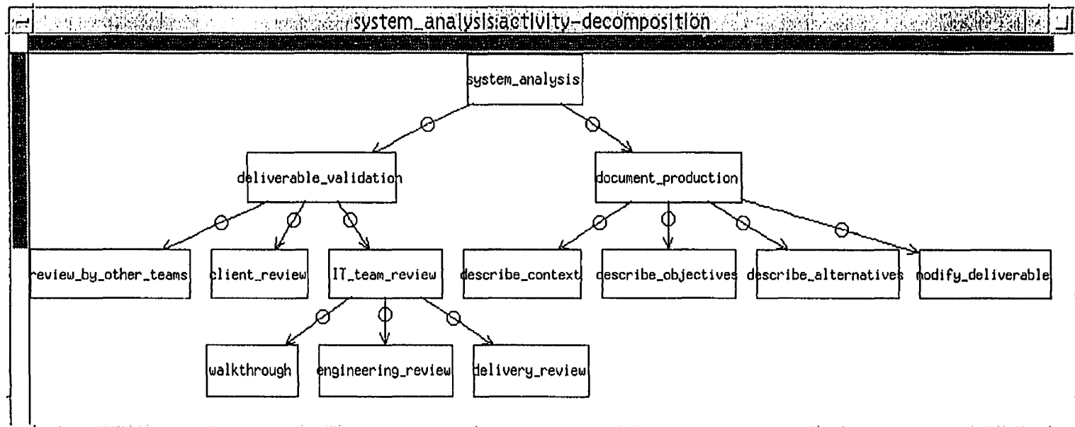
Figure 93 - Activity decomposition aspect of the final model
