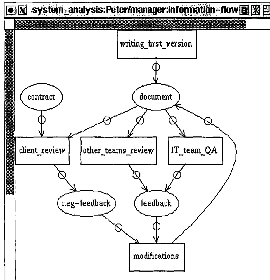
Figure 86 - Peter's information flow aspect
