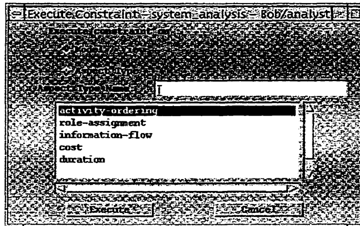
Figure 44 - Choosing the aspect on which the constraint is evaluated
