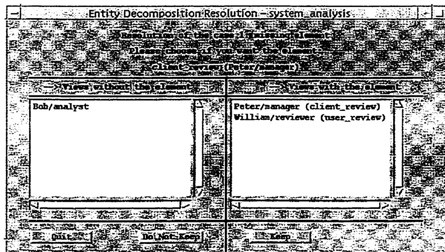
Figure 65 - Resolving when an entity is missing in some views
