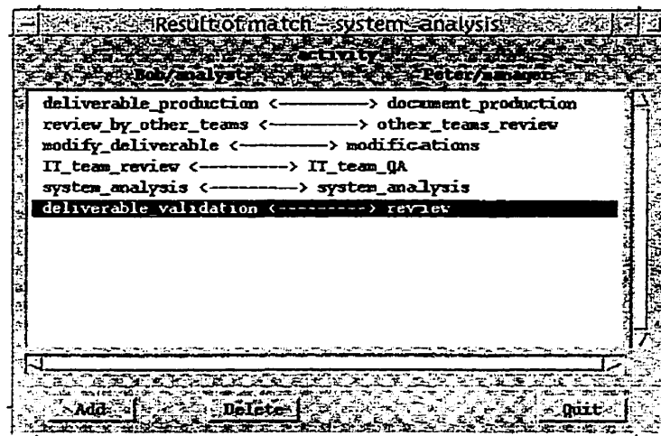
Figure 59 - Final matches for the activities between Bob's and Peter's views
