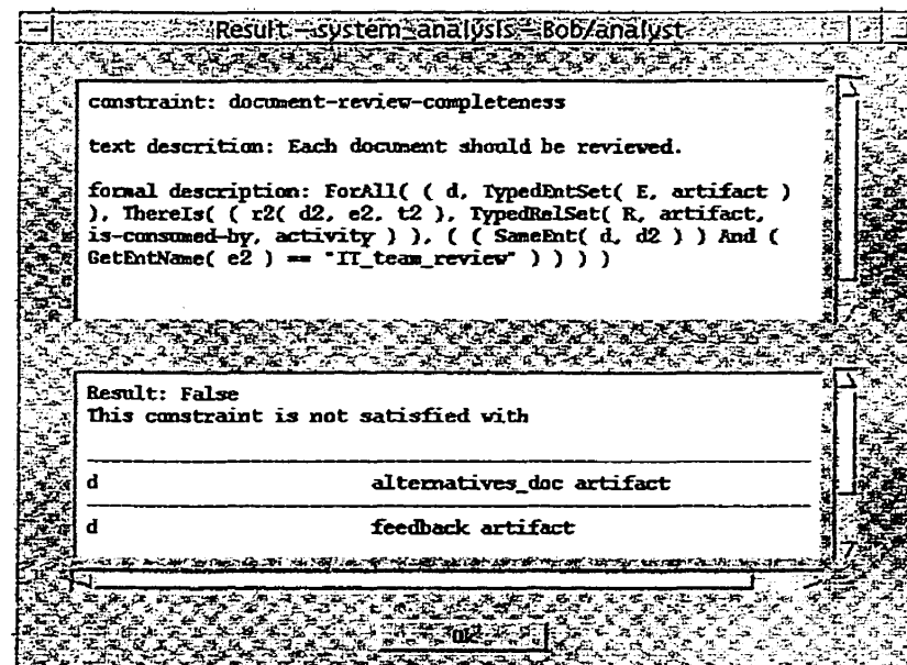
Figure 48 - Result of a constraint related to the meaning of the information
