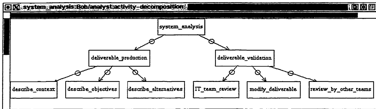
Figure 42 - Activity decomposition aspect elicited for Bob's view
