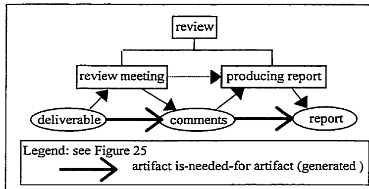
Figure 74 - Sam's view modified (including generated relationships)
