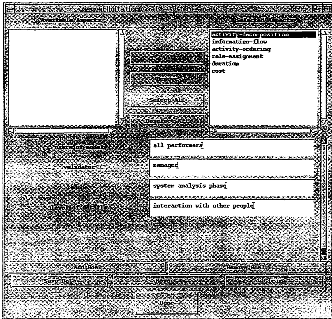
Figure 31 - Specifying elicitation goals
