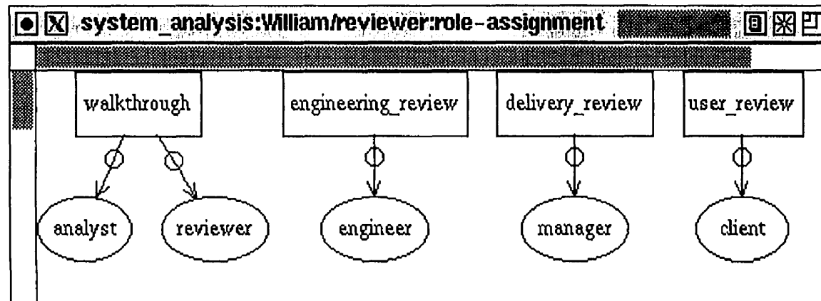
Figure 92 - William's role assignment aspect
