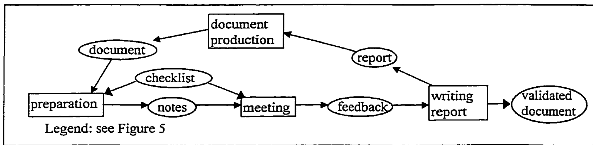
Figure 8 - Example of an aspect (information-flow aspect)
