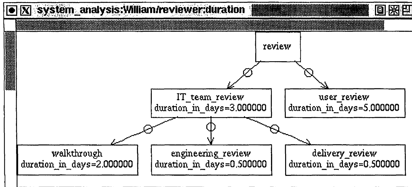
Figure 90 - William's activity duration aspect
