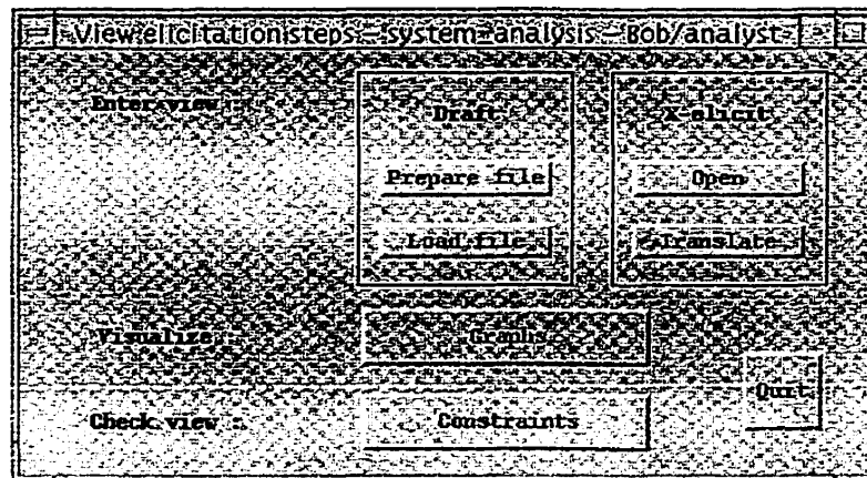
Figure 36 - Steps for eliciting a view
