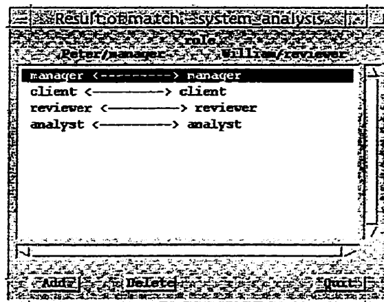
Figure 54 - Result of matching the roles between Peter's and William's views
