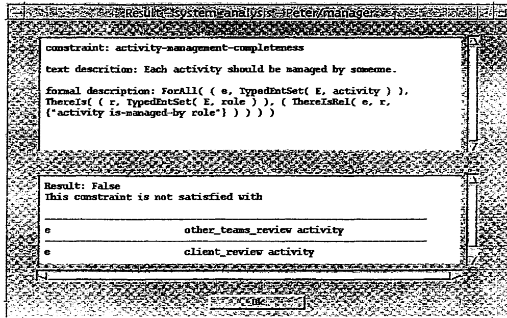
Figure 47 - Result of the evaluation of a constraint that is not satisfied
