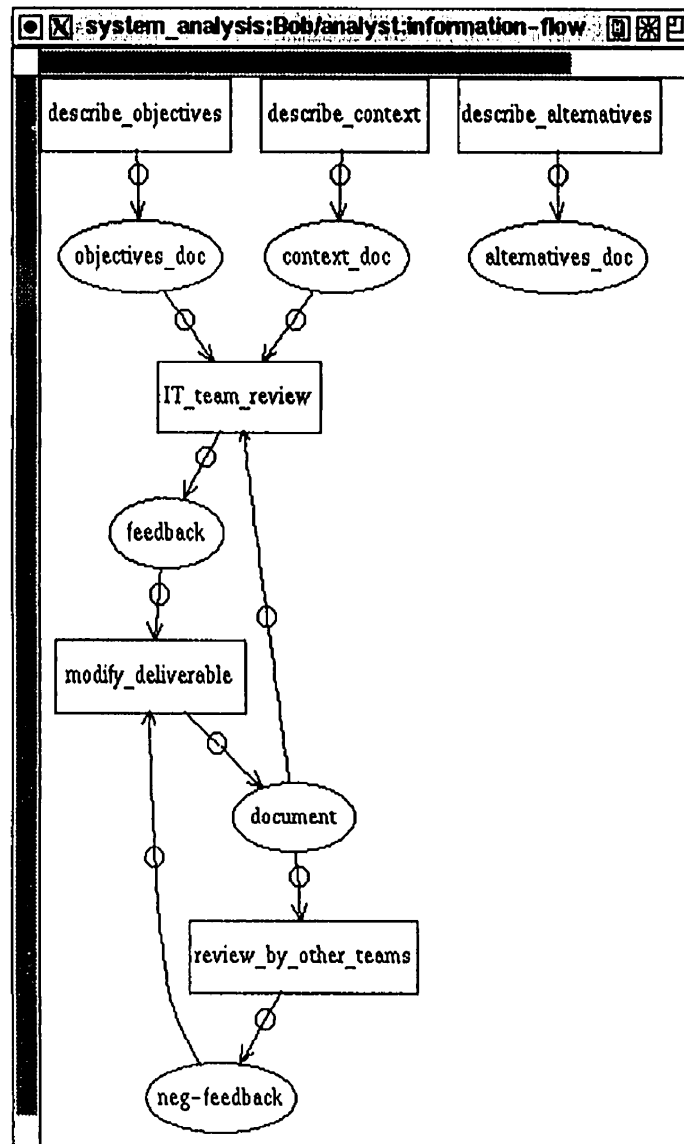
Figure 80 - Bob's information flow aspect
