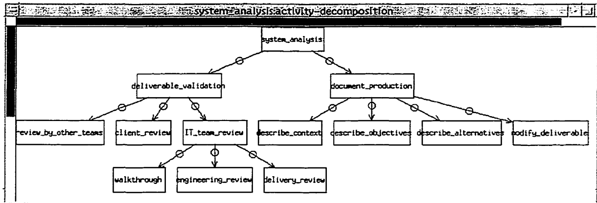
Figure 66 - Final model after resolving the inconsistencies (activity decomposition only)
