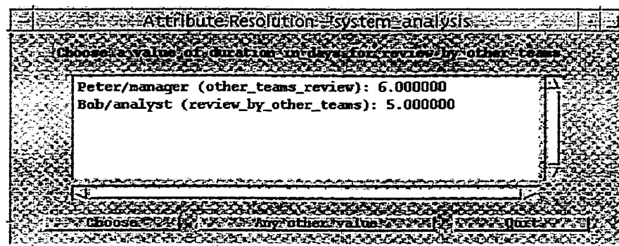
Figure 68 - Resolving an inconsistency in the attributes
