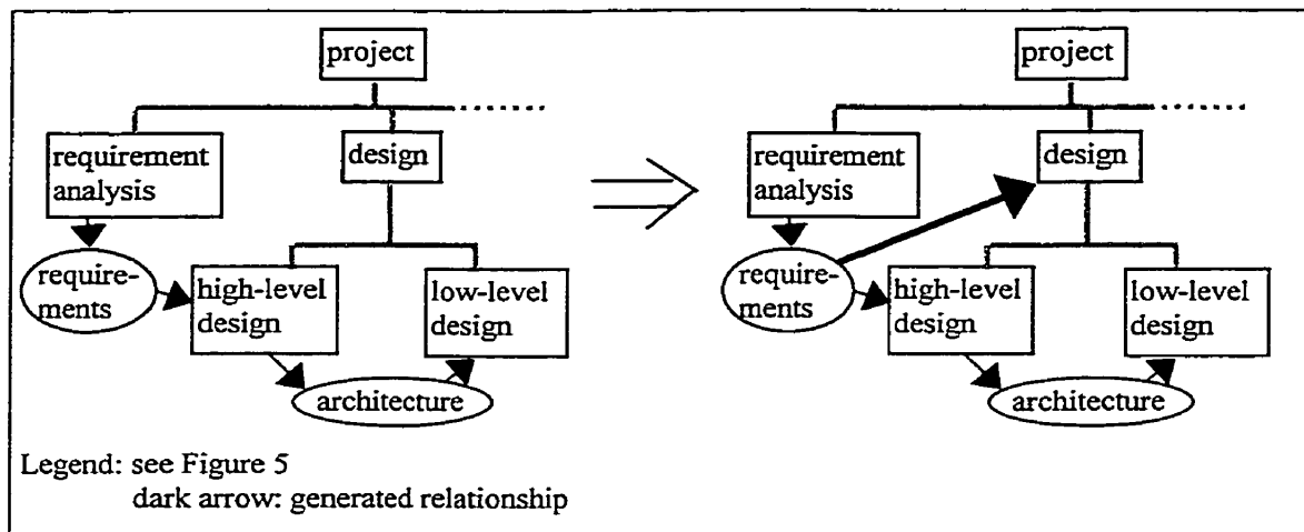
Figure 16 - Generating information flow relationships
