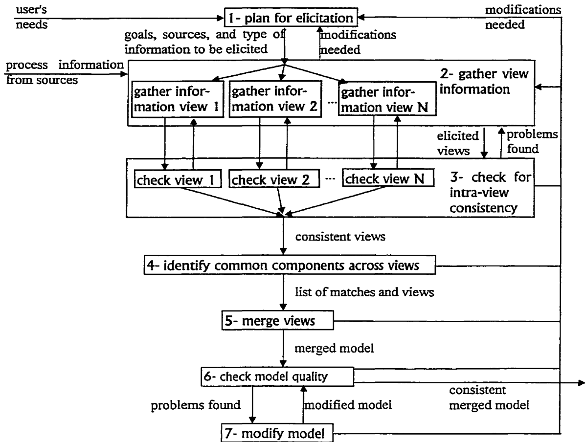
Figure 24 - Elicitation steps (dataflow)
