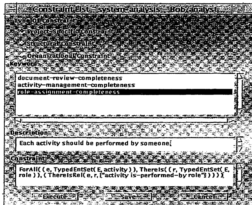
Figure 49 – Selecting a constraint from a list
