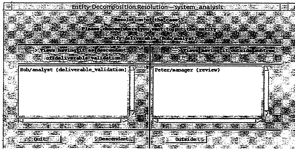
Figure 63 - Resolving when an entity is under different subtrees
