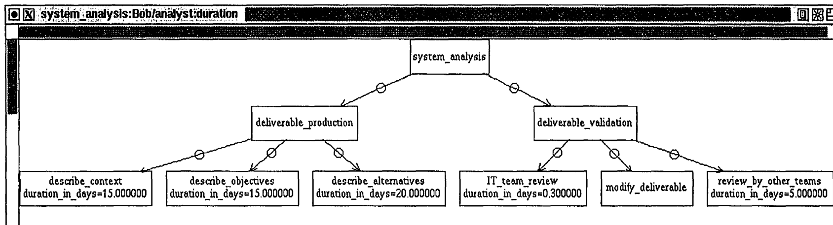
Figure 79 - Bob's activity duration aspect
