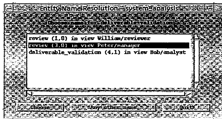
Figure 67 - Resolving an inconsistency related to entity names
