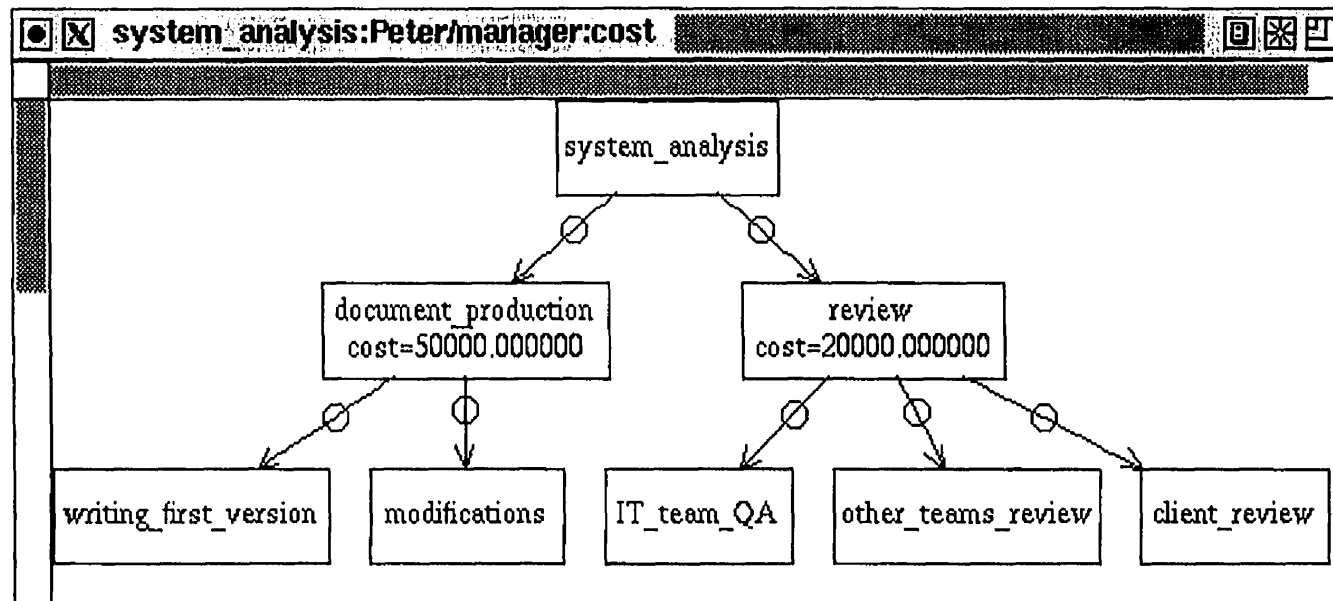
Figure 84 - Peter's cost of activity aspect
