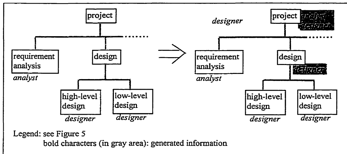
Figure 14 - Generating the relationship "activity is-performed-by role"
