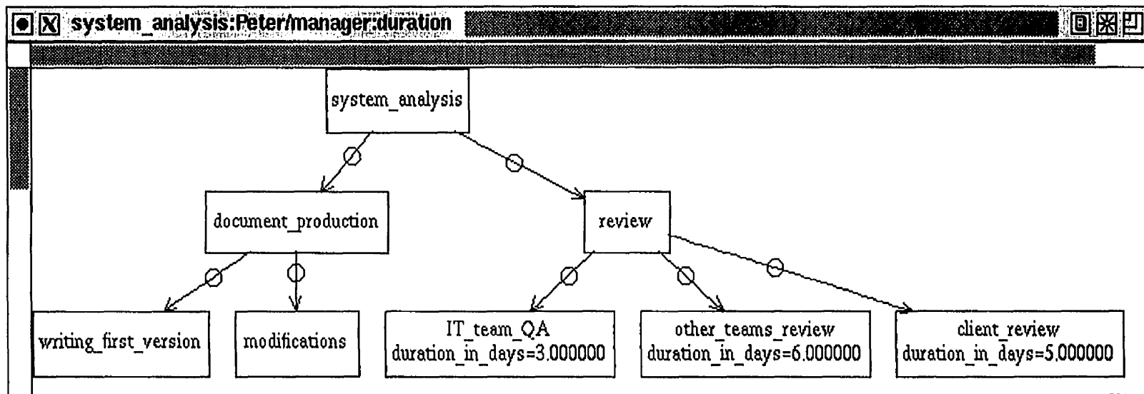
Figure 85 - Peter's activity duration aspect
