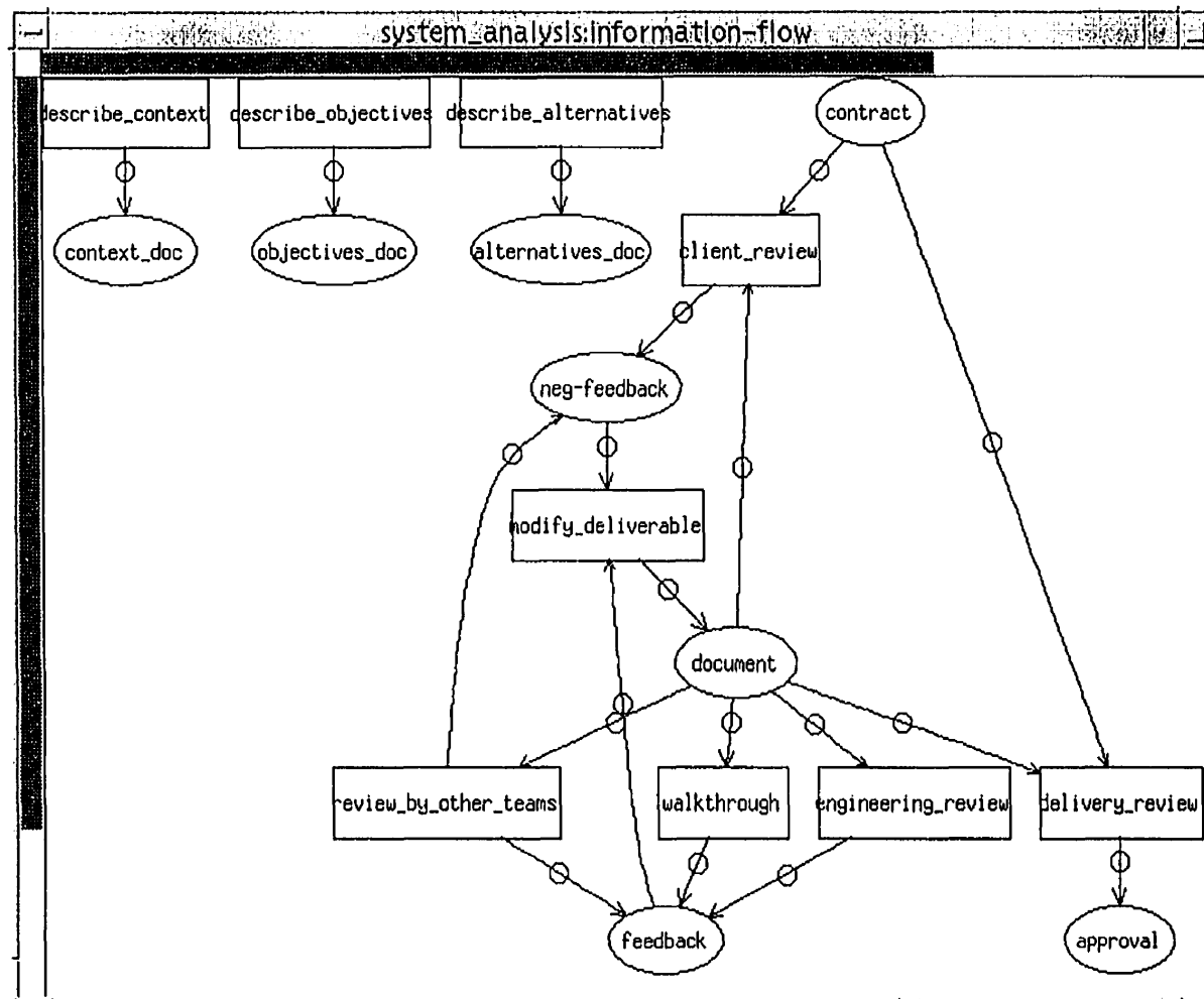
Figure 95 - Information flow aspect of the final model
