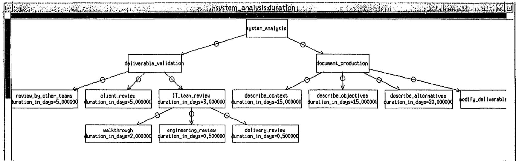
Figure 94 - Activity duration aspect of the final model
