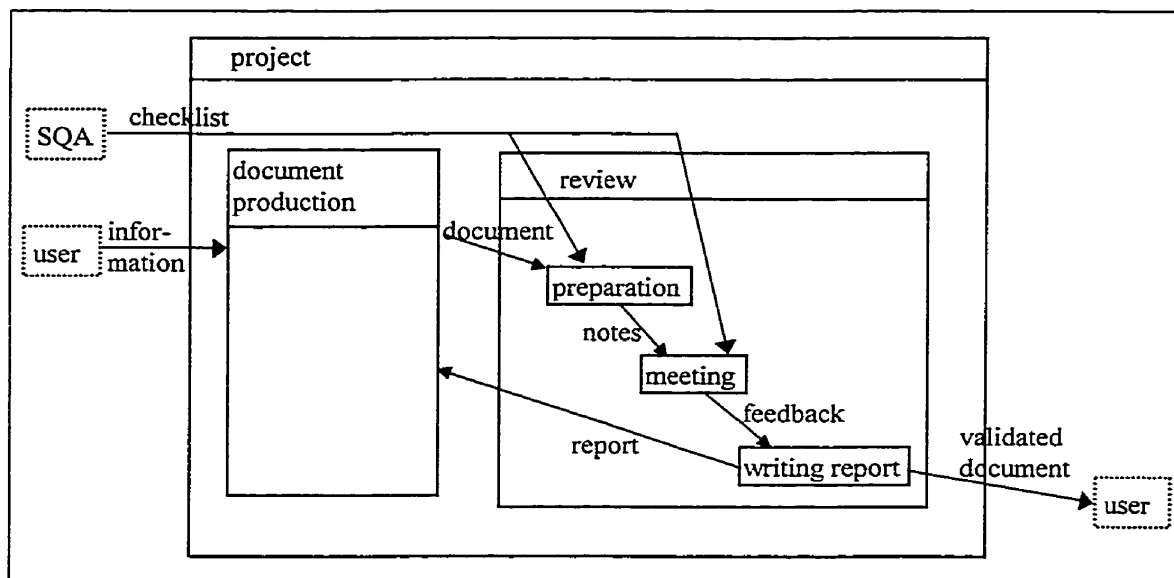
Figure 1 - Functional perspective of a review process
