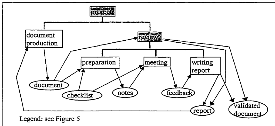
Figure 10 - Example of a view: the reviewer's view
