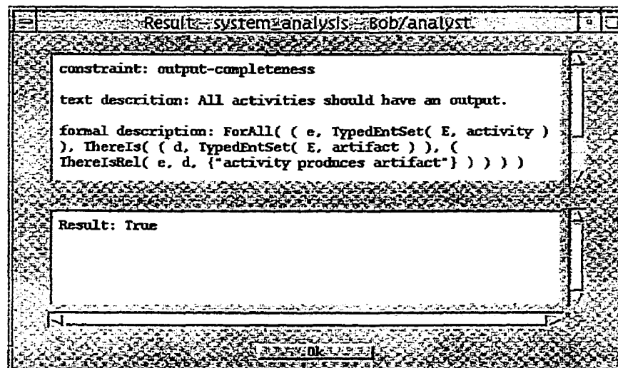
Figure 45 - Result of the evaluation of a constraint that is satisfied
