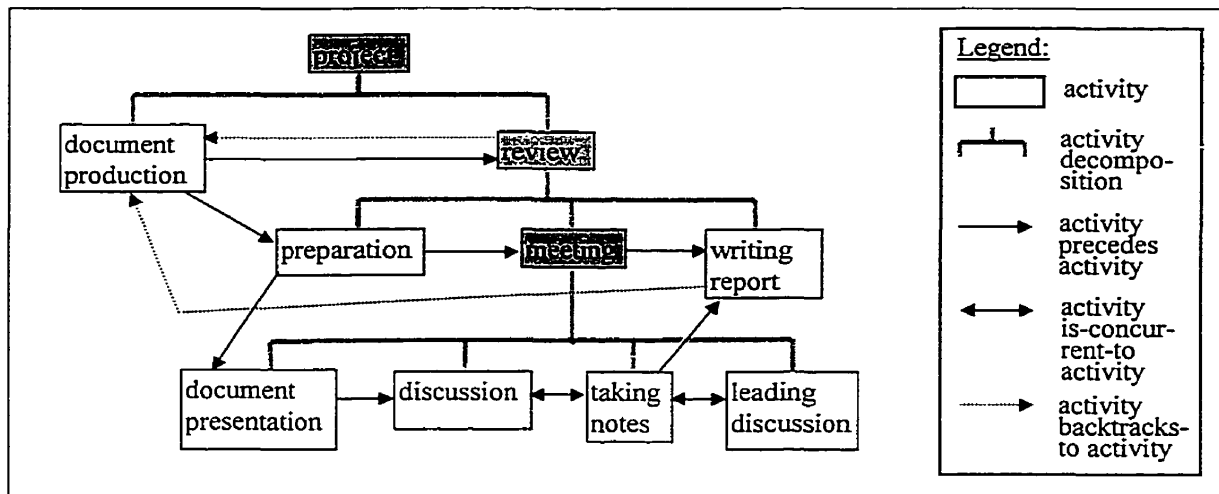
Figure 6 – Modeling behavioral process information
