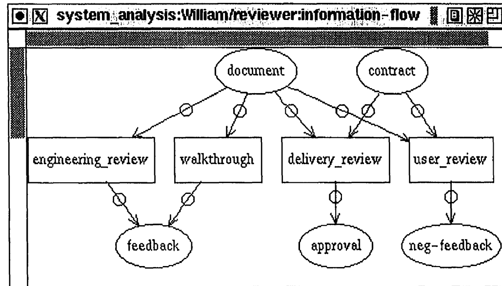
Figure 91 - William's information flow aspect
