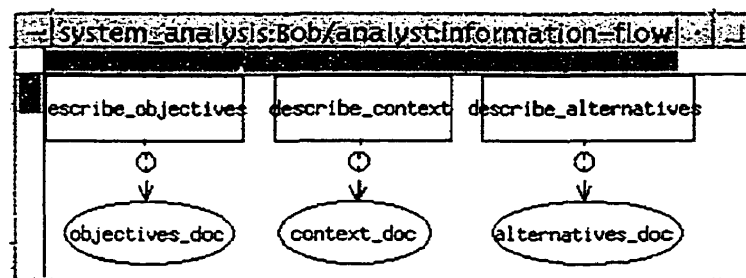
Figure 39 - Bob's information flow aspect (incomplete) as specified in Figure 38
