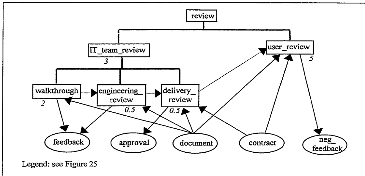
Figure 27 - William's partial view
