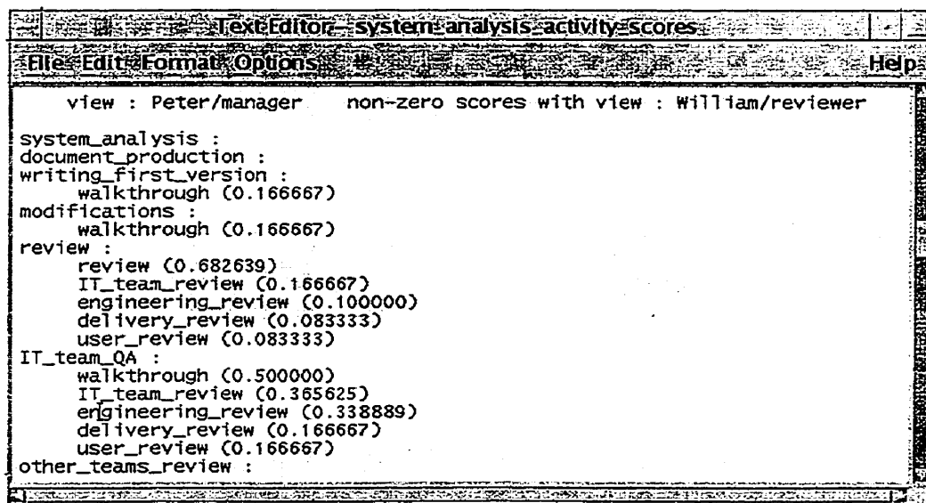
Figure 57 - Report generated by the matching algorithm showing similarity scores 17
