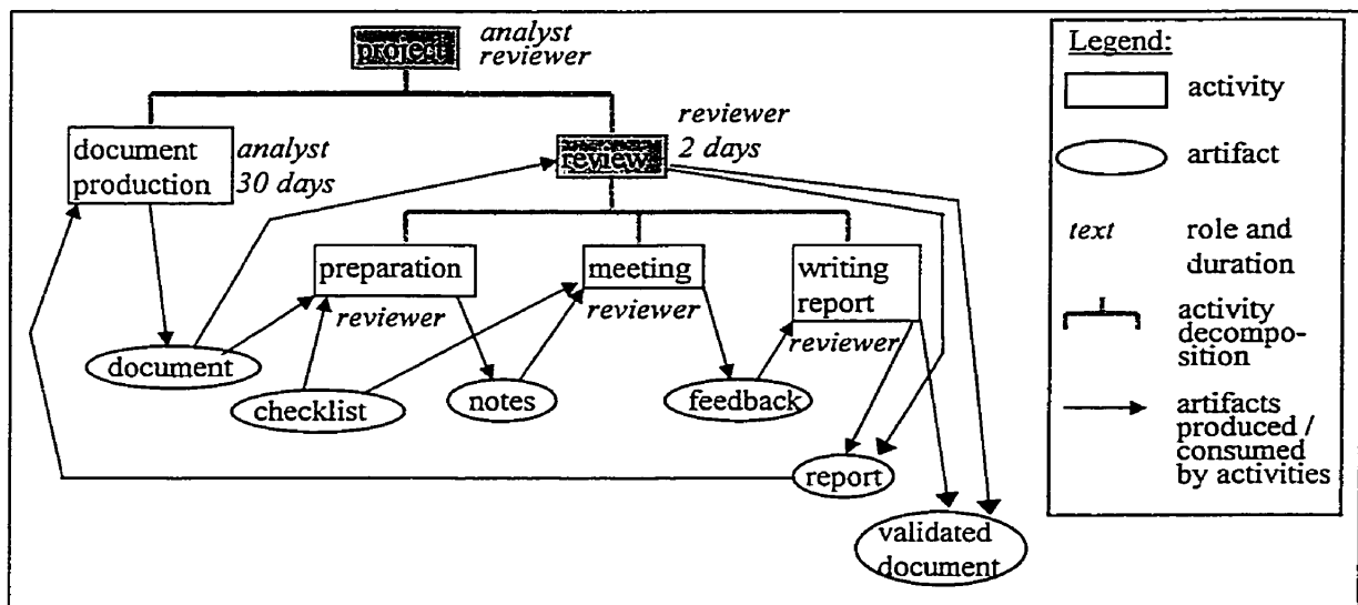
Figure 5 – Example of an entire model
