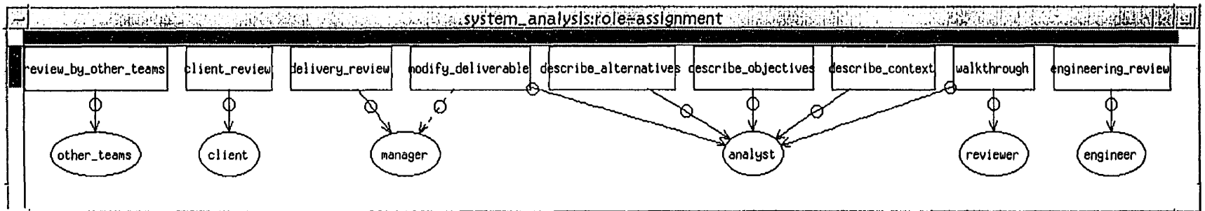
Figure 96 - Role assignment aspect of the final model
