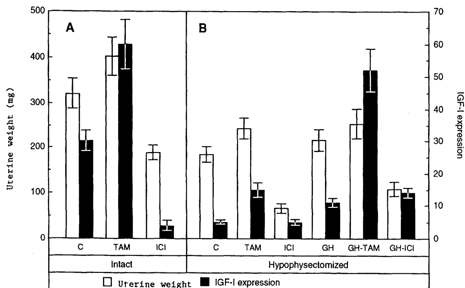
Fig. 1. (A) Effect of tamoxifen and ICI 182780 on uterine weight and uterine IGF-I expression in intact female rats. (B) Effect of tamoxifen and ICI 182780 on uterine weight and uterine IGF-I expression in hypox and hypox, growth hormone-replaced female rats. Treatments were administered as described in "Materials and Methods." Gene expression was quantified by densitometric scanning of individual Northern blots obtained from individual animals in each experimental group. Mean values \pm SD (bars) are plotted; each experimental group comprised 4 animals. C, control.
