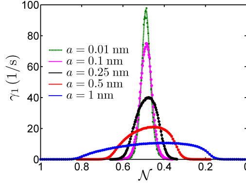
FIGURE 2–4: The first peak in the dot is theoretically calculated for several oscillation amplitudes. Large oscillation amplitudes (i.e. Aa \gg k_B T ) enhance the asymmetric peak lineshape [53]. Image courtesy of Steven Bennett.
