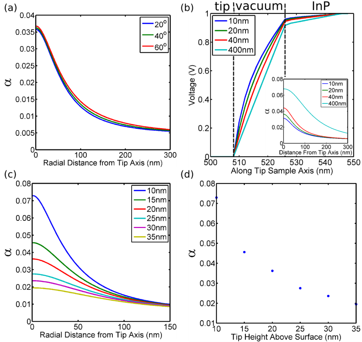
FIGURE 4–10: Change in \alpha for different tip cone angles (a) and radii (b). In (a) the tip radius is 20 nm and in (b) the tip cone angle is 40°. For (a) and (b) the tip-sample gap is 20 nm. The change in \alpha along the surface for different tip-sample distances (c) for a tip with 20 nm radius and 40° cone angle. In (d) the value in (c) directly underneath the tip is plotted to show how \alpha changes with tip-sample gap.
