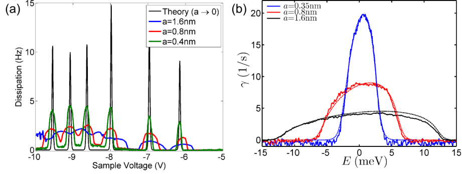
FIGURE 4–18: (a) Three spectra at different oscillation amplitudes (in the strong coupling regime), taken over the same dot, are compared to the theoretically displayed thermally limited peaks in black (which represents weak coupling). With increasing oscillation amplitude, the peaks clearly skew away from the center of the shell. (b) Comparison between strong coupling theory and data for the first peak for different oscillation amplitudes [53]. All data shown was taken at 5 K. (b) is courtesy of Steven Bennett.
